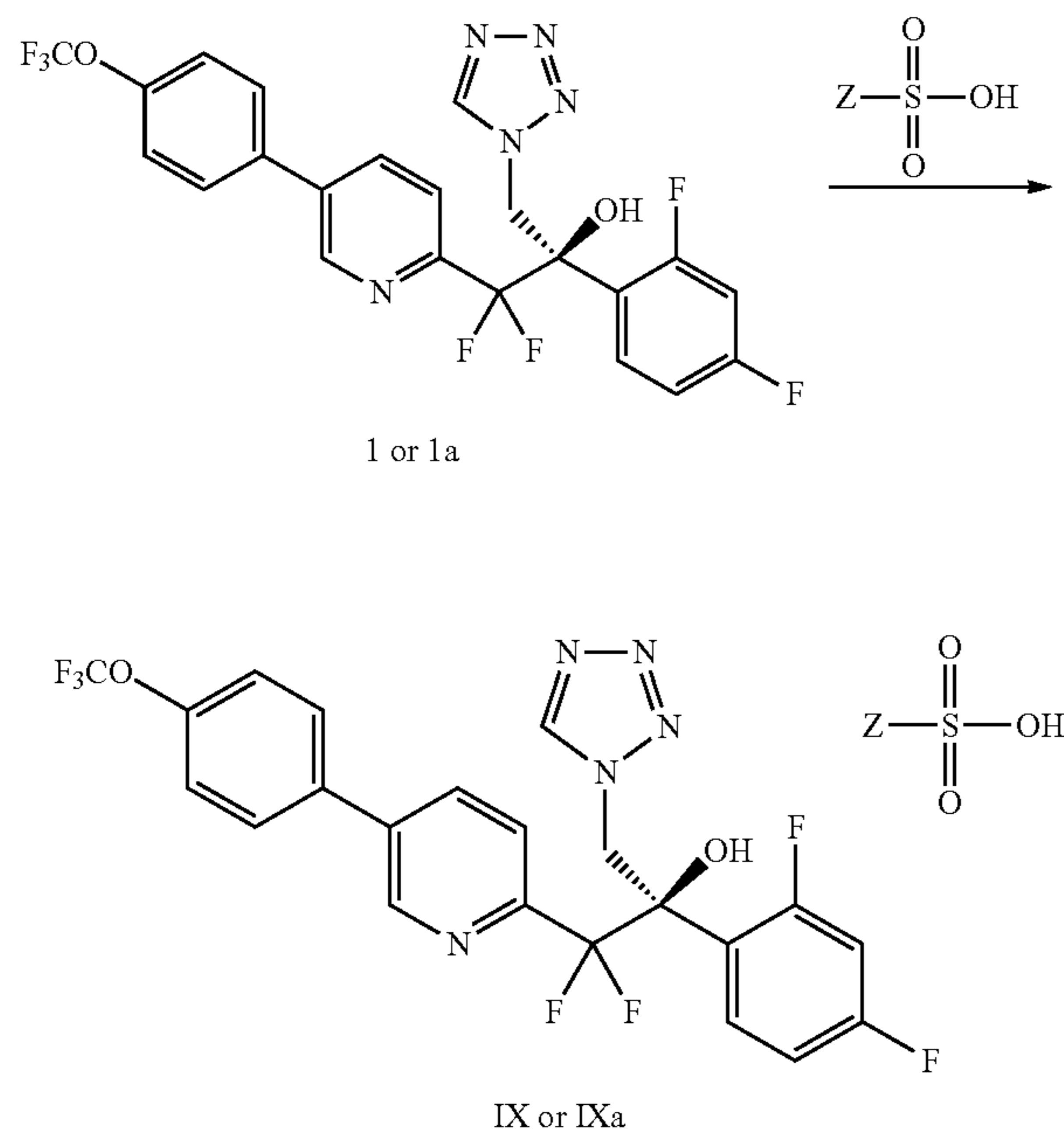
Scheme 4. Synthesis of a Sulfonic Acid Salt of Compound 1 or 1a
