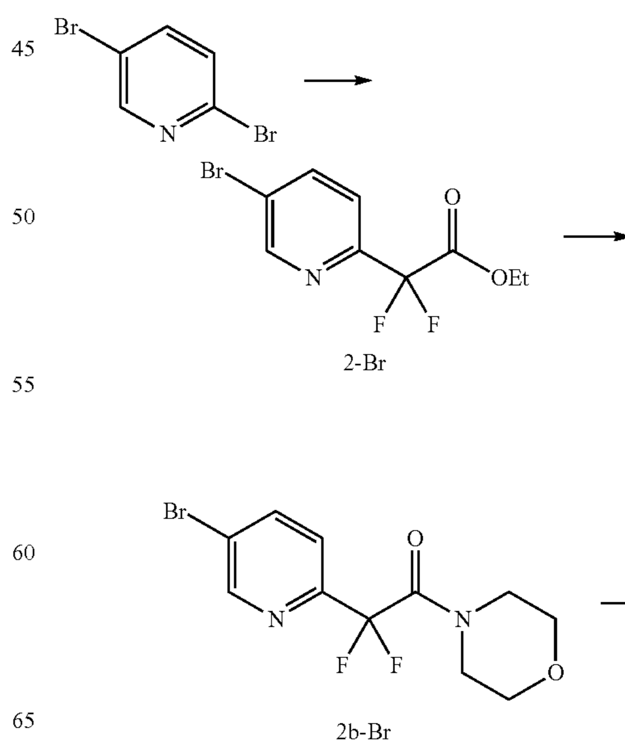
Scheme 1. Synthesis of ketone 3-Br
