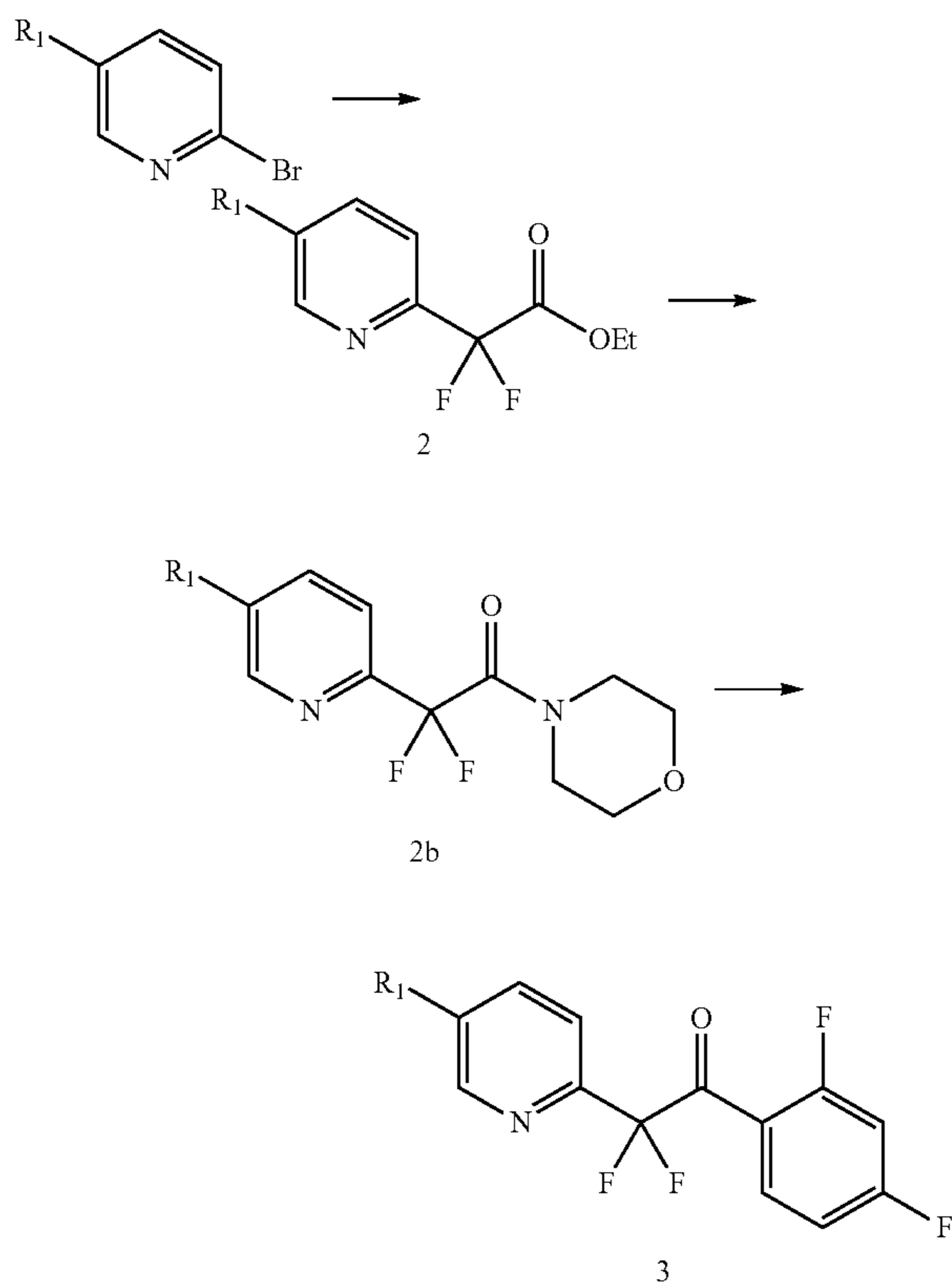
Scheme 2. Synthesis of ketone 3
