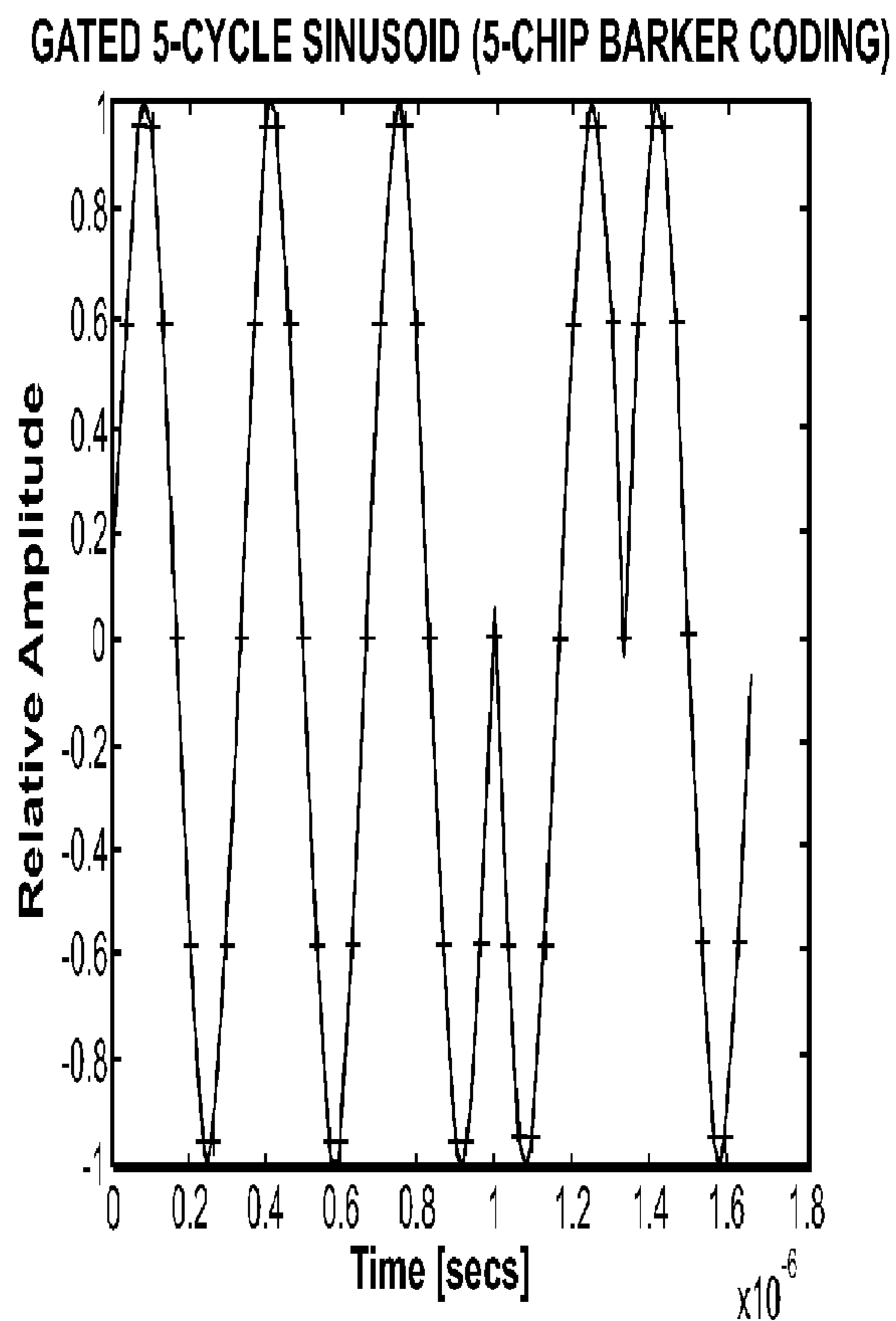
GATED 3 MHz SINUSOID WITH 5-CHIP BARKER CODING [1 1 1 -1 1]
