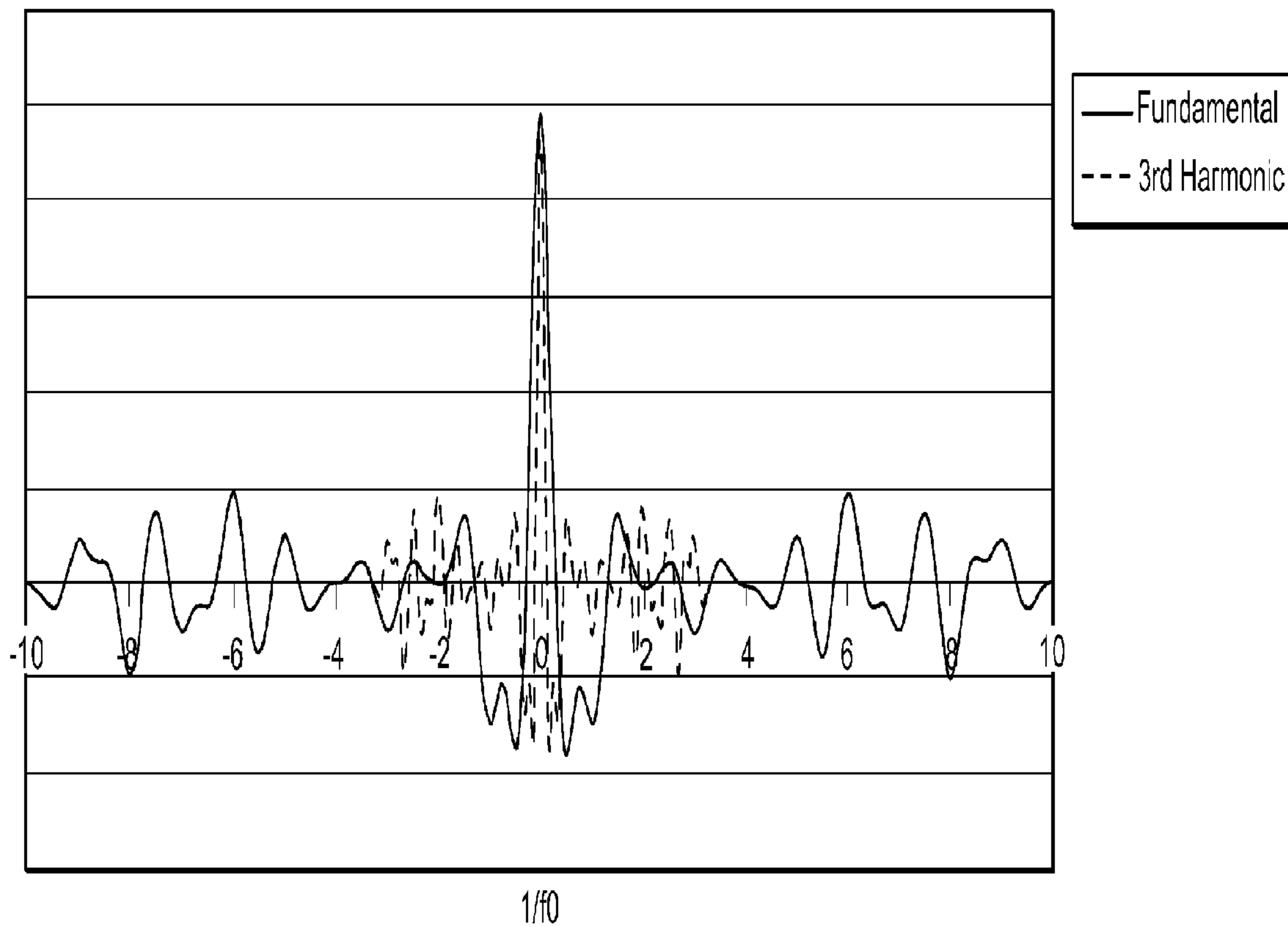
Autocorrelation of match filter templates of 1st Golay code
