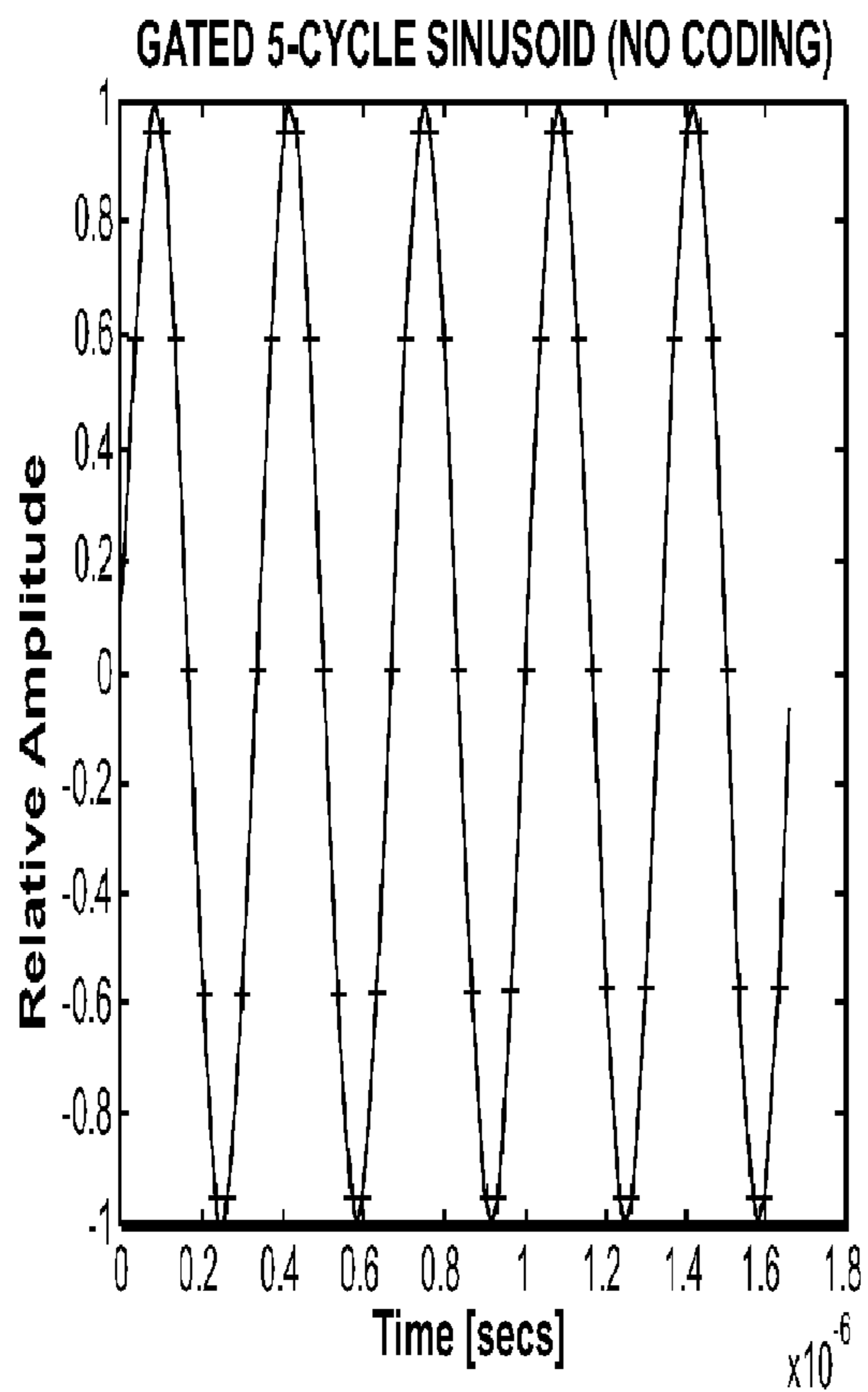
5-CYCLE 3 MHz SINUSOID WITHOUT SPREAD-SPECTRUM CODING
