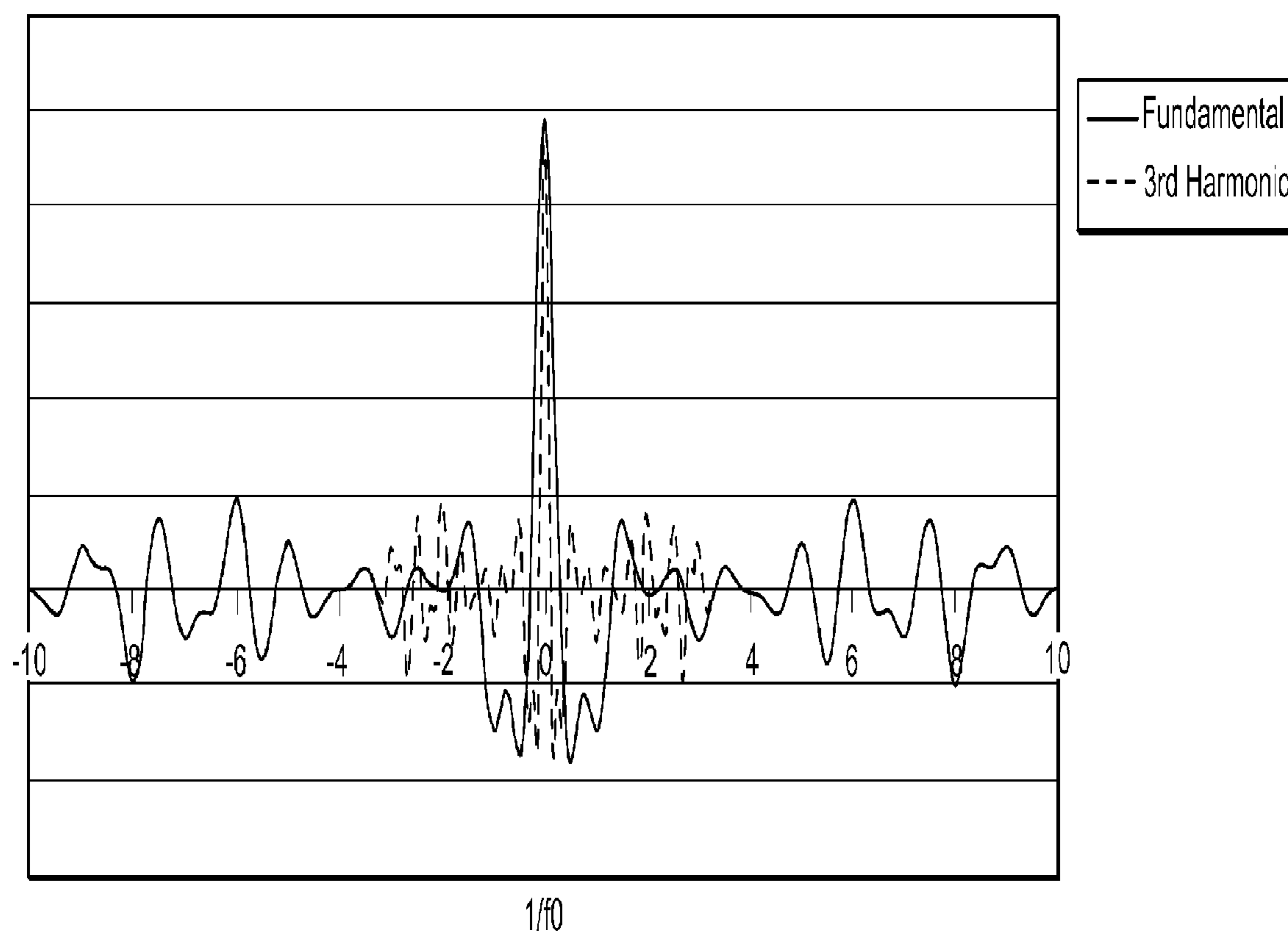
Autocorrelation of match filter templates of 1st Golay code
