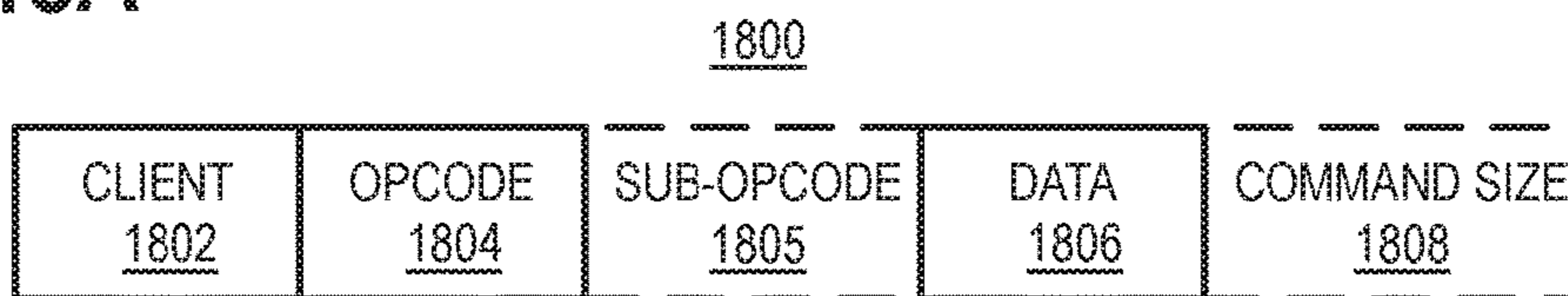
FIG. 18A GRAPHICS PROCESSOR COMMAND FORMAT
