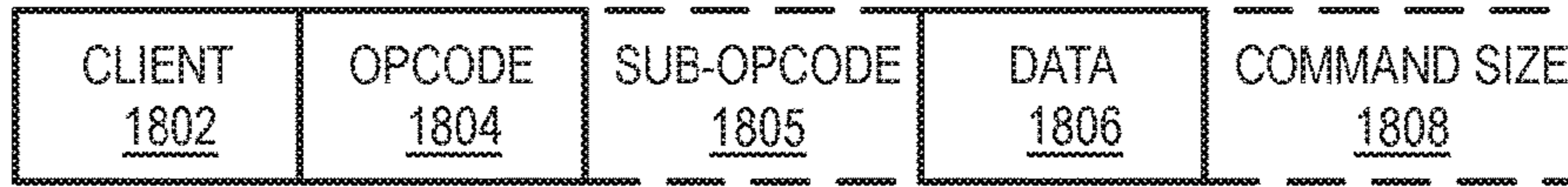
FIG. 18A GRAPHICS PROCESSOR COMMAND FORMAT 1800
