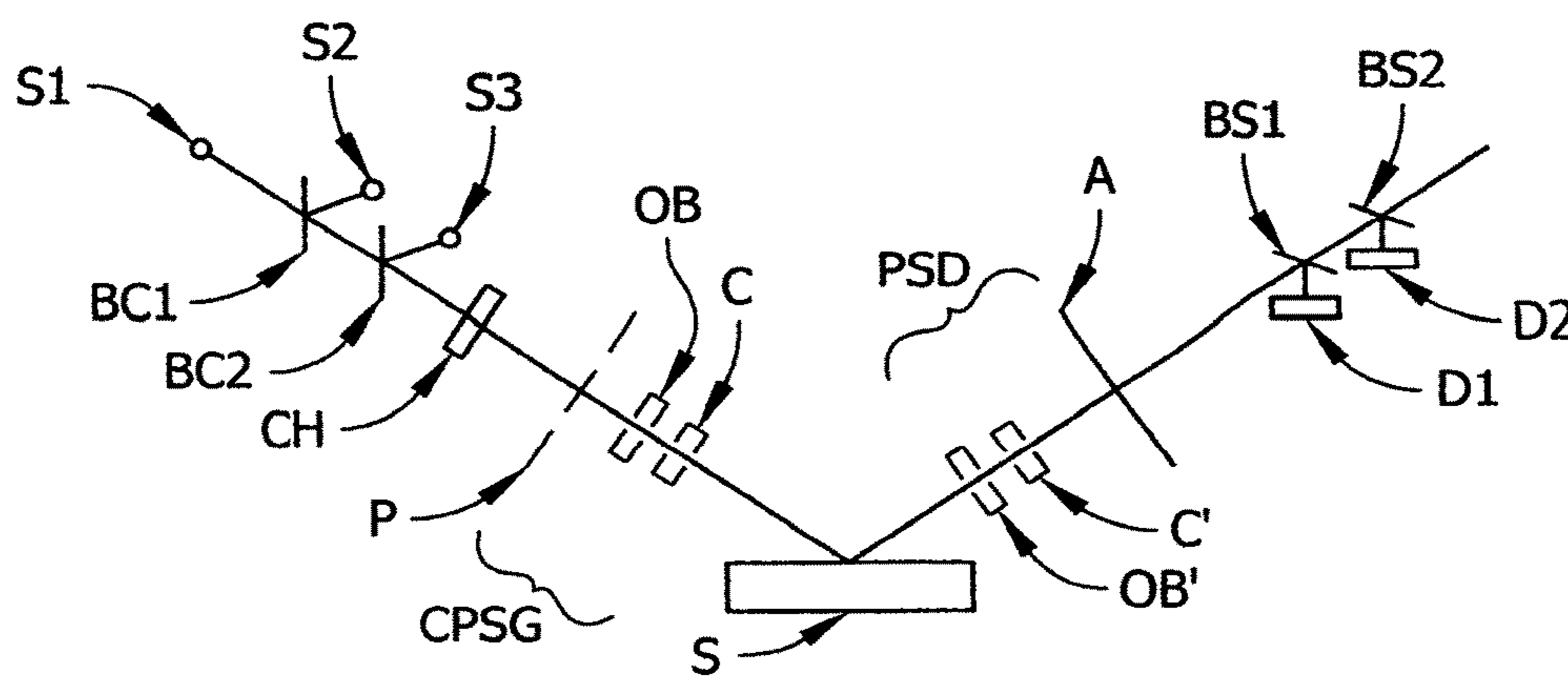
Fig. 6 PRIOR ART
