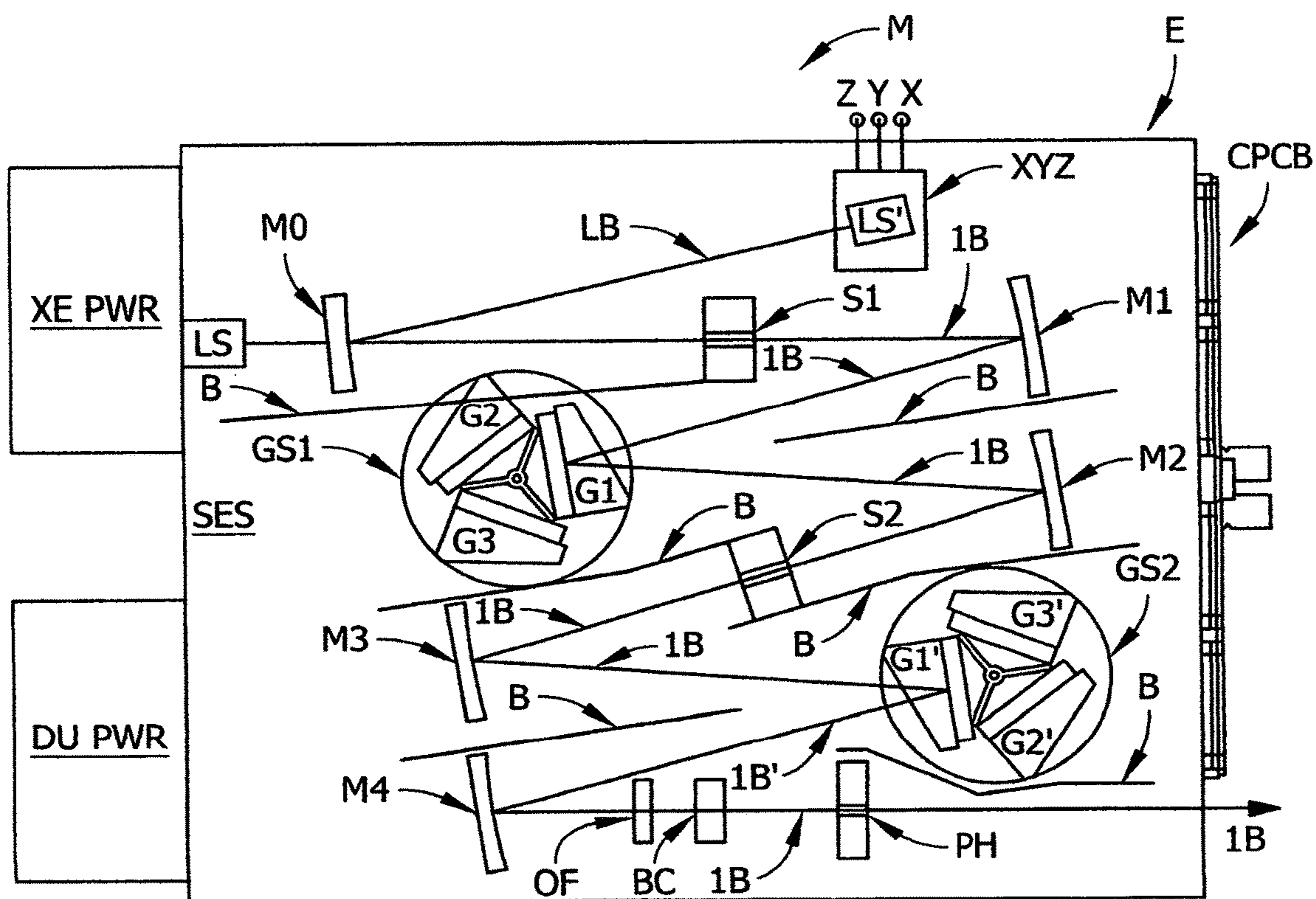
Fig. 5 PRIOR ART
