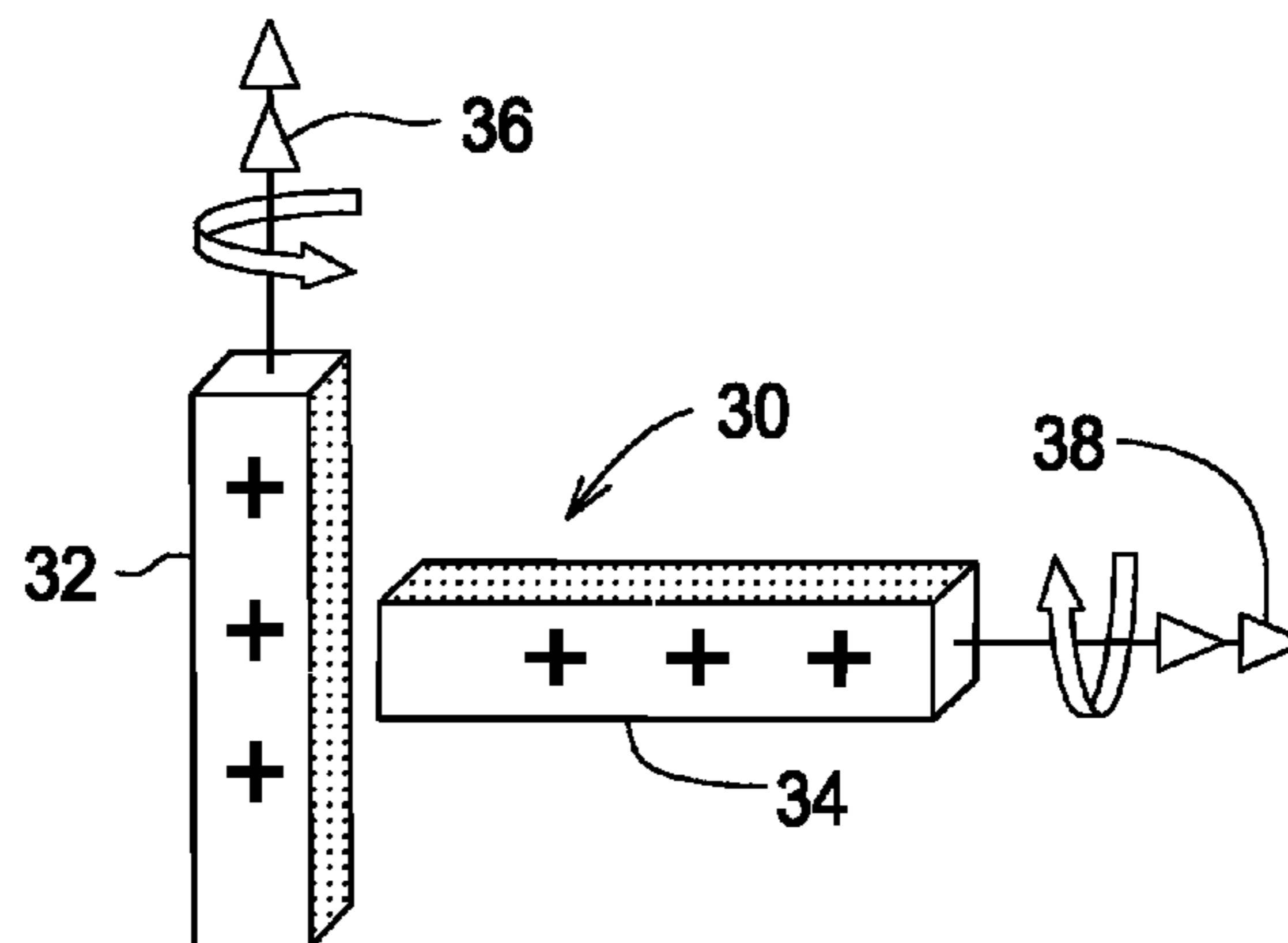
VERTICAL AND HORIZONTAL MAGNETS IN SAME HOUSING
