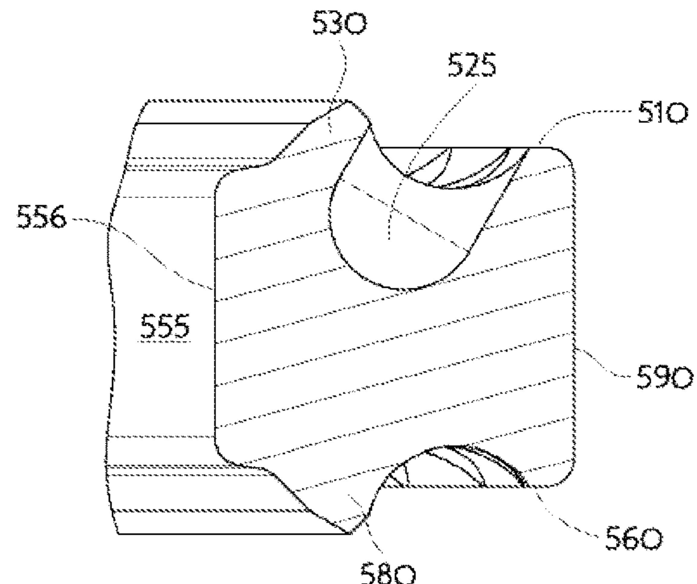
DETAIL A
