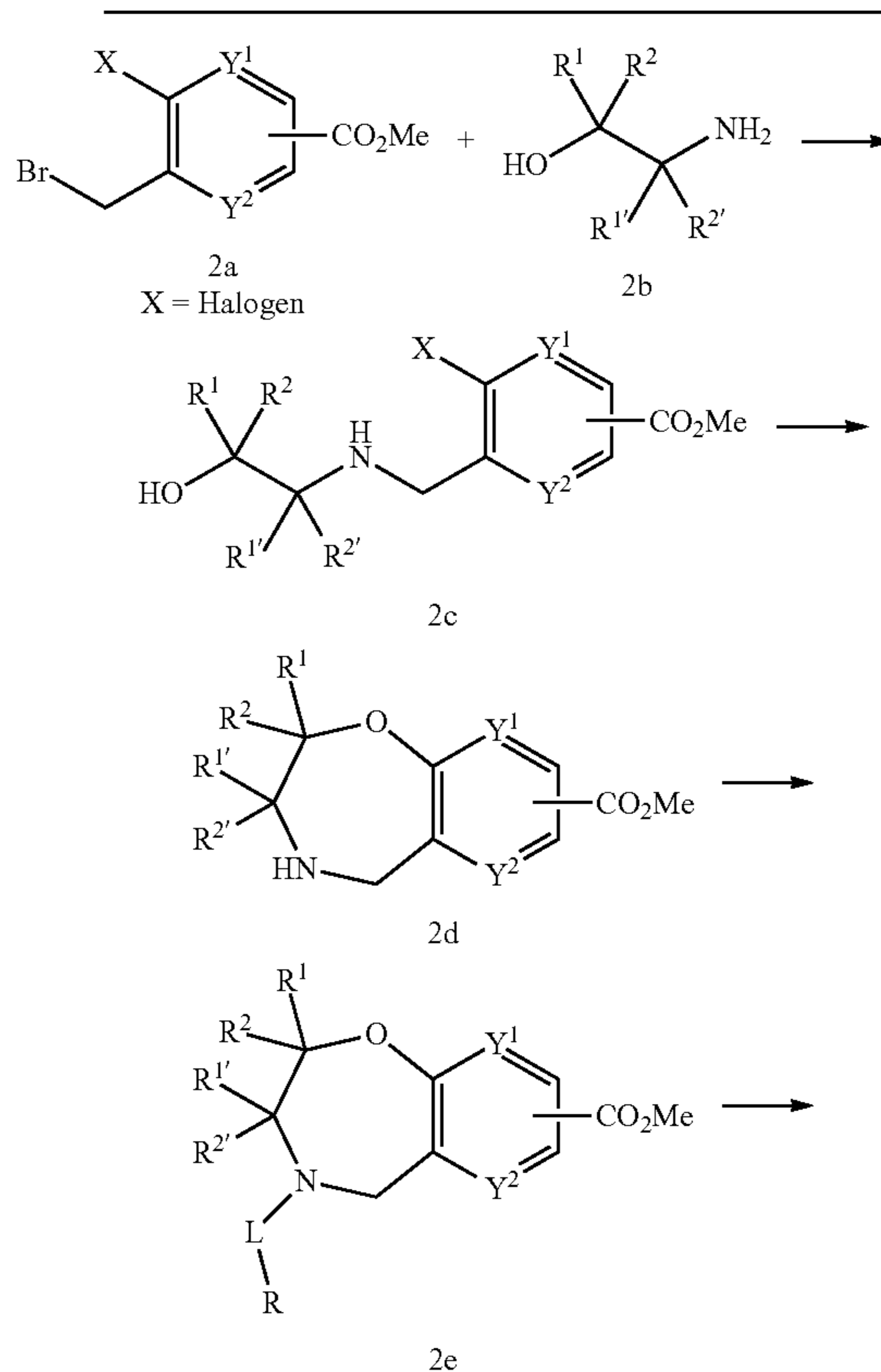
Scheme 1. General synthesis of ethers, thioethers, or sulfones described in the disclosure.
