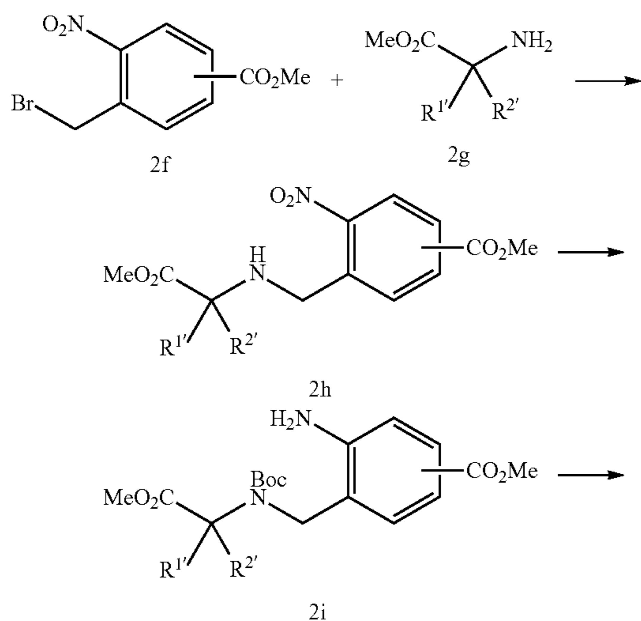
Scheme 2. General synthesis of amides described in the disclosure.
