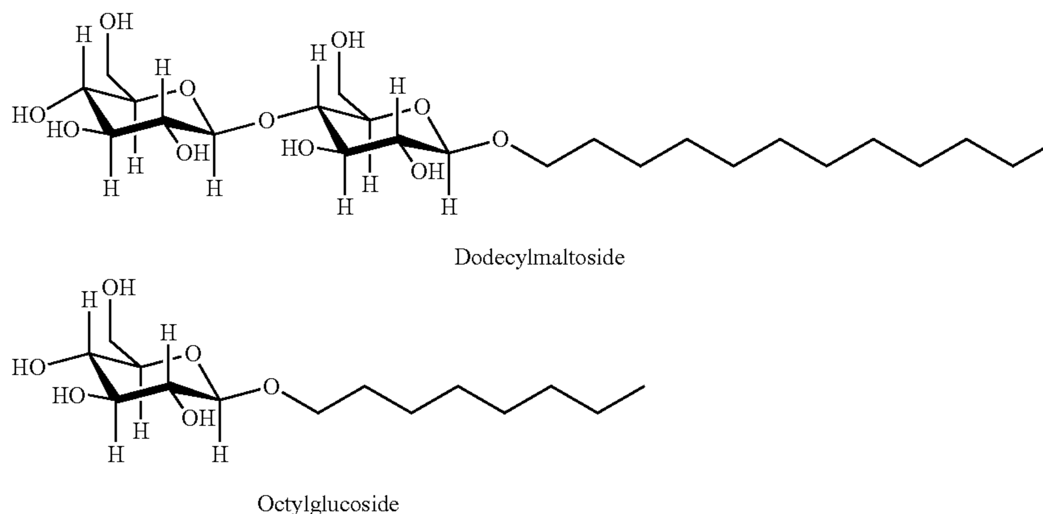
Scheme 1. Examples of commercially-available non-ionic surfactants of the alkyl glycoside class
