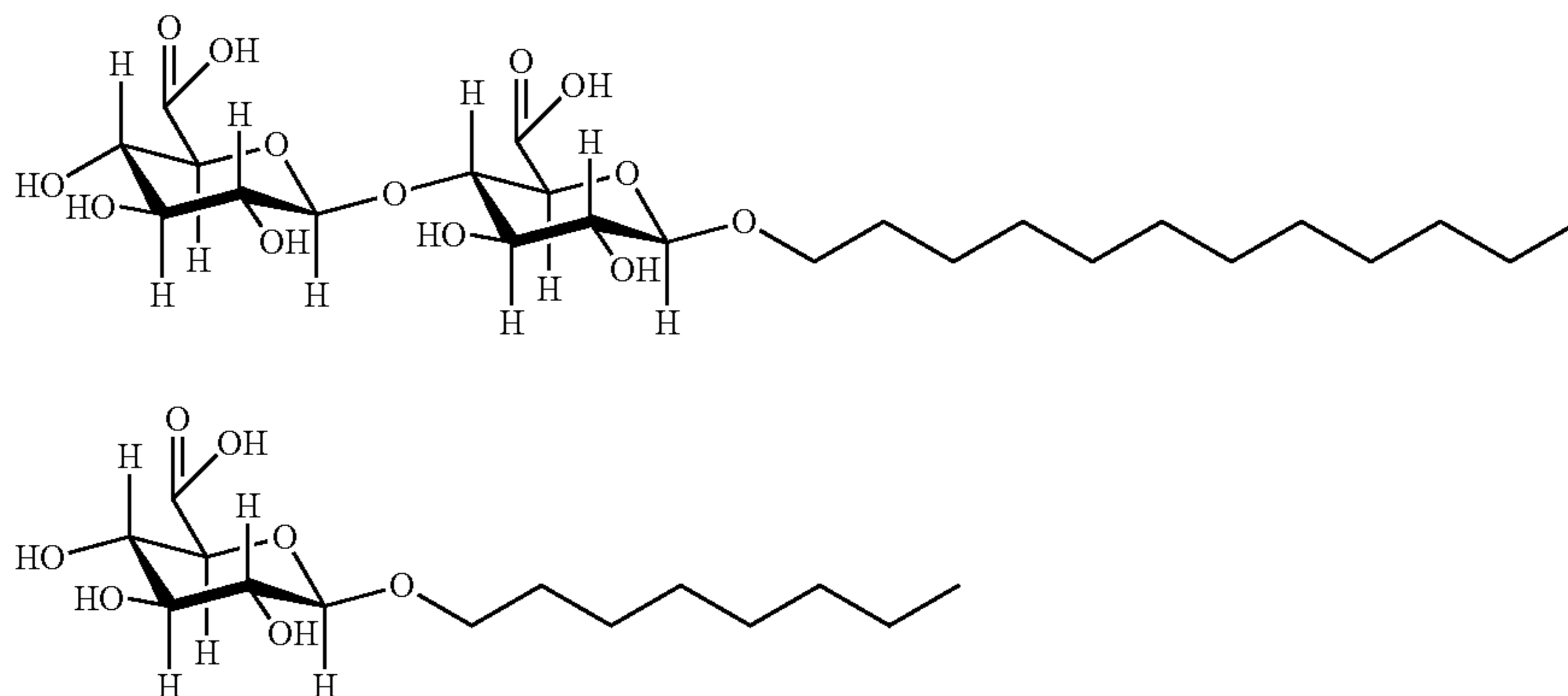
Scheme 2. Examples of alkyl glucuronic and diglucuronic acid class reagents.
