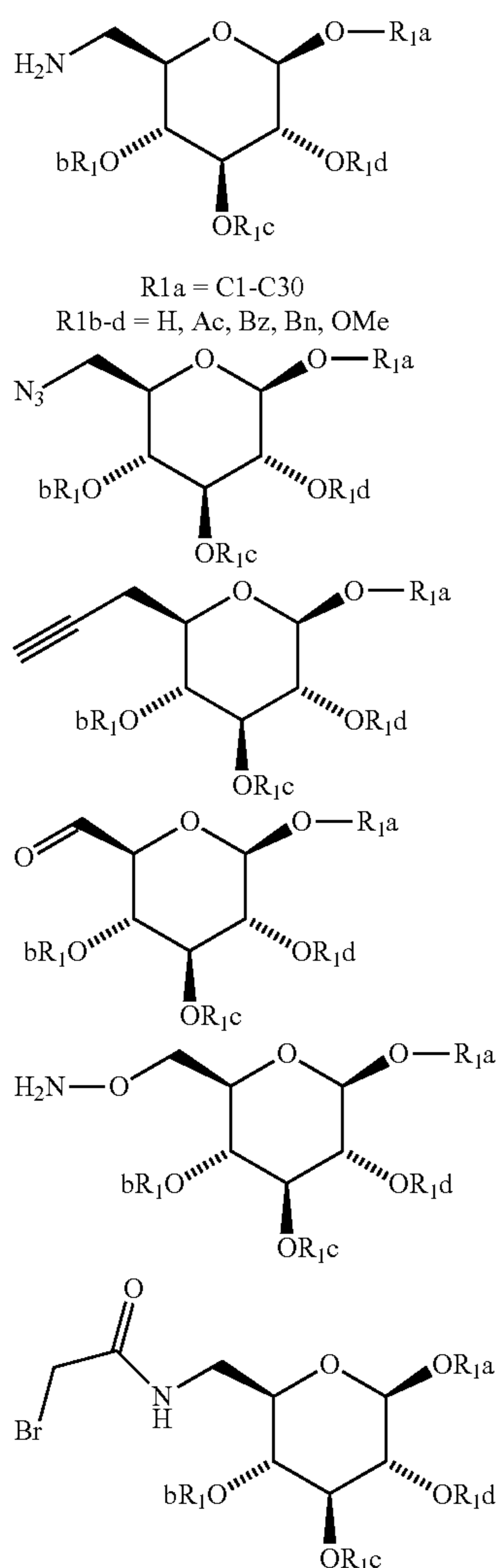
Scheme 6. Additional reagent examples.
