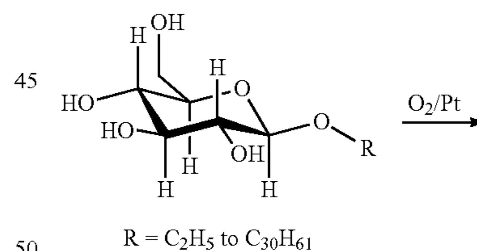
Scheme 4. Example of a preparation of a reagent
