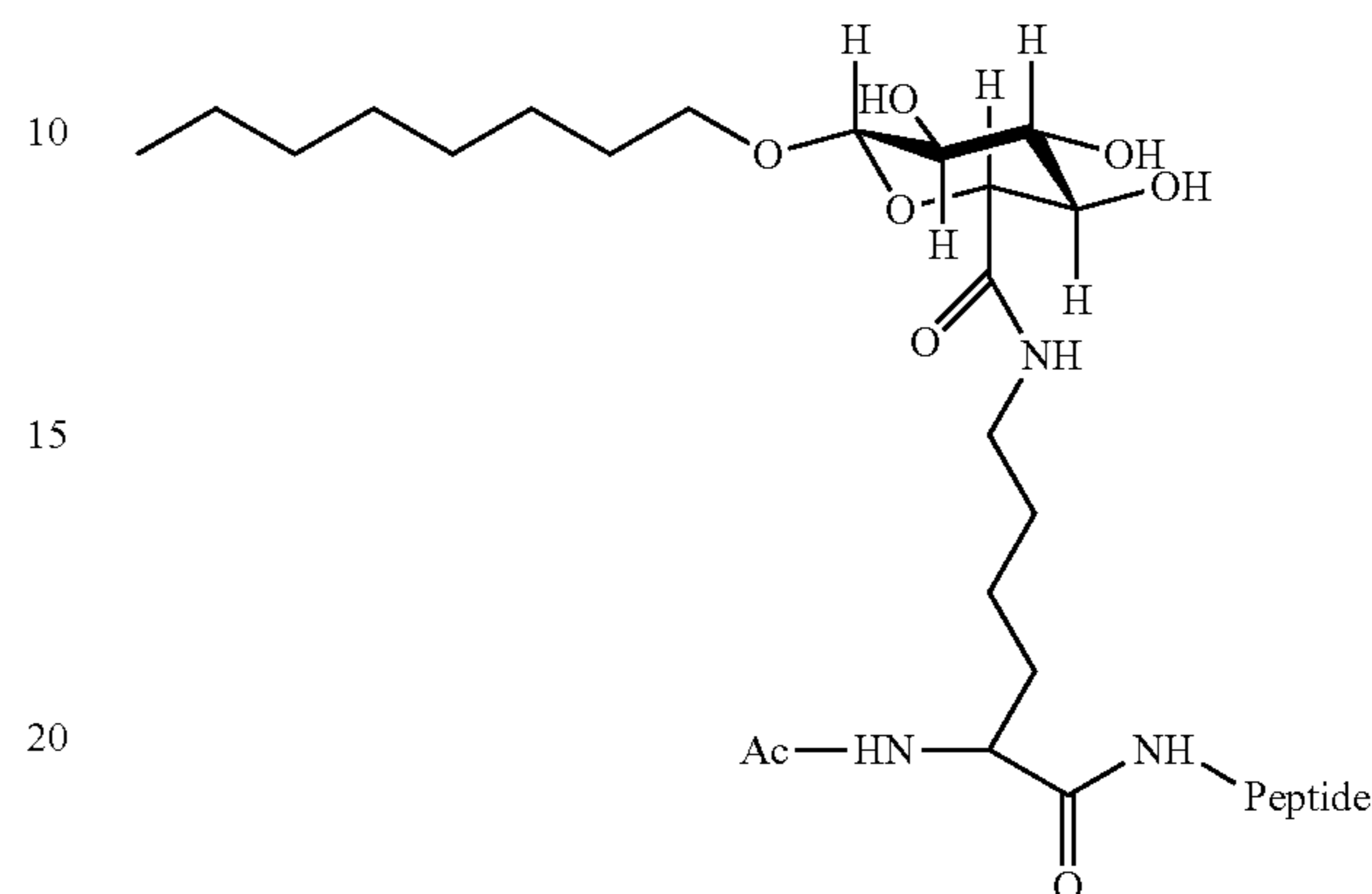
Scheme 5. Illustrative example of a peptide intermediate.
