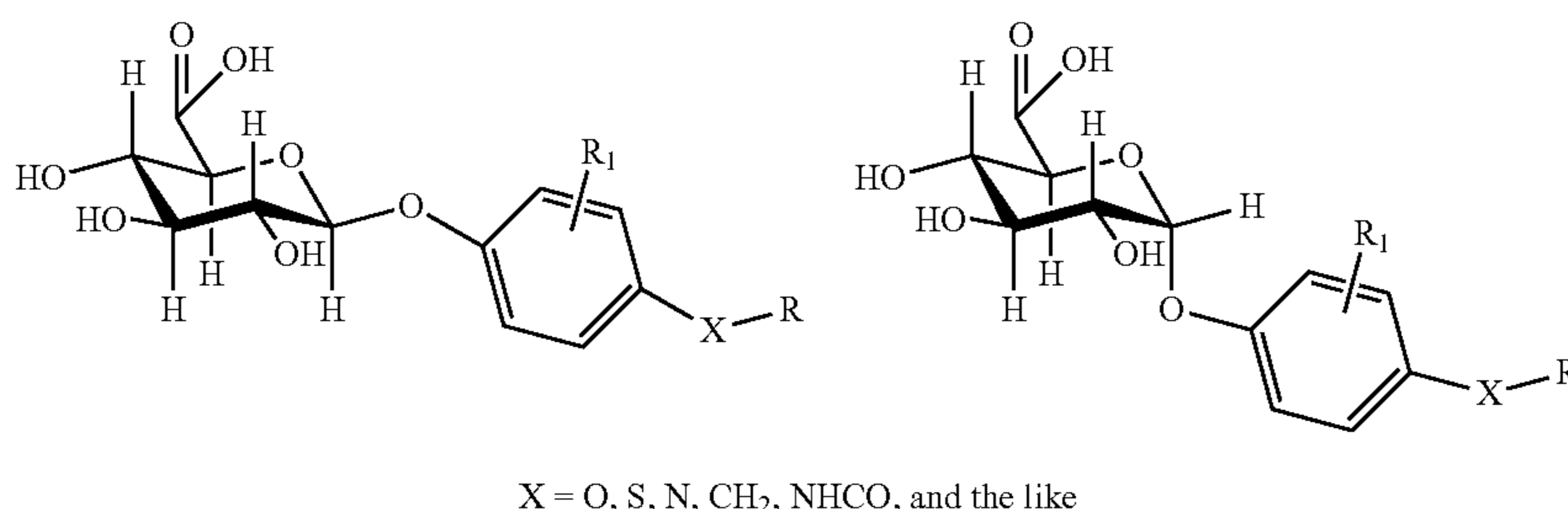
Scheme 3. Illustrative members of aralkyl or alkoxyaryl surfactant moiety.
