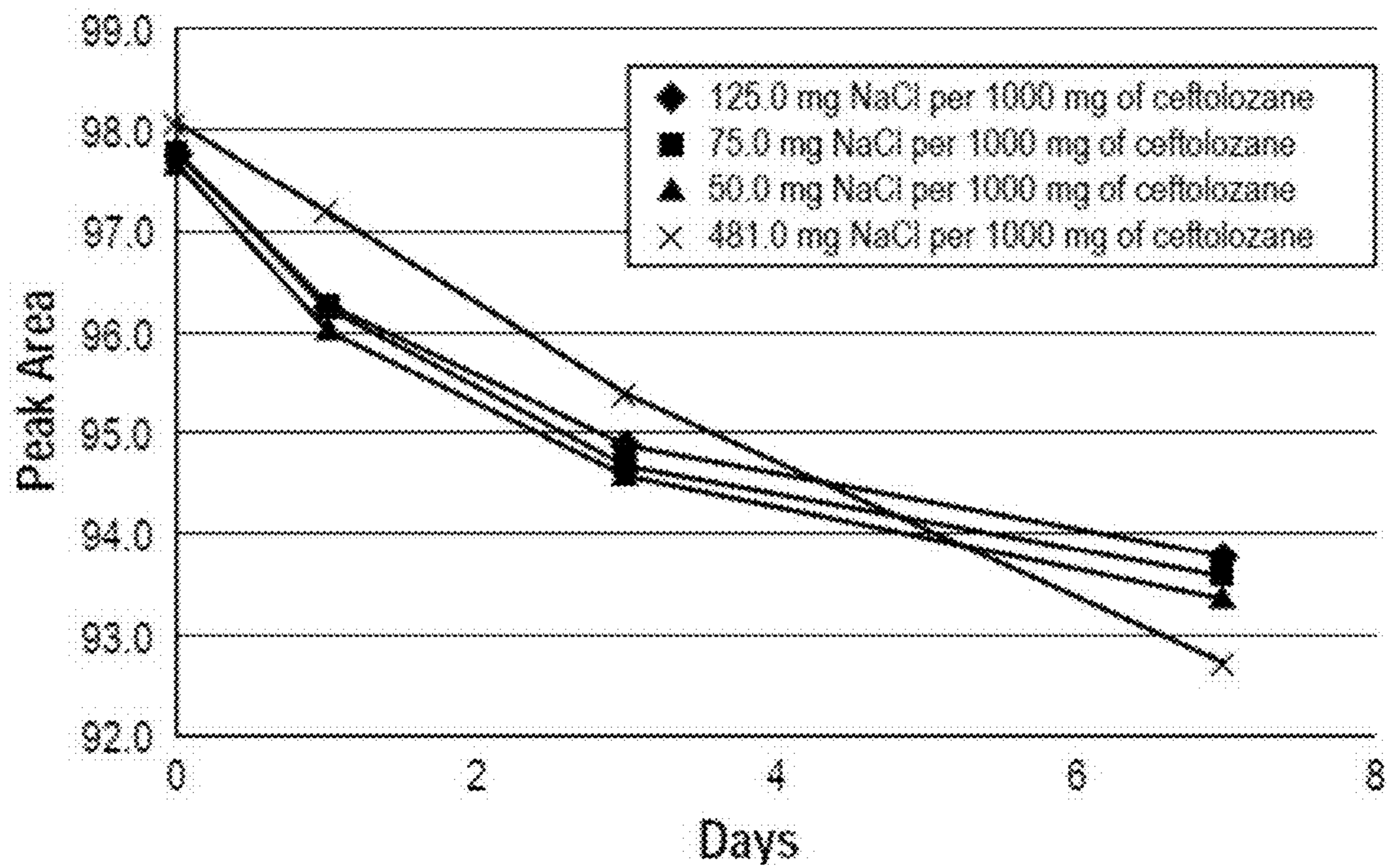
Figure 7 The Purity of Cefotolozane, 60°C
