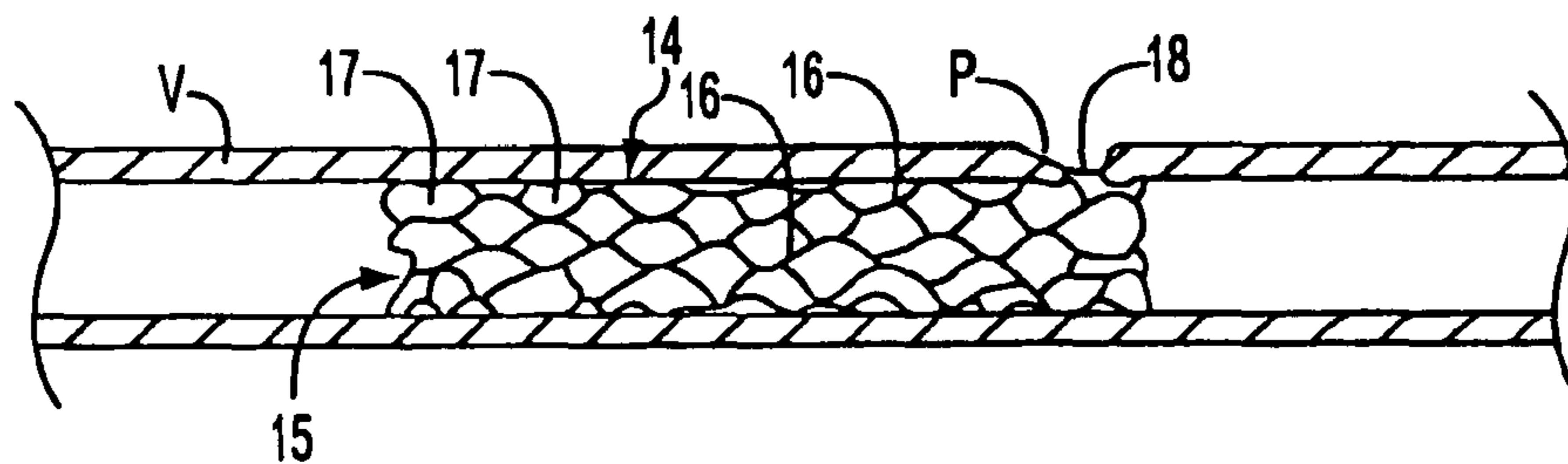
FIG. 6C (PRIOR ART)
