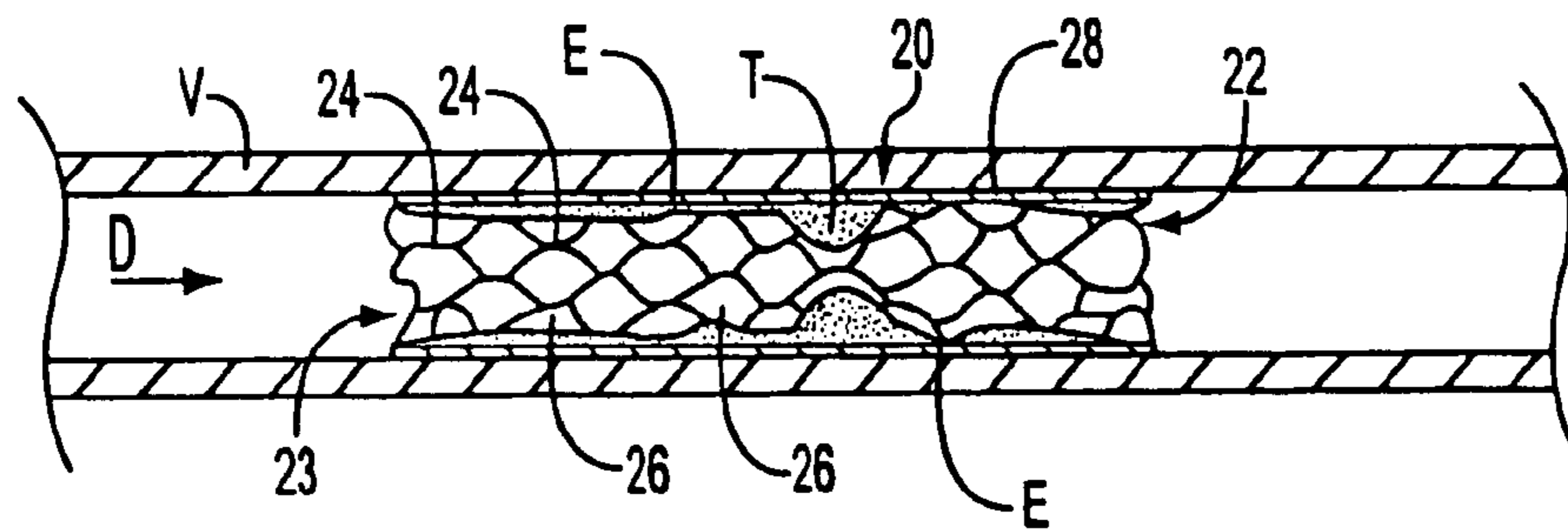
FIG. 7 (PRIOR ART)
