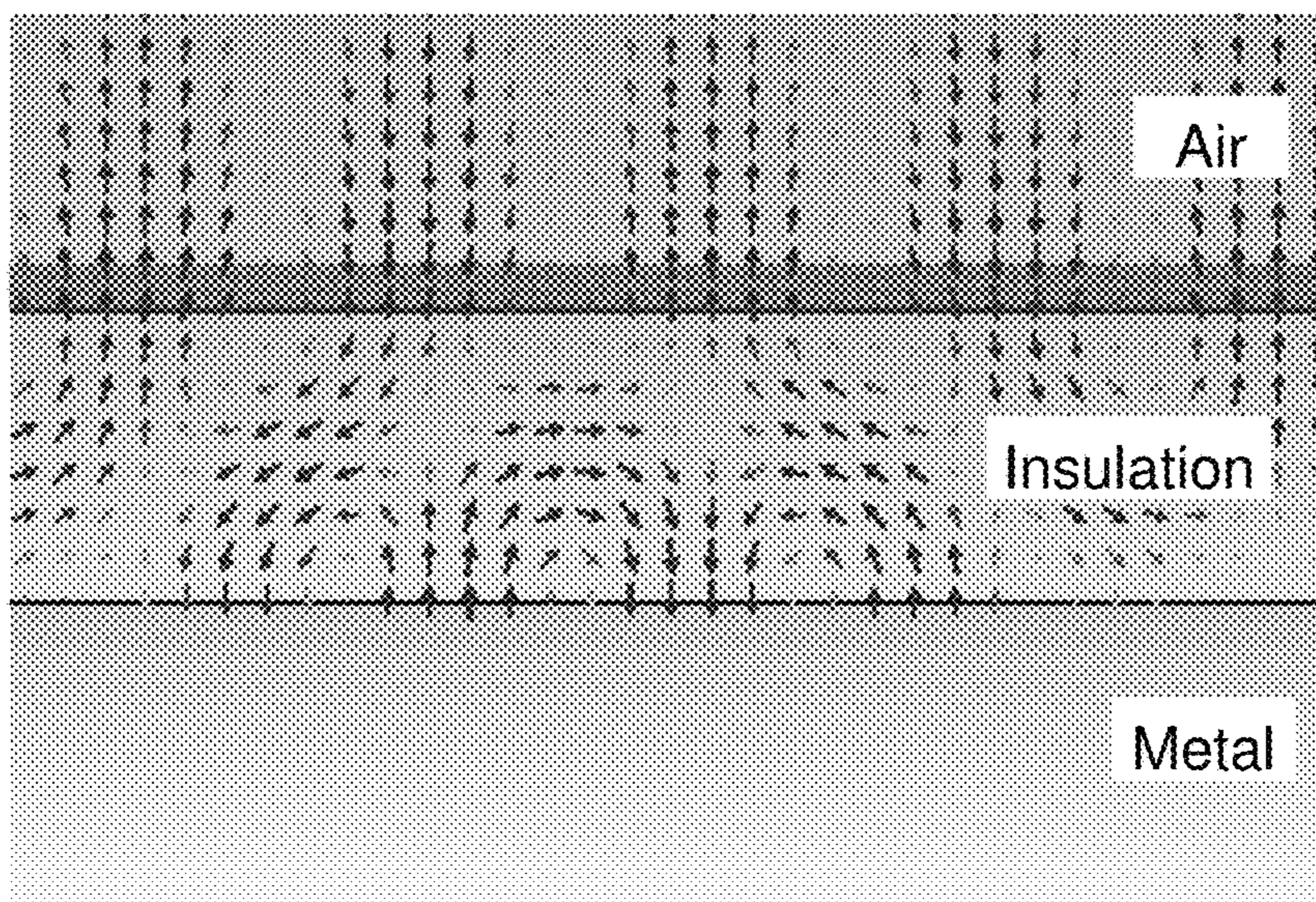
Longitudinal Section of Cable showing e-fields of TM 01 waves at 40 GHz
