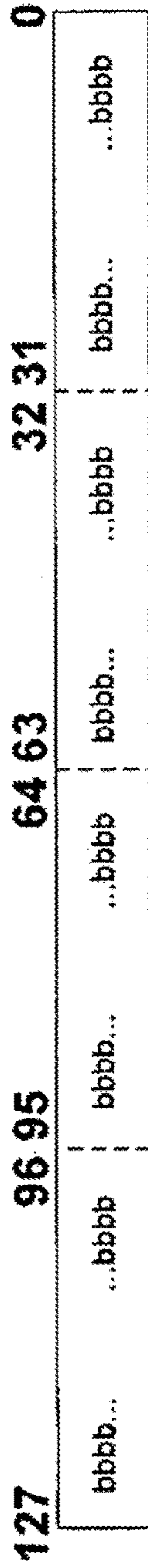
Unsigned packed doubleword in-register representation 514
