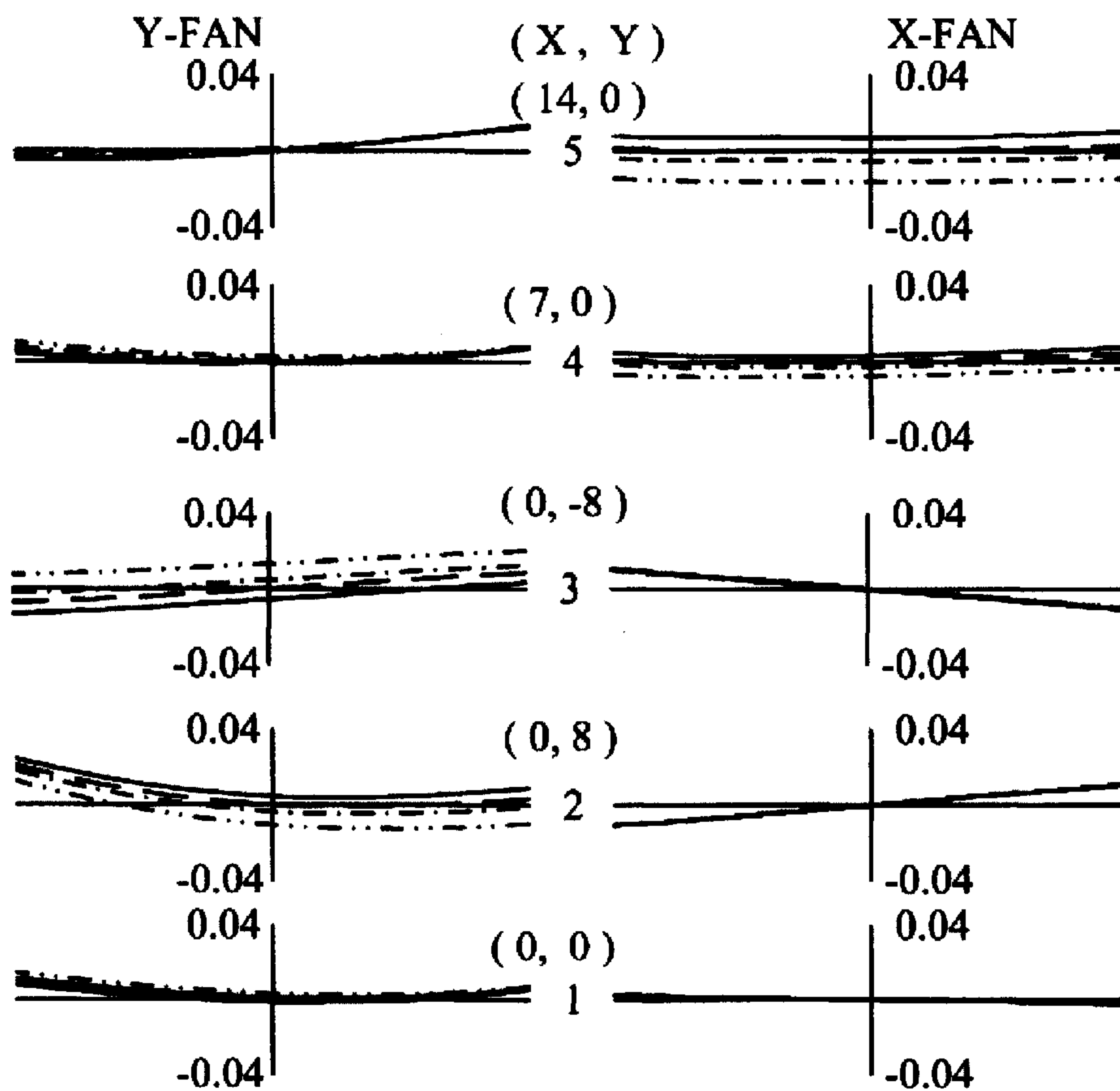
RAY ABERRATIONS (mm)
