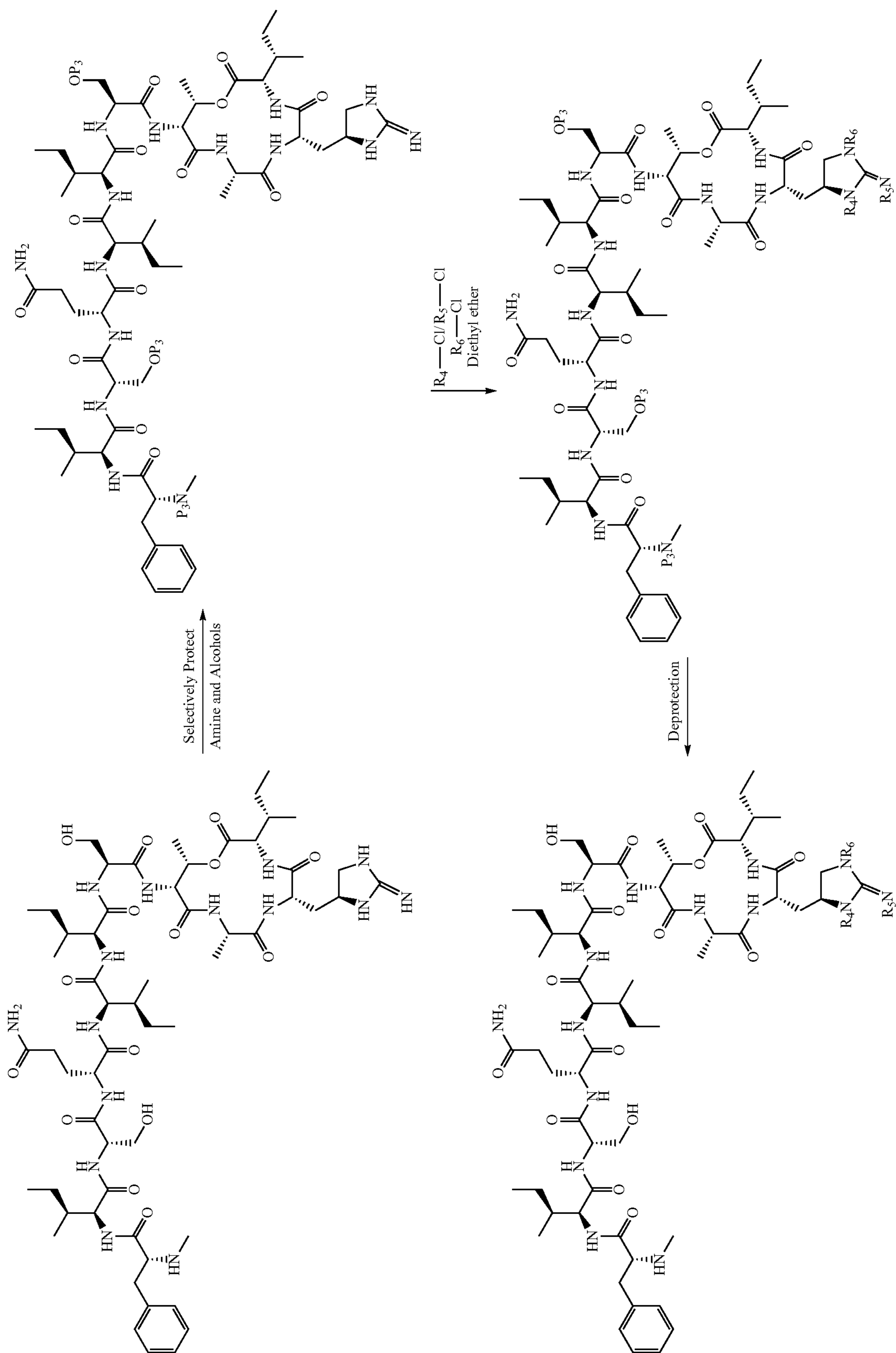
Scheme 1.
