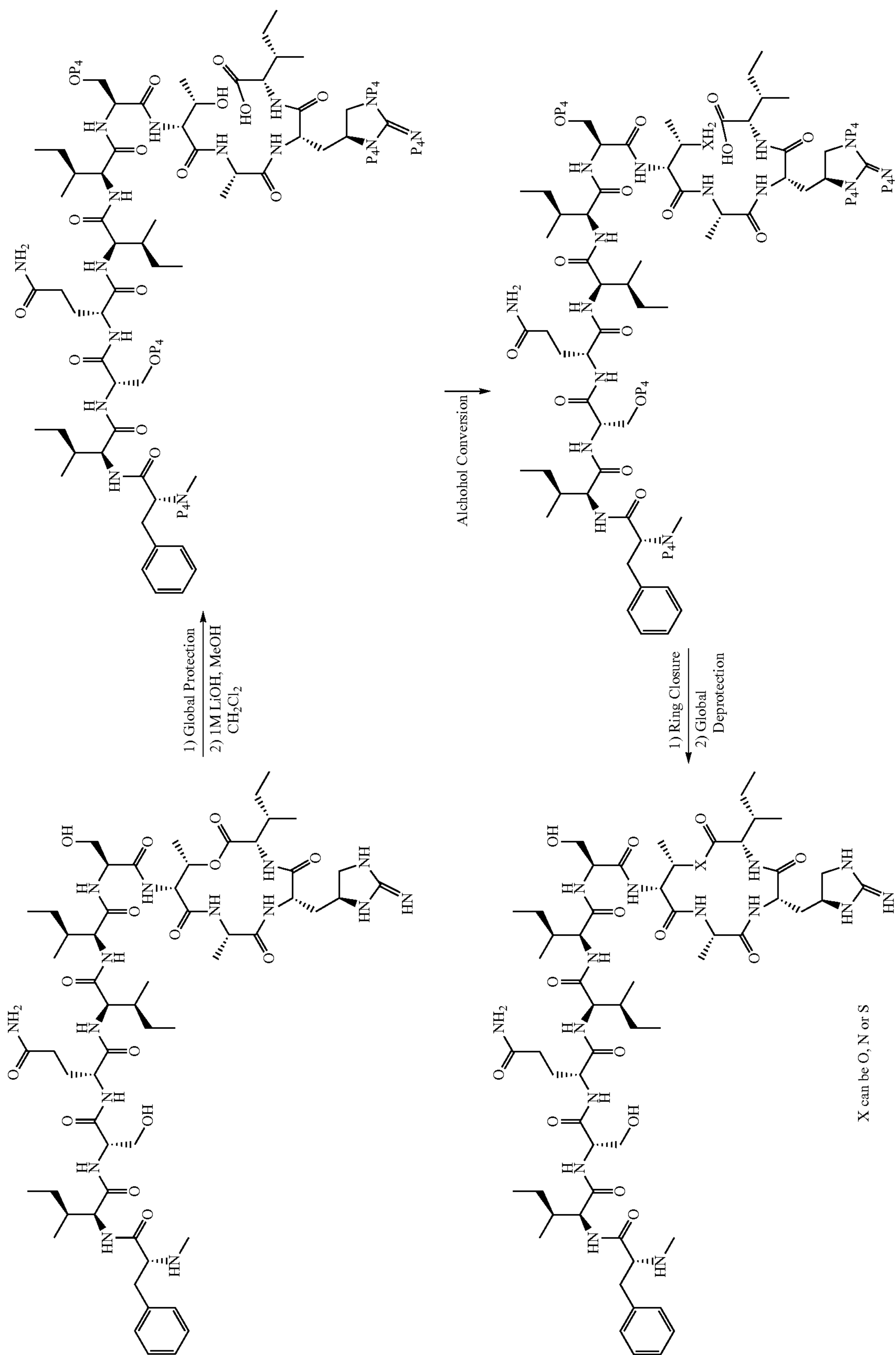
Scheme 4.
