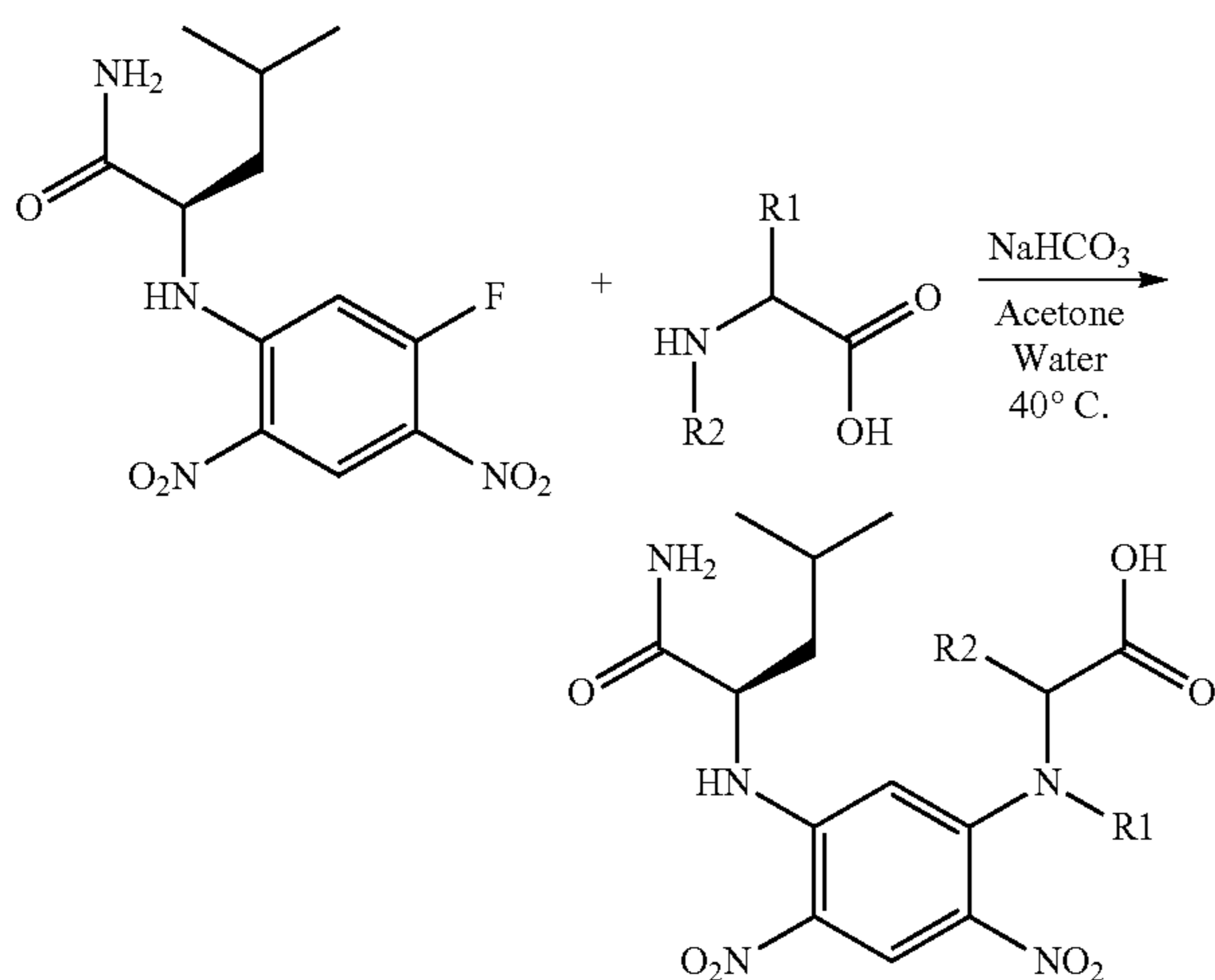
Scheme 5
