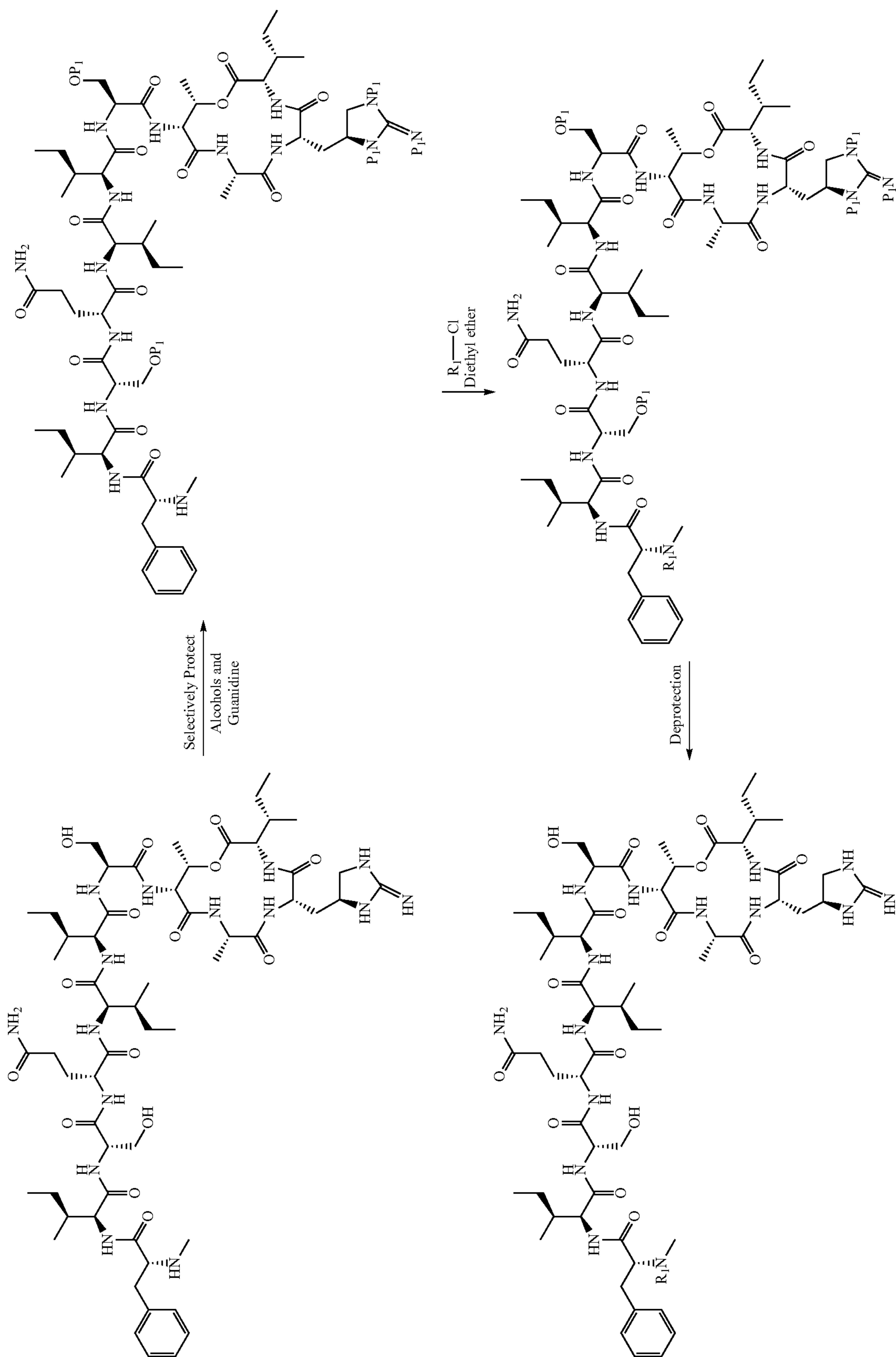
Scheme 2.
