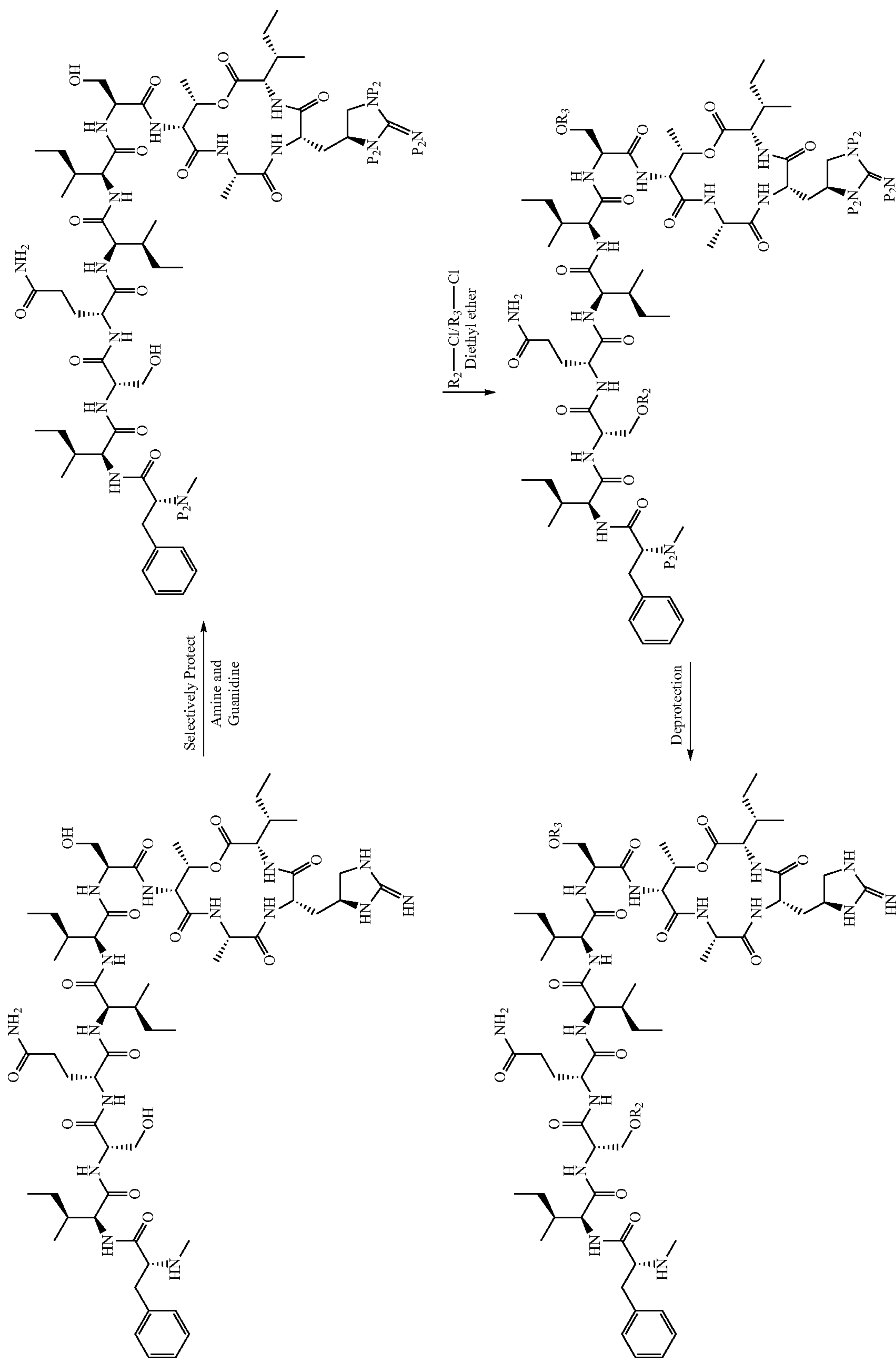
Scheme 3.
