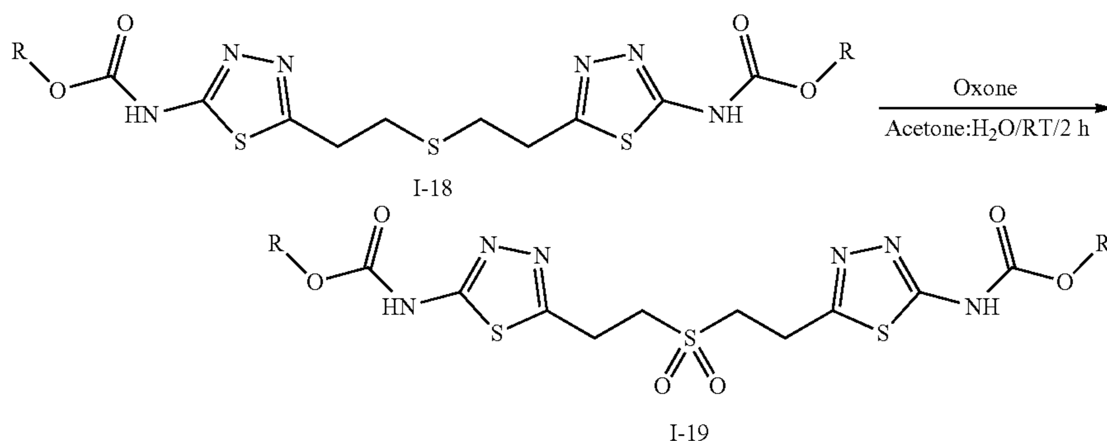
Scheme 9
