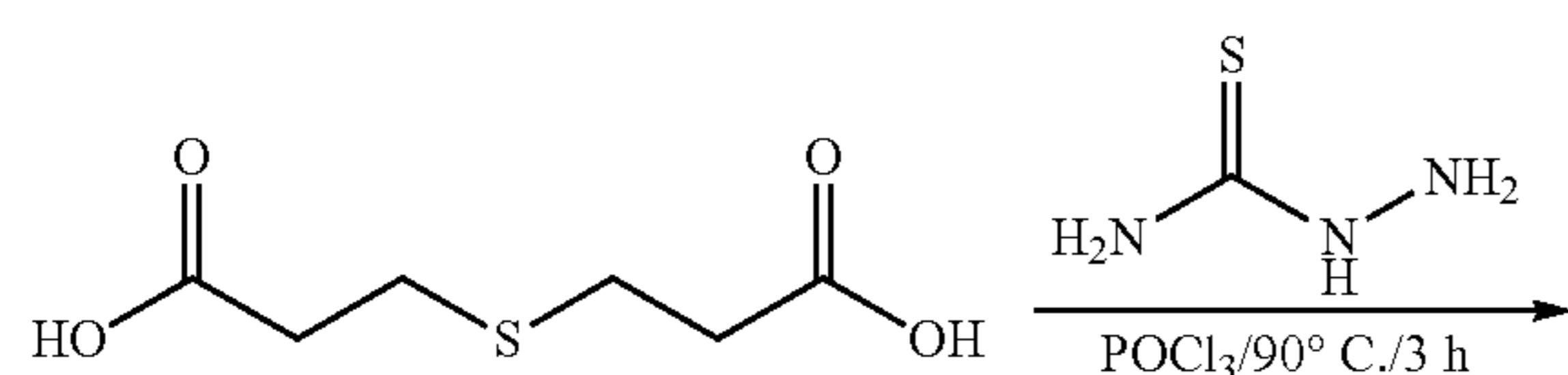
Scheme 25
