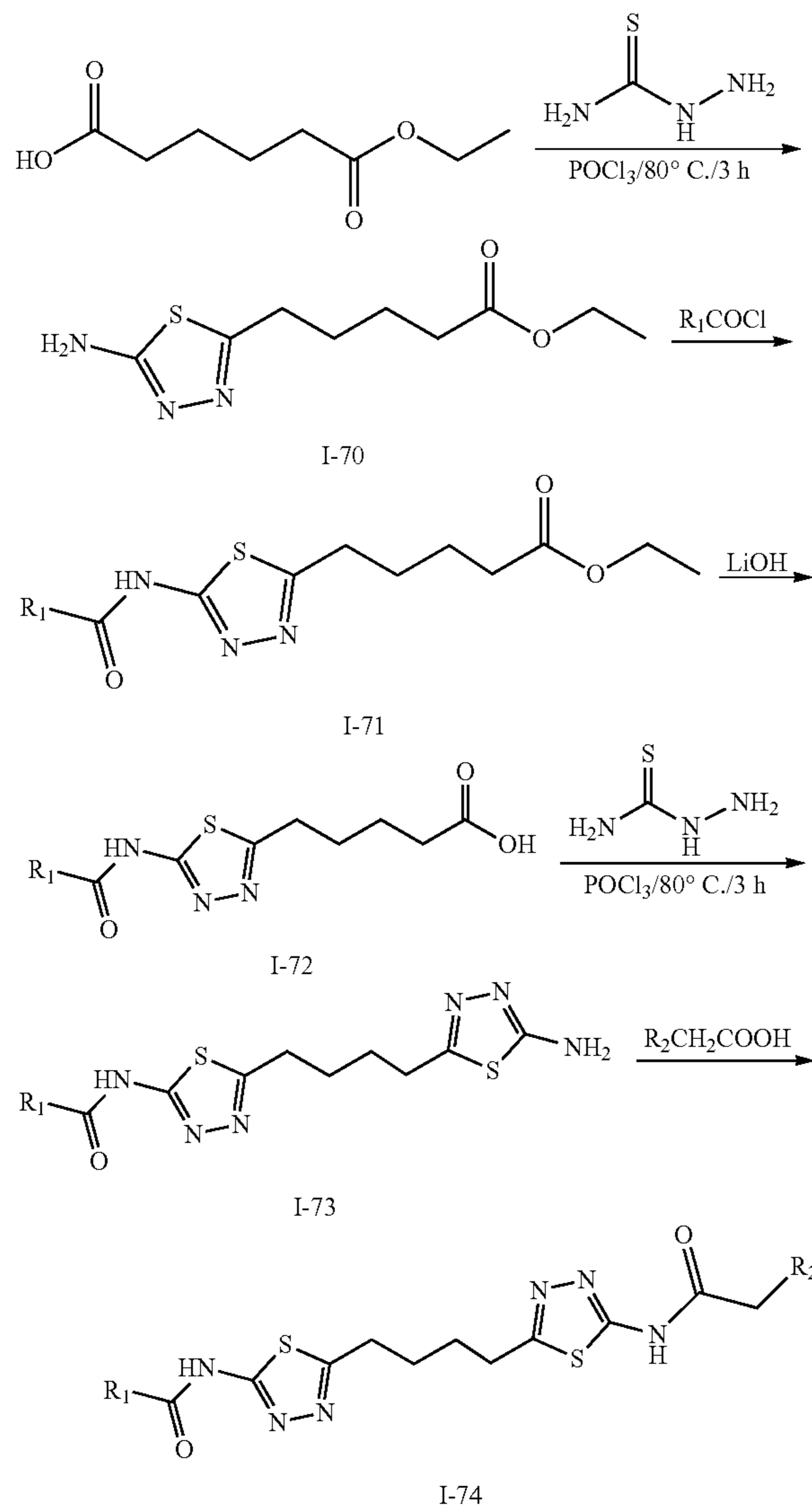
Scheme 17
