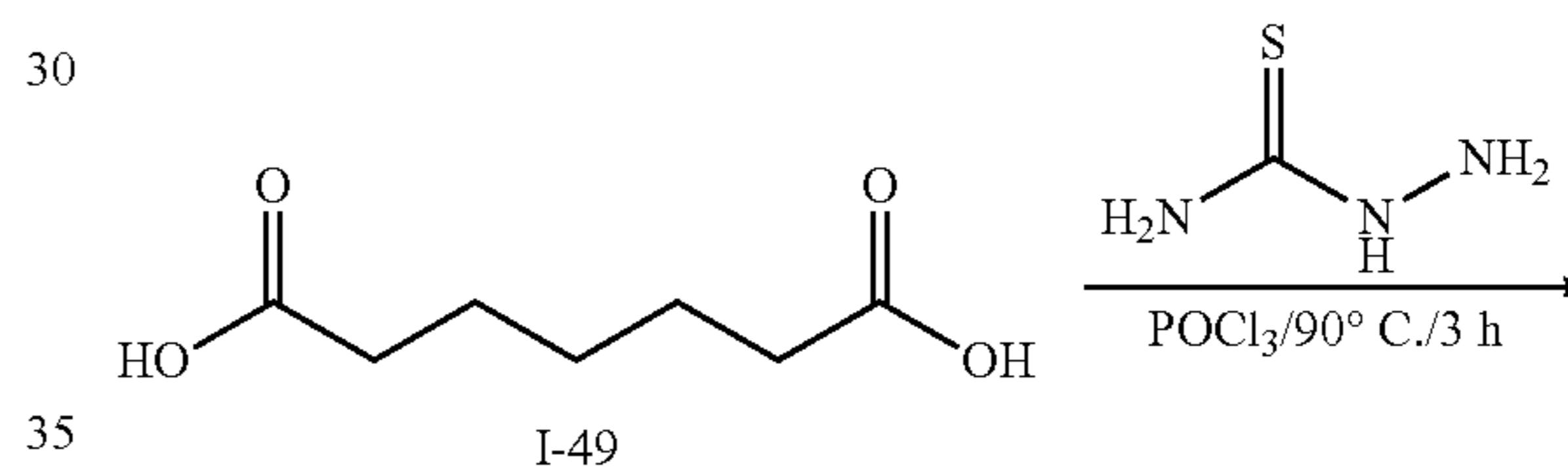
Scheme 16
