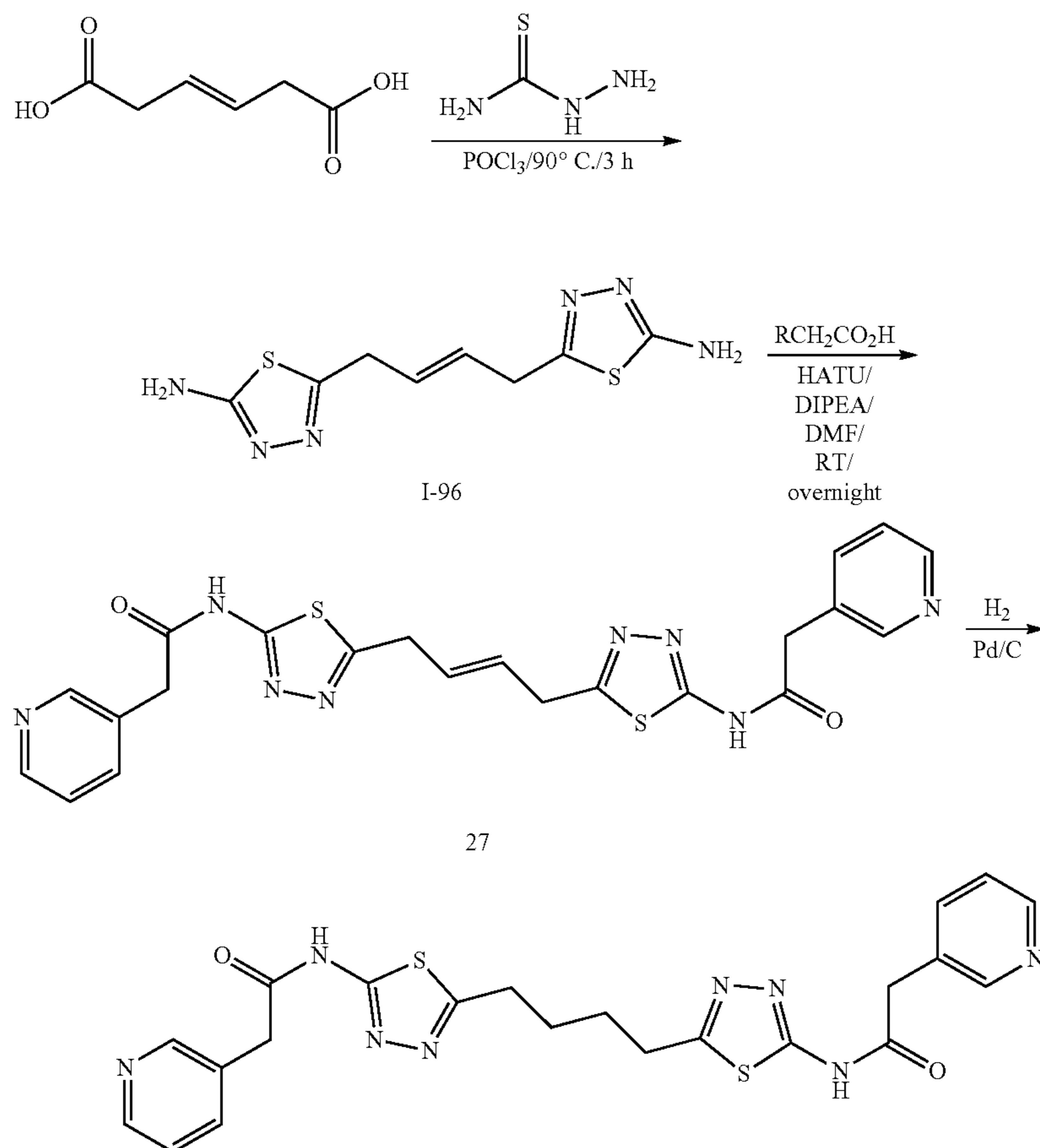
Scheme 22
