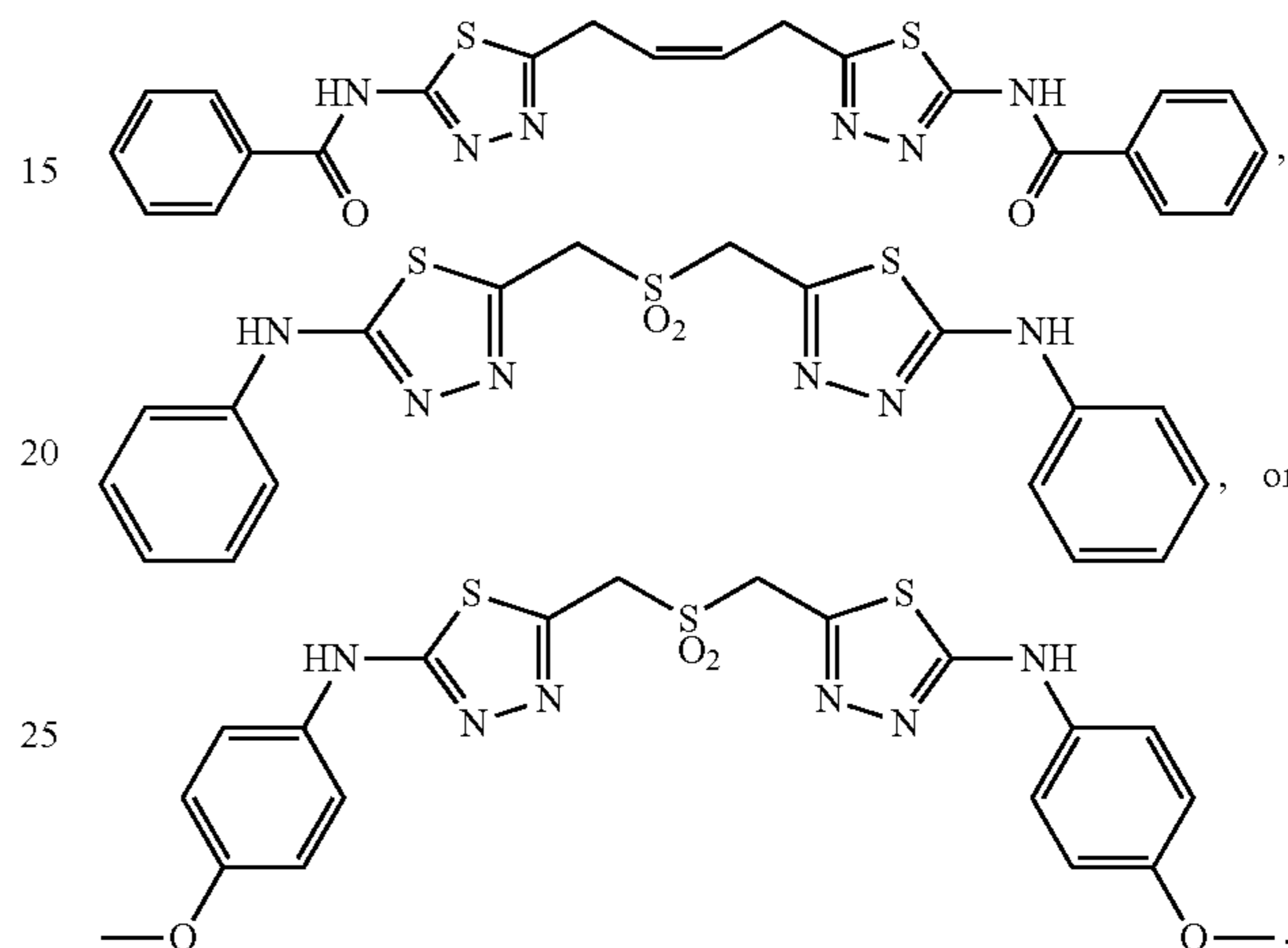
Formula (I)
