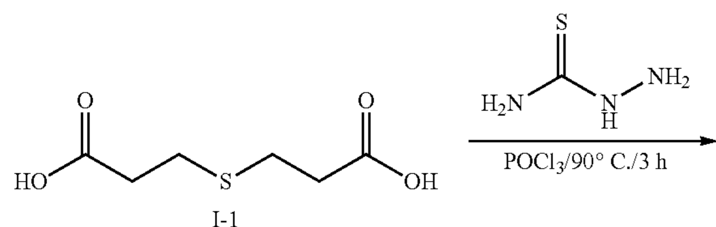
Scheme 1
