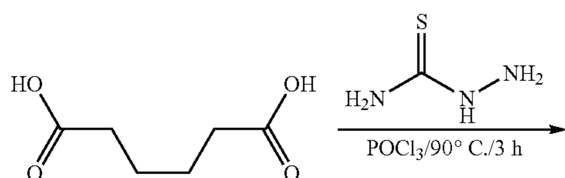
Scheme 23
