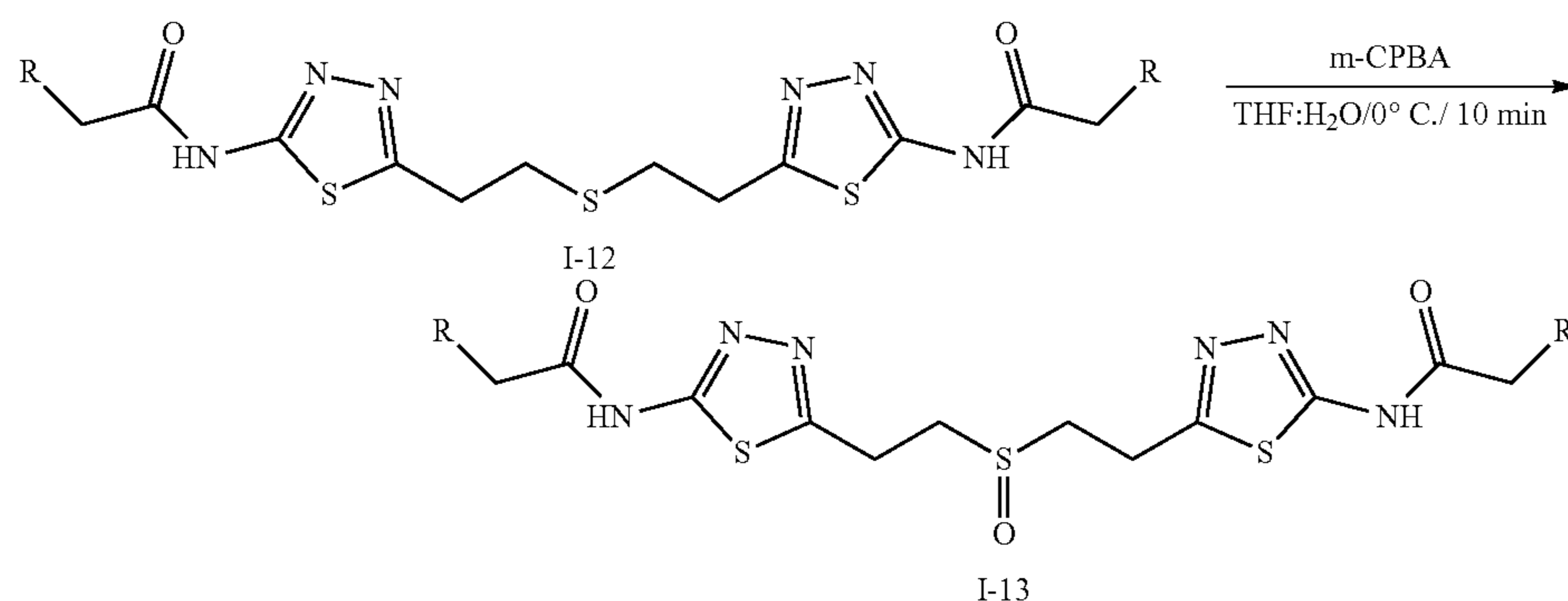
Scheme 7
