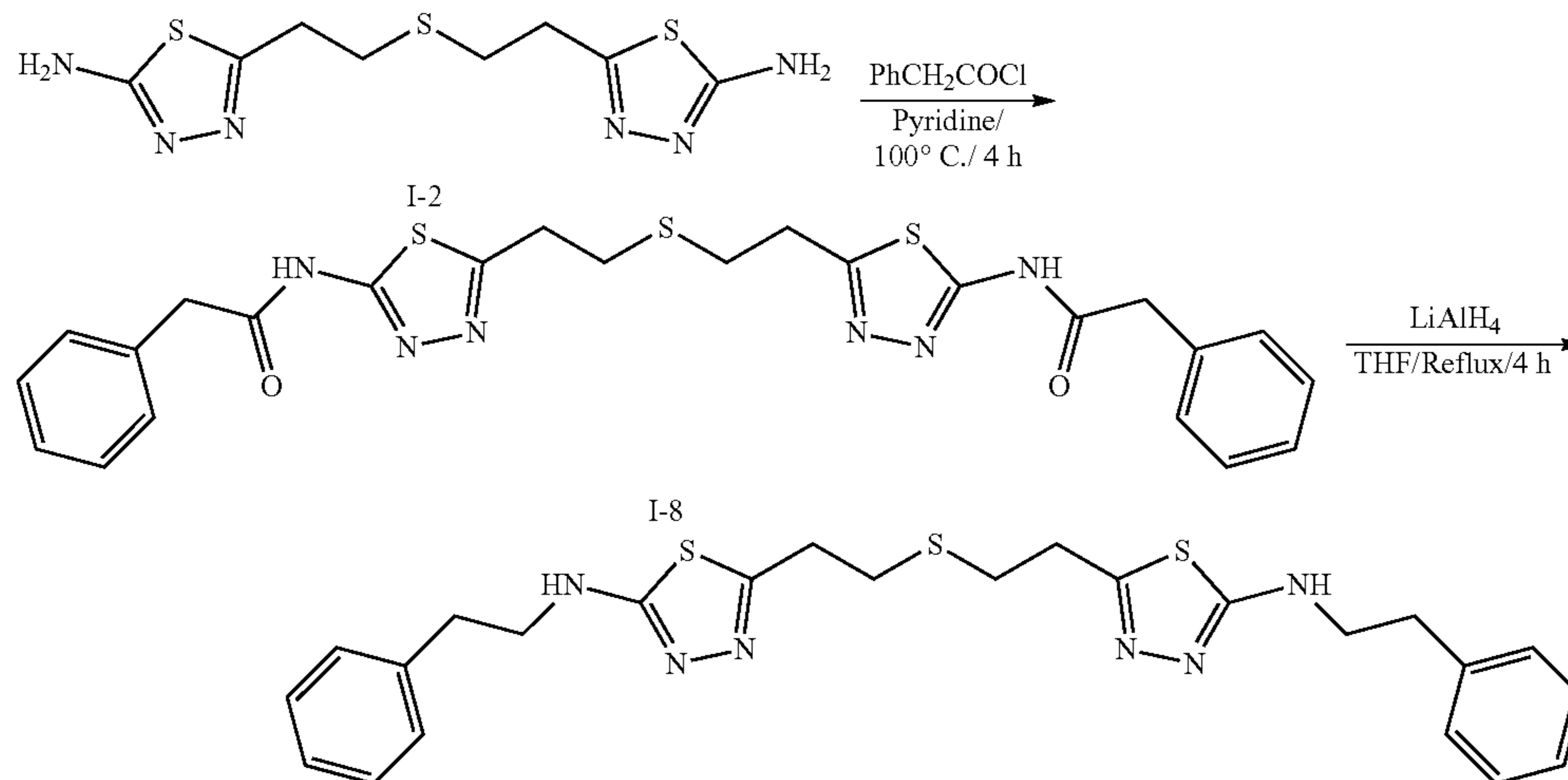
Scheme 5
