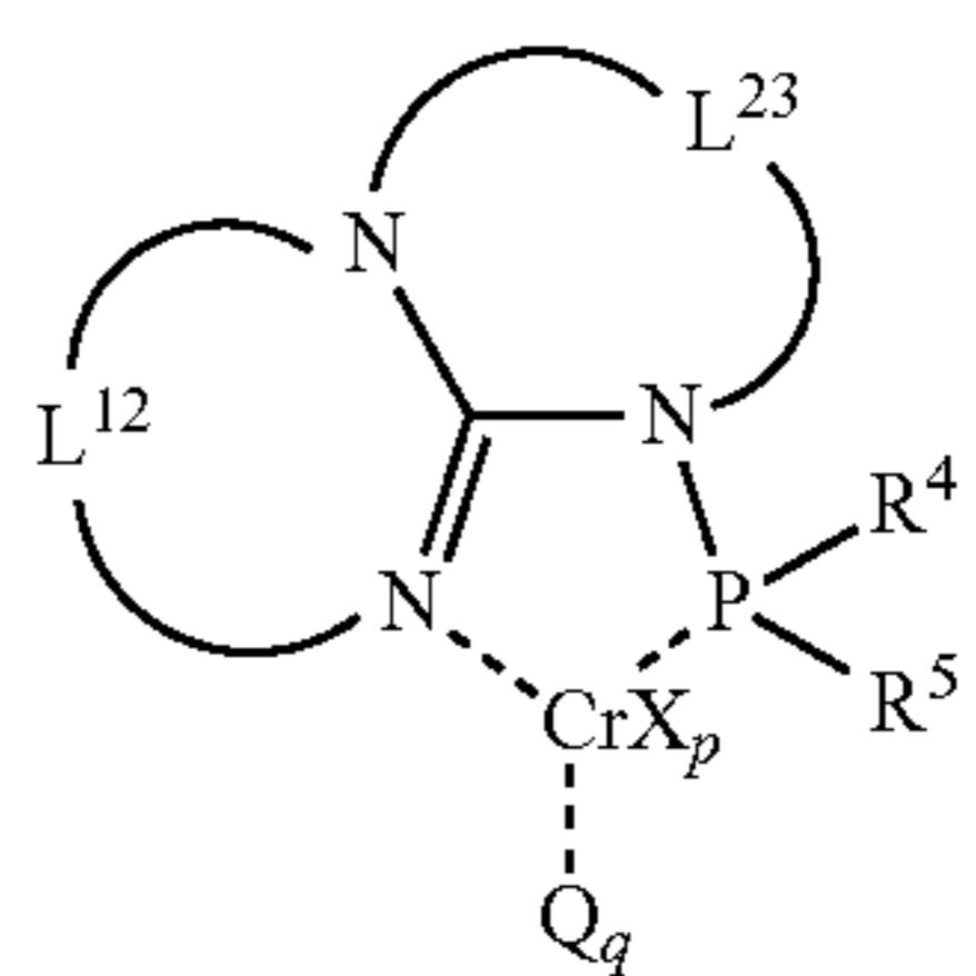
Structure GuCr4
