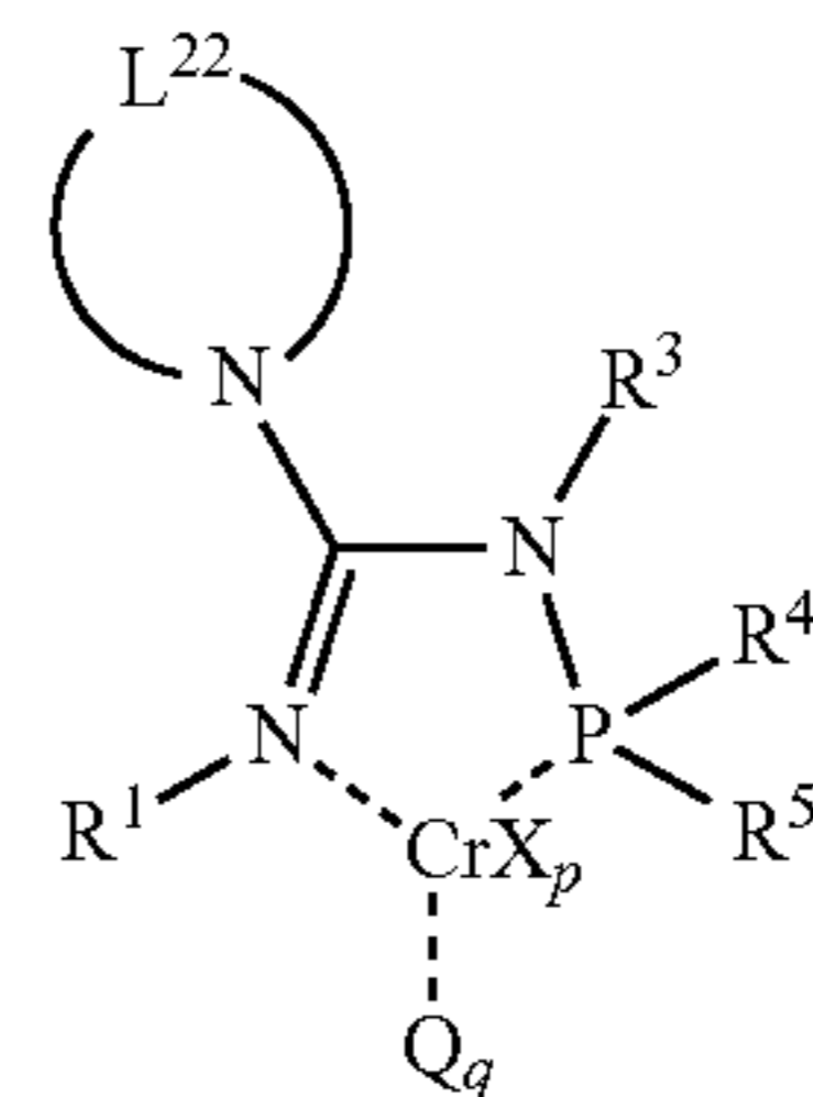
Structure GuCr5
