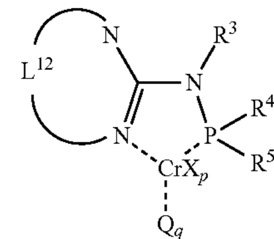
Structure GuCr2
