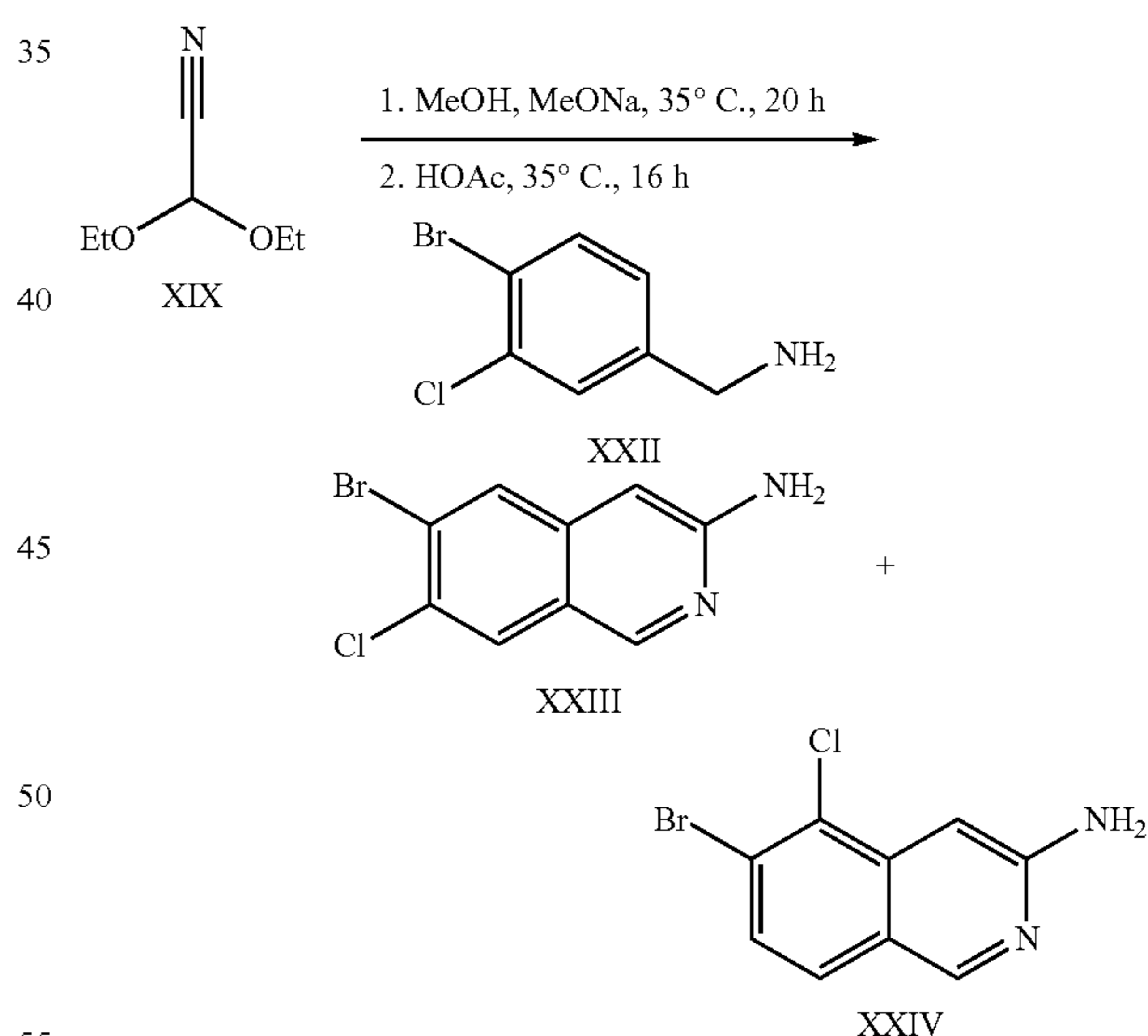
Scheme 7
