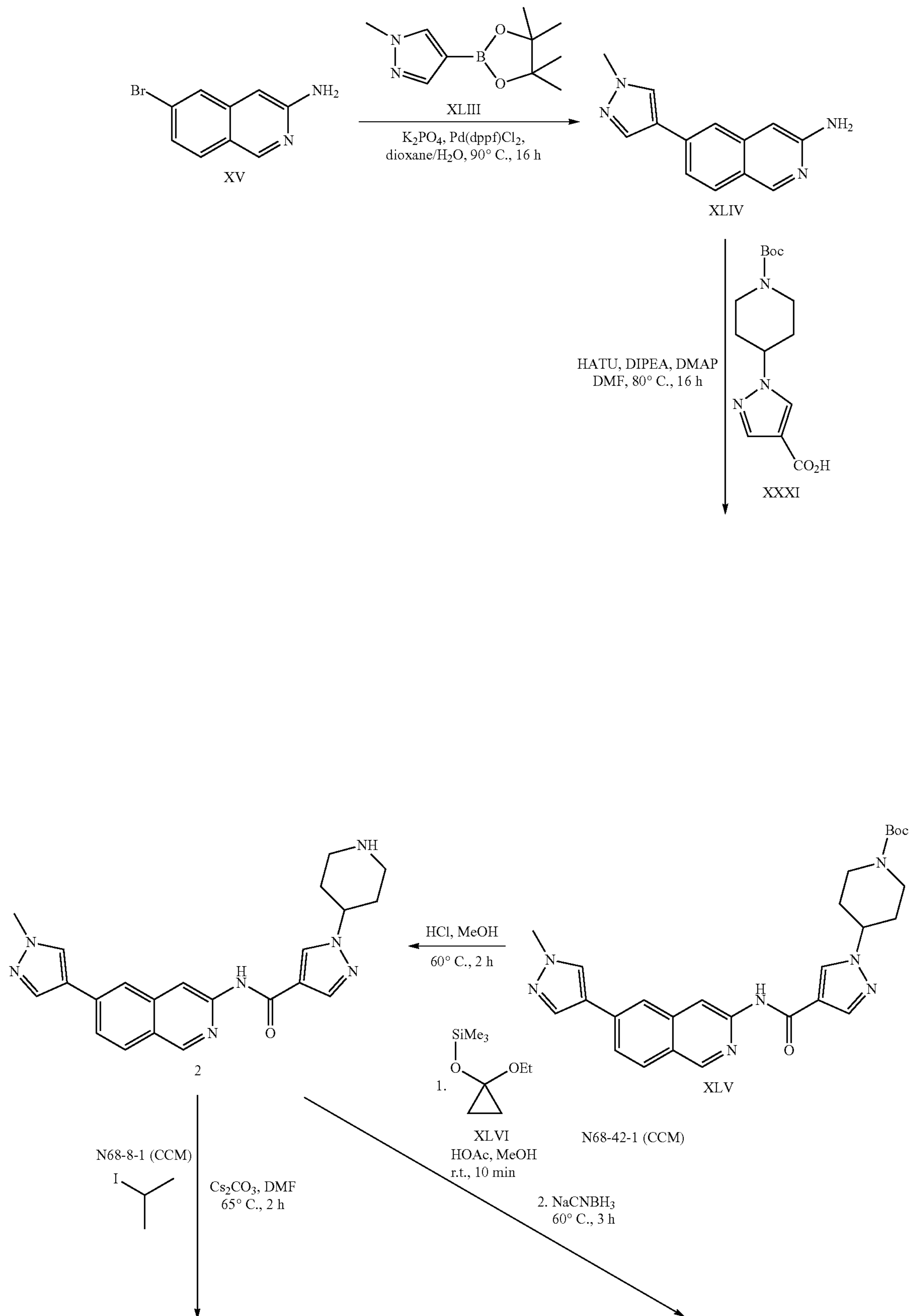
Scheme 13
