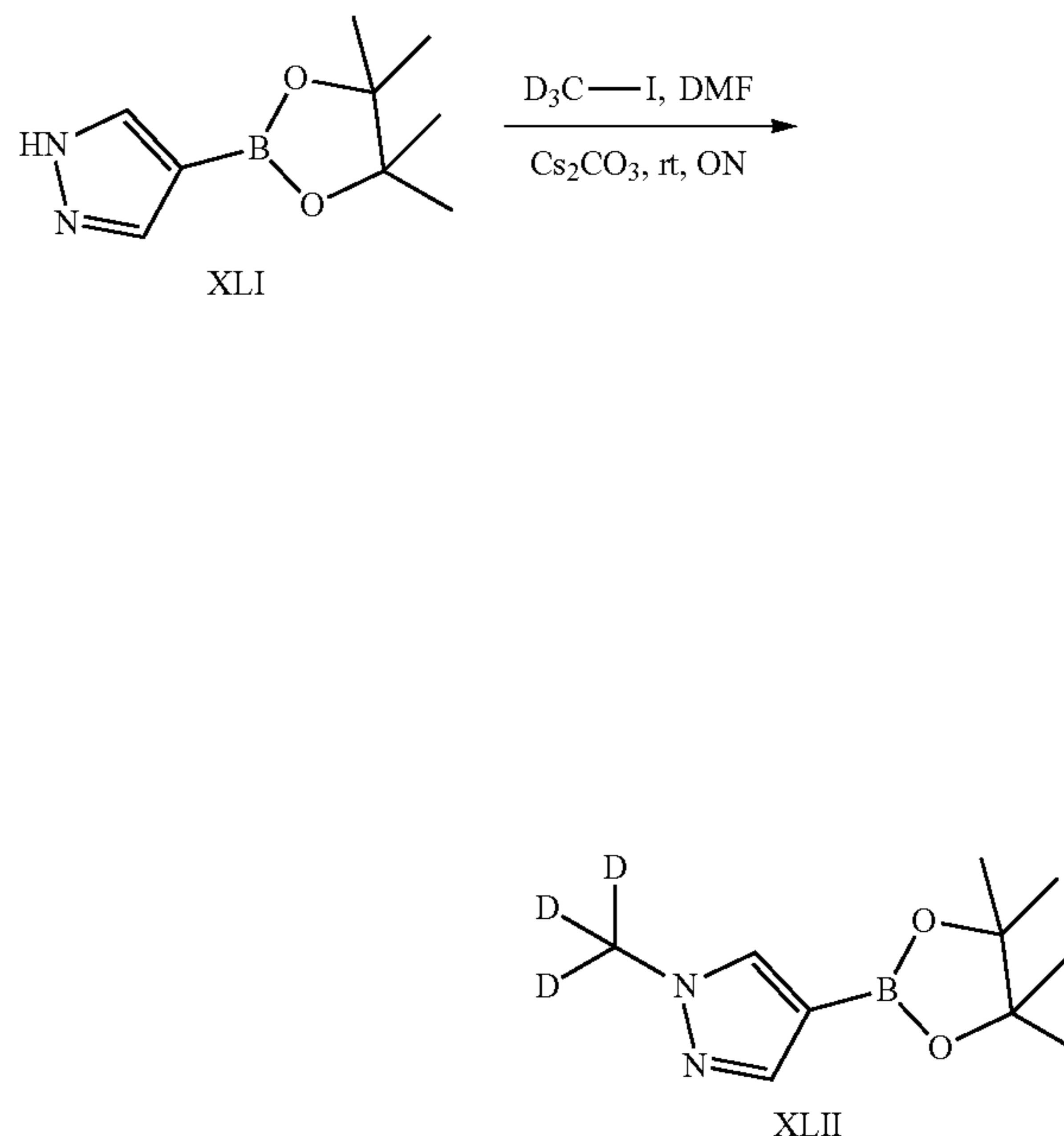
Scheme 12
