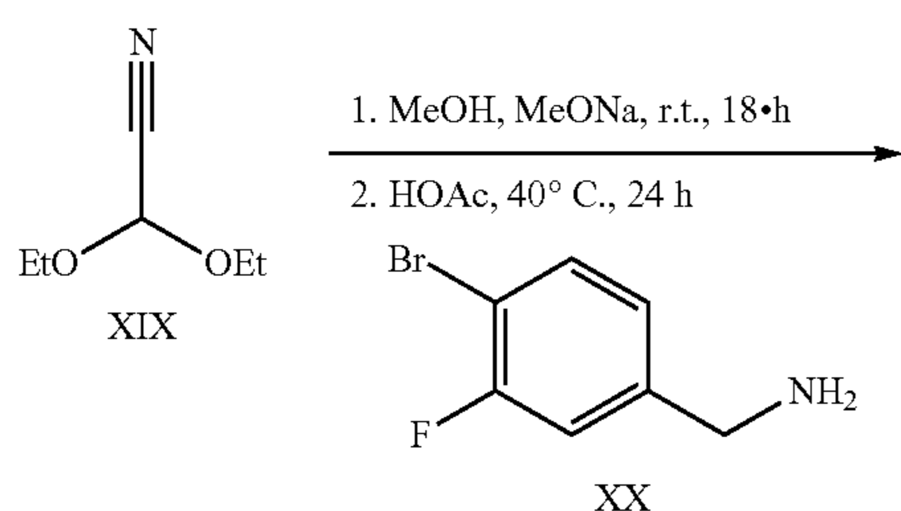
Scheme 6
