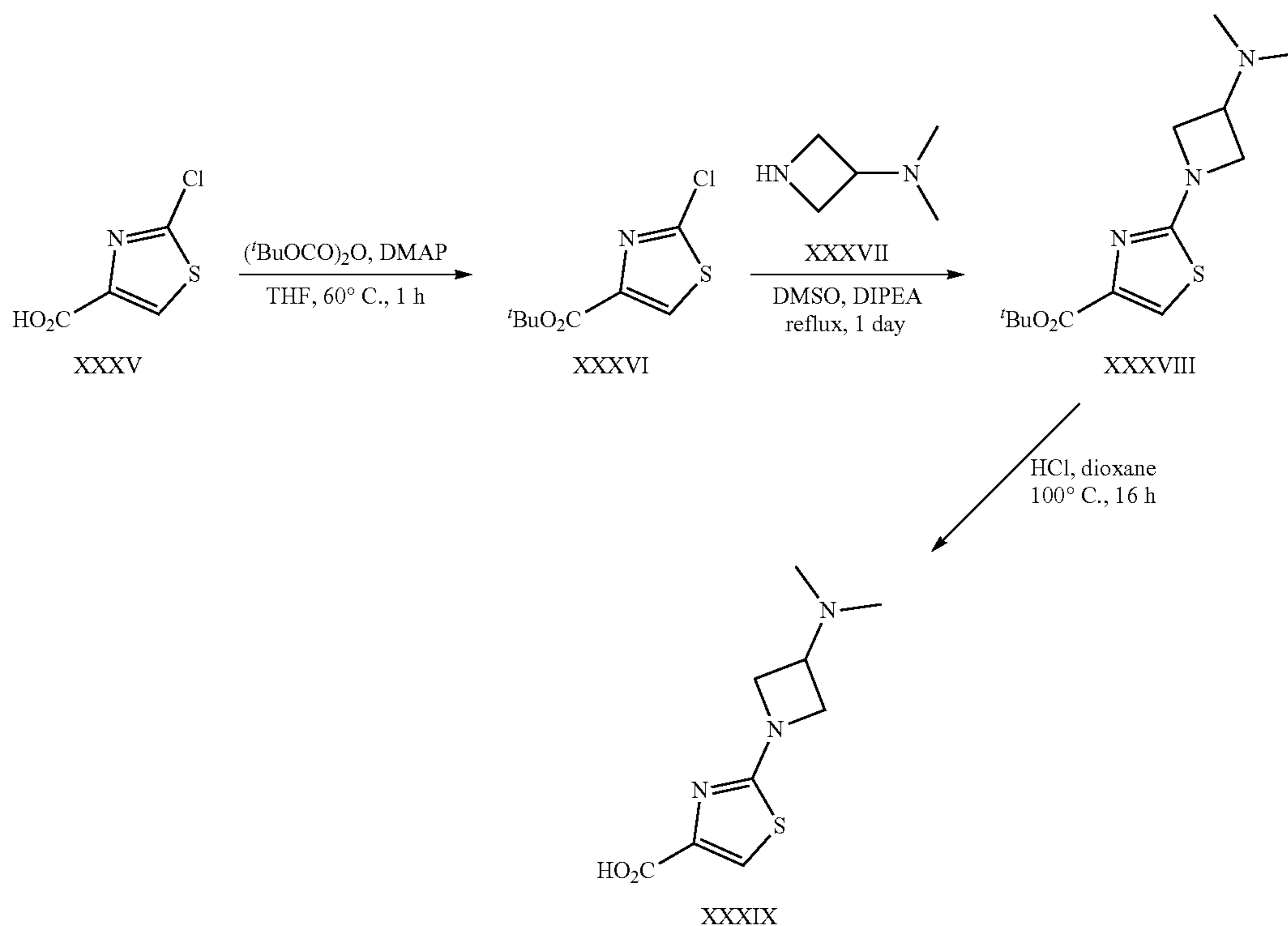
Scheme 11
