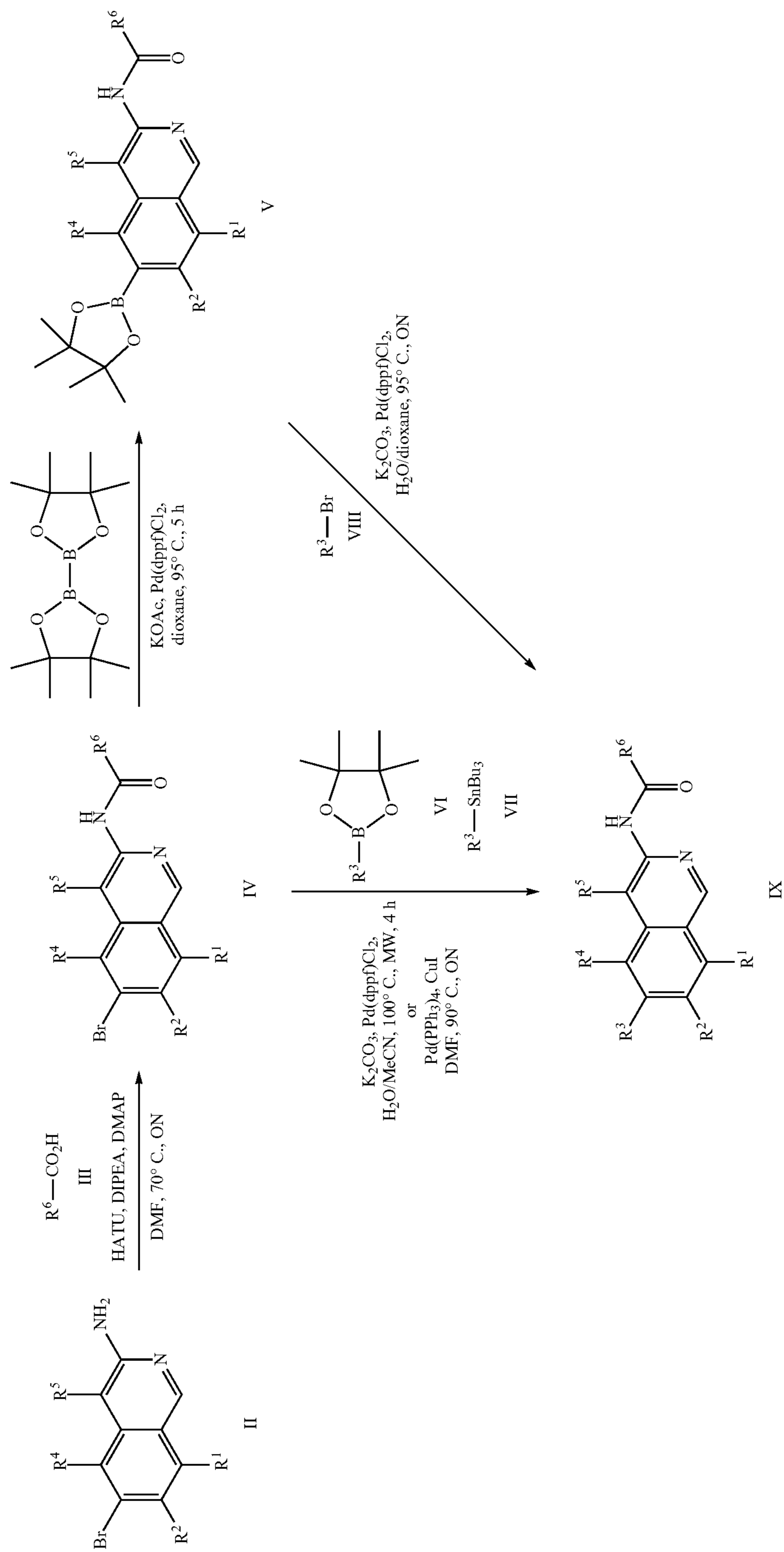
Scheme 1
