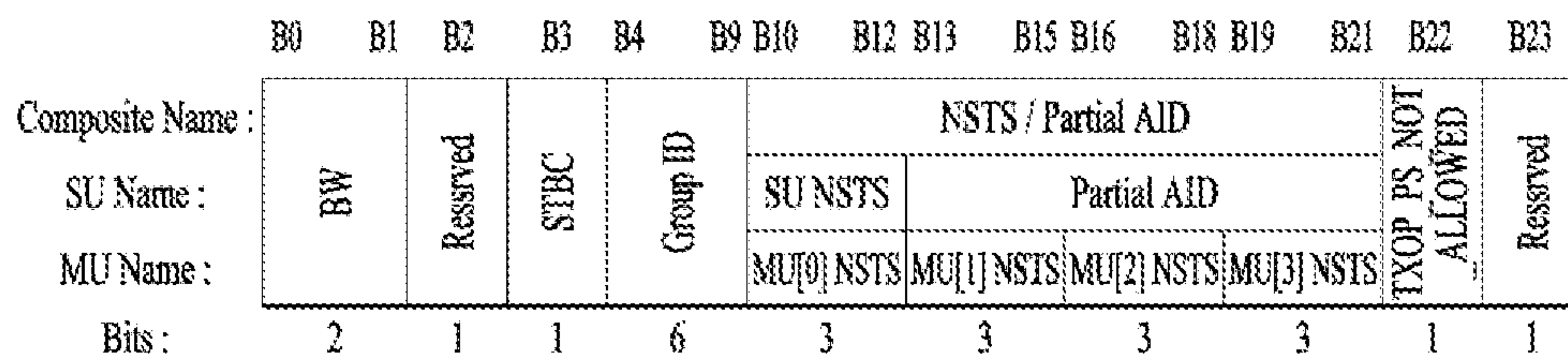
( a ) VHT-SIG-A1 structure
