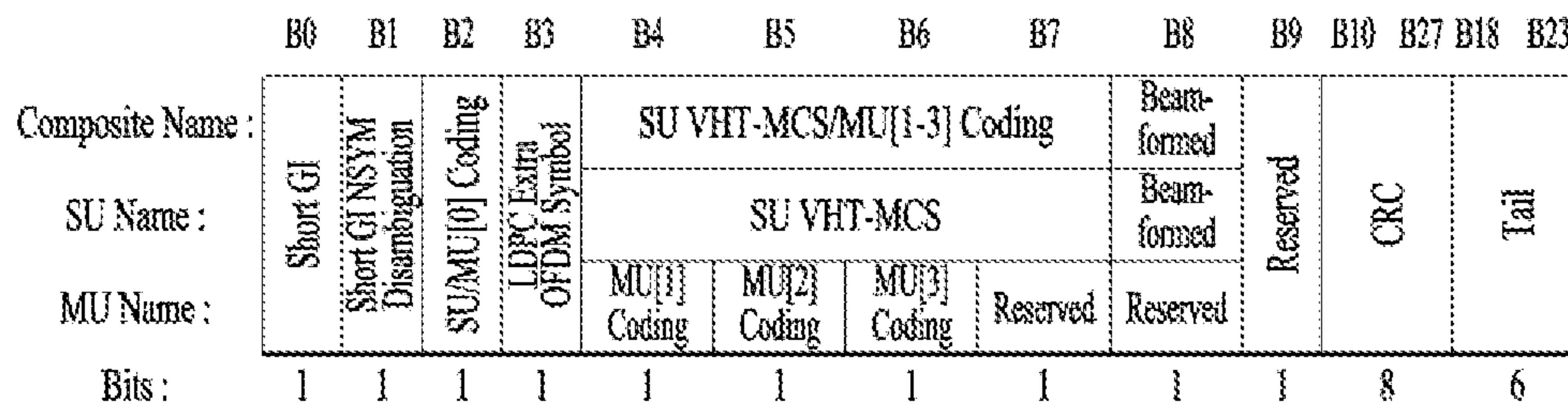
( b ) VHT-SIG-A2 structure
