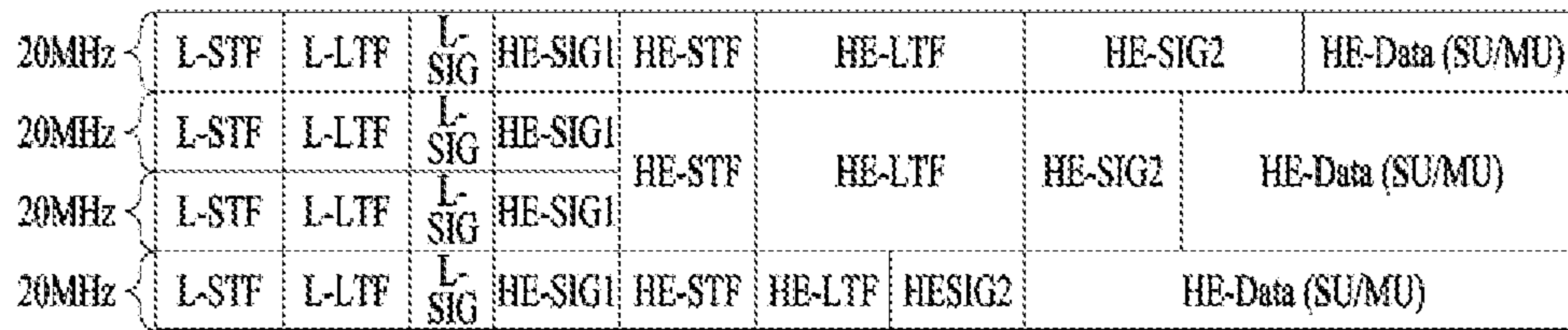
(b) HE PPDU format
