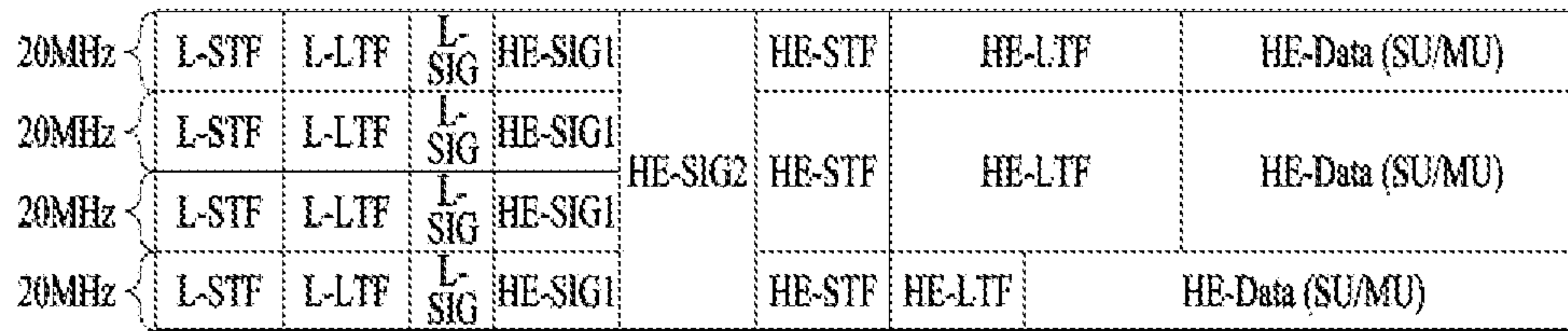
(c) HE PPDU format
