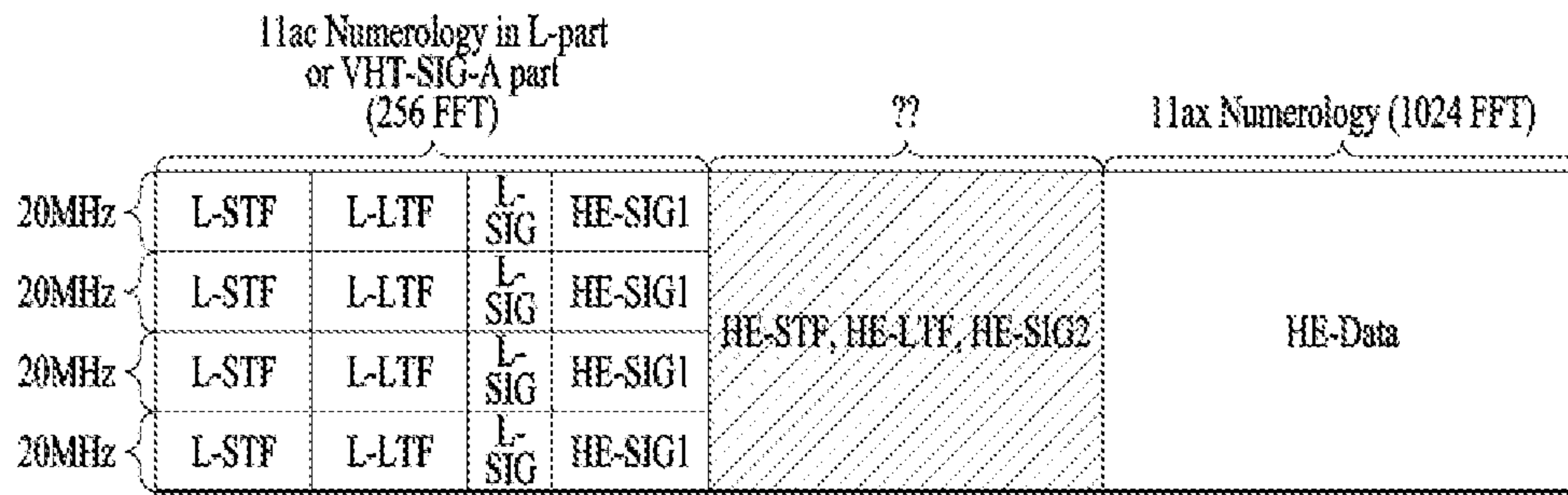
(a) HE PPDU format
