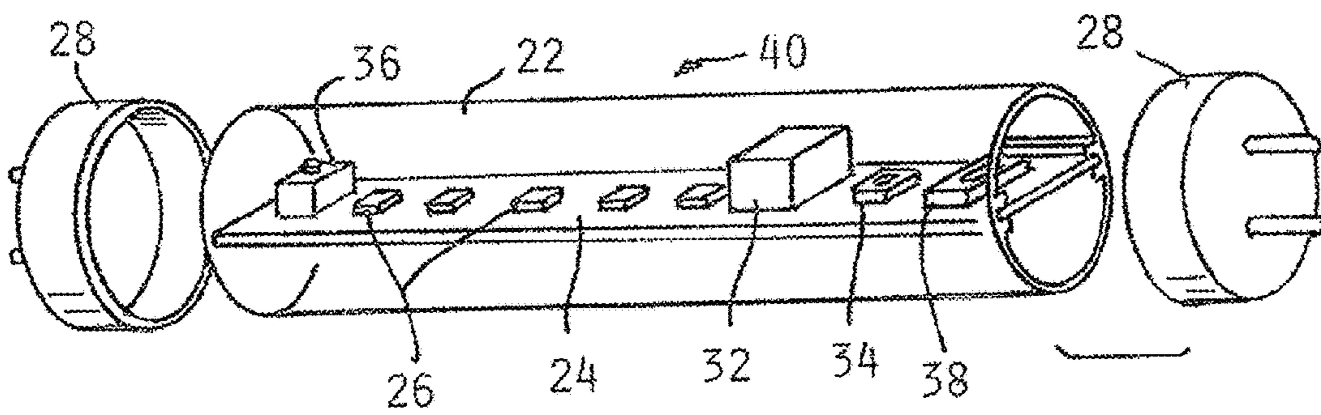
FIG. 2 (PRIOR ART)
