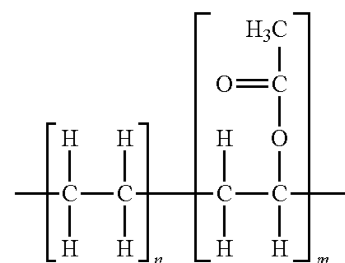
Ethylene-vinyl acetate
