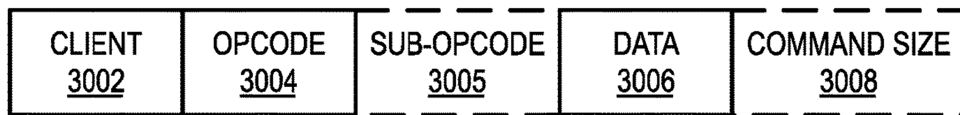
FIG. 30A GRAPHICS PROCESSOR COMMAND FORMAT 3000
