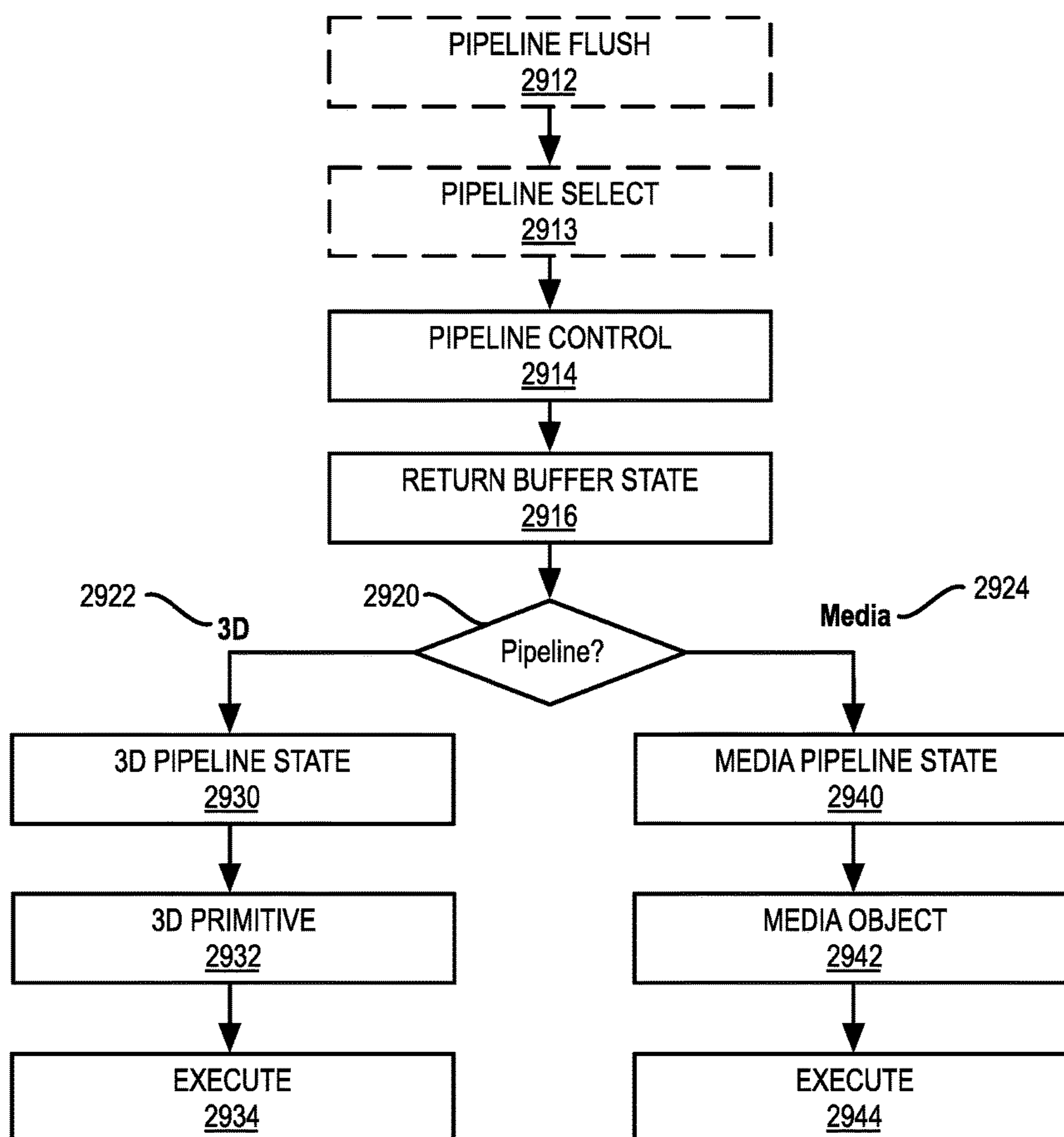
FIG. 29B GRAPHICS PROCESSOR COMMAND SEQUENCE 2910
