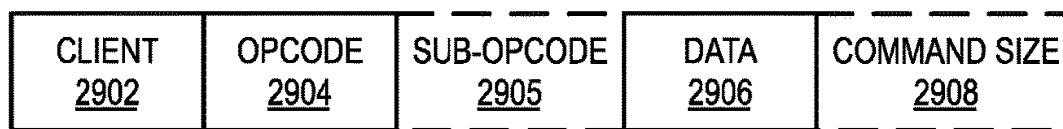
FIG. 29A GRAPHICS PROCESSOR COMMAND FORMAT 2900
