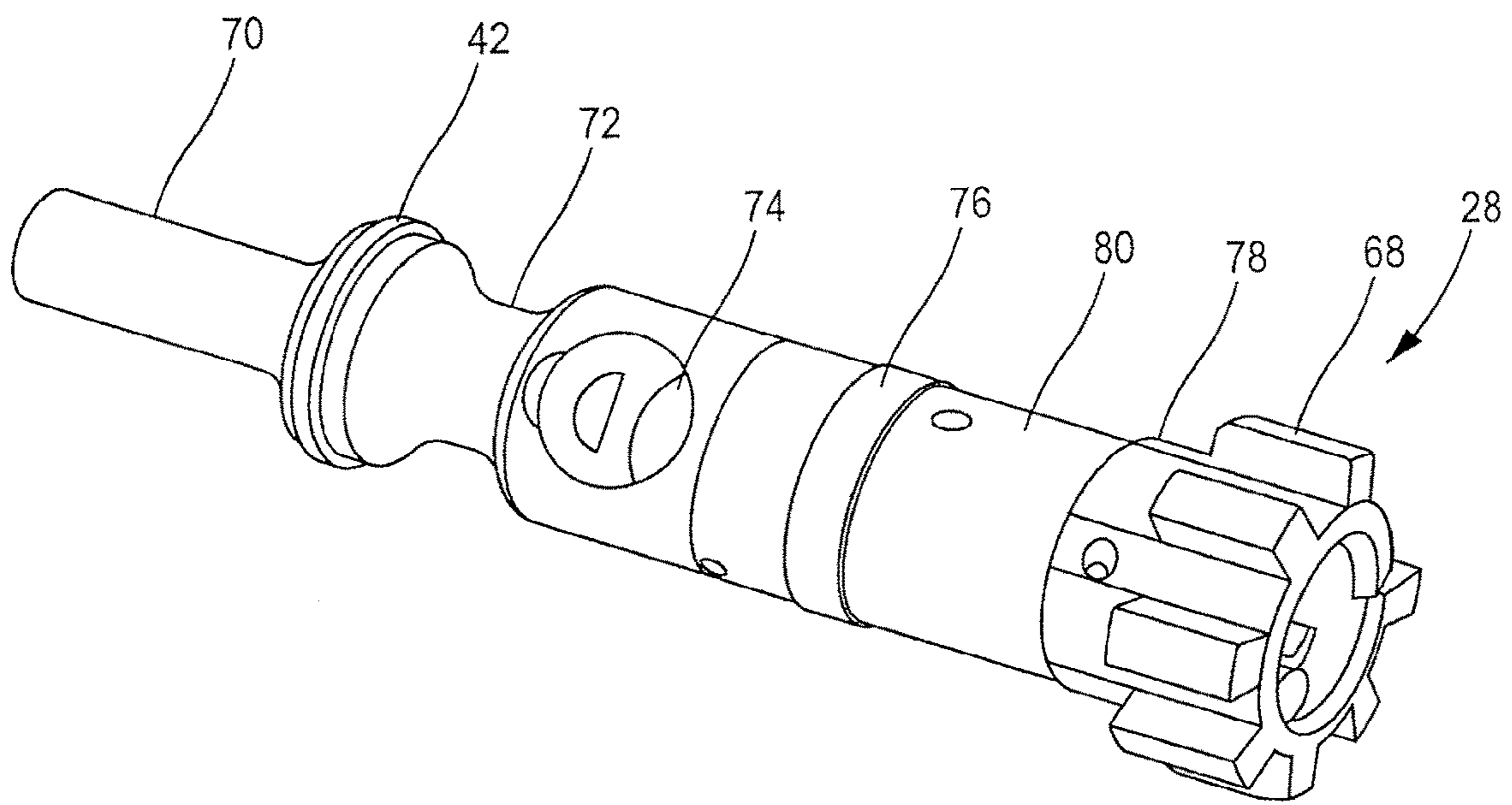
Fig.16 PRIOR ART
