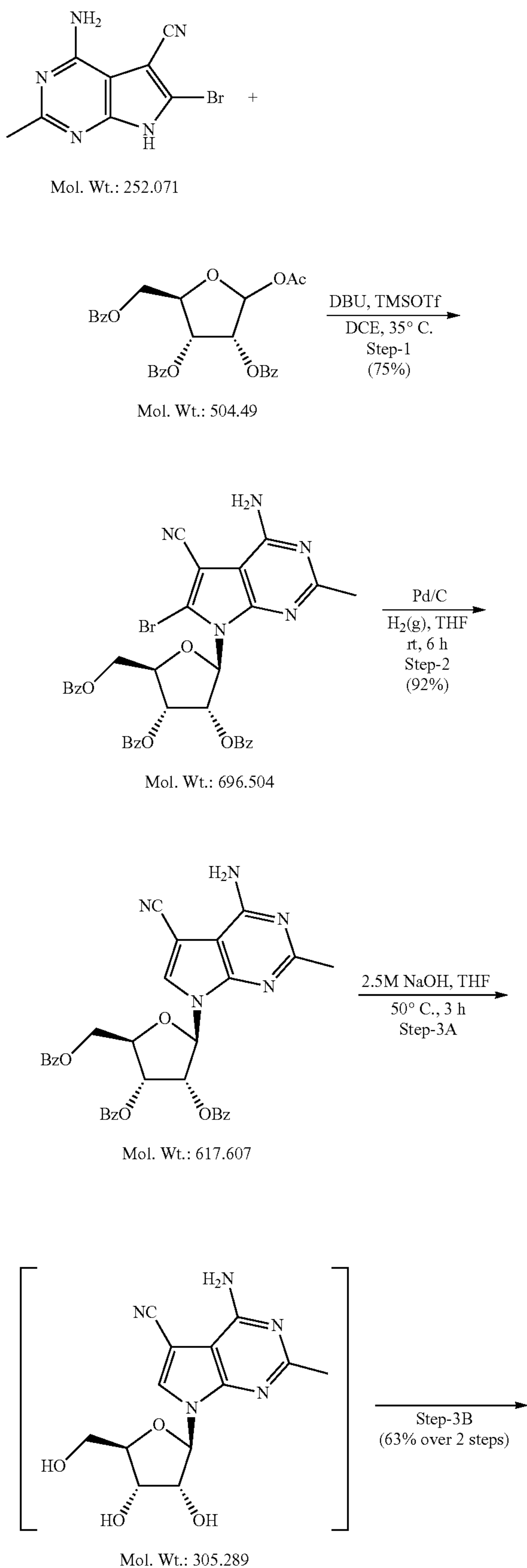
Scheme 2: General Synthesis of Compounds of the Invention
