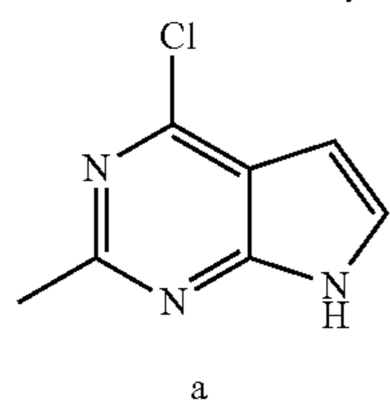
Scheme 1: General Synthesis of Compounds of the Invention
