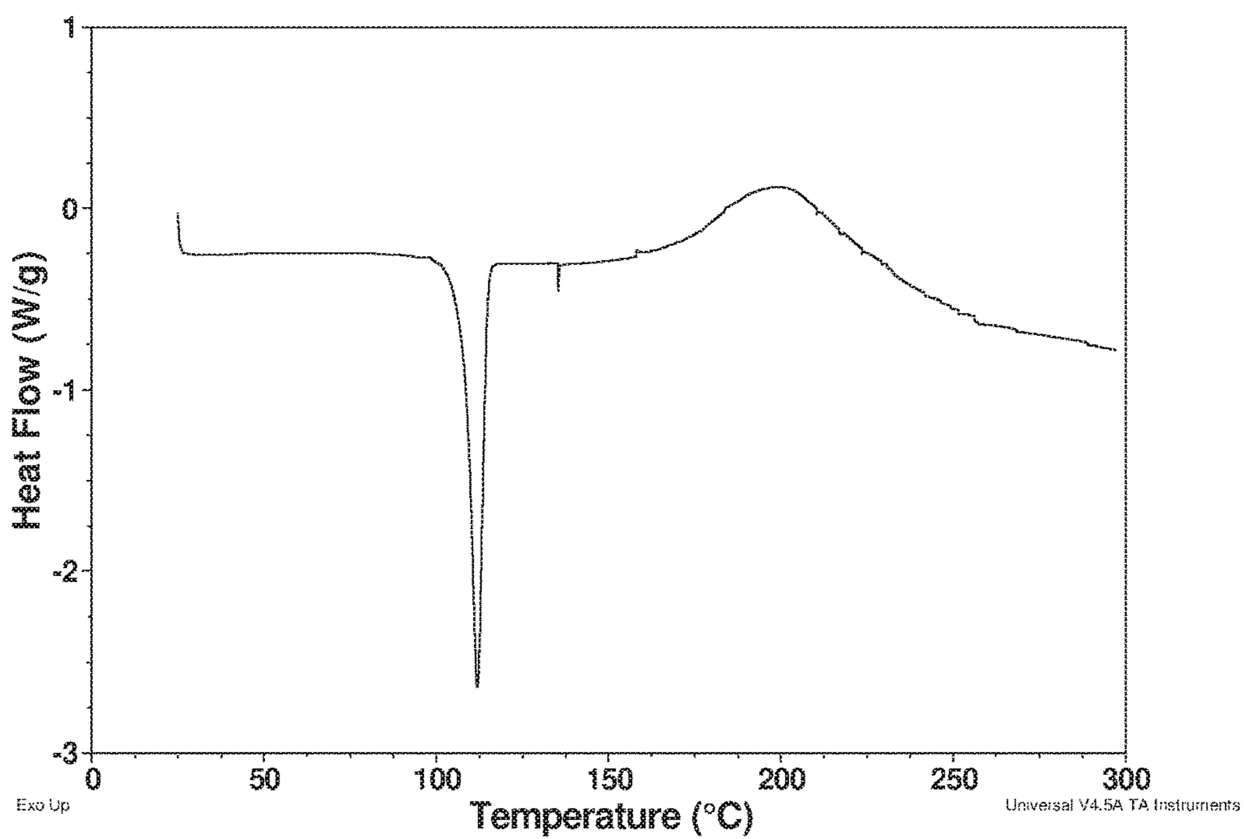
Figure 2: DSC Thermogram Compound A, Form A
