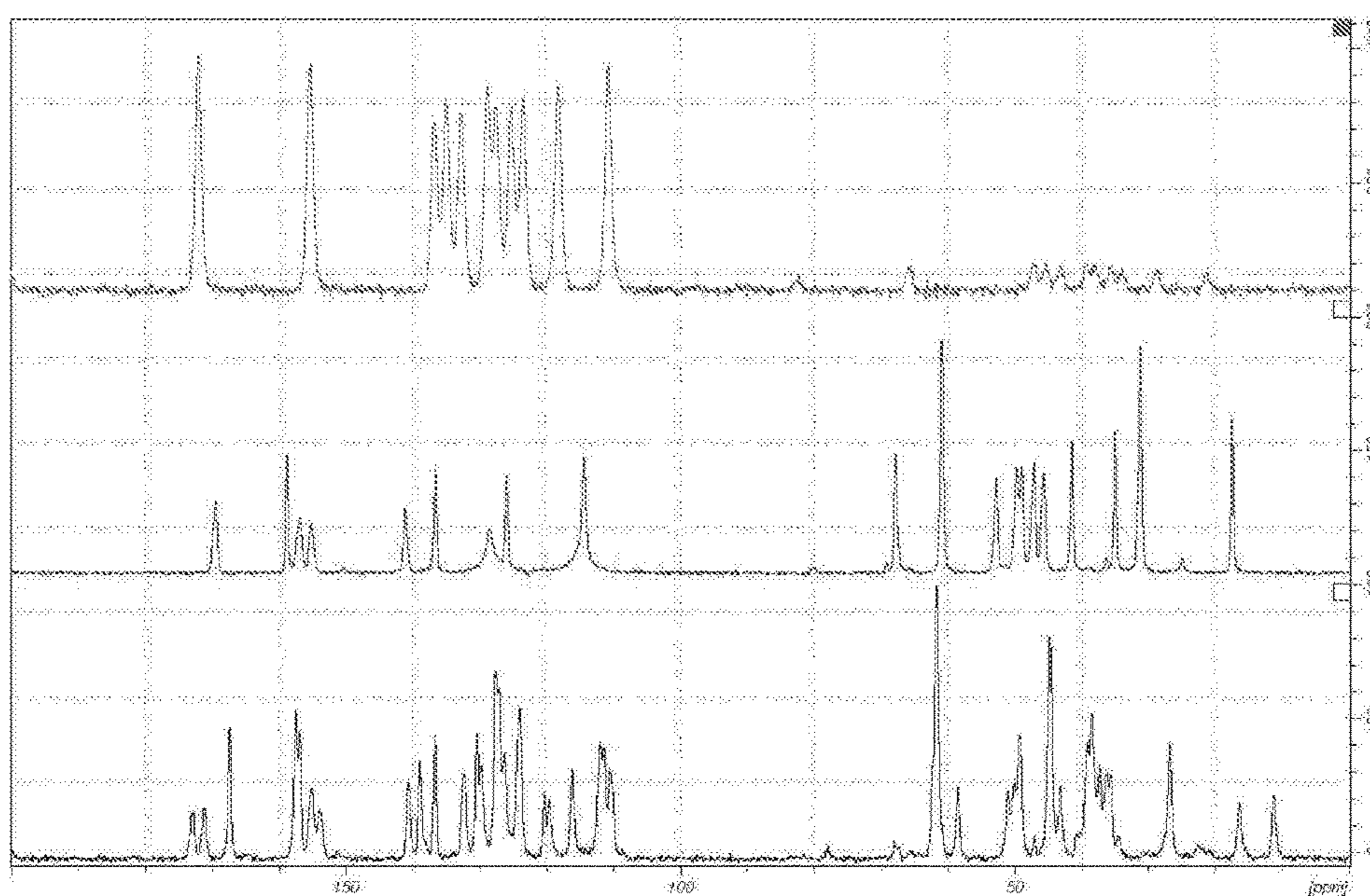
Figure 6: Stacked plot of 13 C ss NMR spectra
