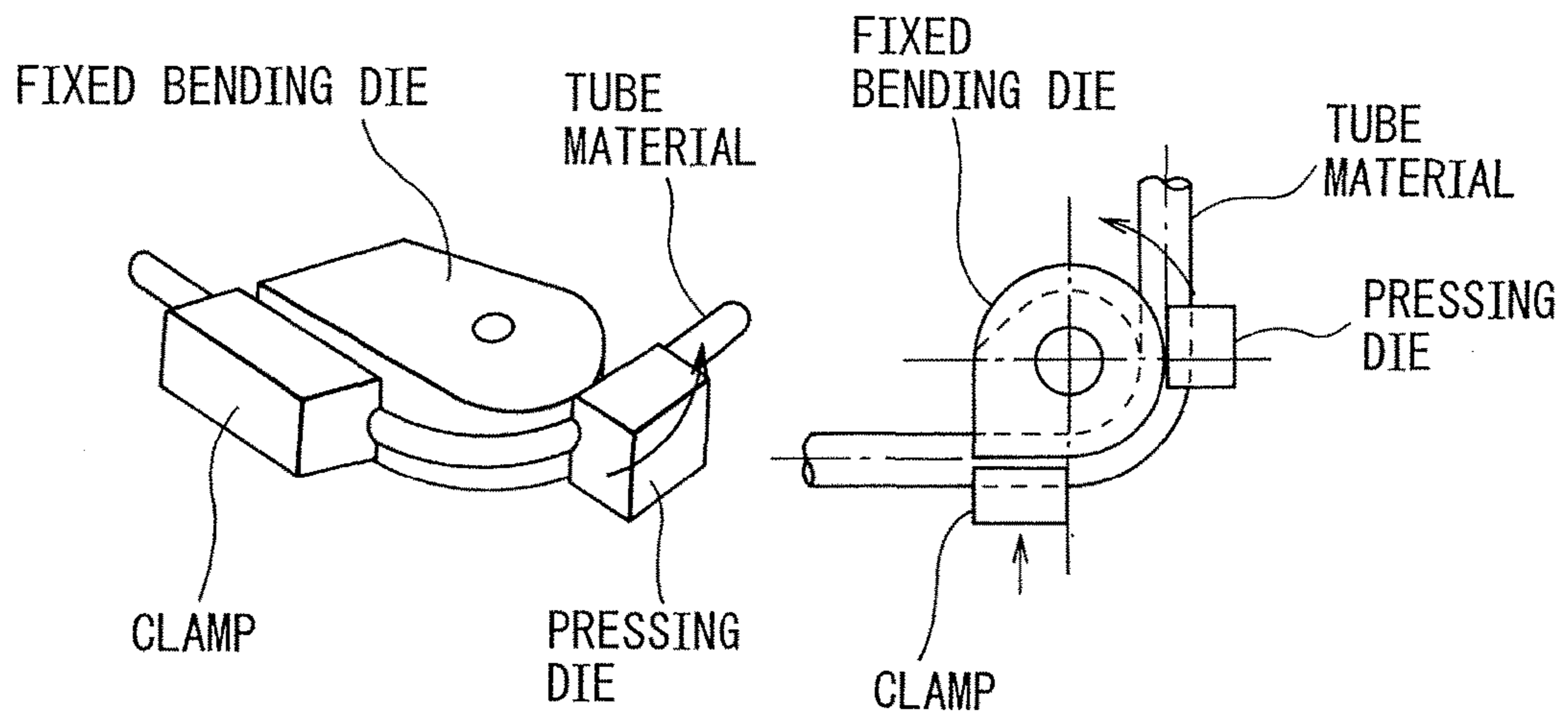
FIG. 3 (Prior Art)
