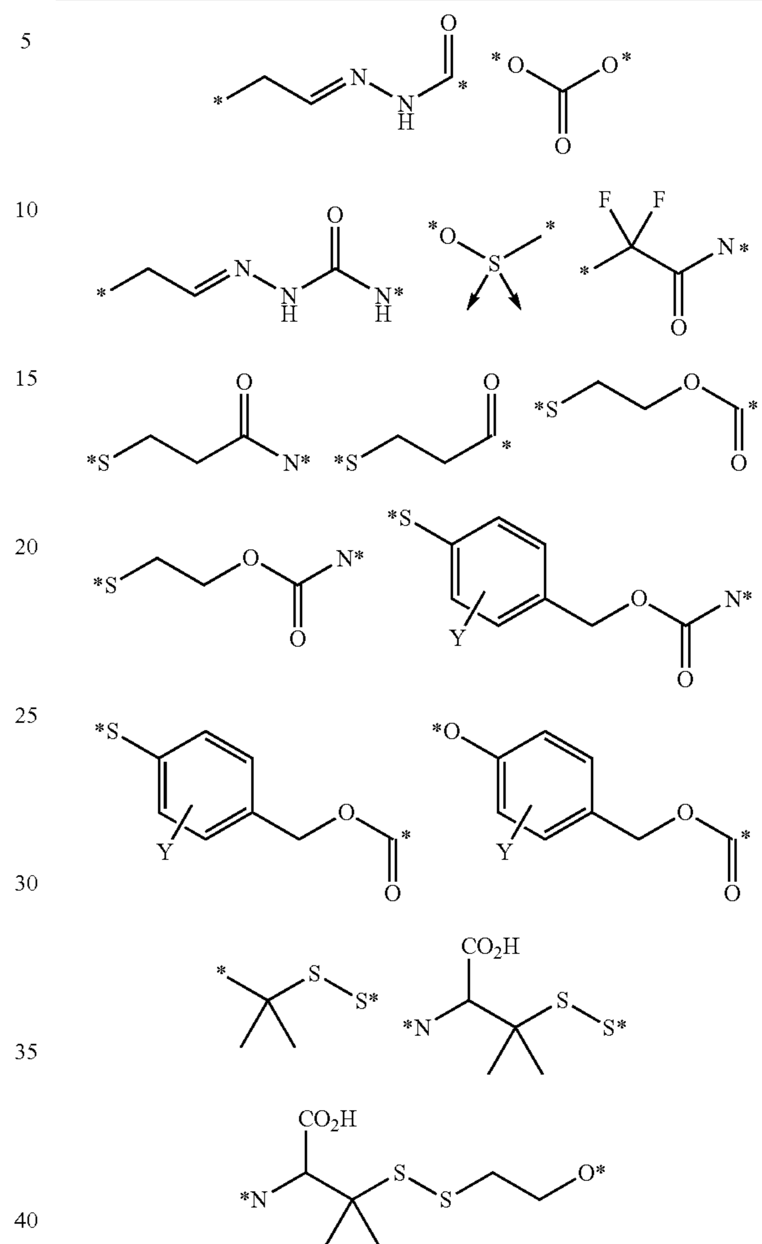
Illustrative releasable linkers.
