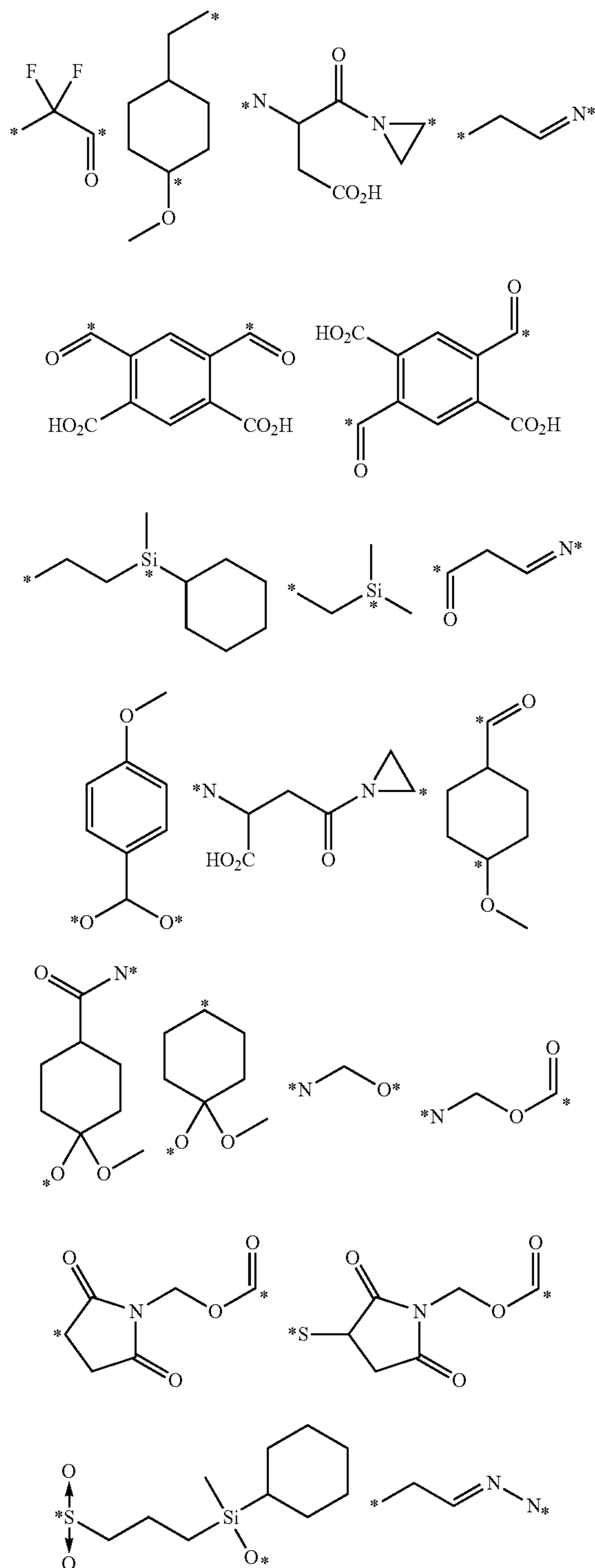
Illustrative releasable linkers.
