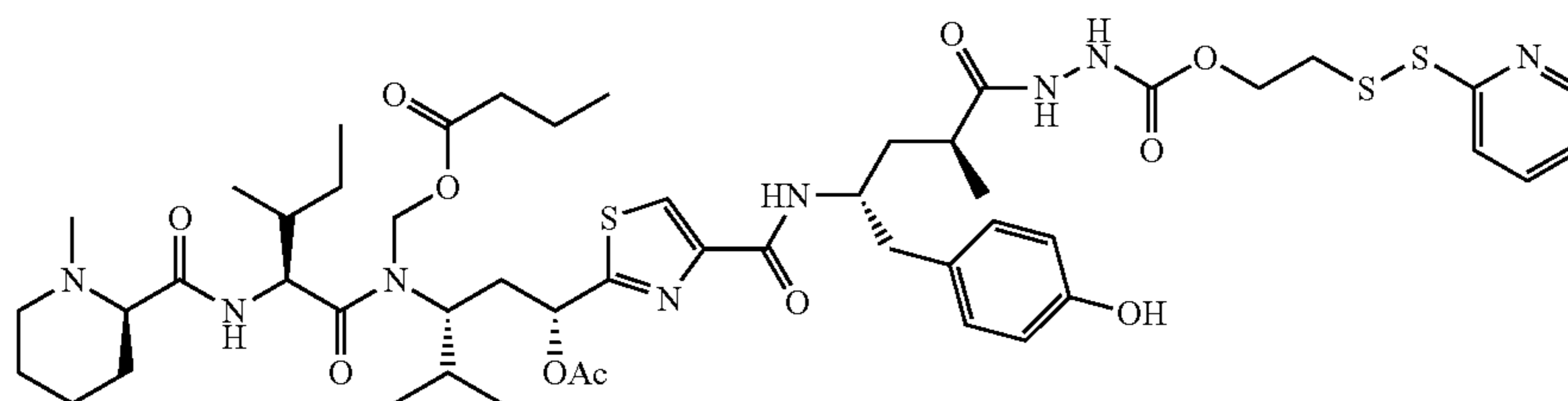
EC0312 C_{50}H_{72}N_8O_{11}S_3 Mol. Wt.: 1057.35
