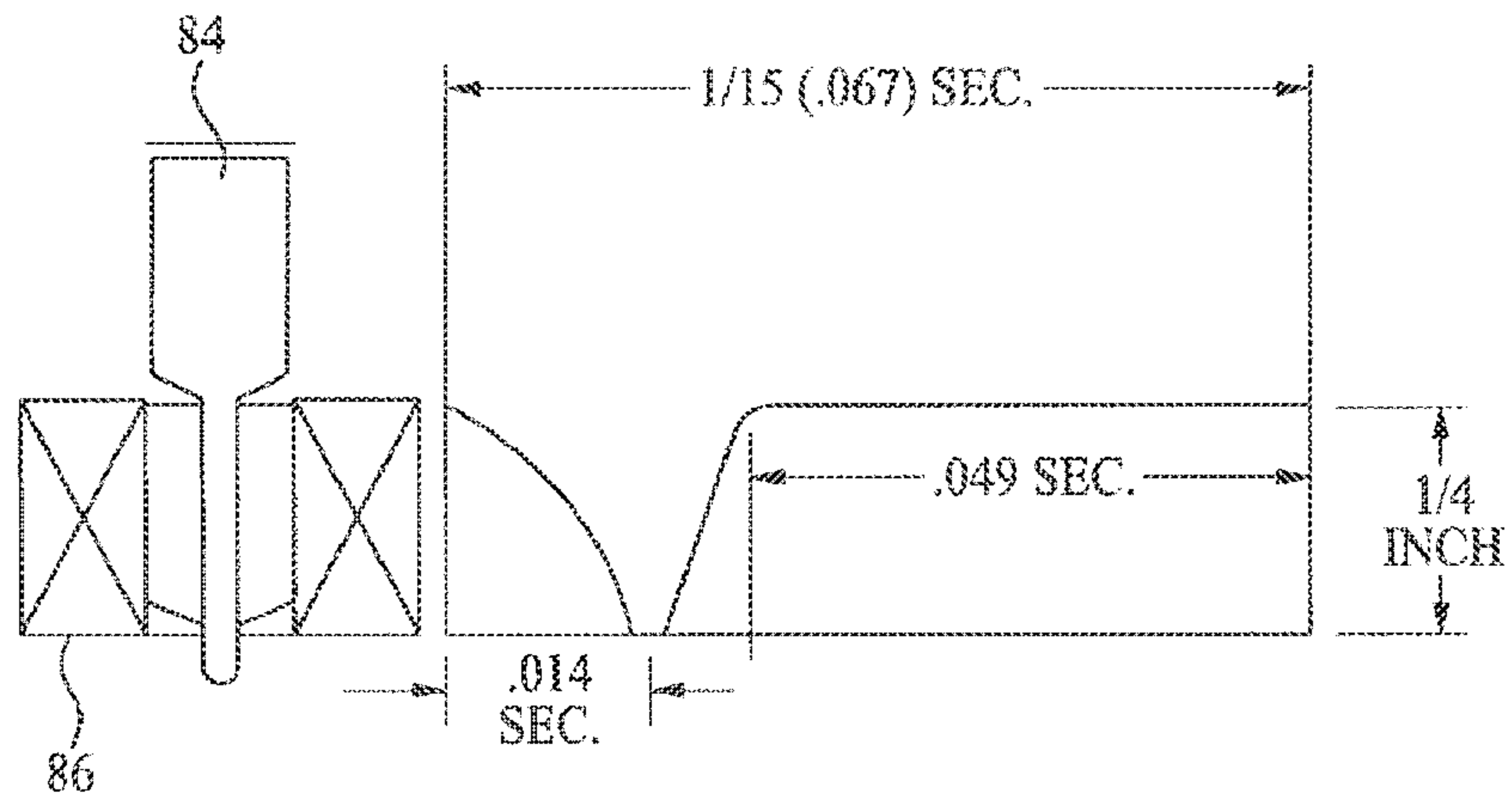
FIG. 2C PRIOR ART
