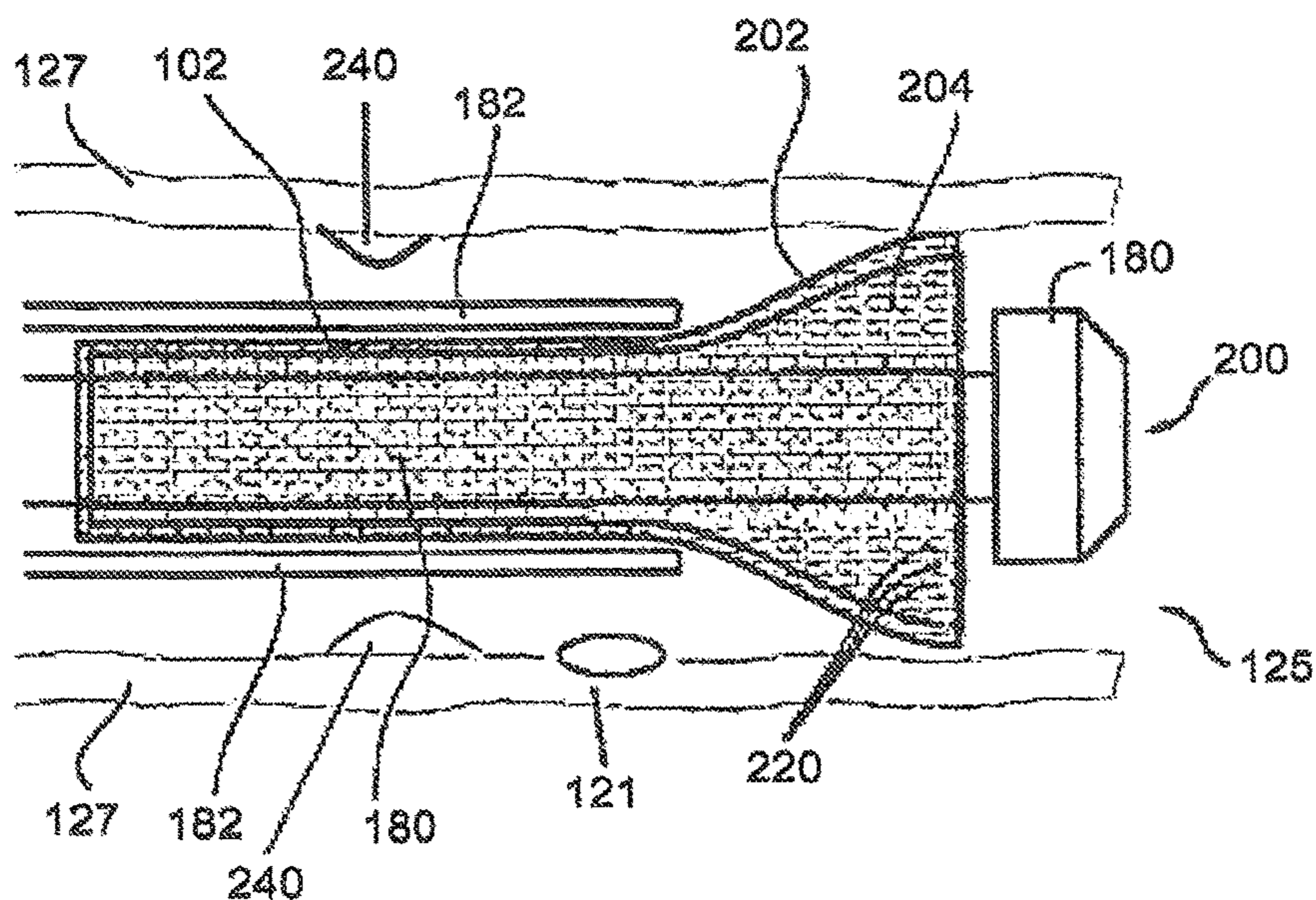
Fig. 24c (Prior Art)
