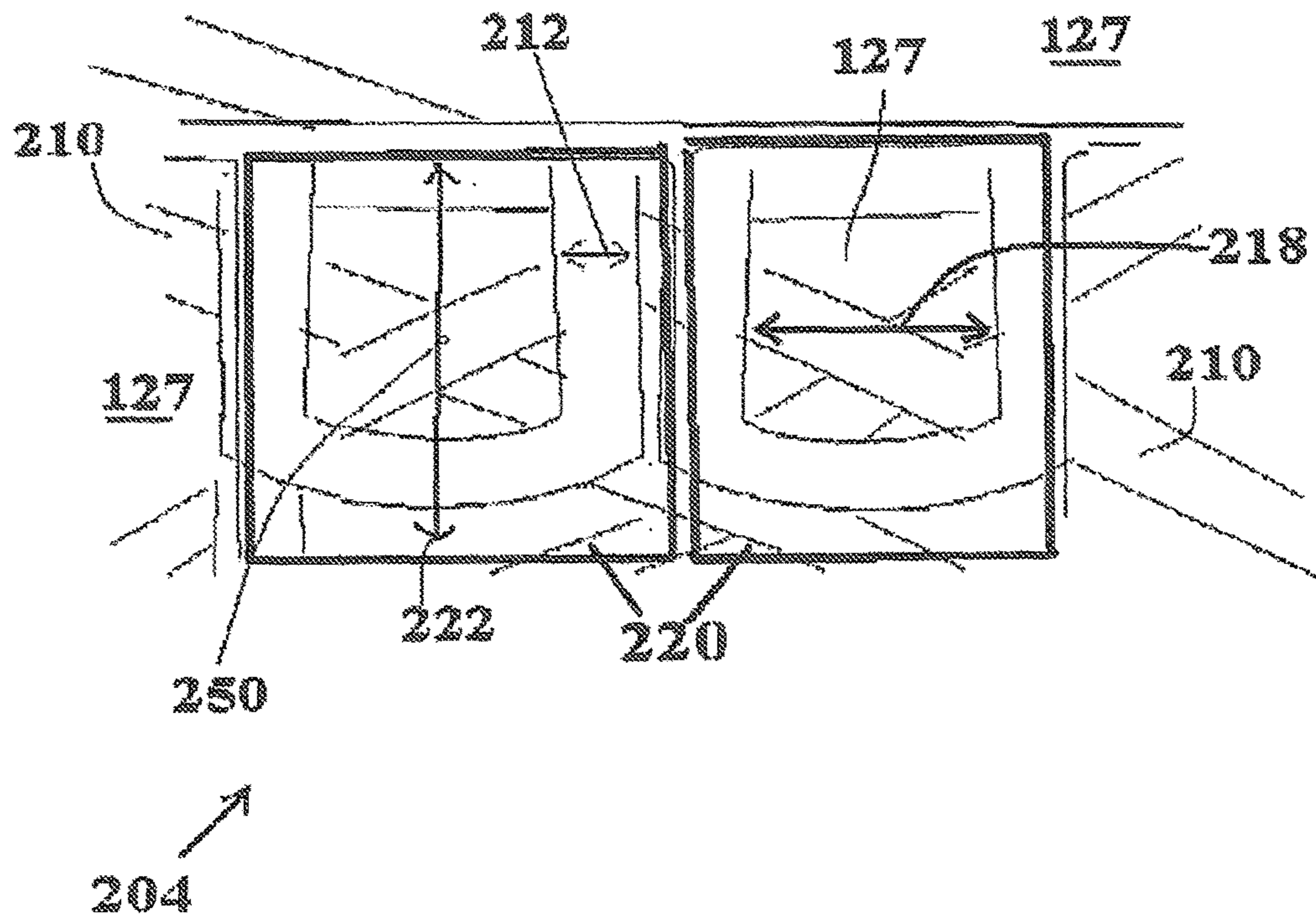
Fig. 25 (Prior Art)
