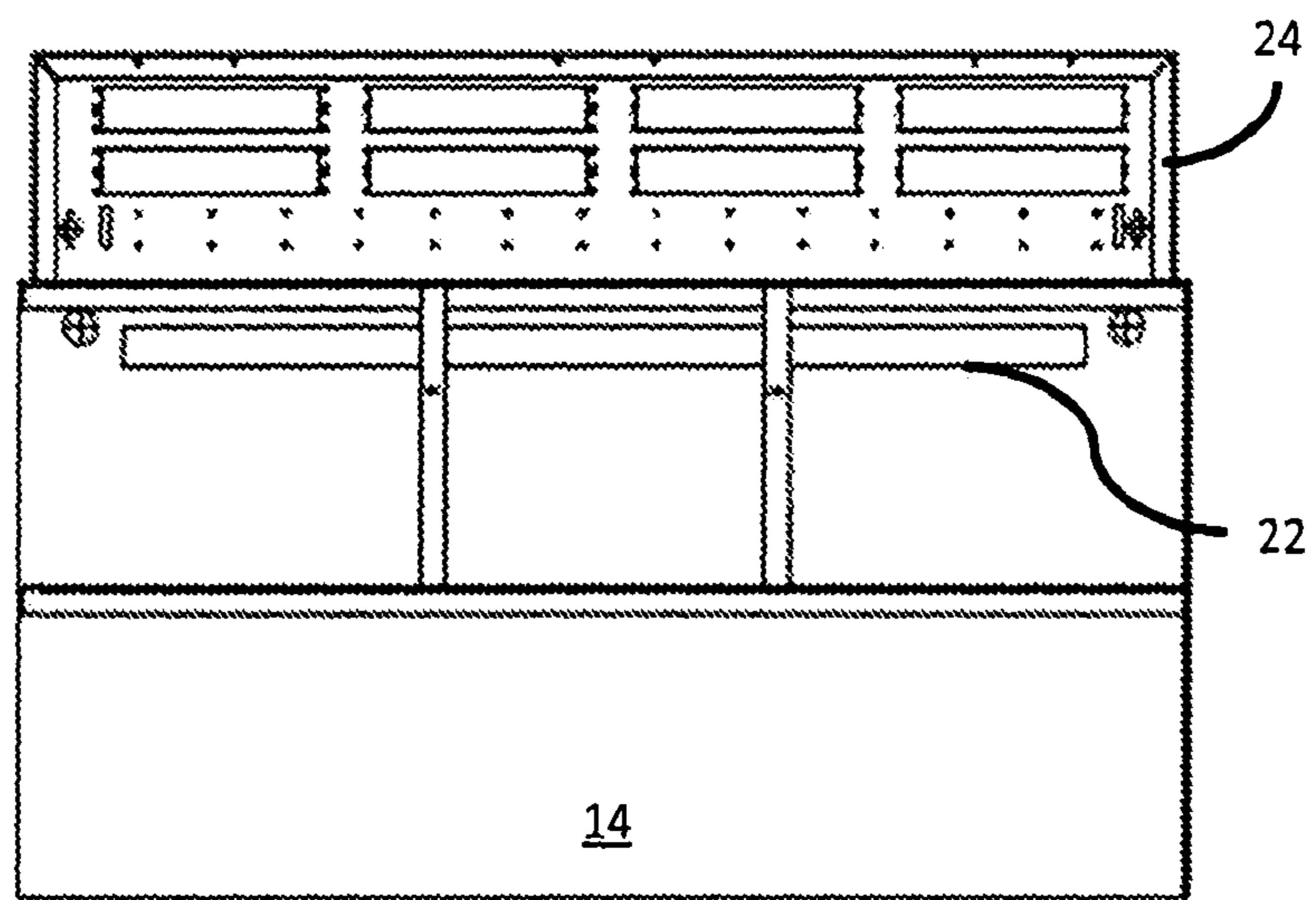
Section C-C Fig. 6
