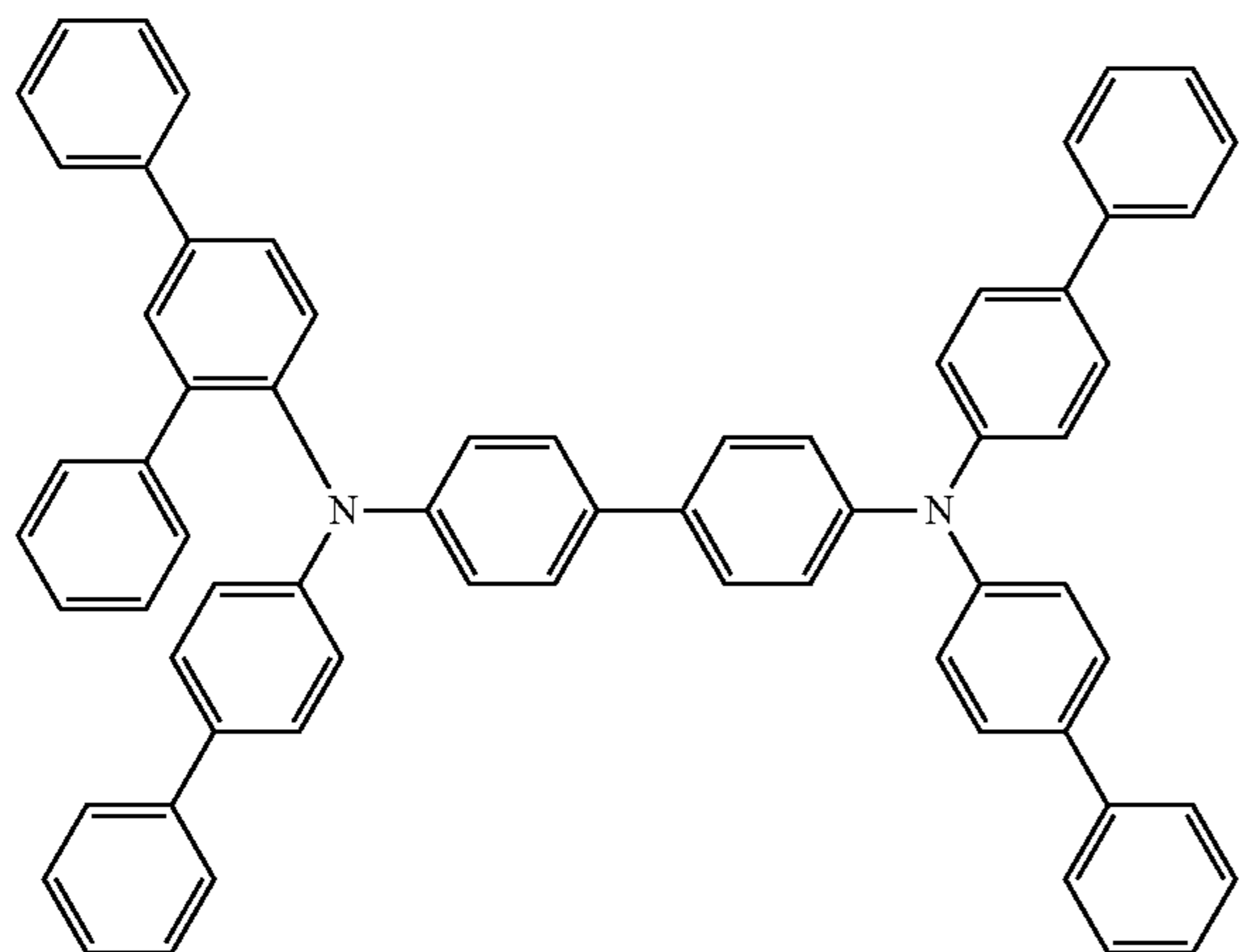
PPh-TPD
