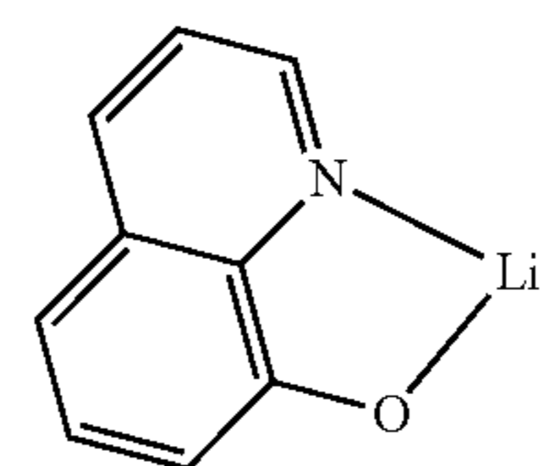
LiQ
