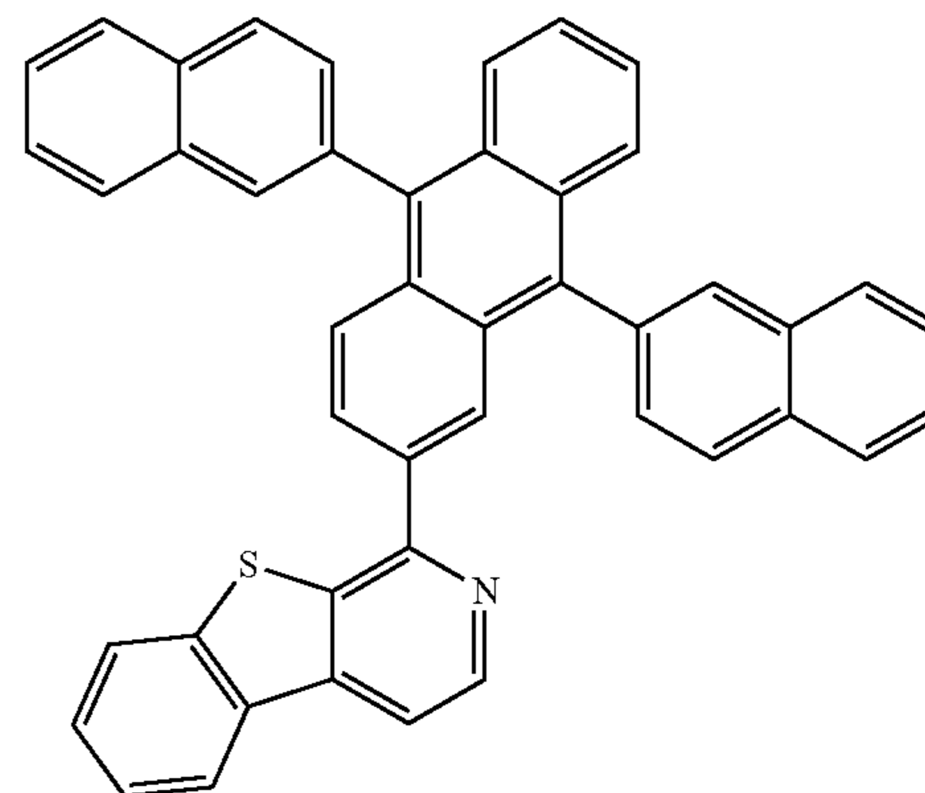
aDBT-ADN
