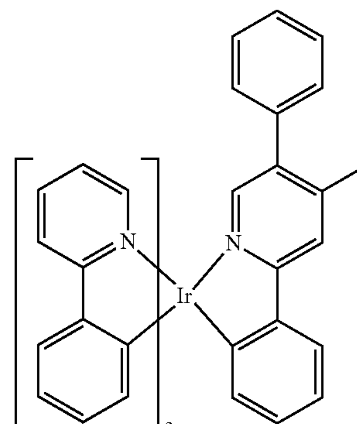
GD
