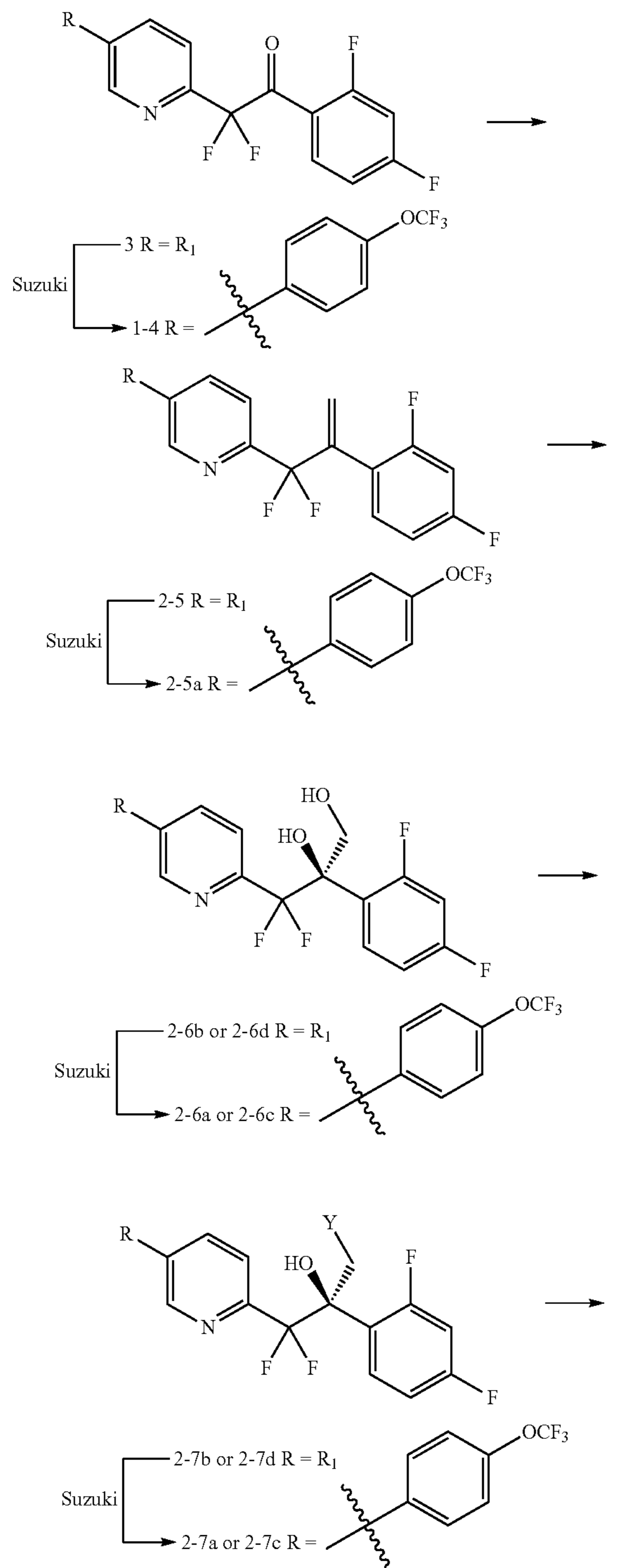
Scheme 3. Synthesis of 1 via Asymmetric Dihydroxylation Method
