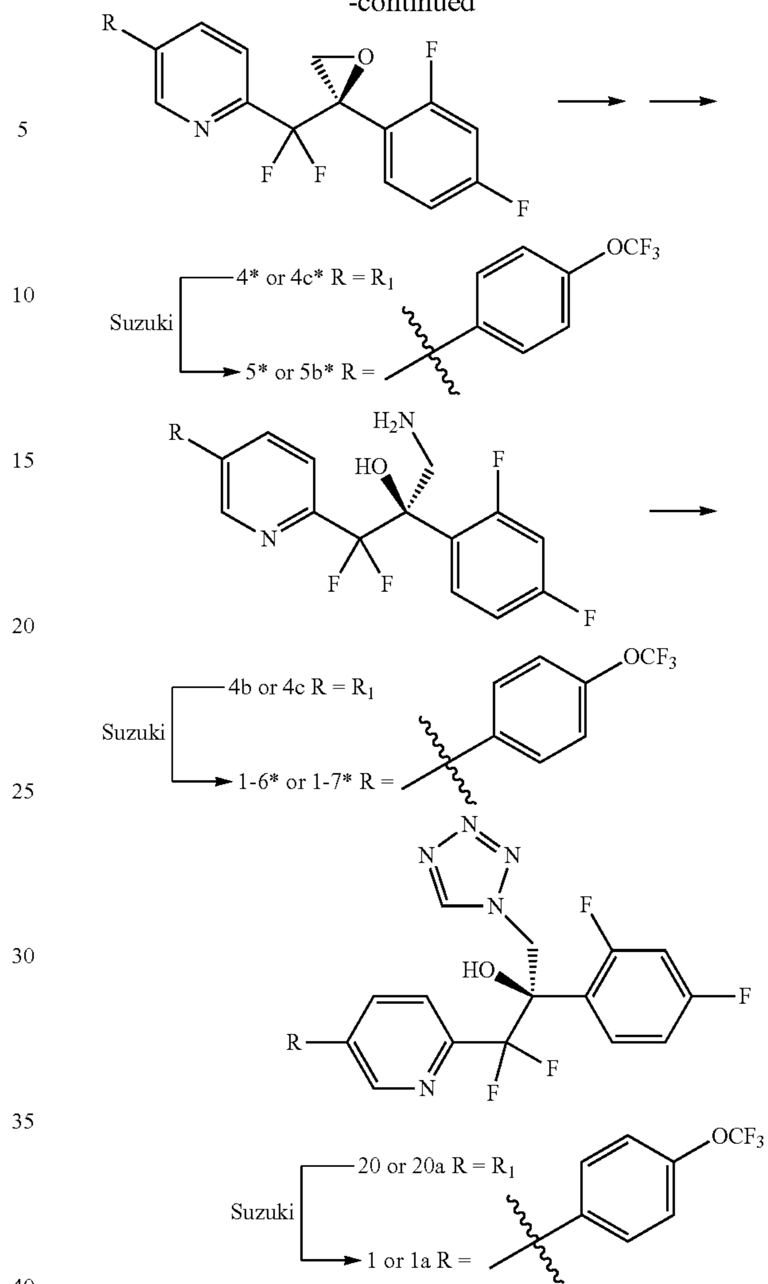
Scheme 3. Synthesis of 1 via Asymmetric Dihydroxylation Method
