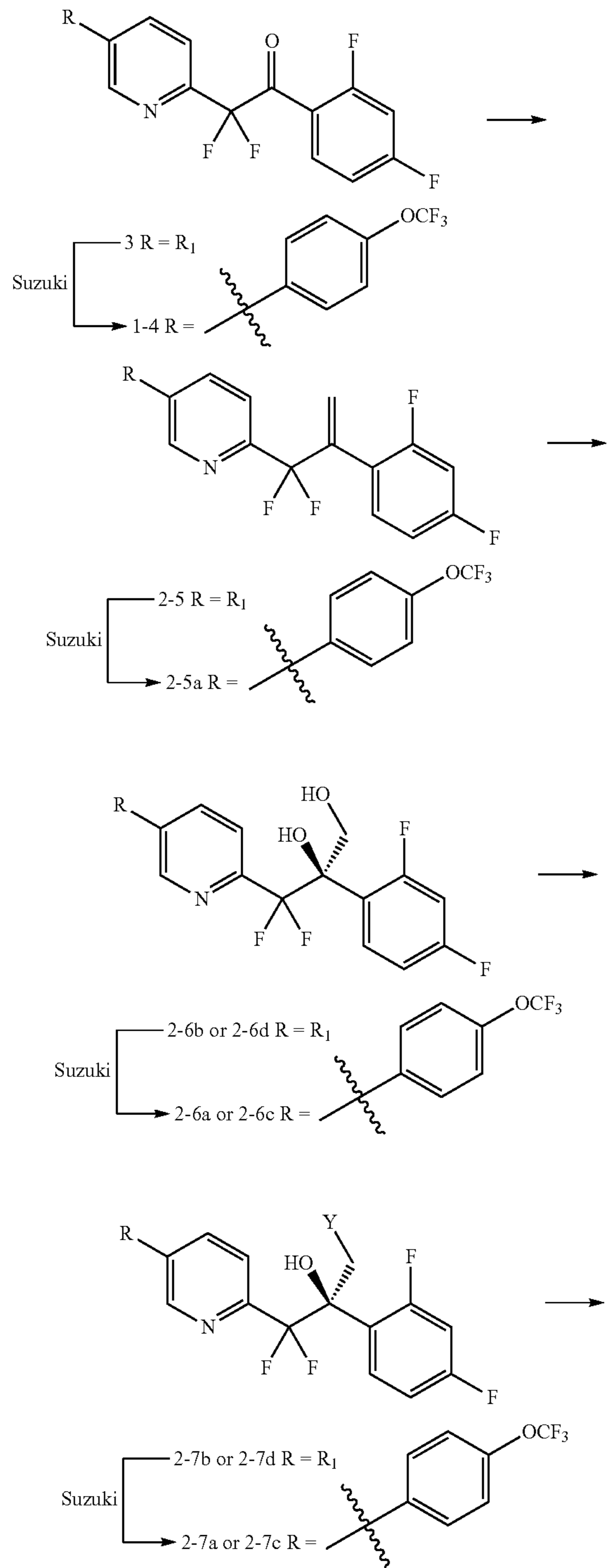
Scheme 3. Synthesis of 1 via Asymmetric Dihydroxylation Method
