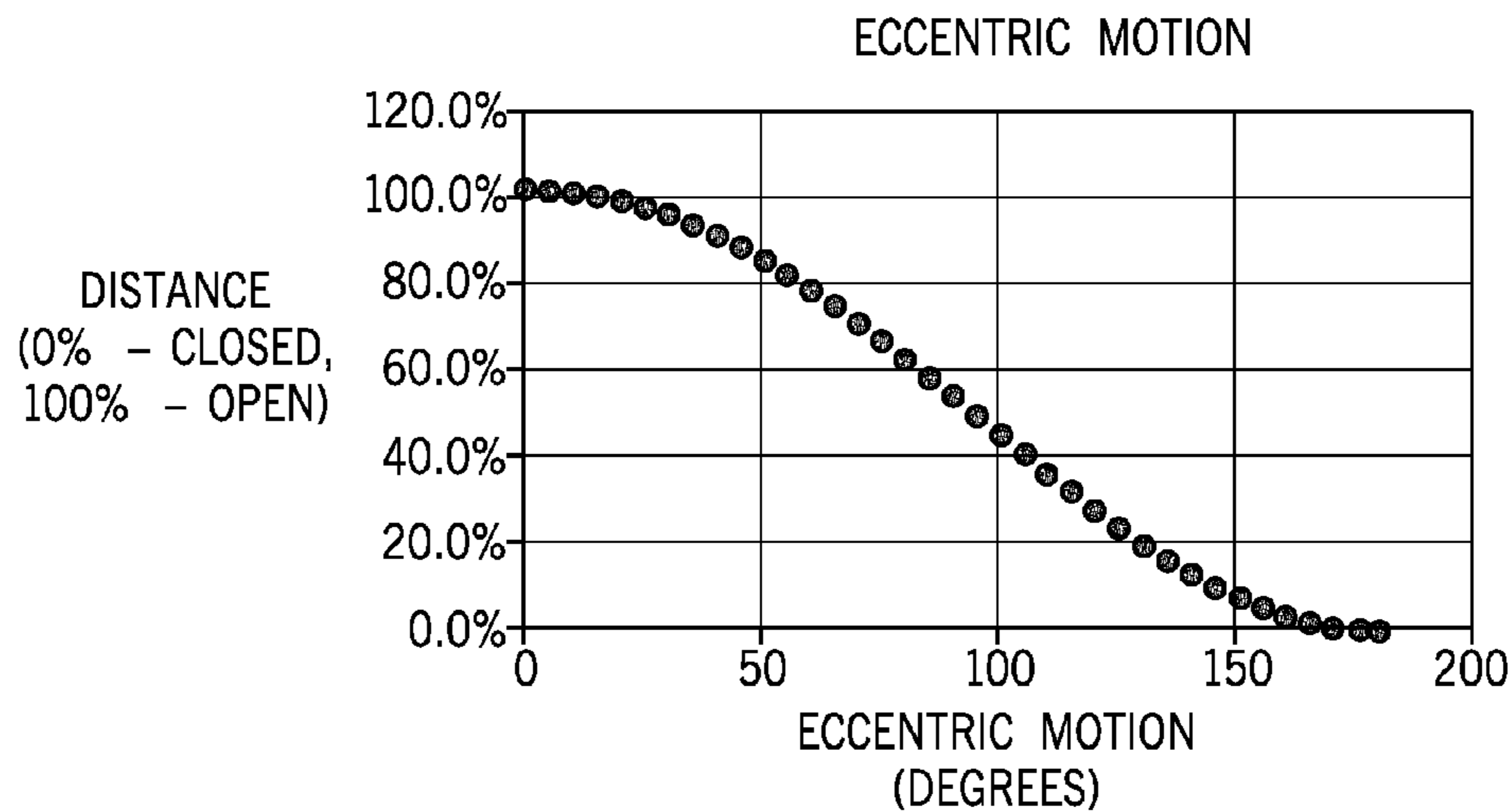
HEAD POSITION VERSUS ECCENTRIC MOTION
