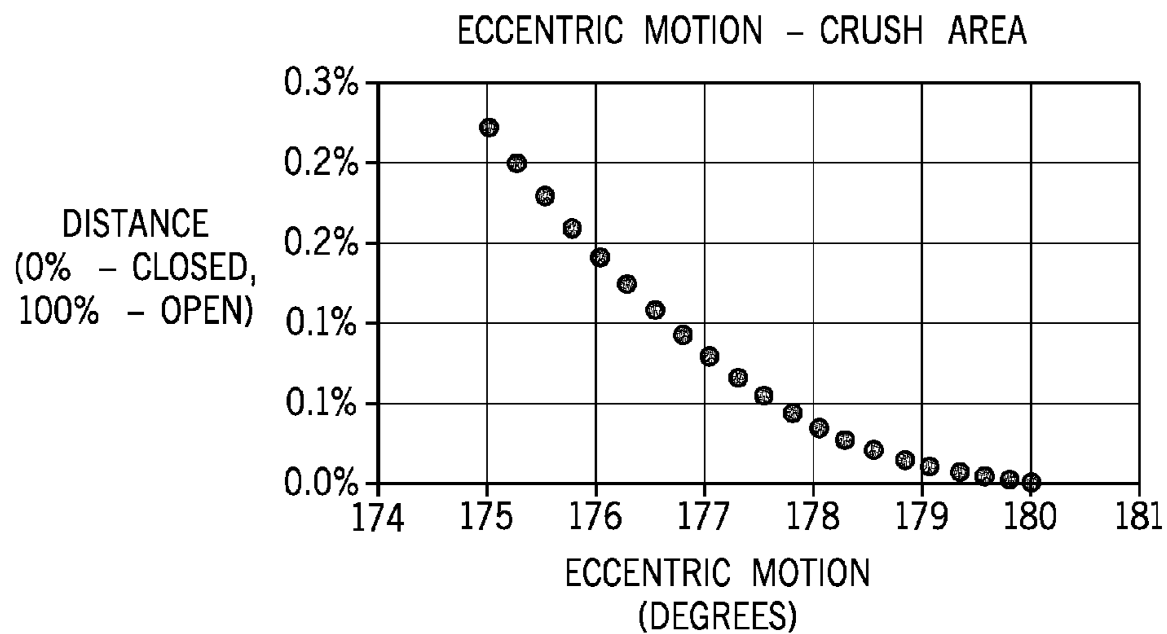
CRUSH AREA - HEAD POSITION VERSUS ECCENTRIC MOTION
