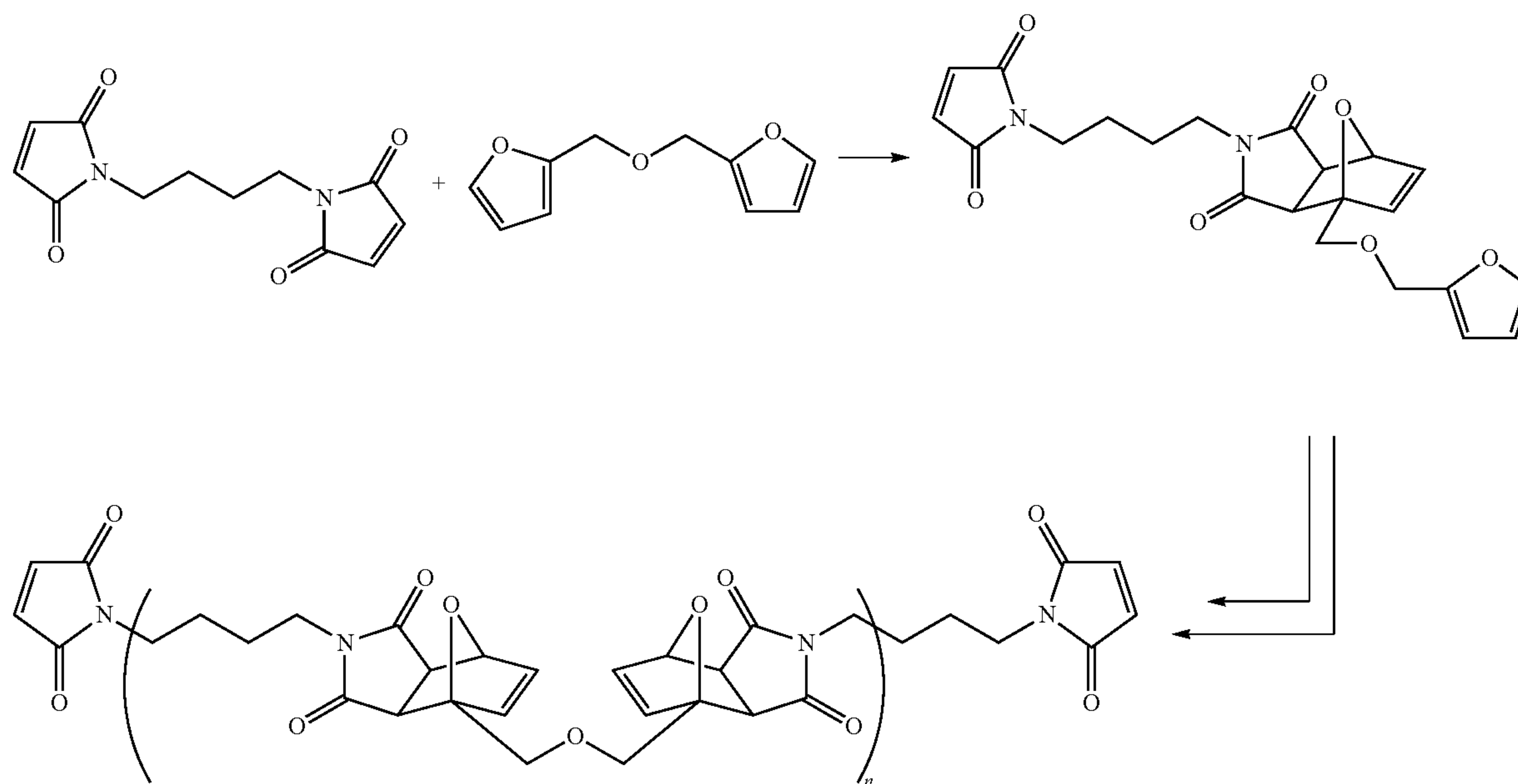
Reaction Example 2
