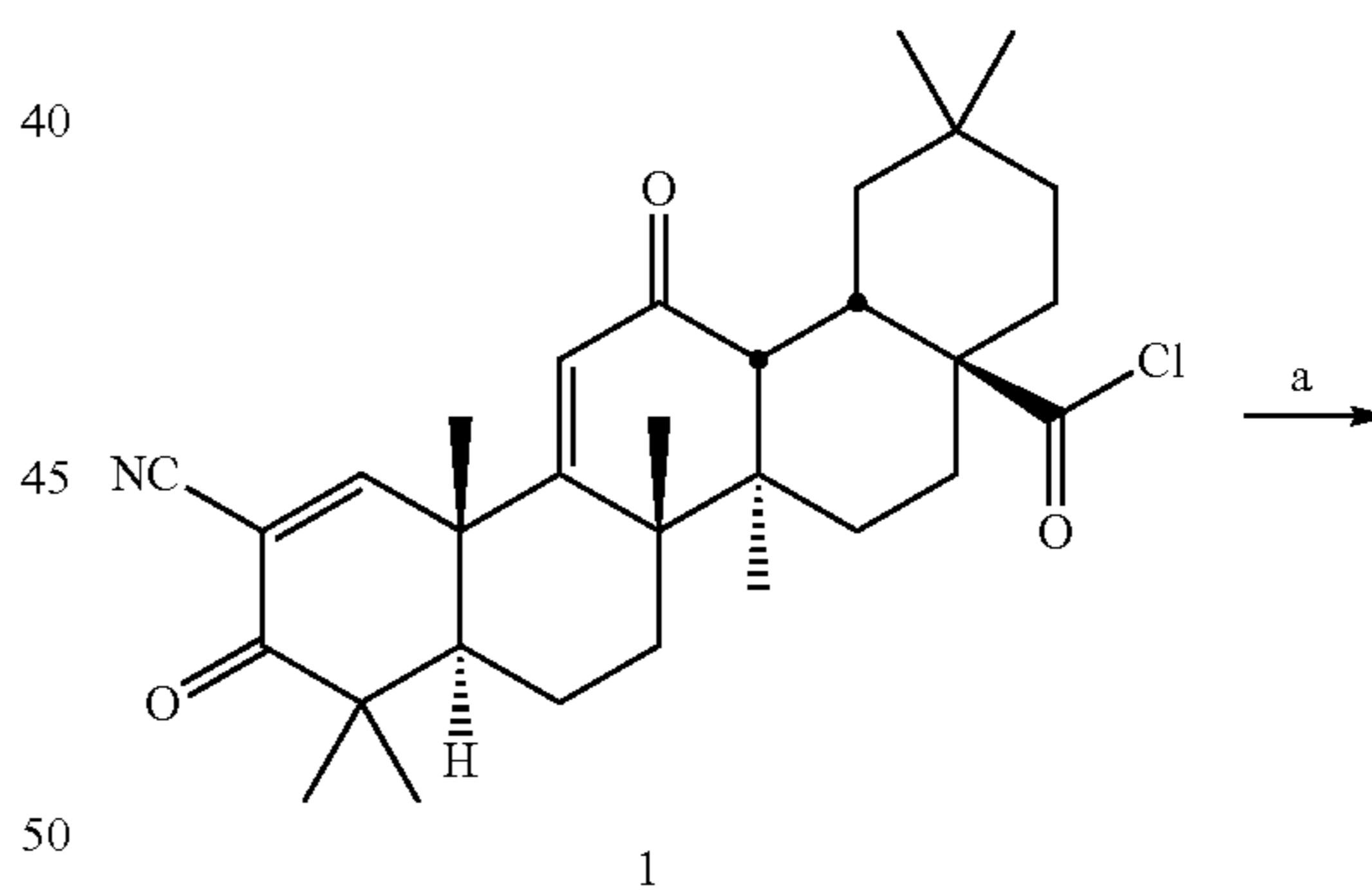
Scheme 4
