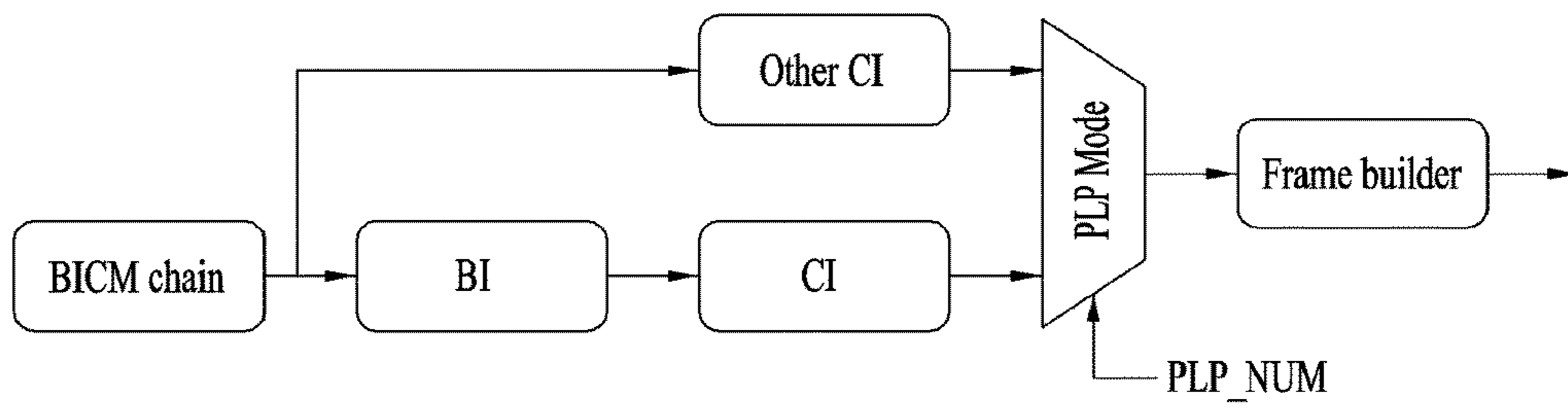
<Hybrid TI structure: example-2>
