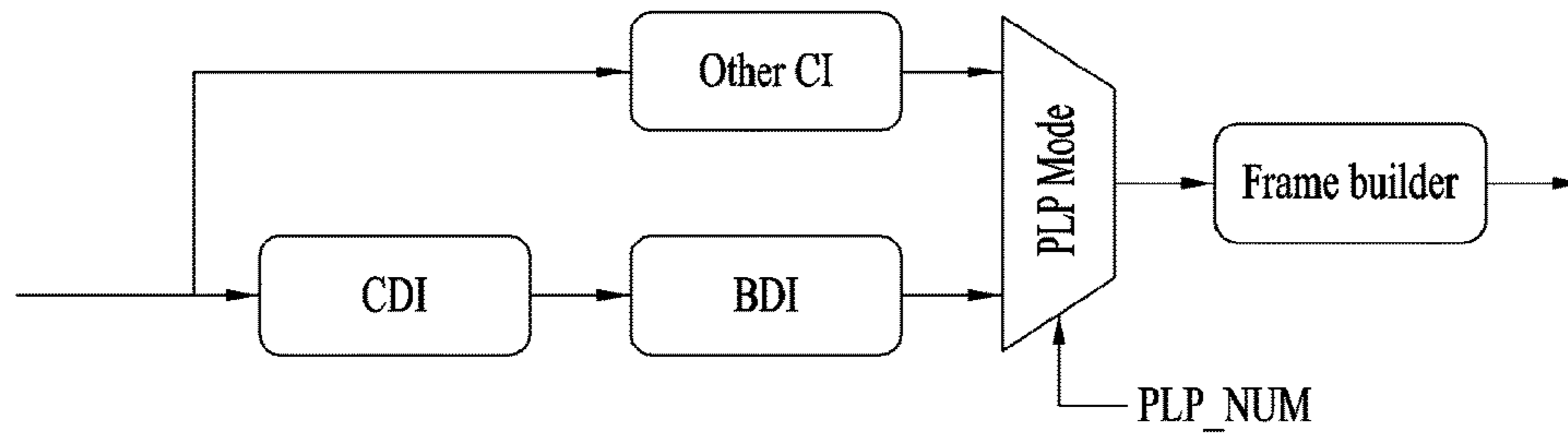
<Hybrid TDI structure: example-2>
