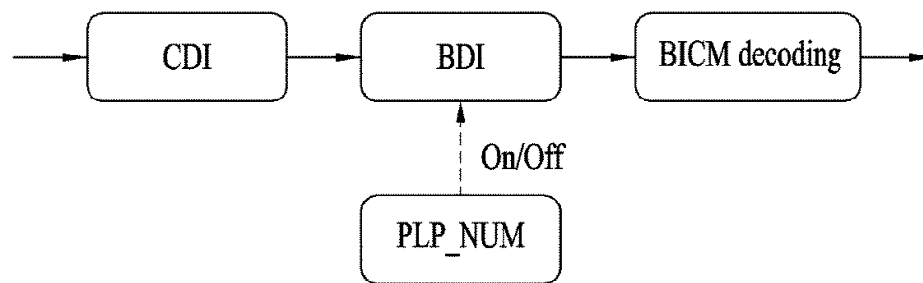
<Hybrid TDI structure: example-1>
