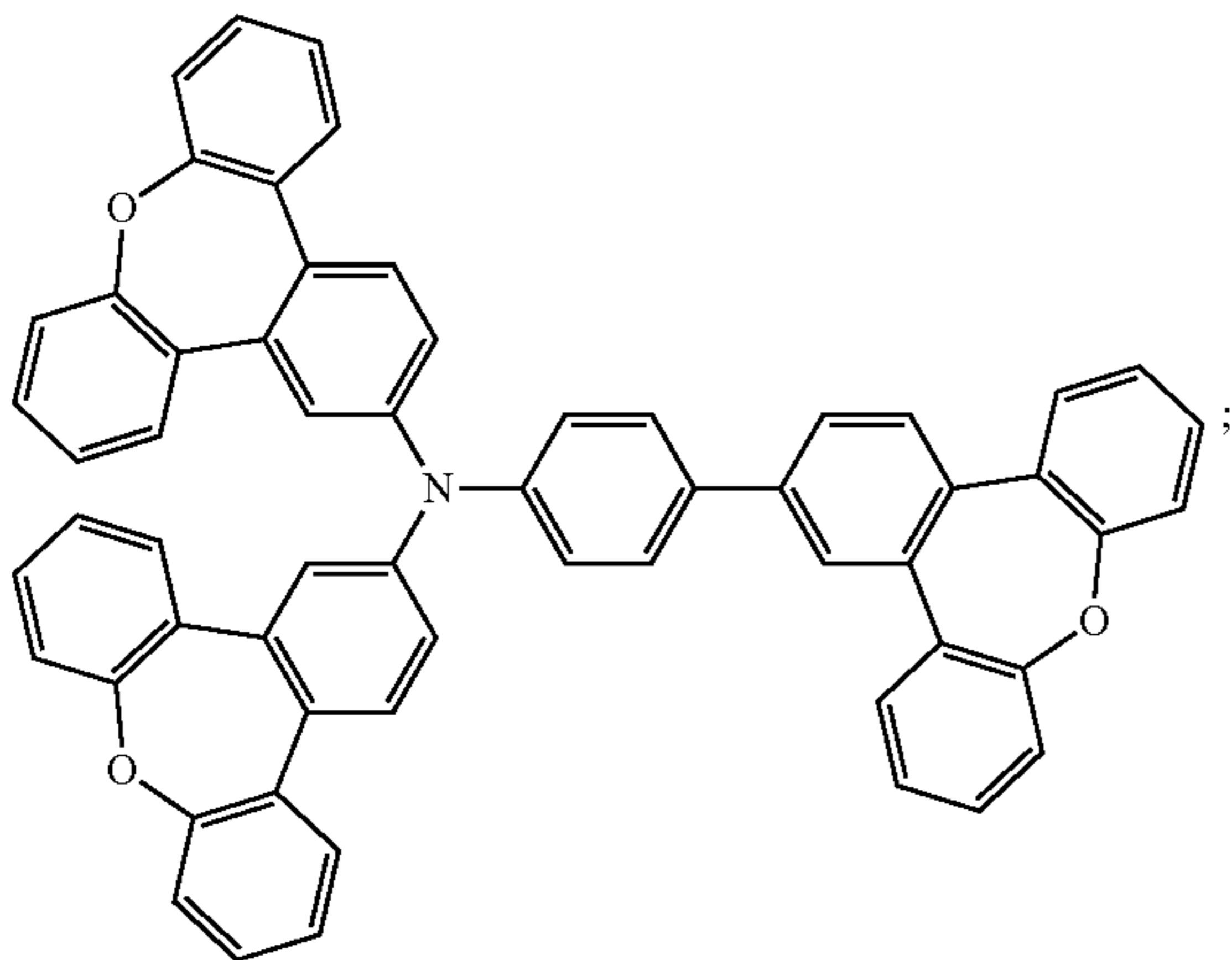
Compound 10
