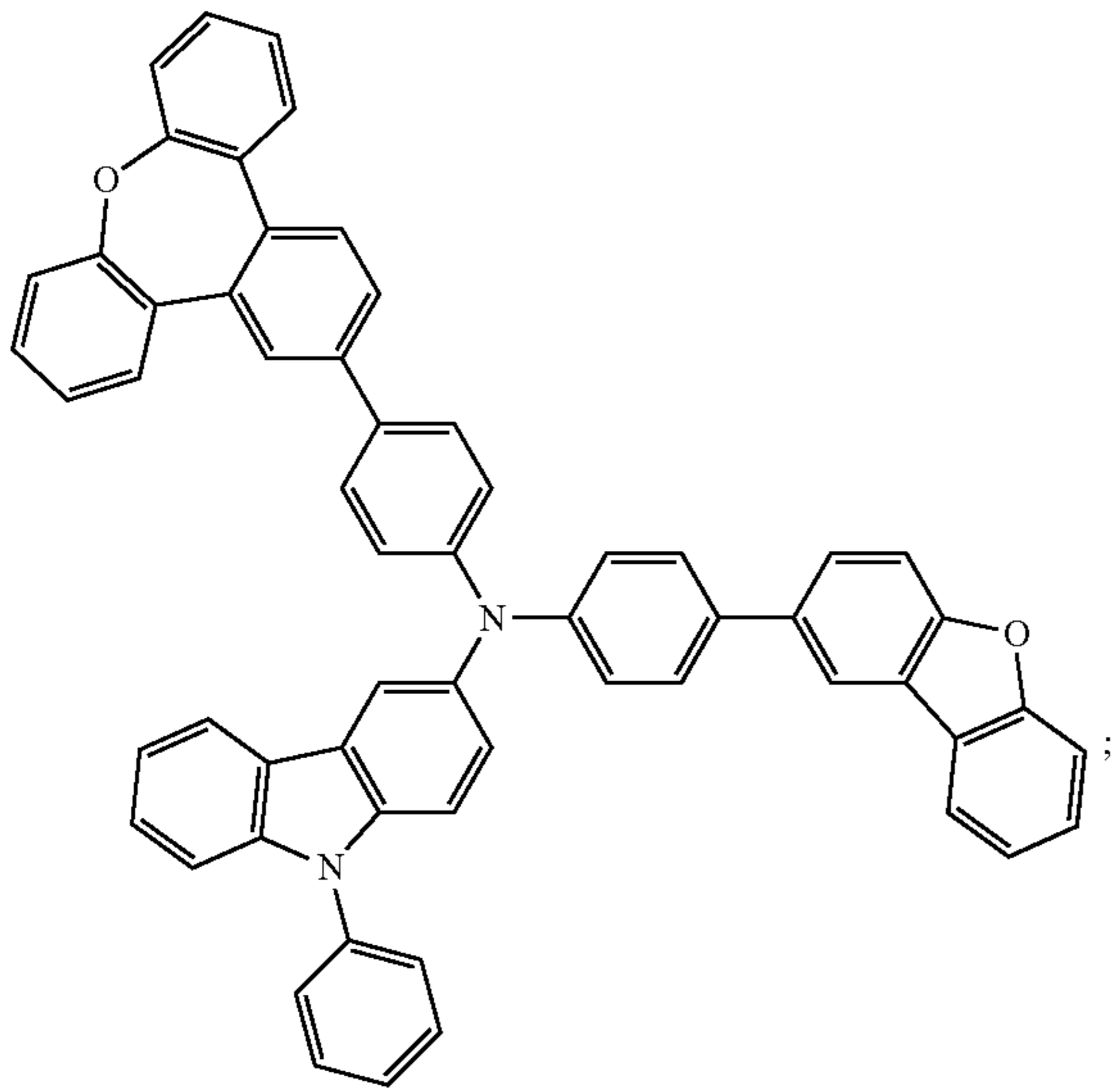
Compound 120
