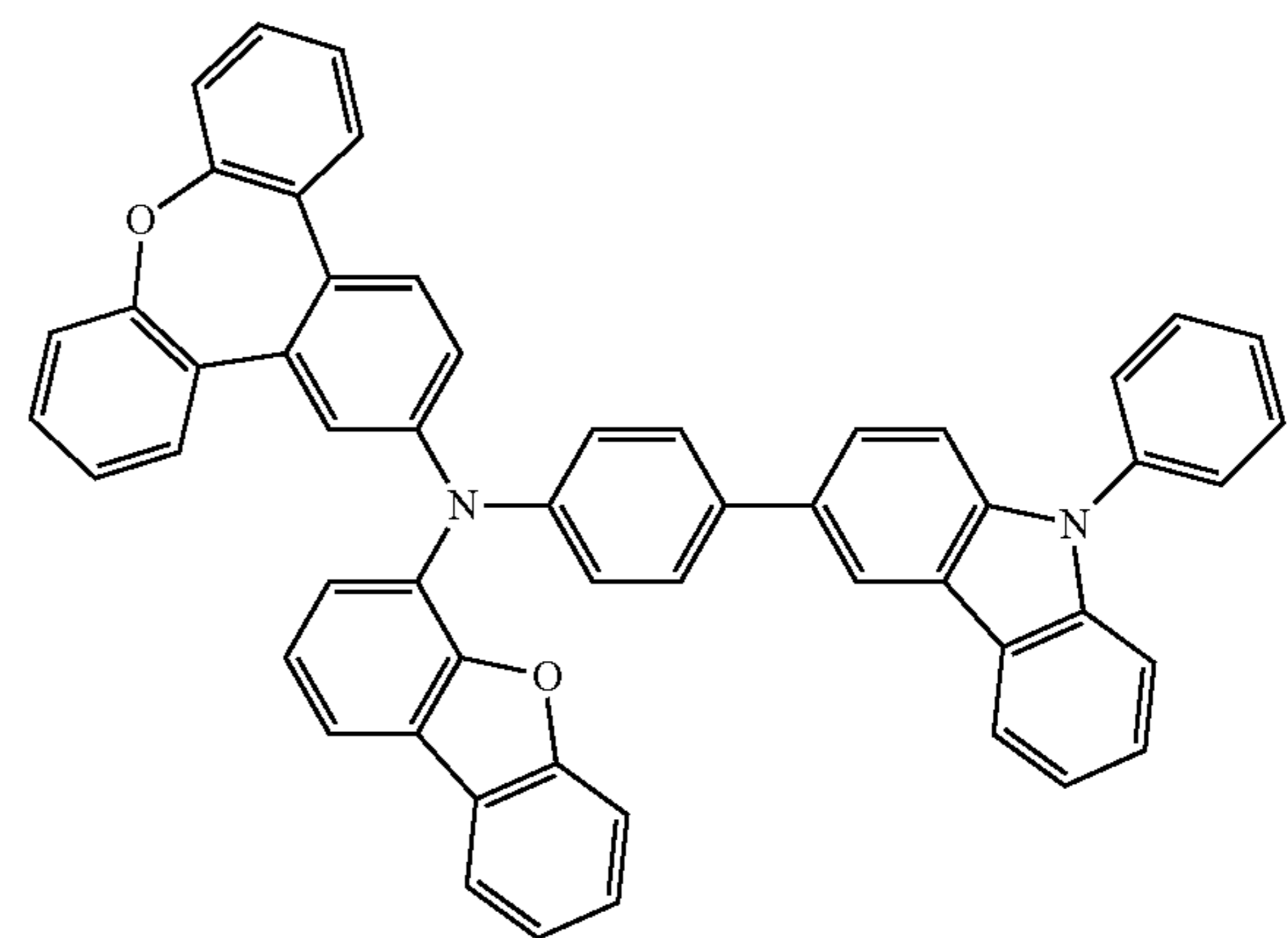
Compound 39
