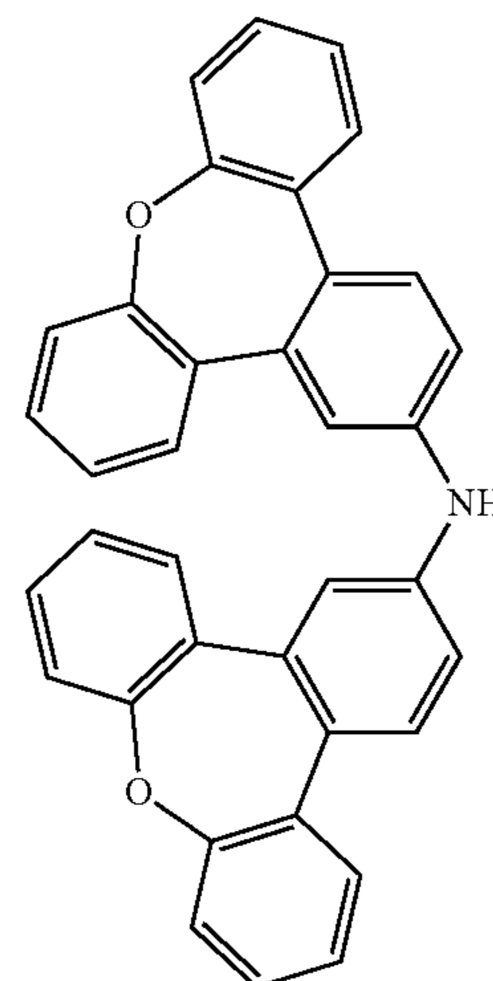
Intermediate C5
