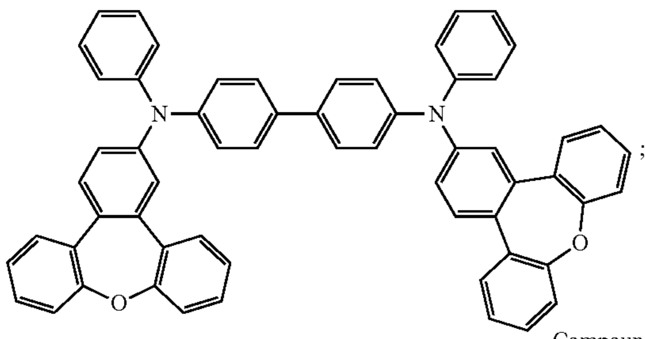
Compound 16
