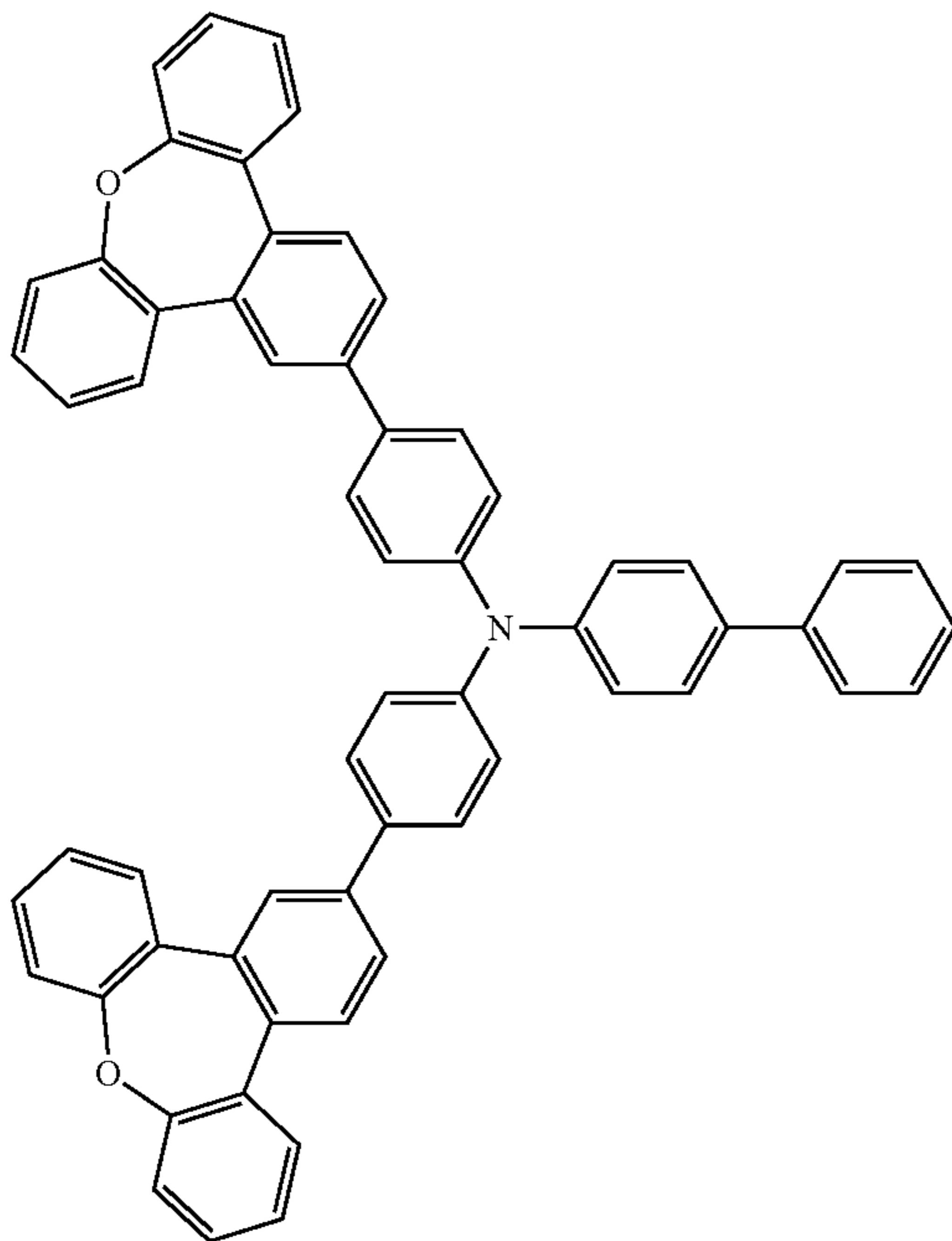
Compound 12
