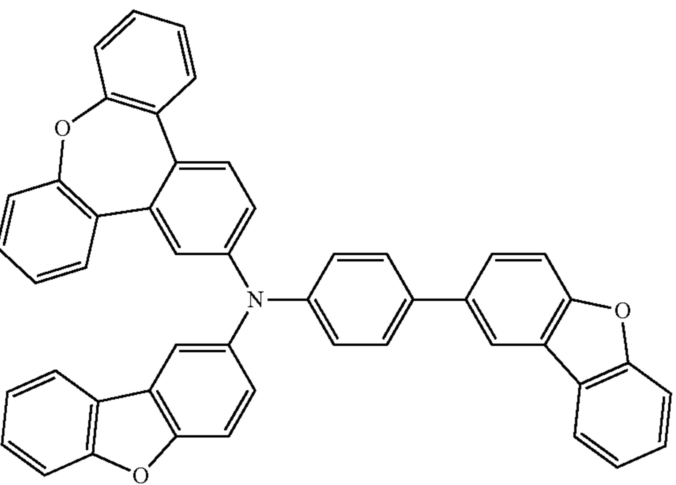
Compound 78
