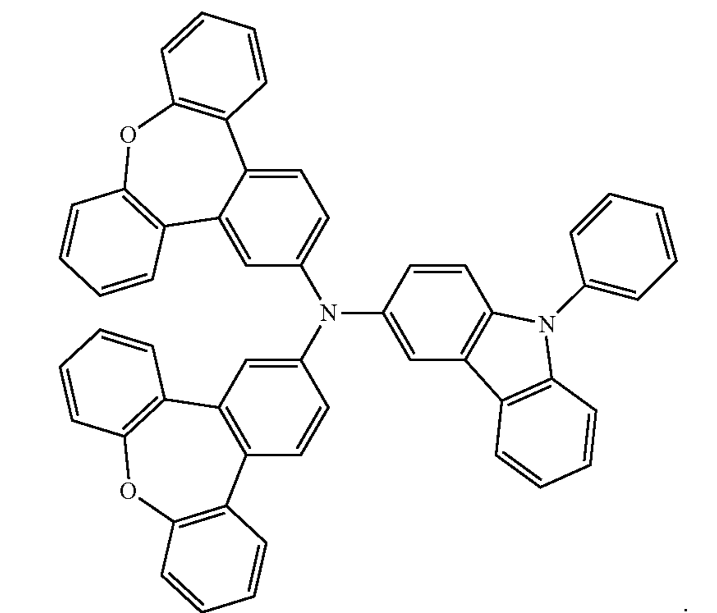
Compound 31
