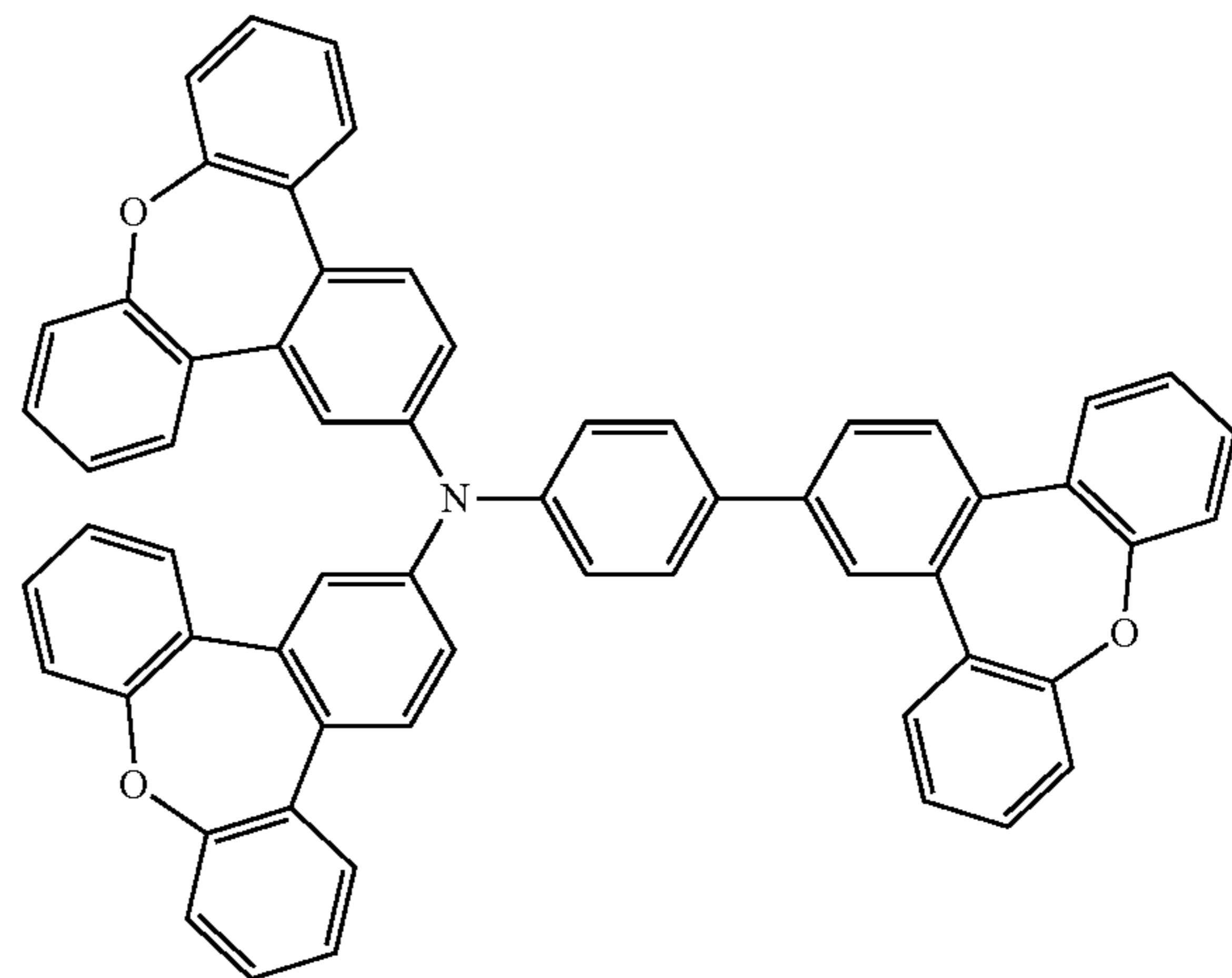
Compound 10
