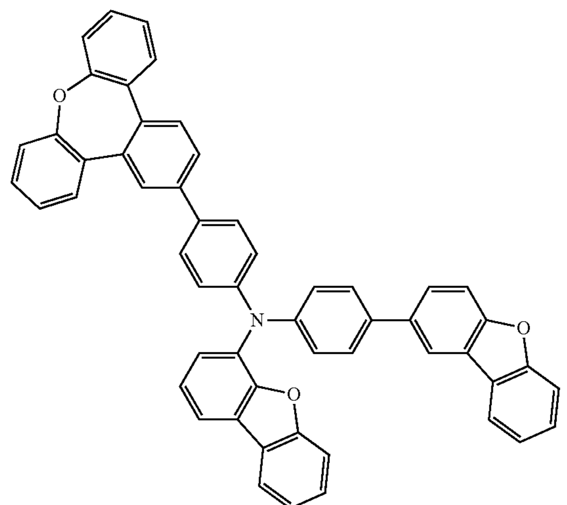
Compound 146
