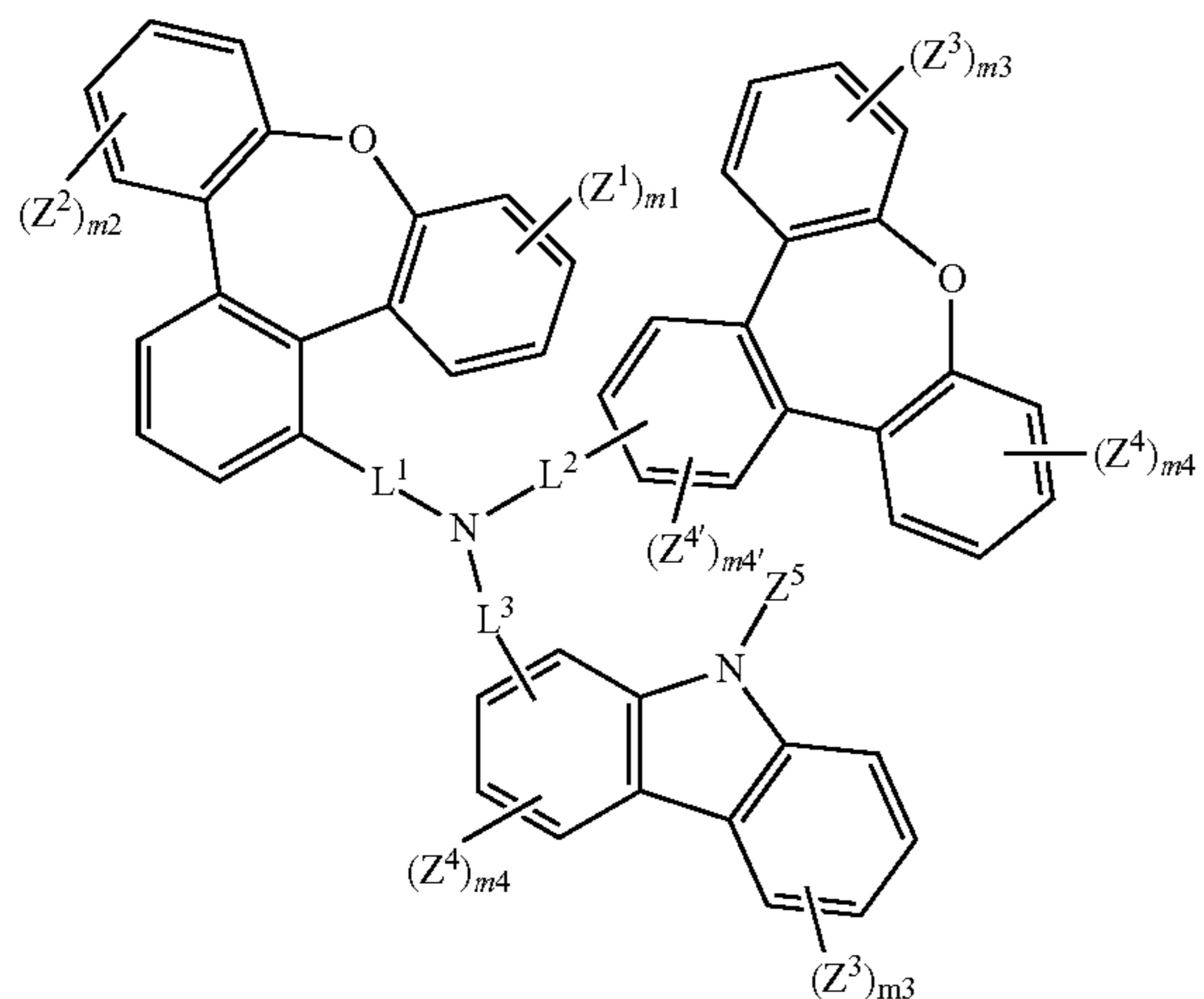
Formula (I-X)
