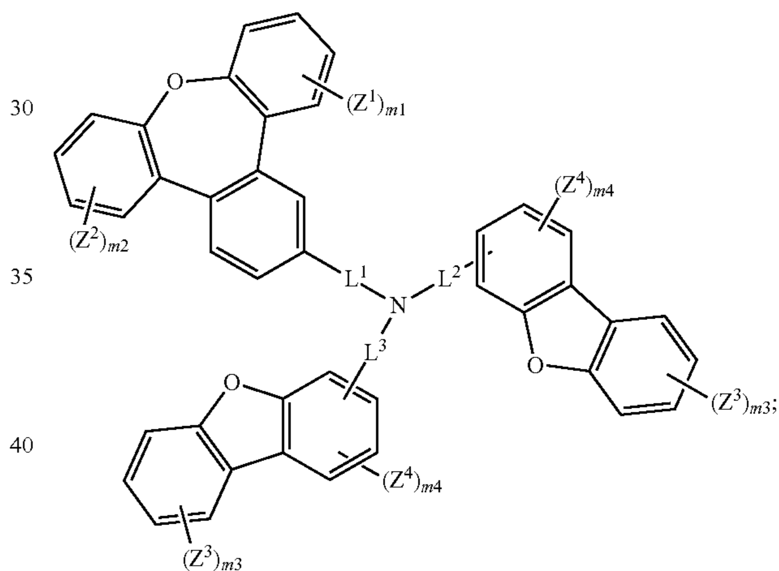
Formula (I-XXX)
