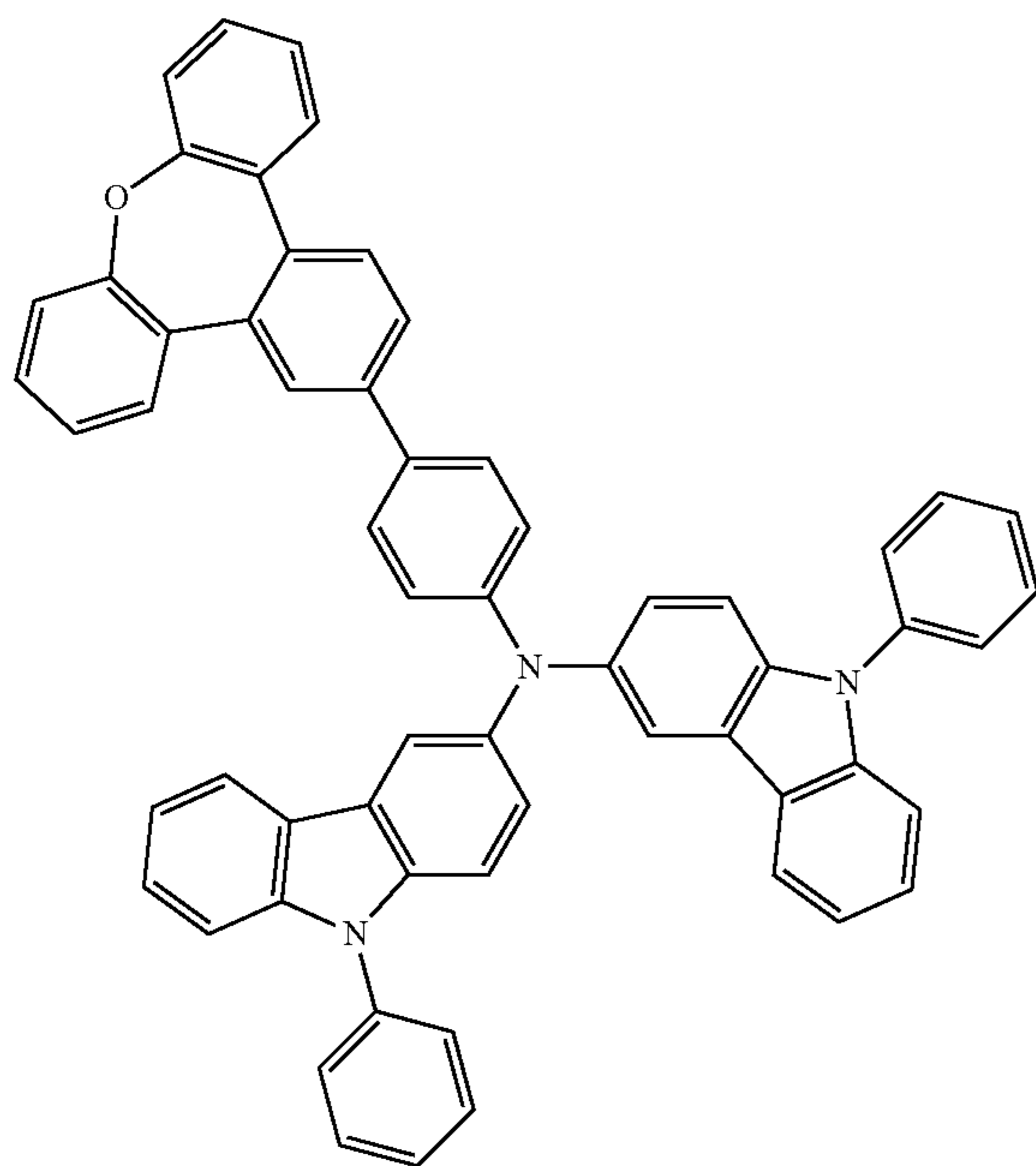
Compound 23
