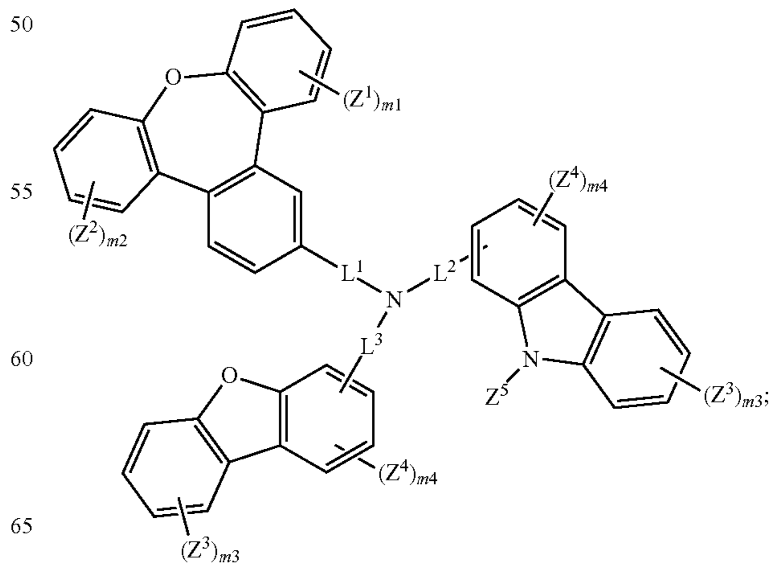
Formula (I-XXXI)
