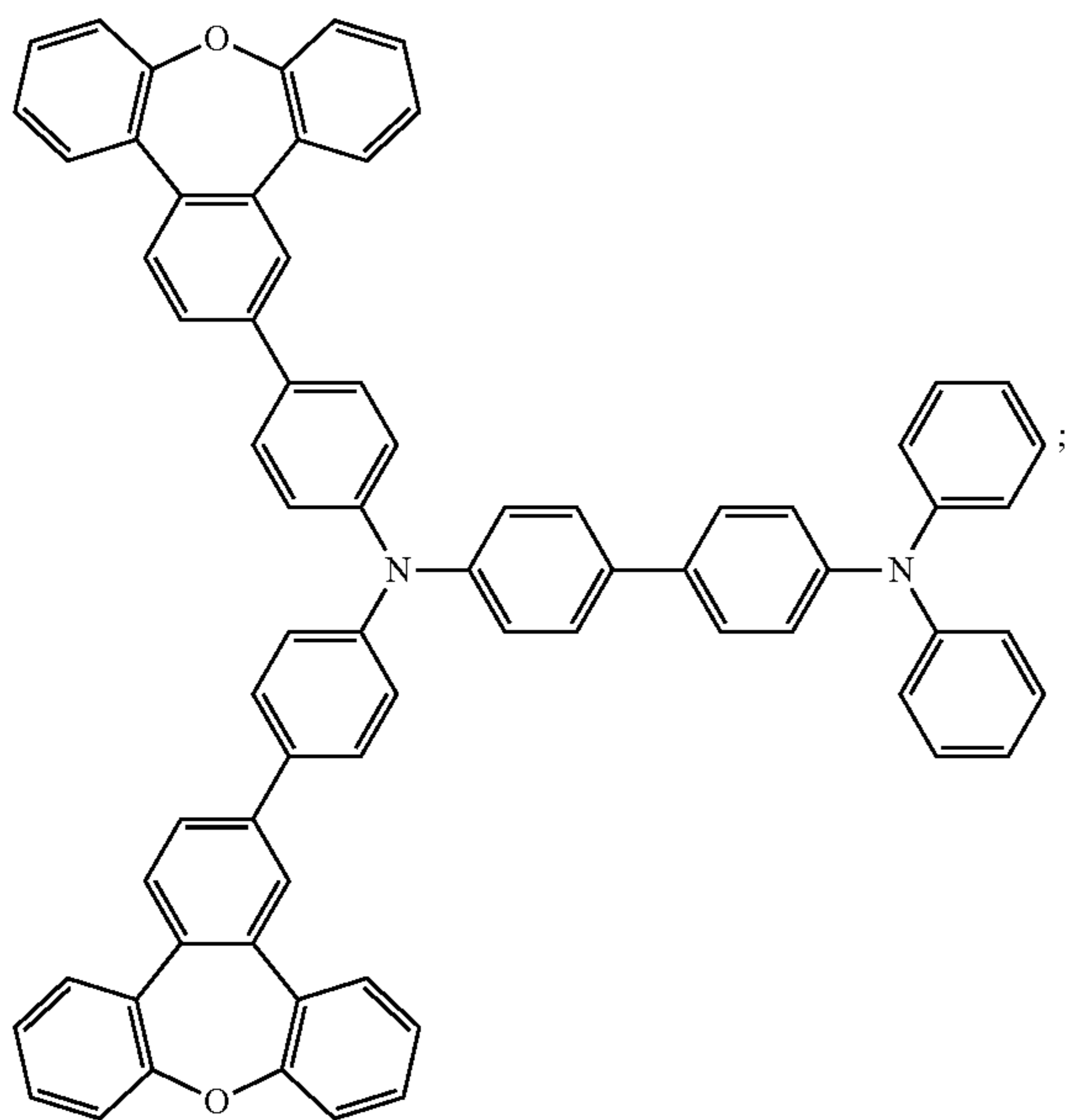
Compound 17
