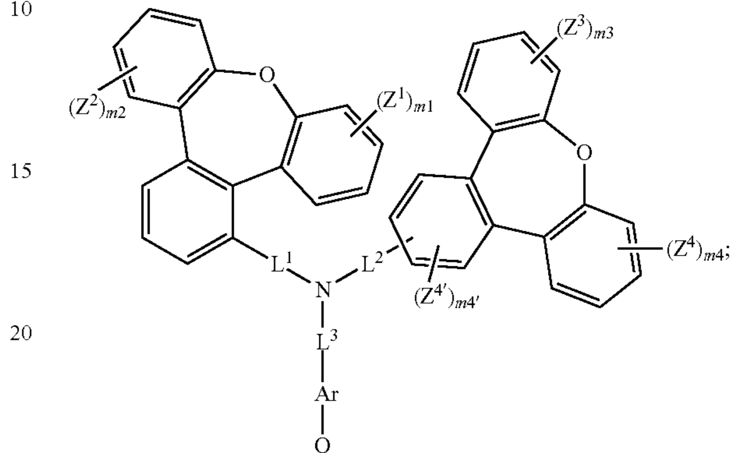
Formula (I-IX)
