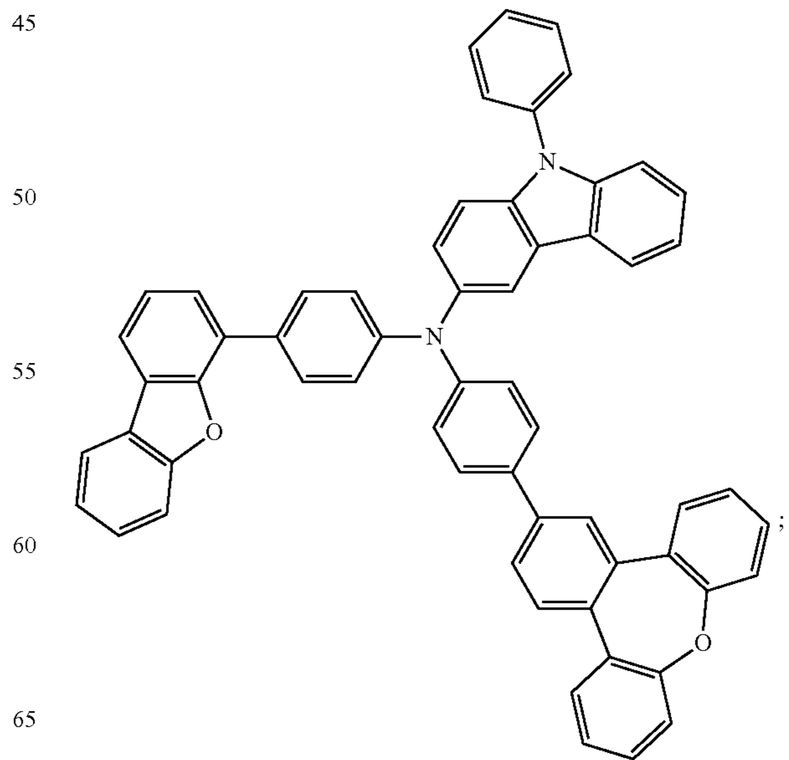
Compound 123
