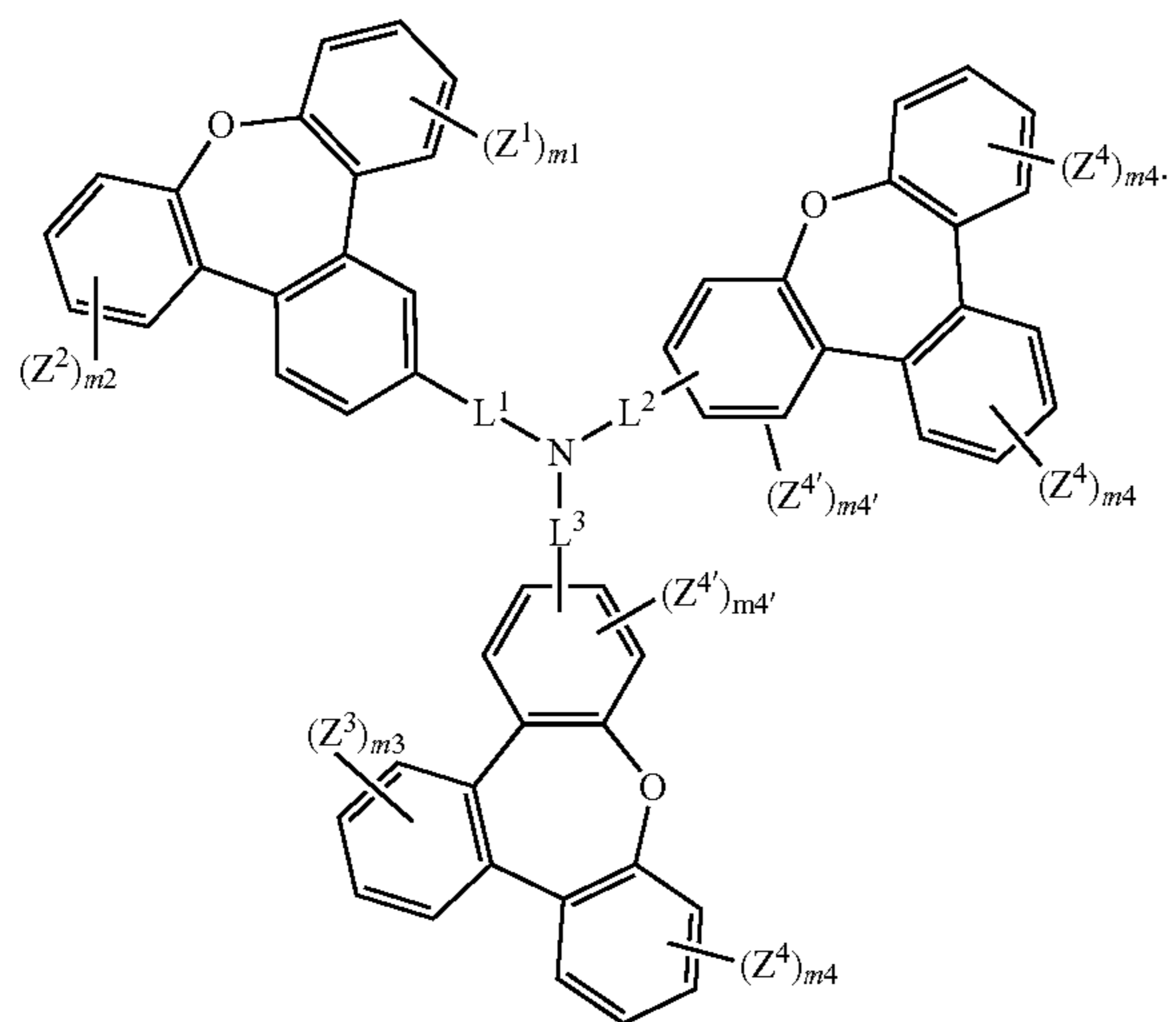
Formula (I-VIII)
