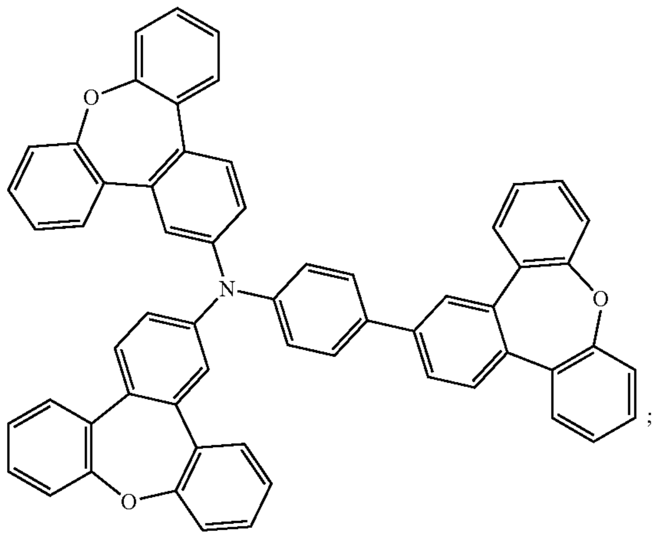
Compound 58
