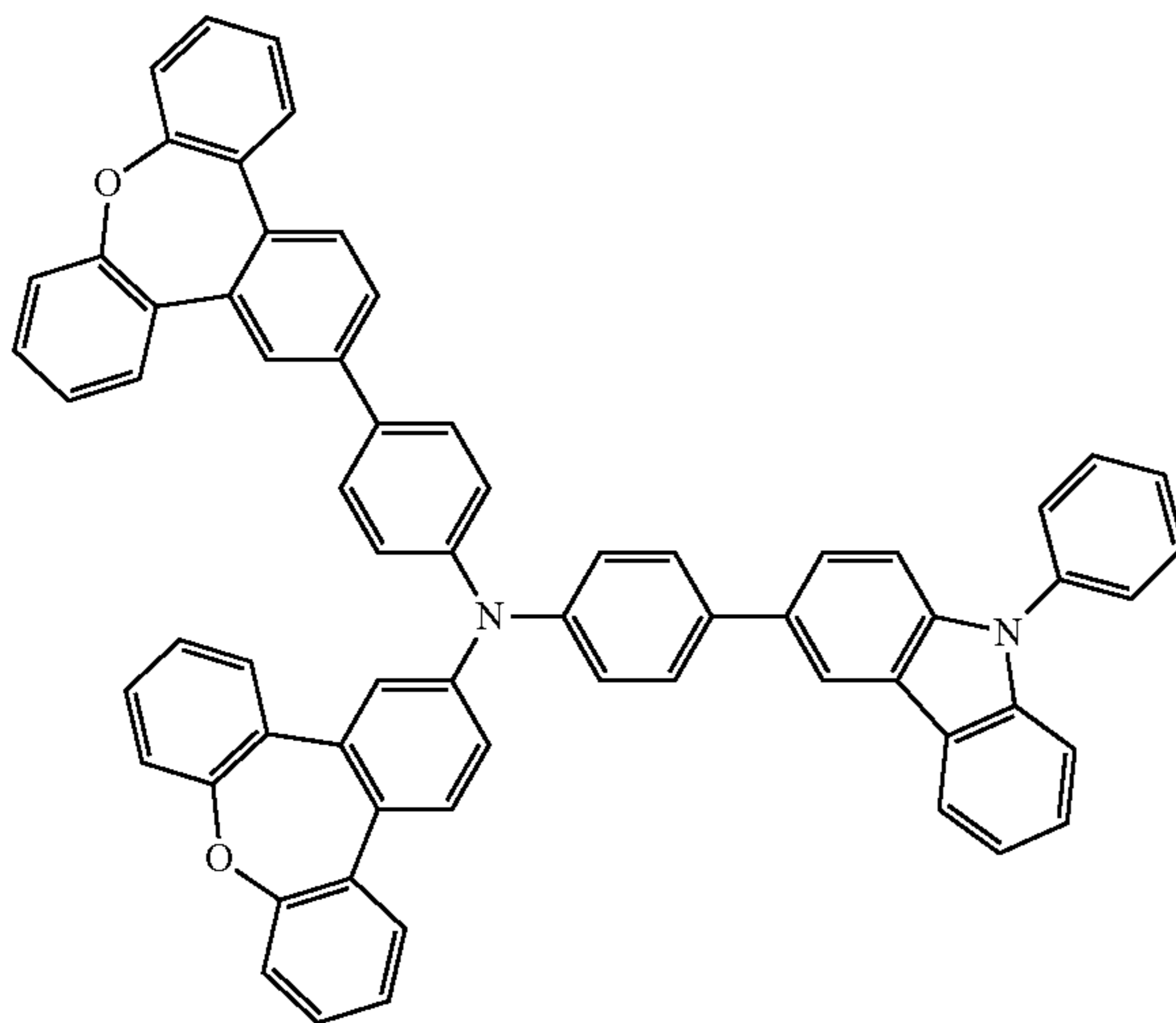
Compound 35
