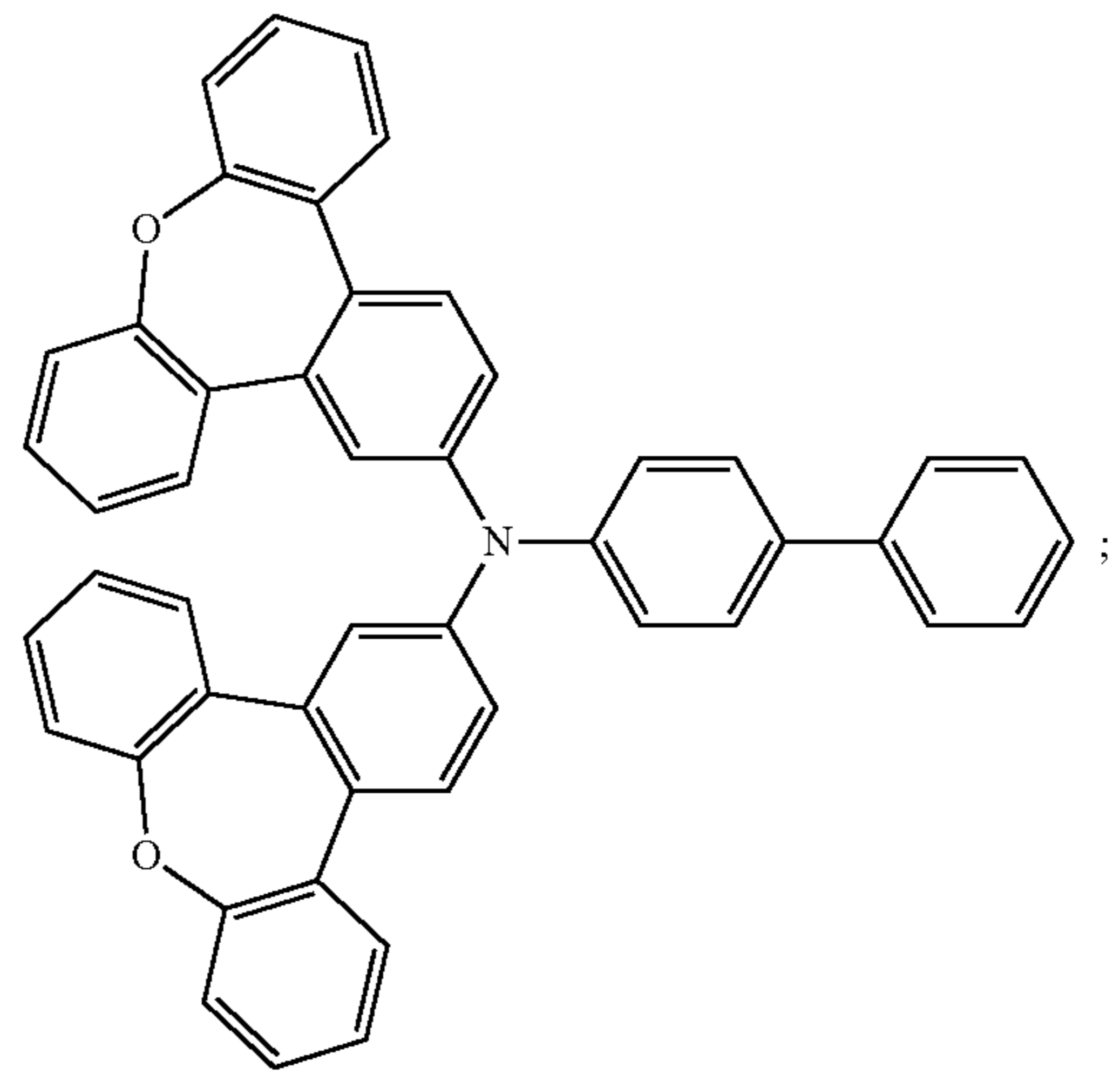
Compound 11
