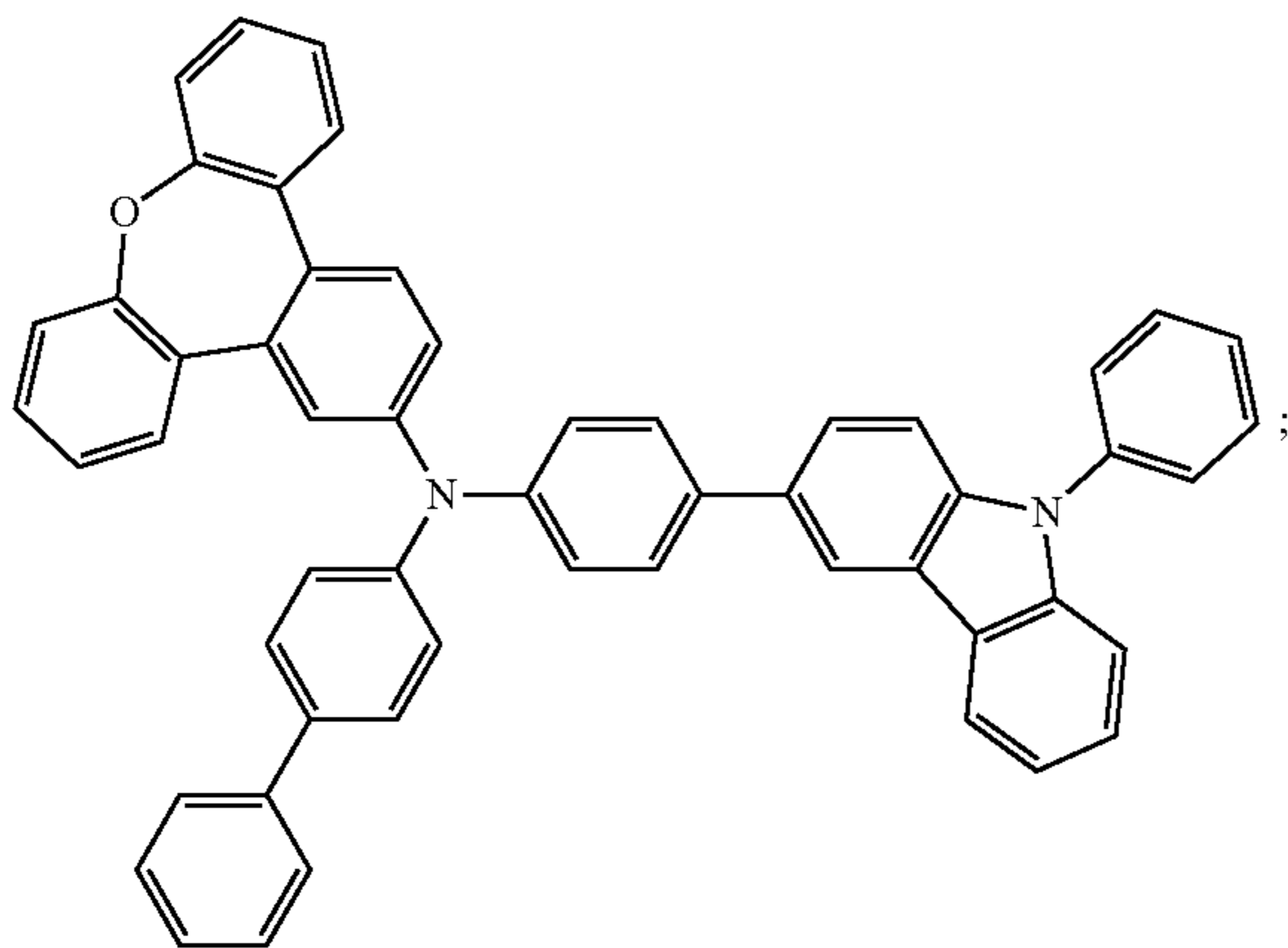
Compound 28
