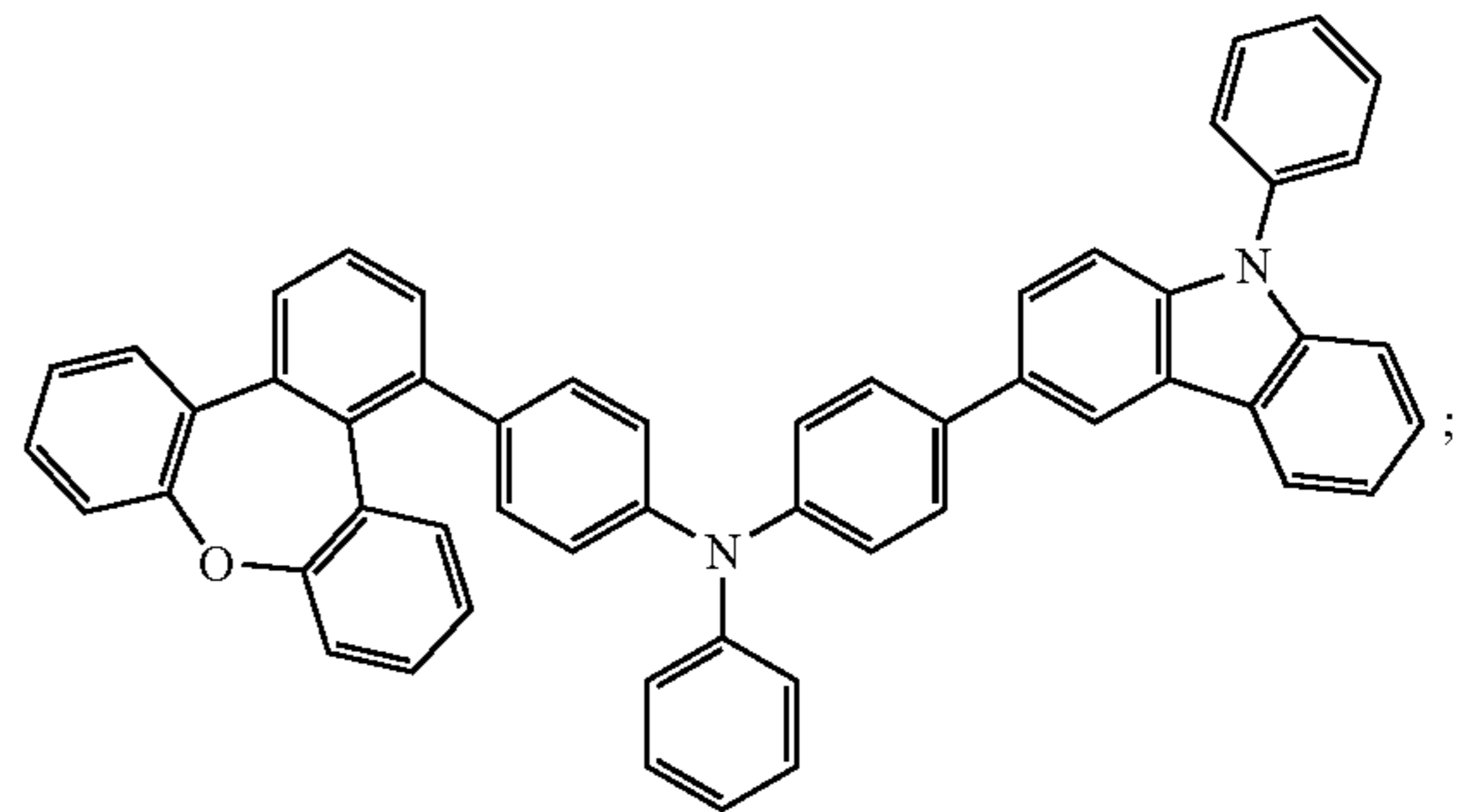
Compound 60
