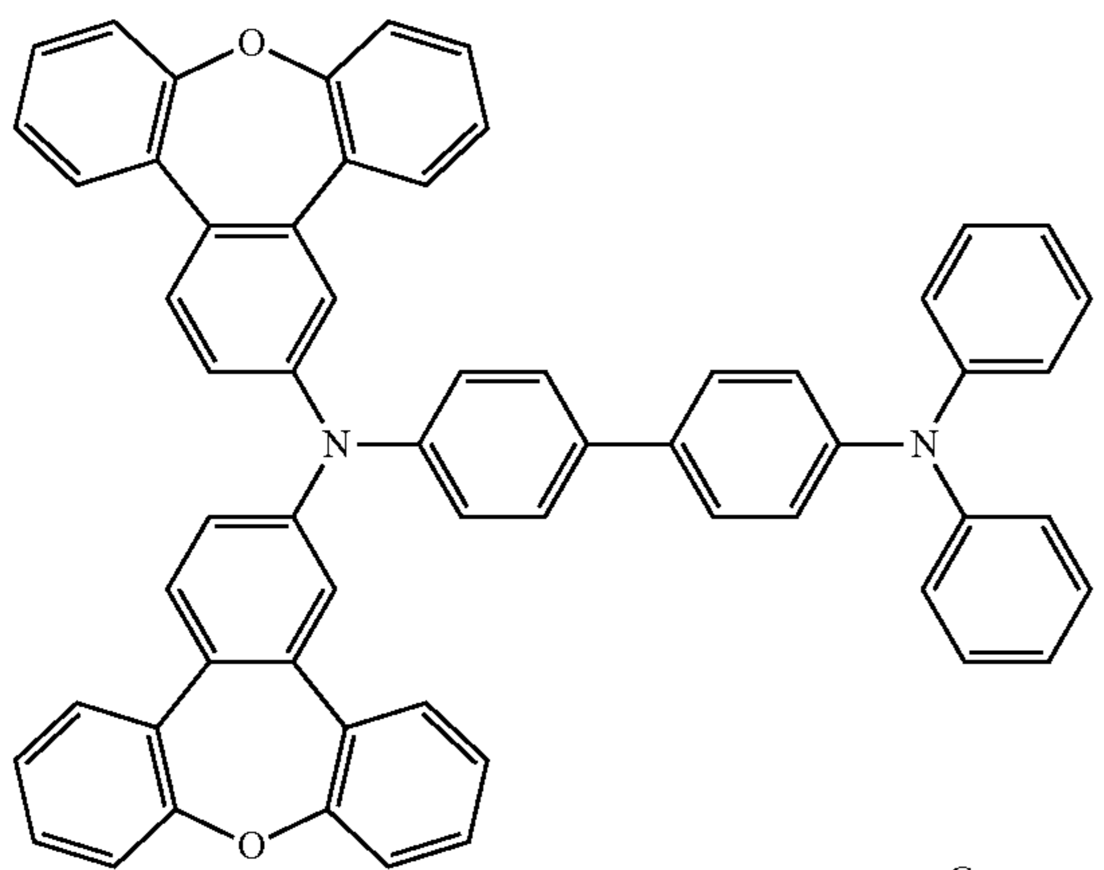
Compound 17
