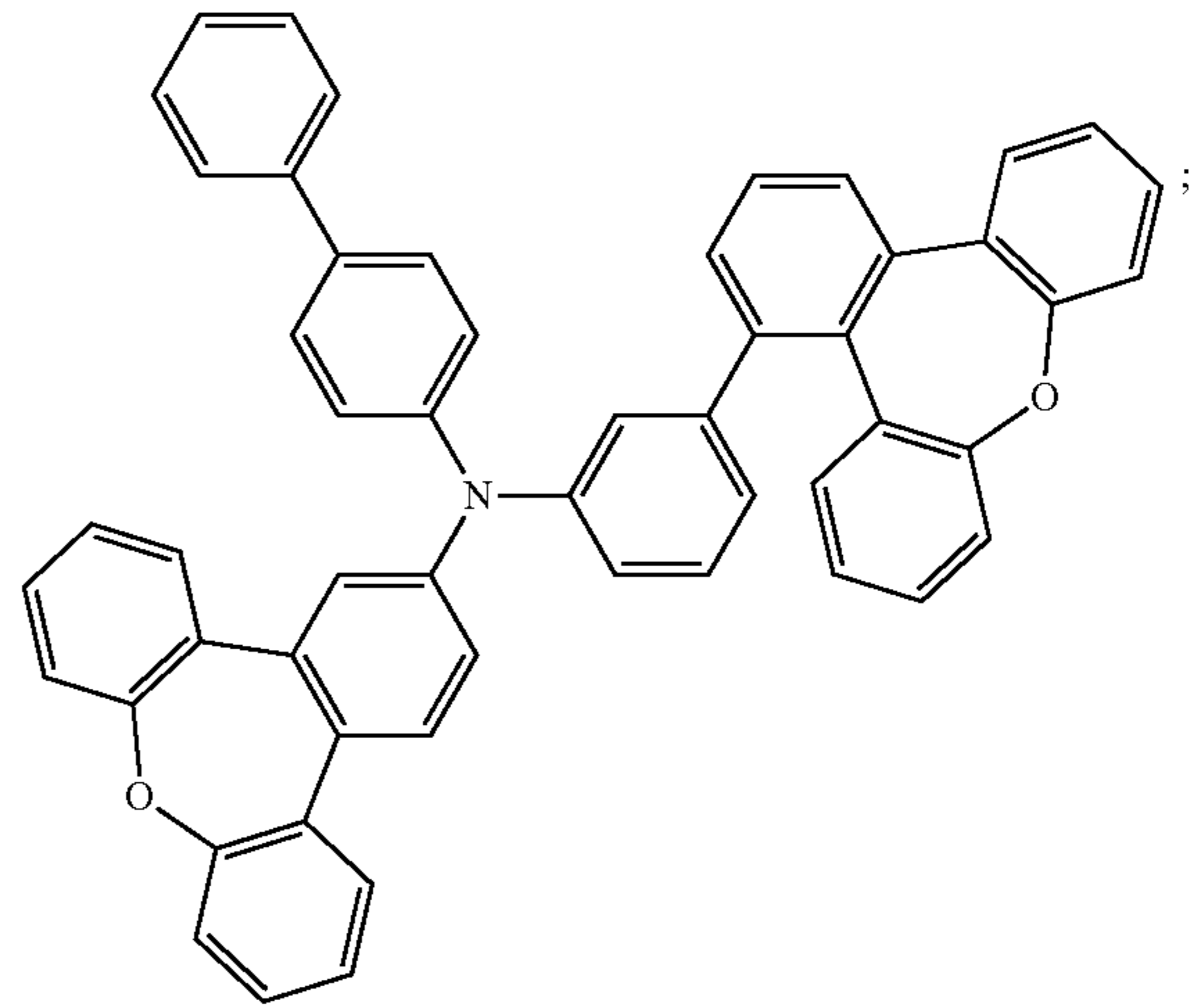
Compound 104
