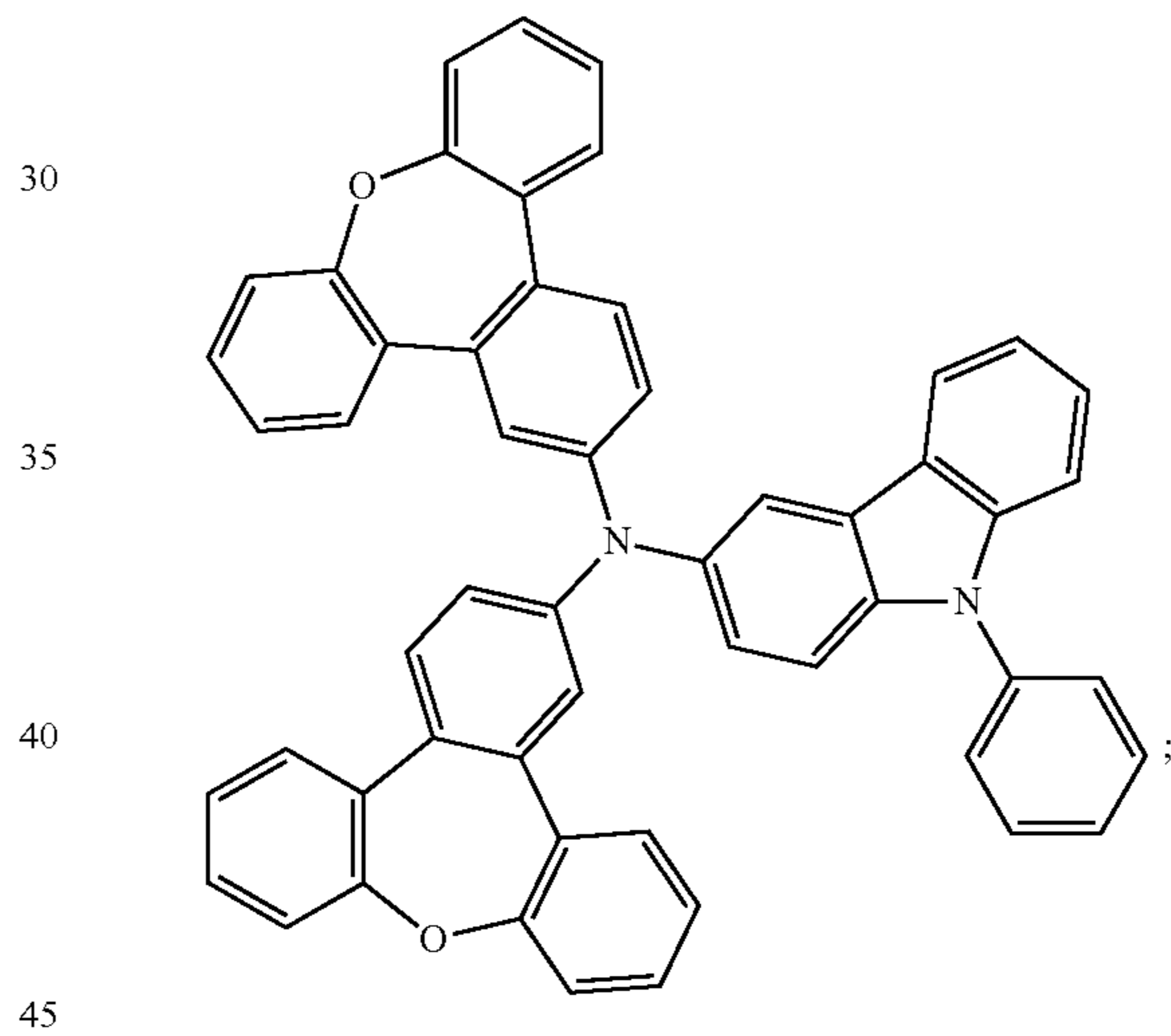
Compound 129
