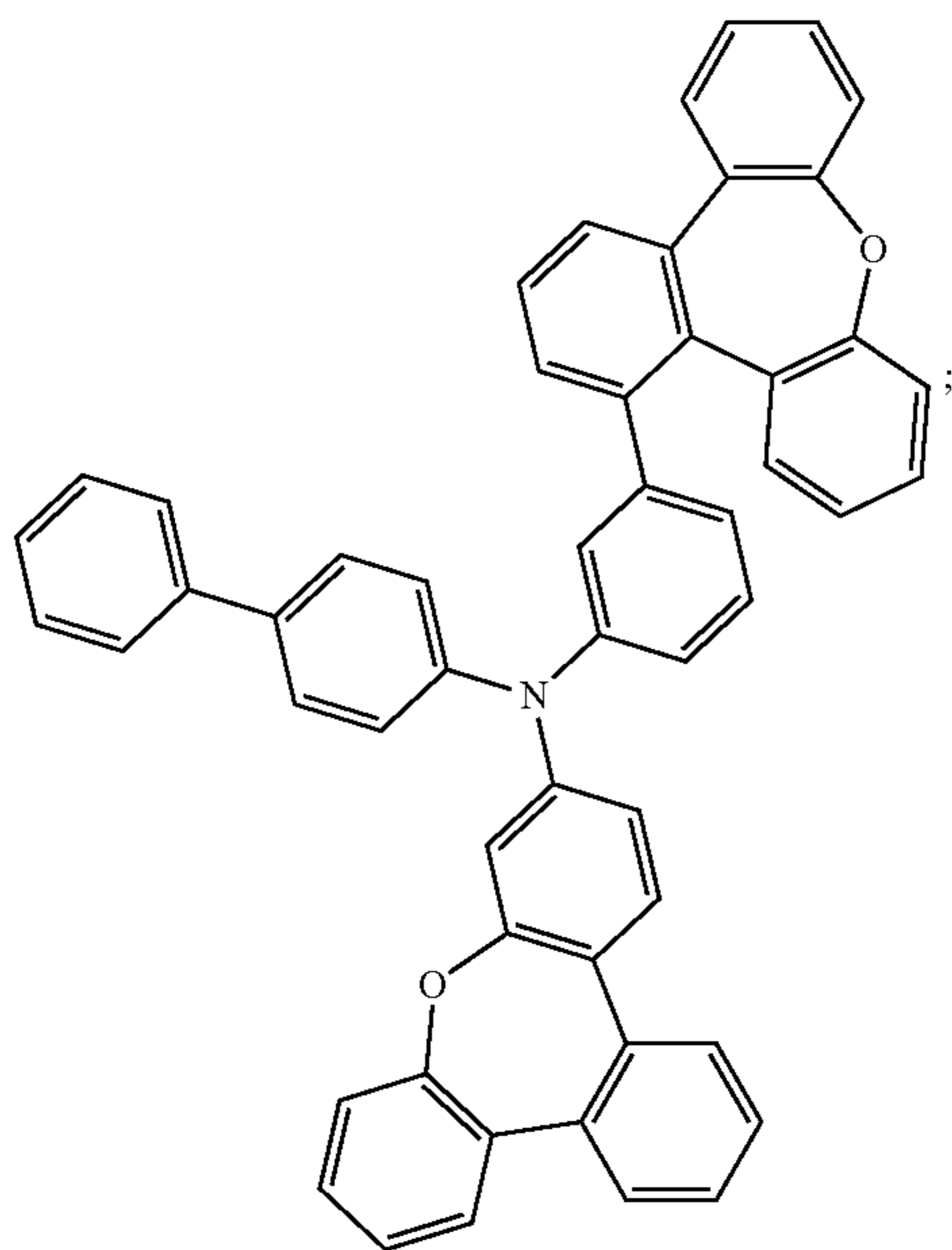
Compound 59
