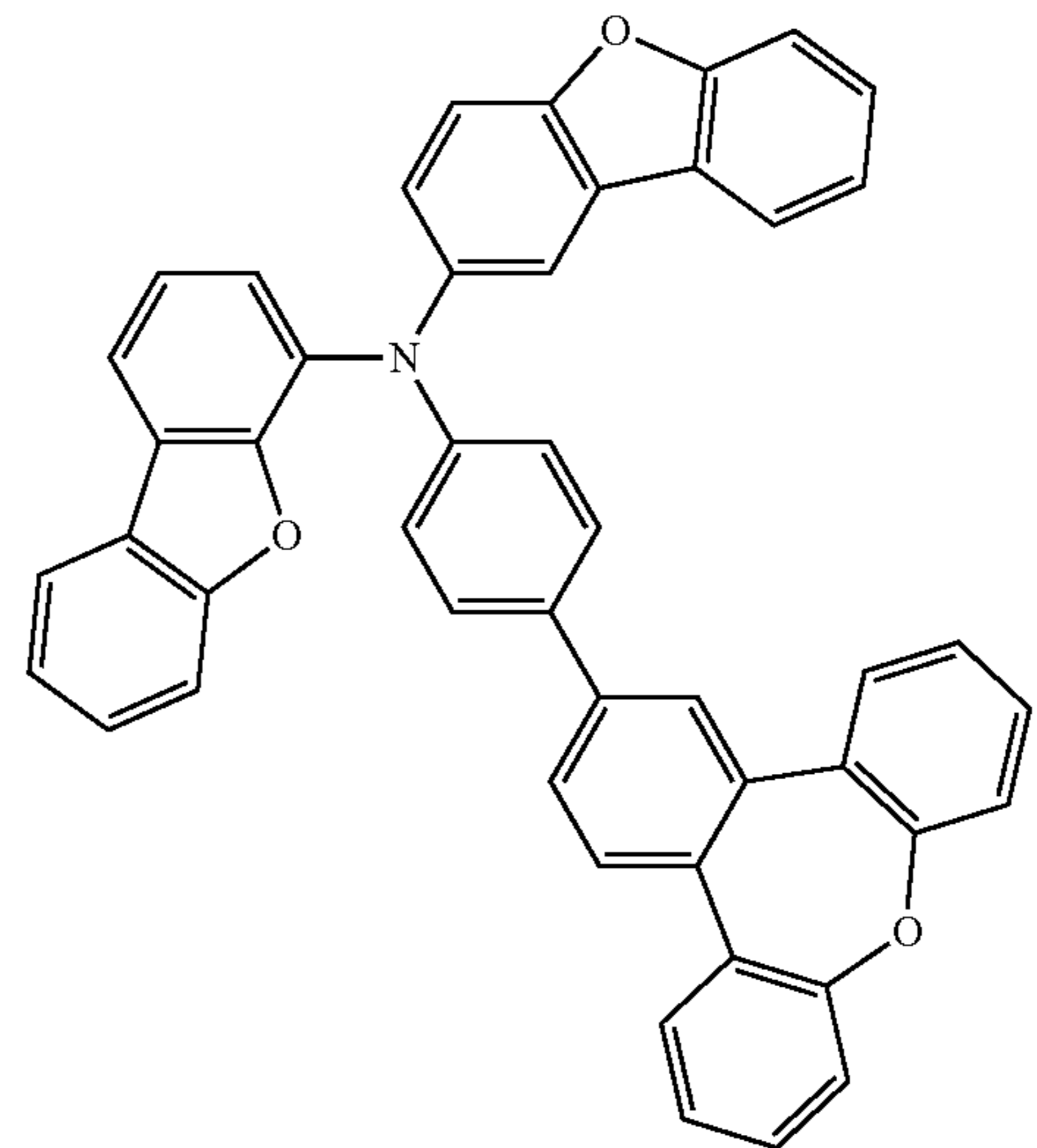
Compound 145
