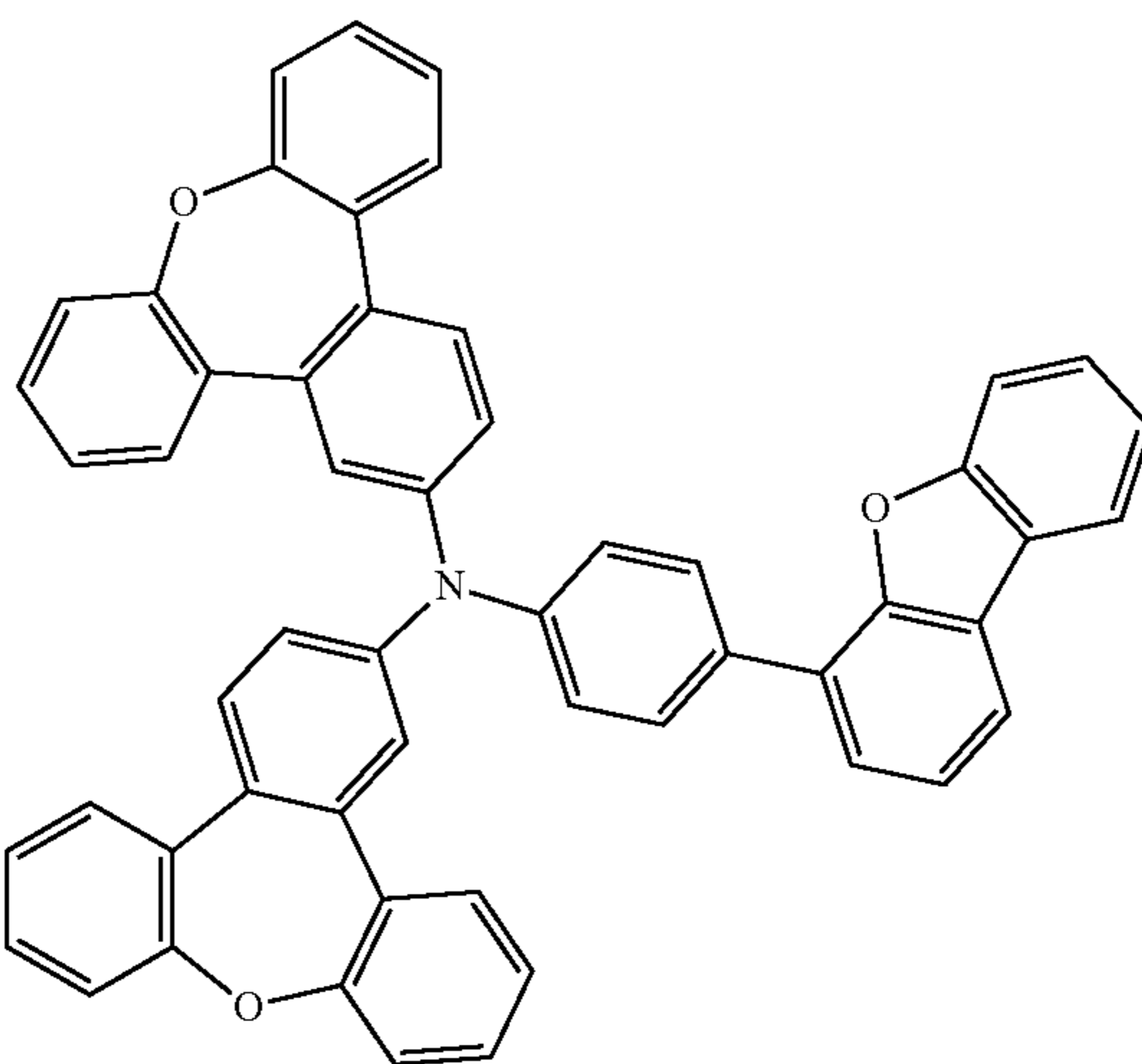
Compound 81
