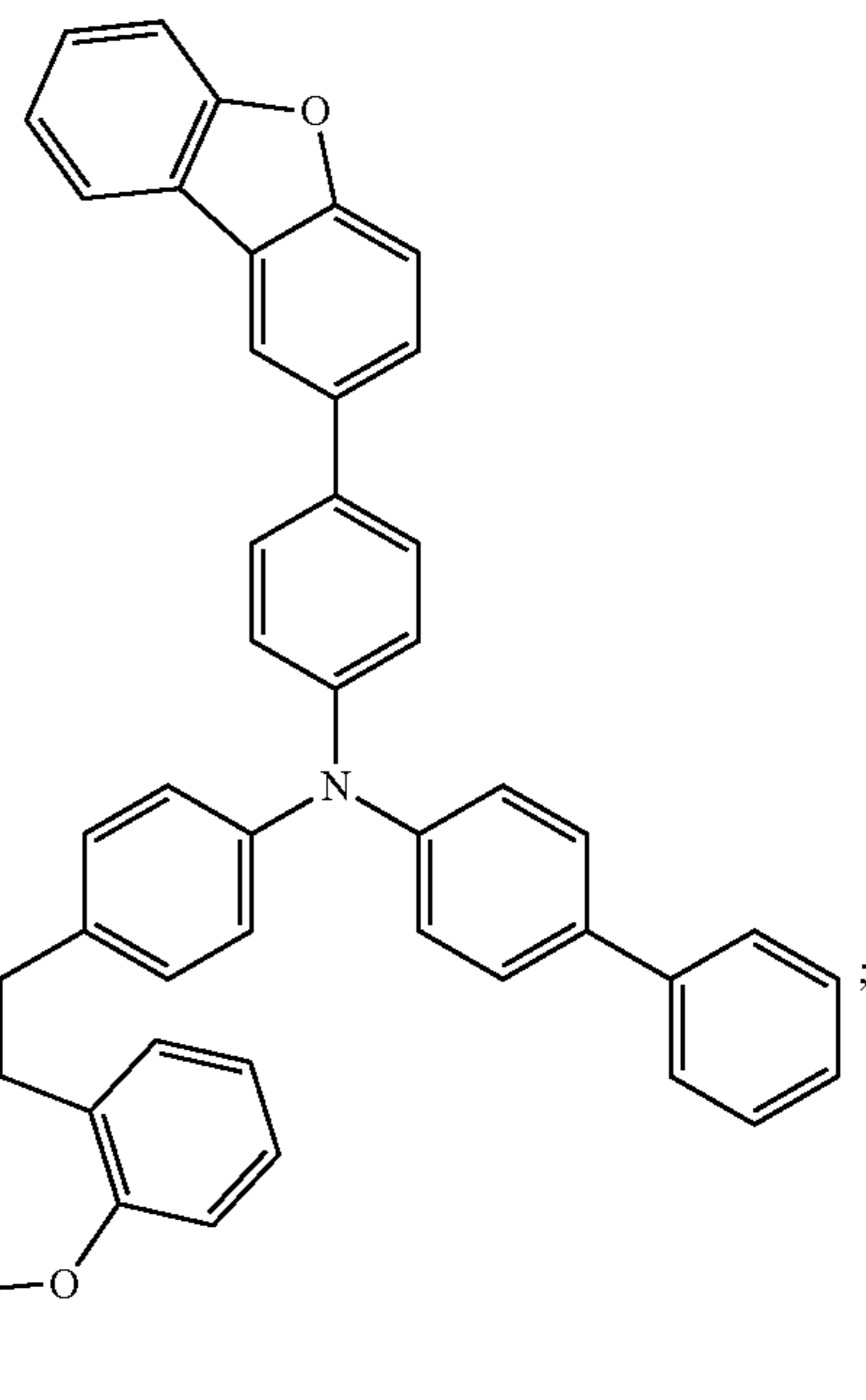
Compound 135
