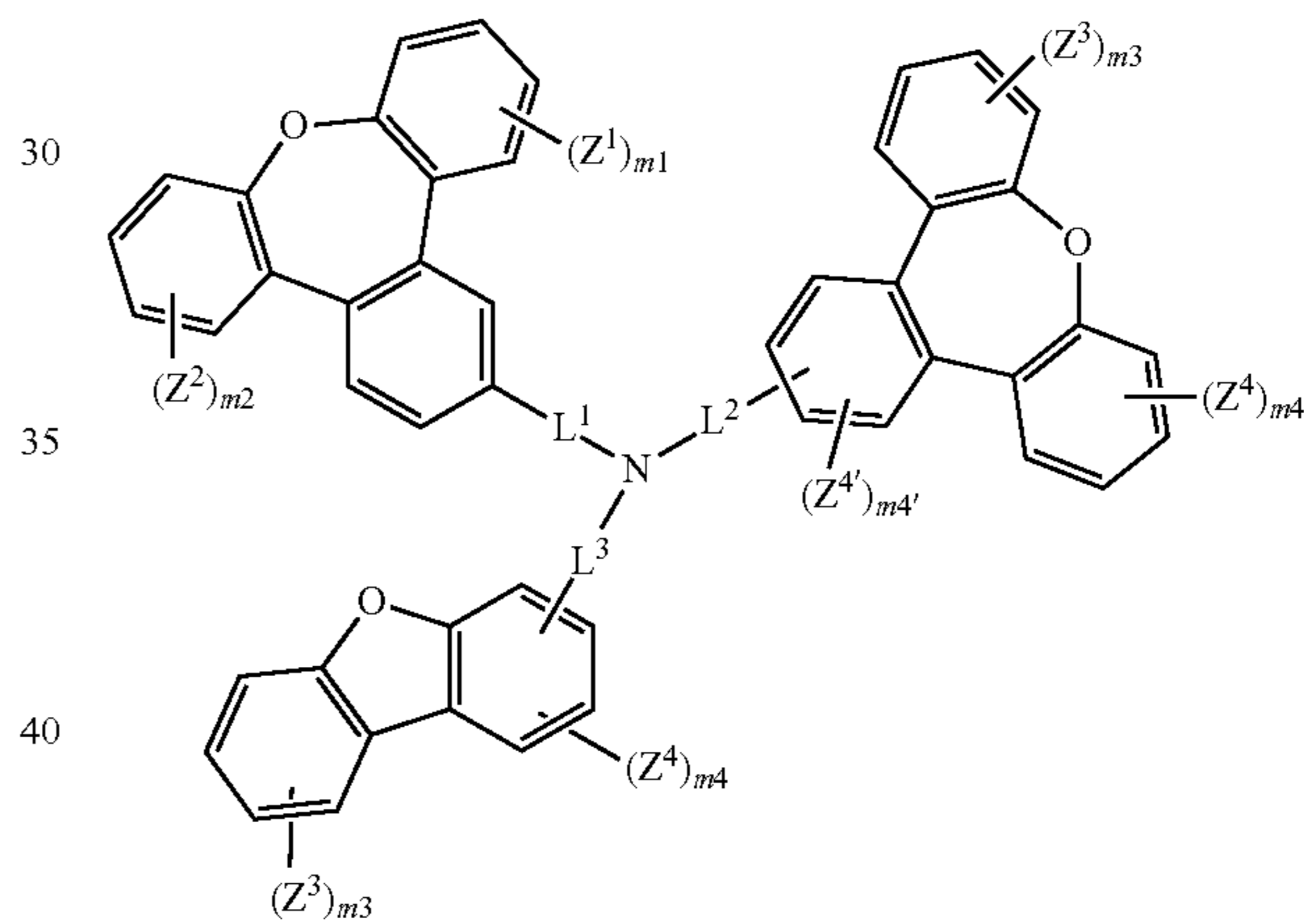
Formula (I-XIV)
