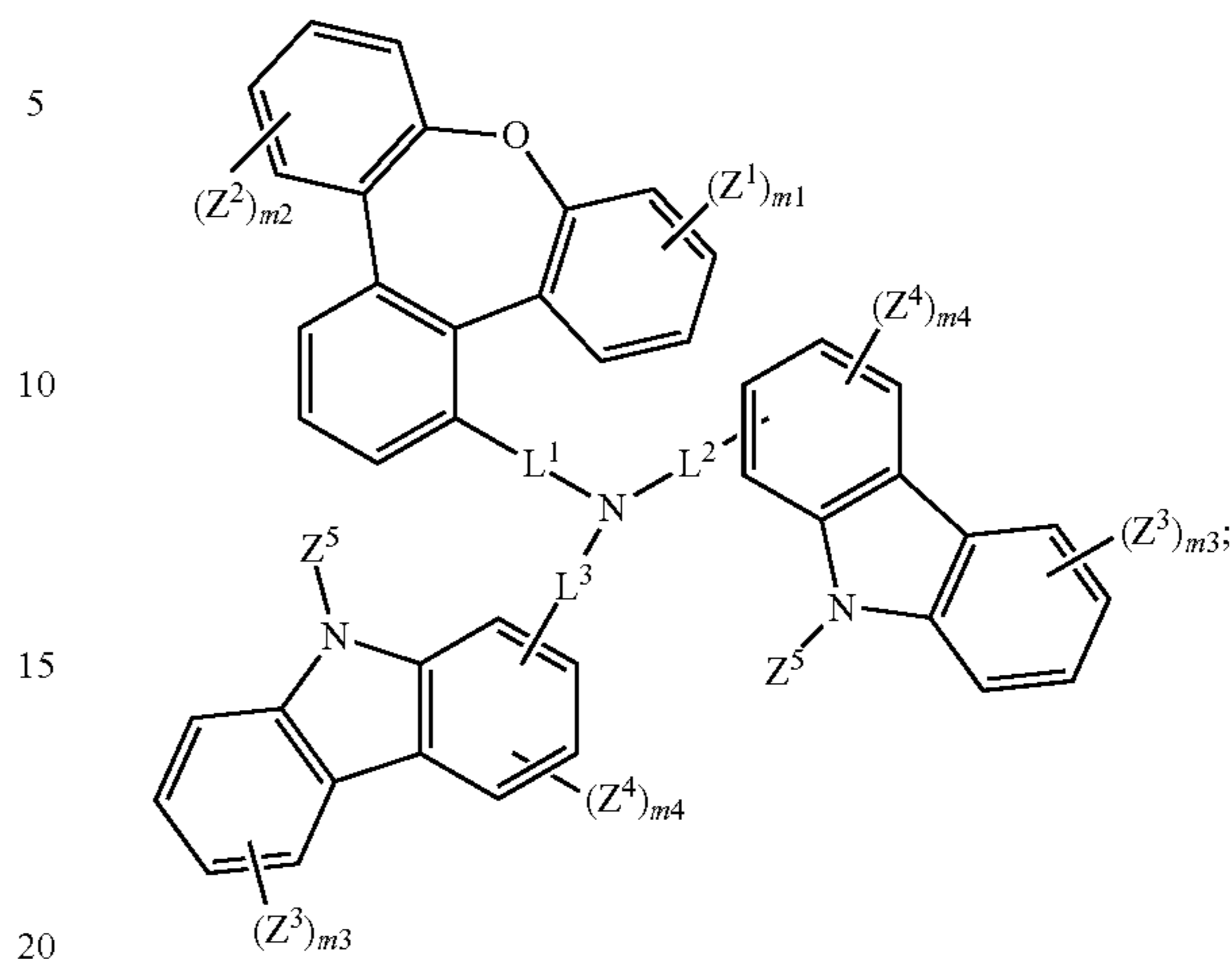
Formula (I-XXIX)
