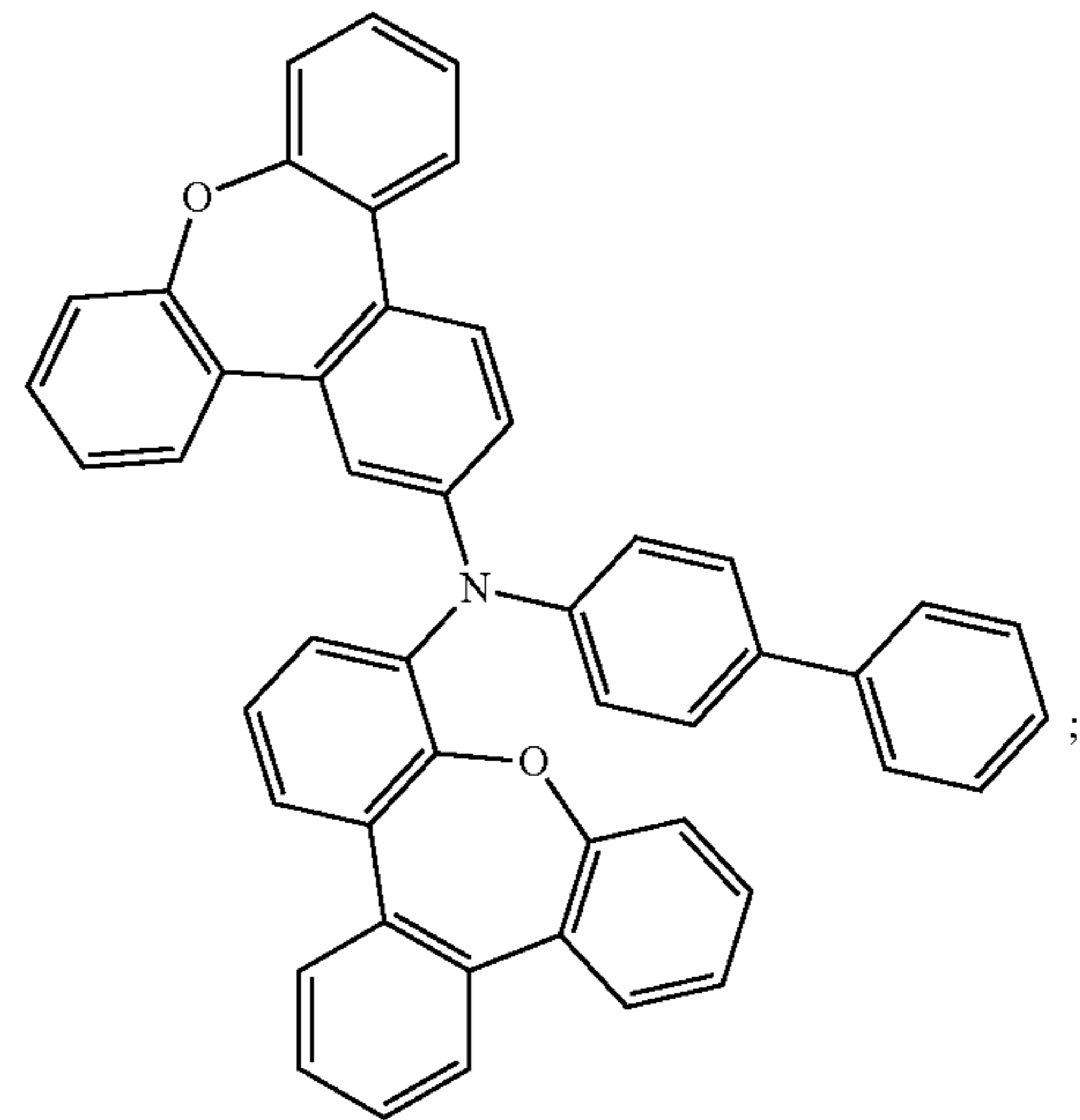
Compound 49
