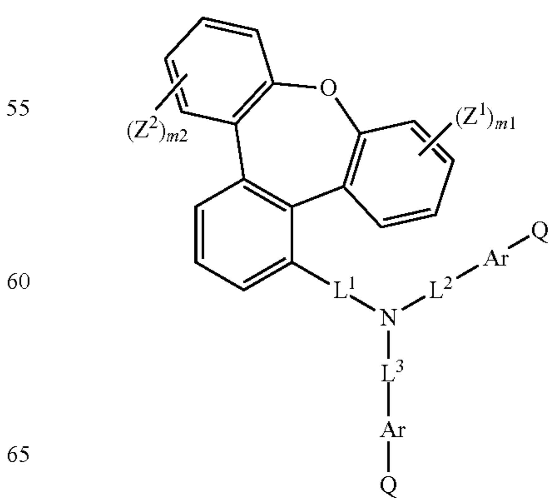
Formula (I-XVIII)
