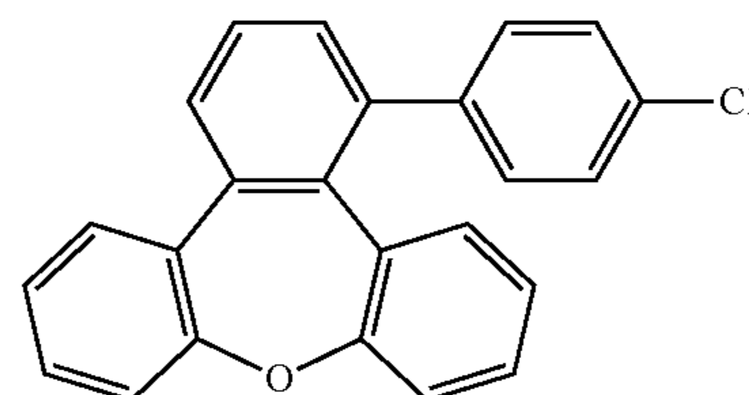
Intermediate C3
