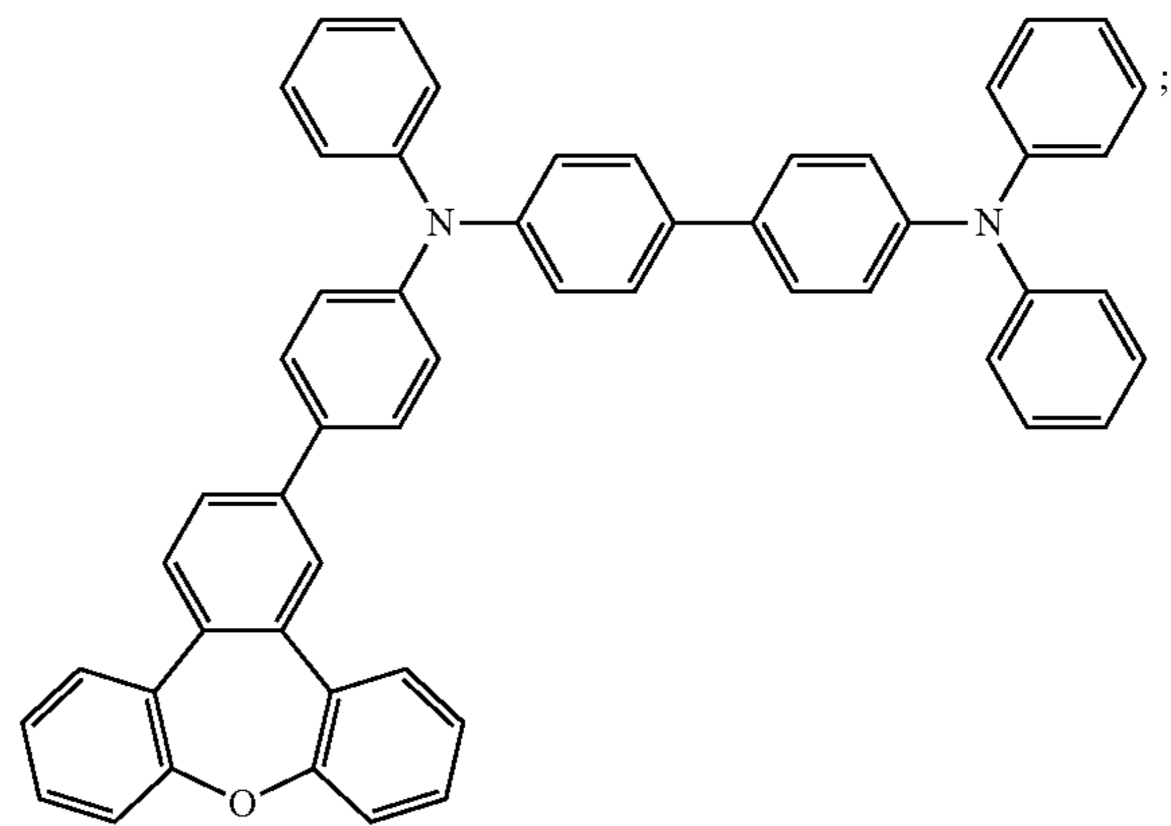
Compound 18
