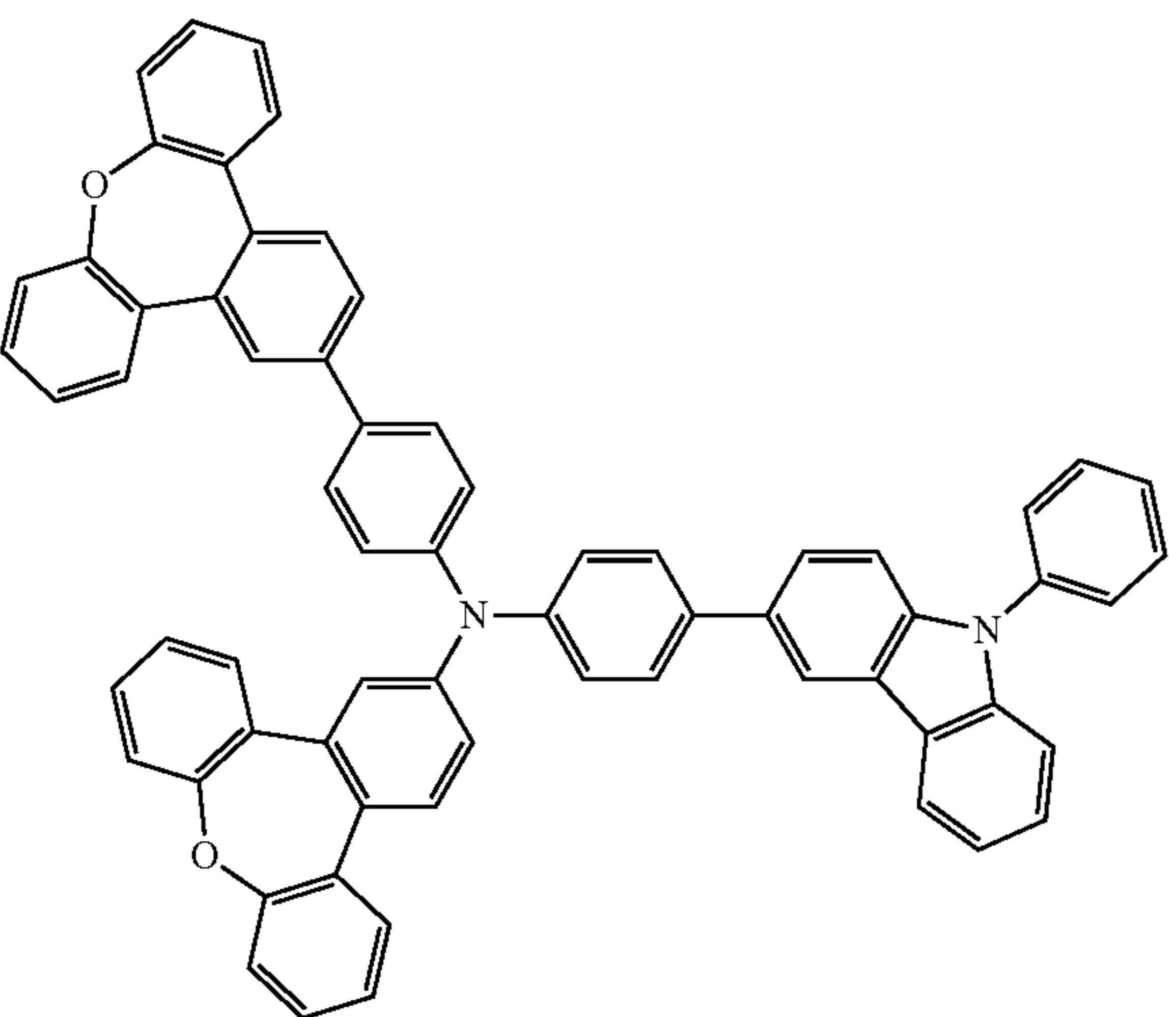
Compound 35
