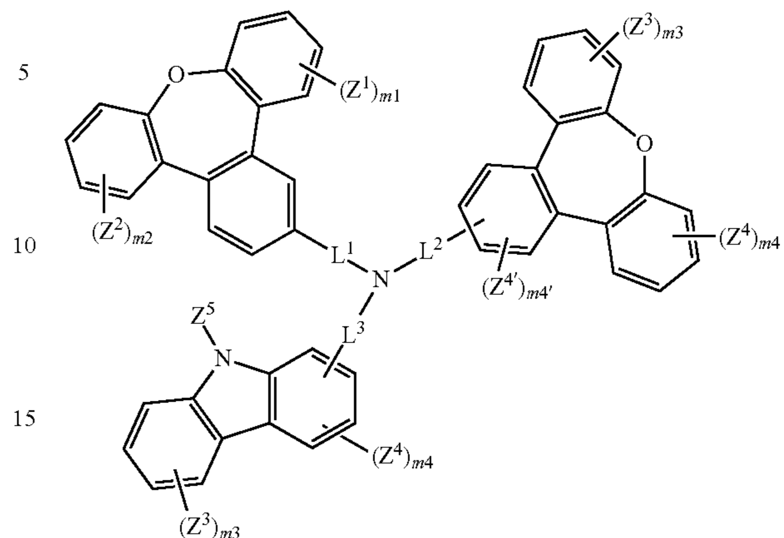
Formula (I-XIII)
