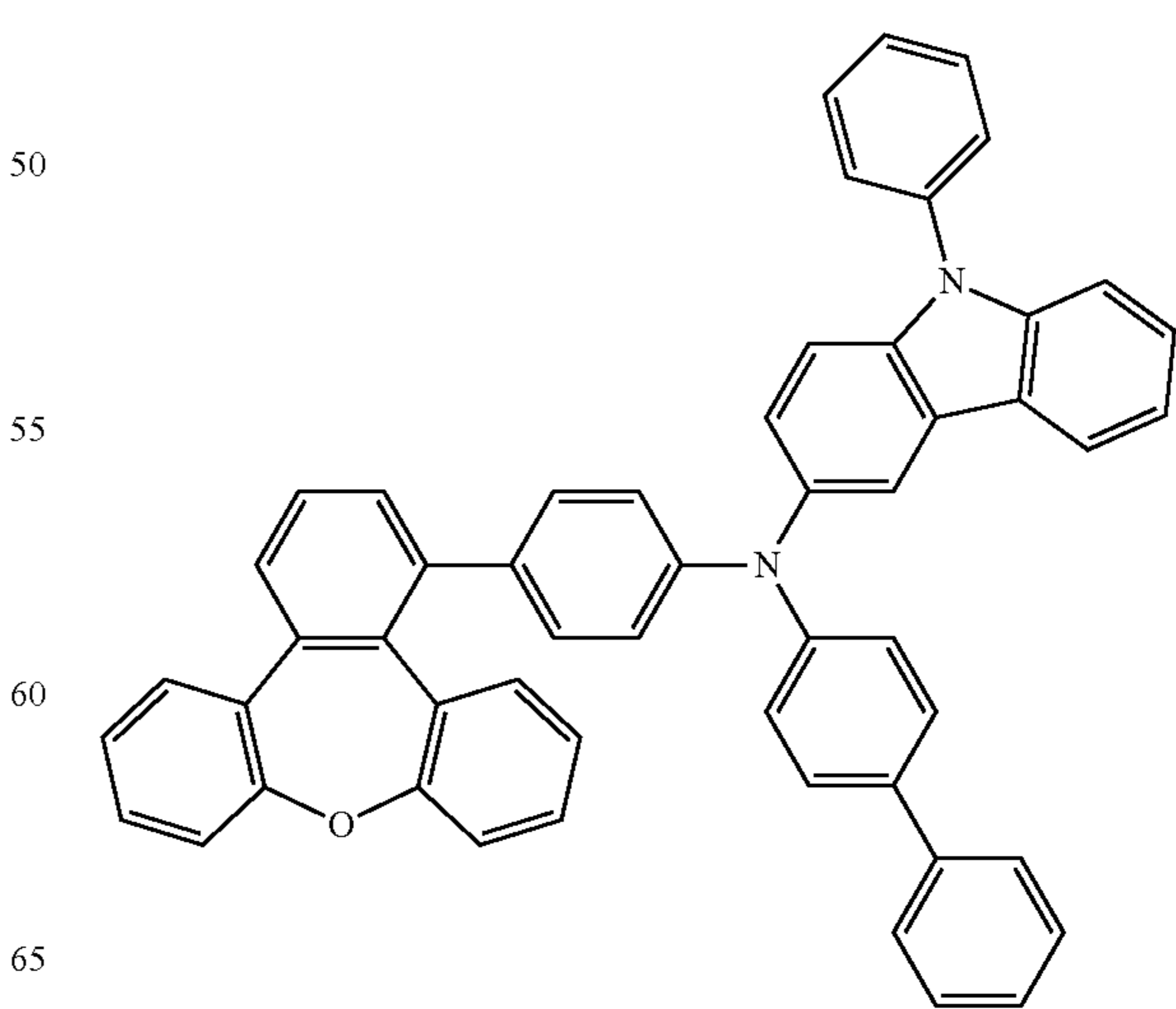
Compound 21
