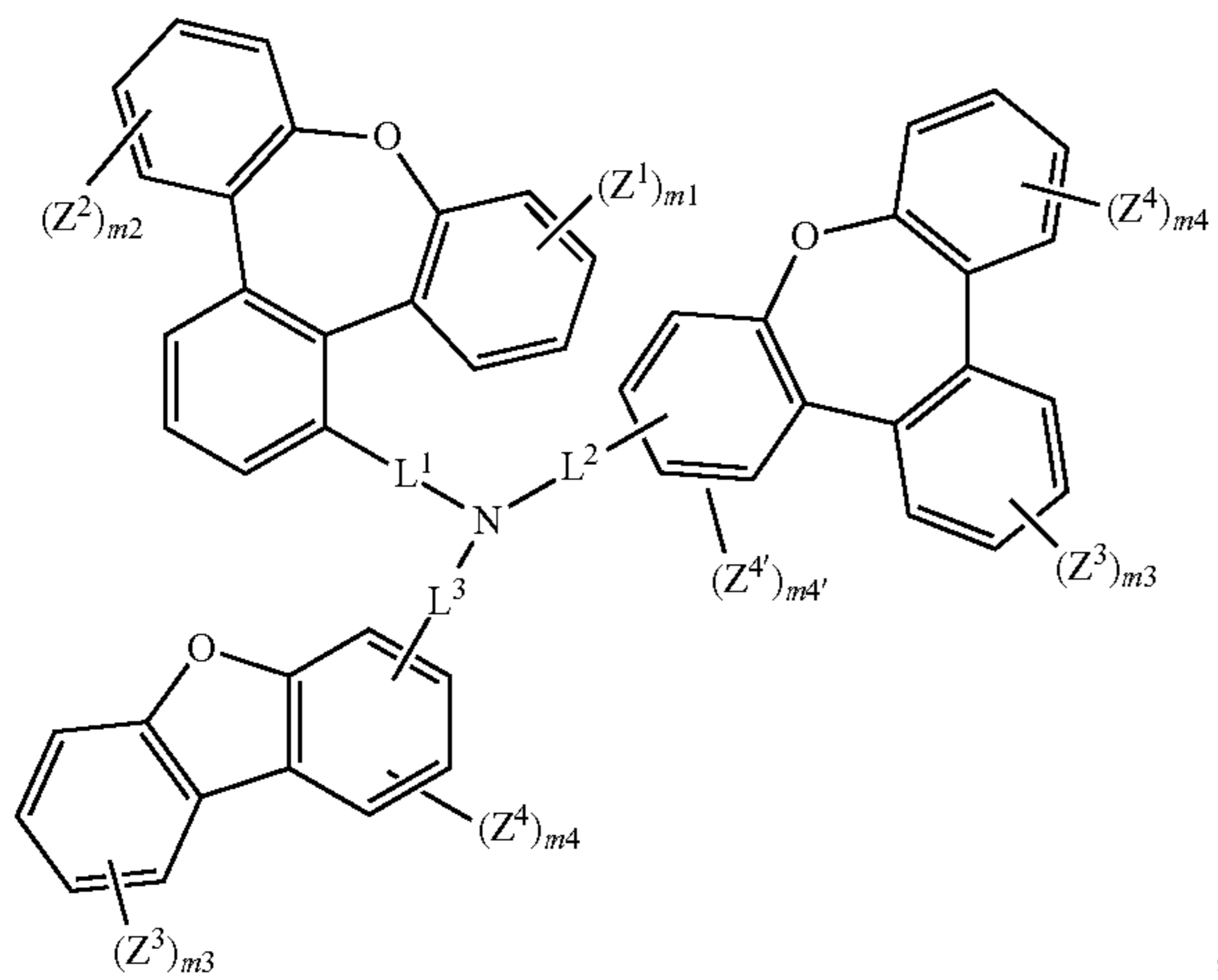
Formula (I-XVII)
