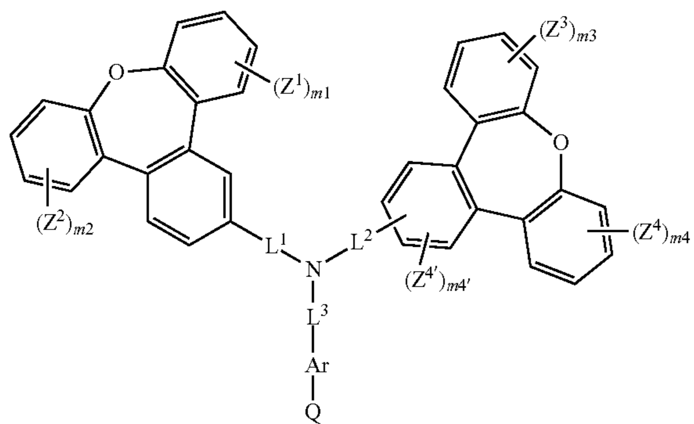
Formula (I-XII)
