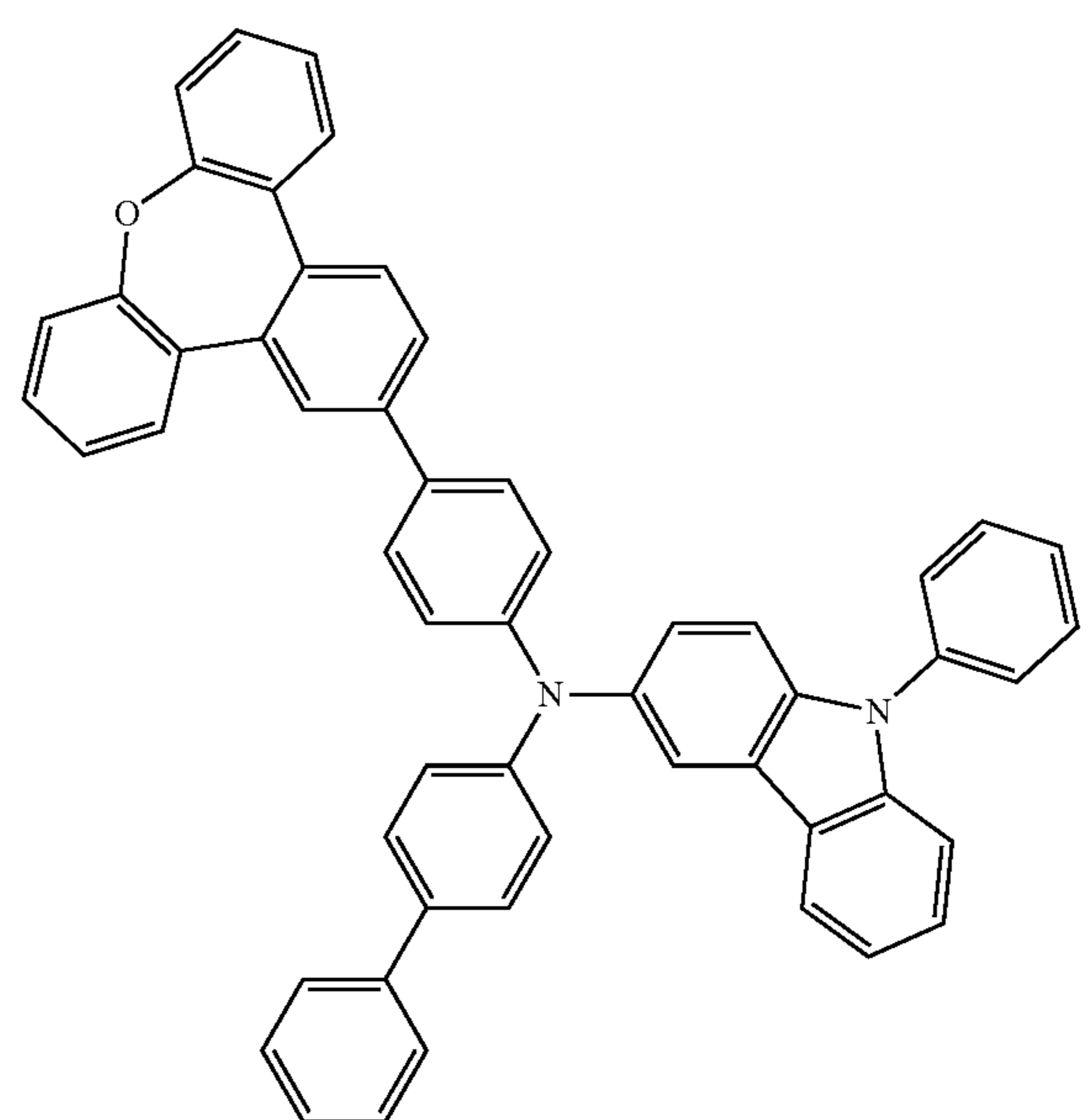
Compound 20
