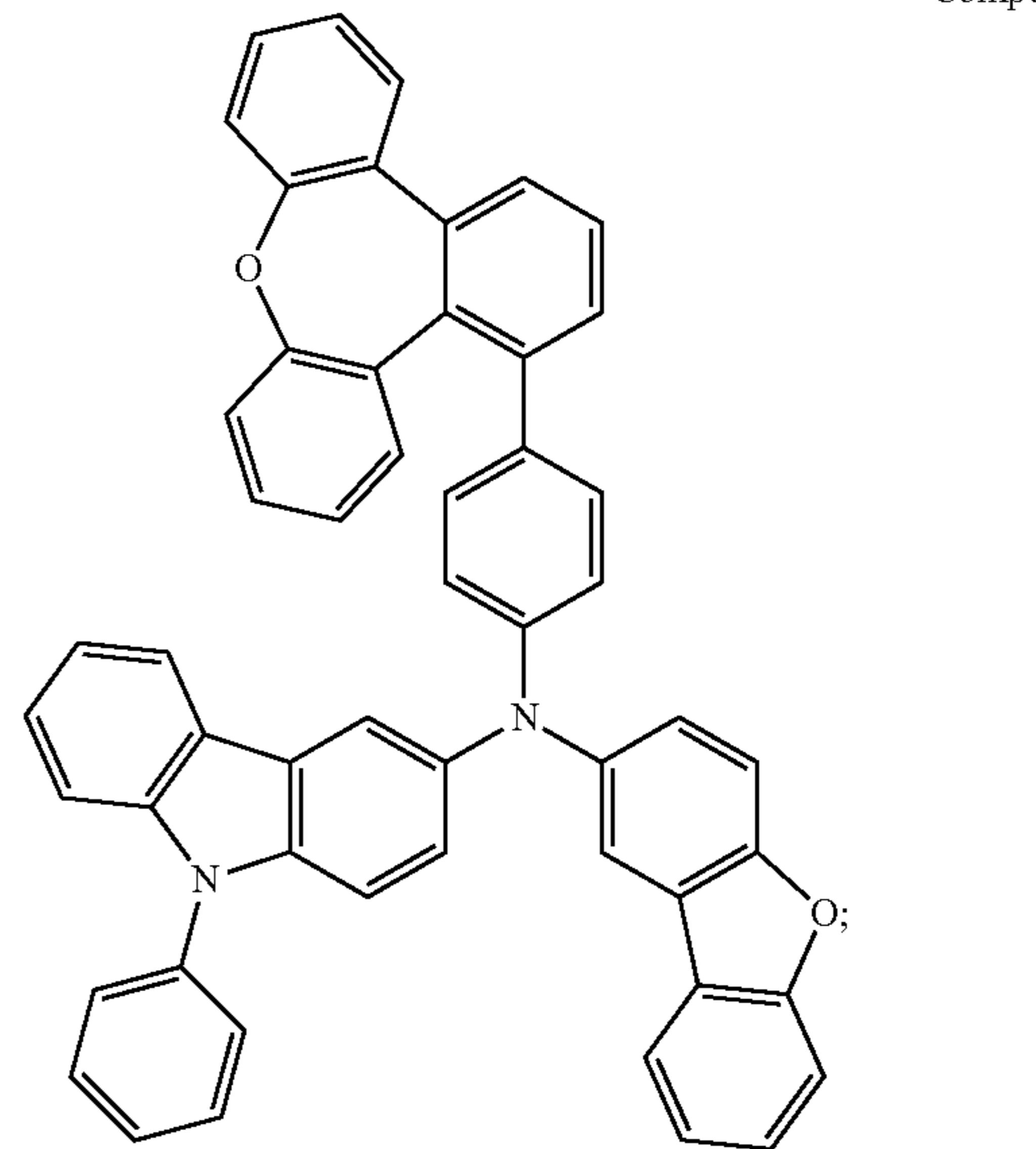
Compound 68
