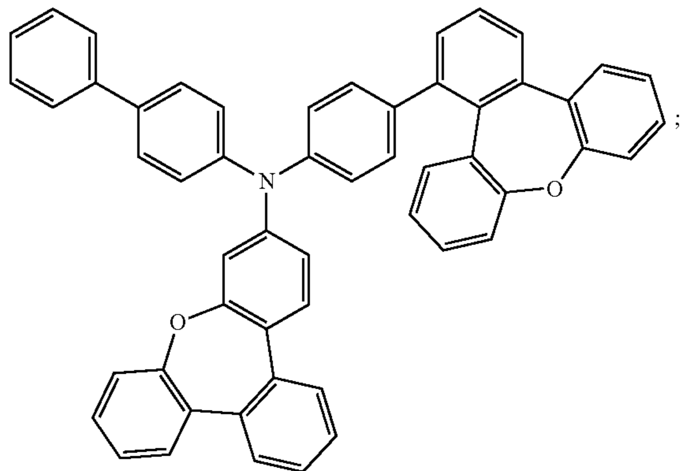
Compound 105
