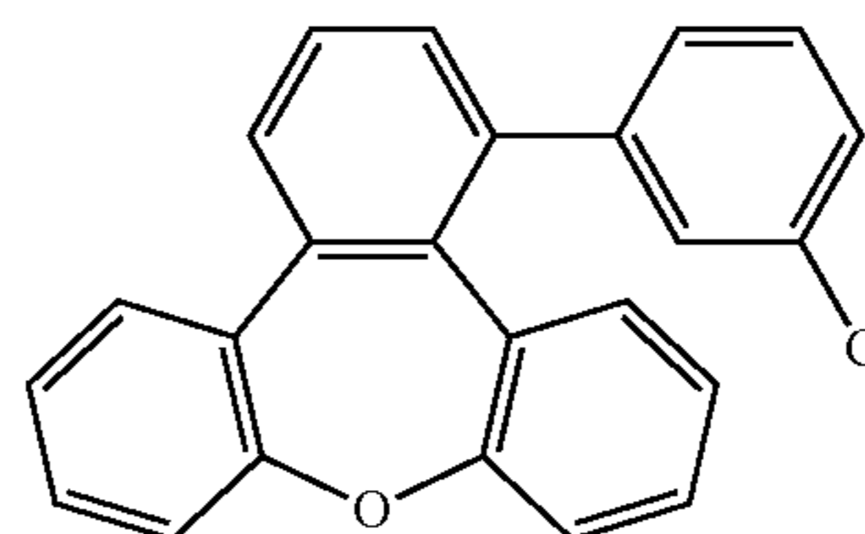
Intermediate C4
