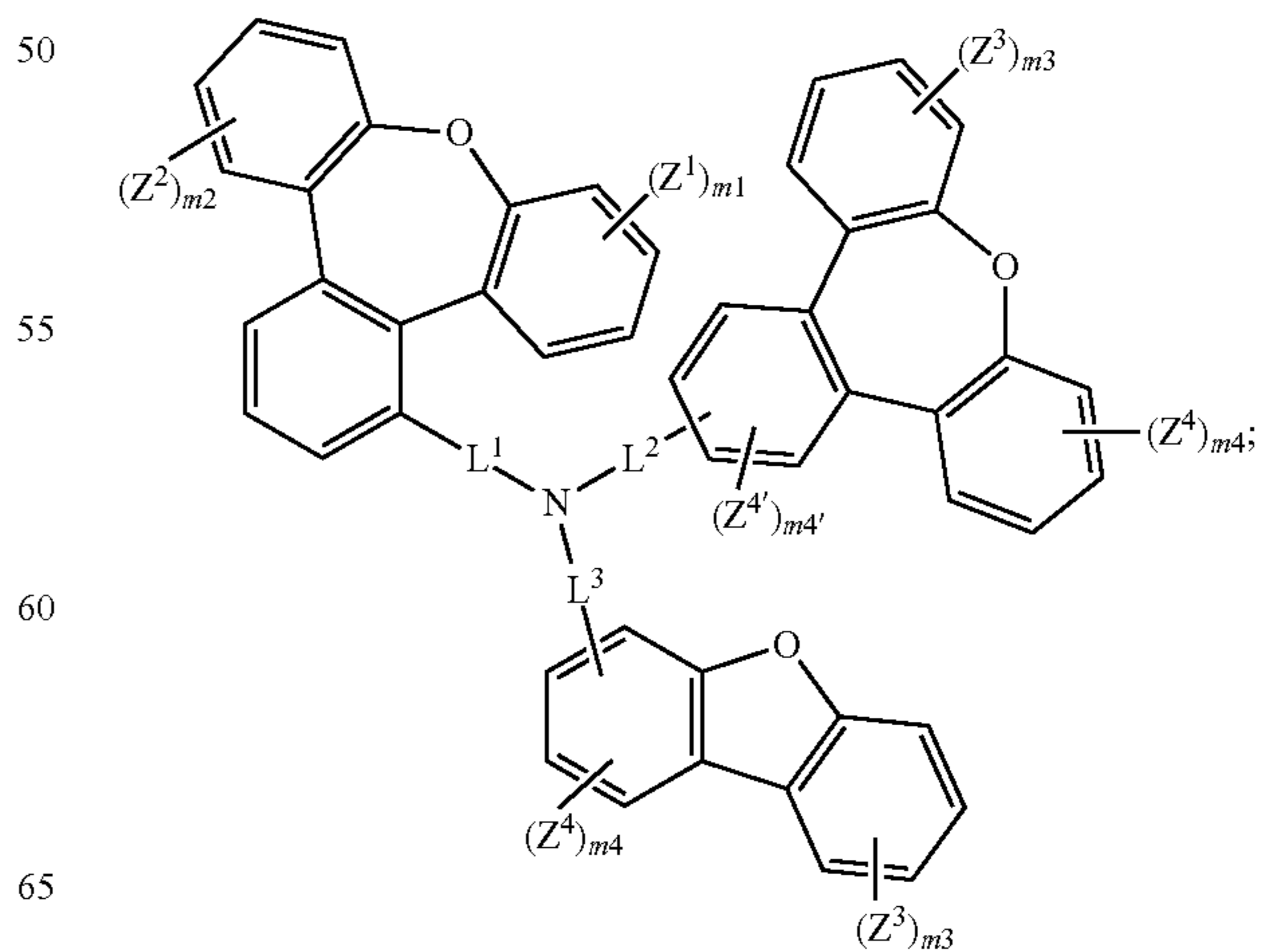
Formula (I-XI)
