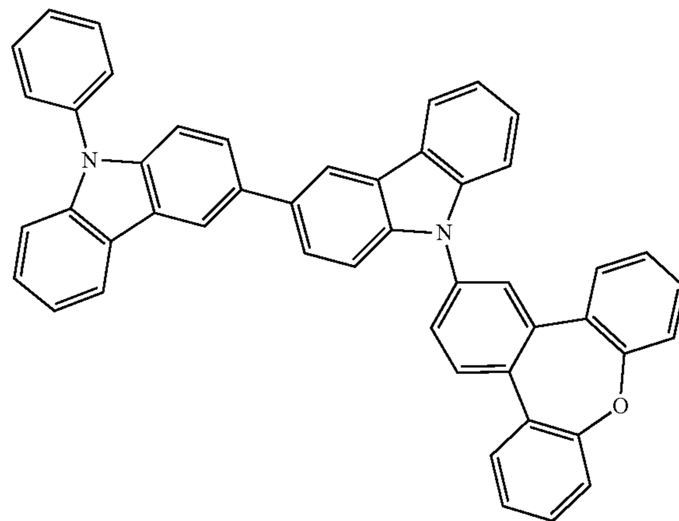
Compound 30
