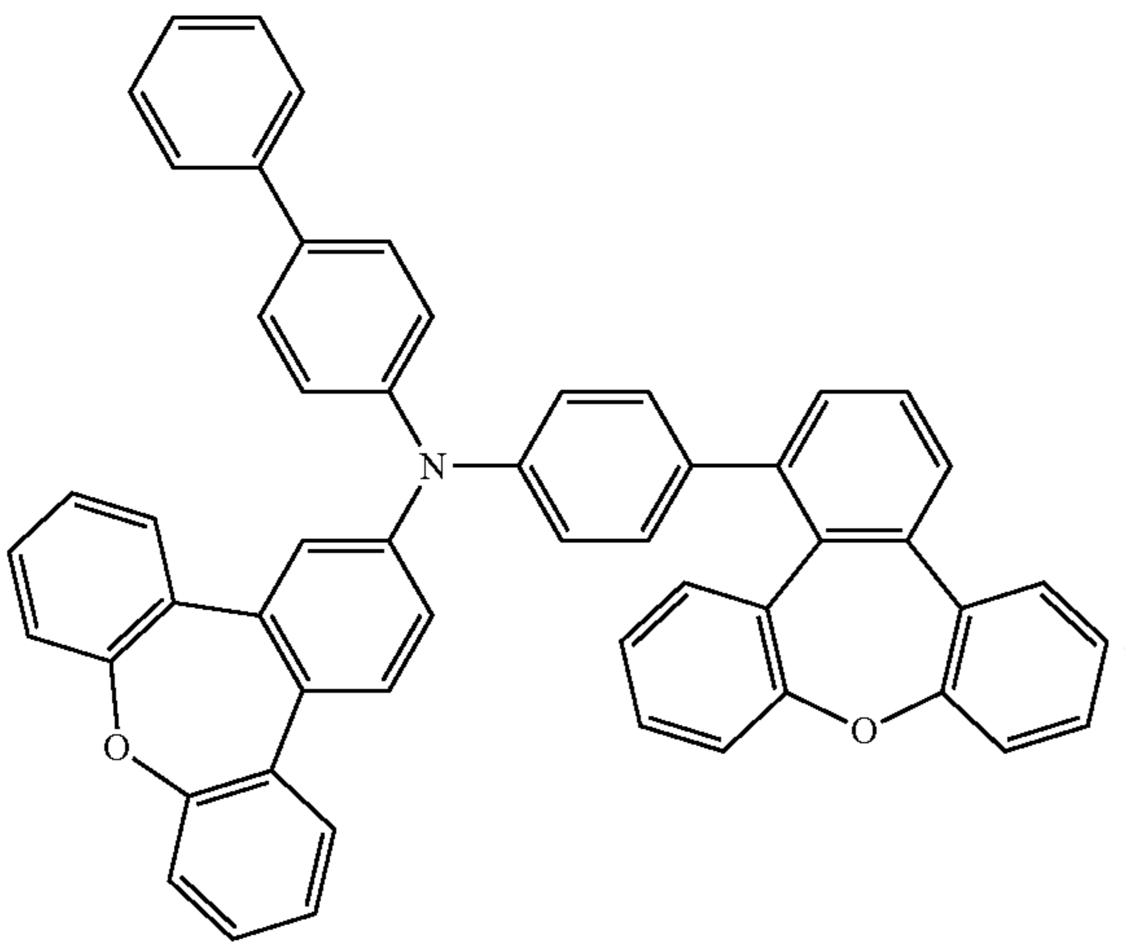
Compound 115
