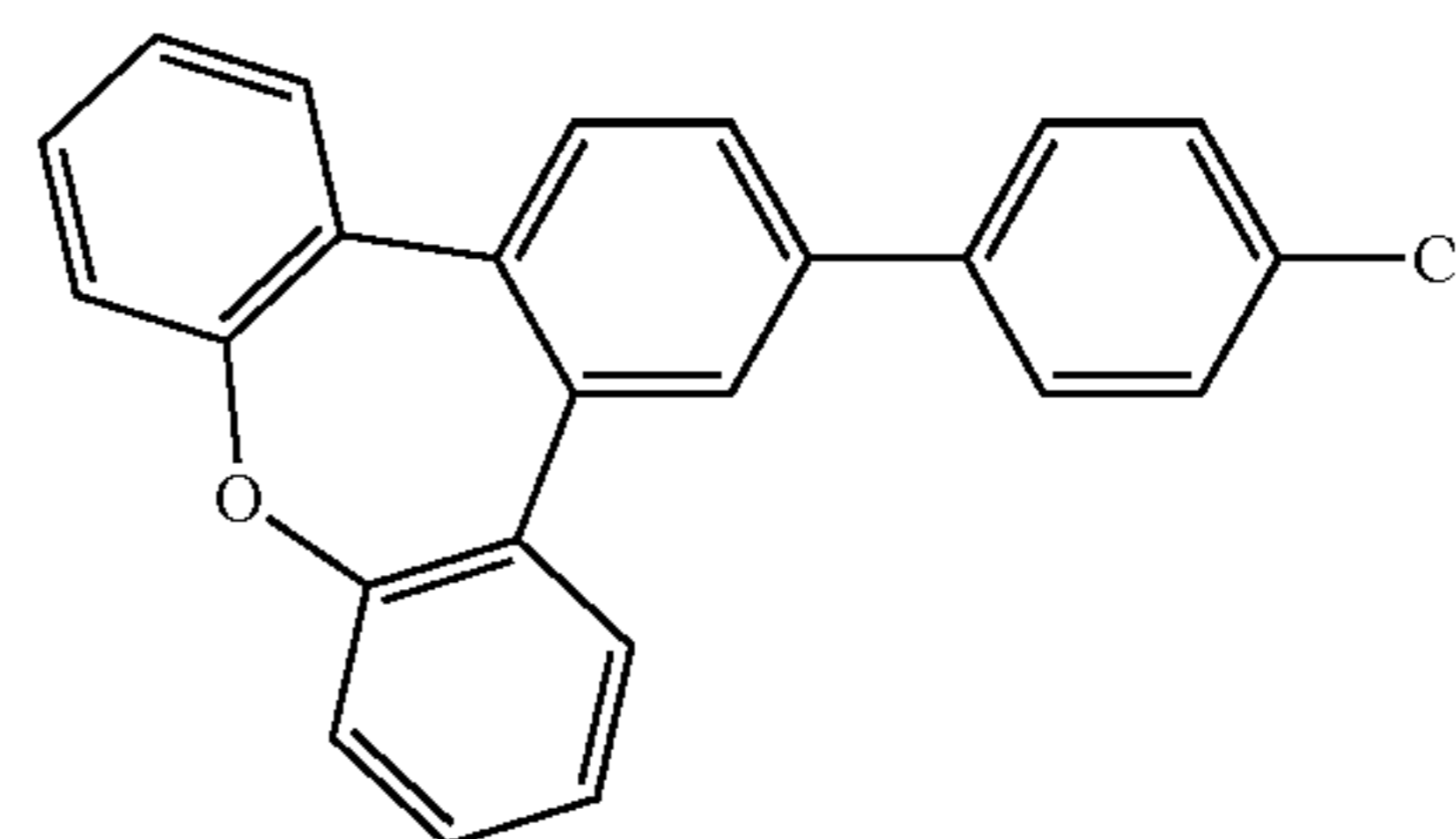
Intermediate C2
