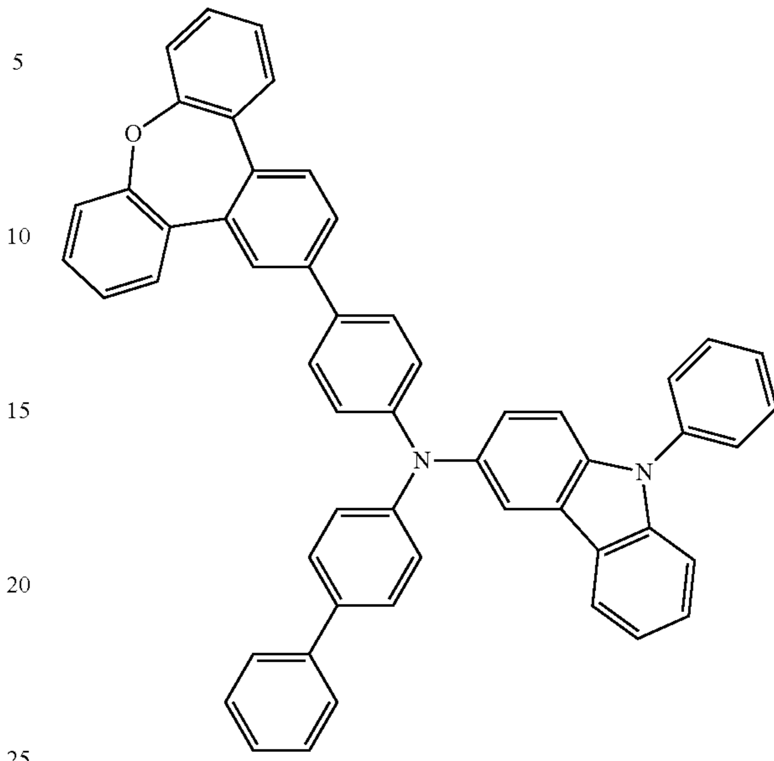
Compound 20
