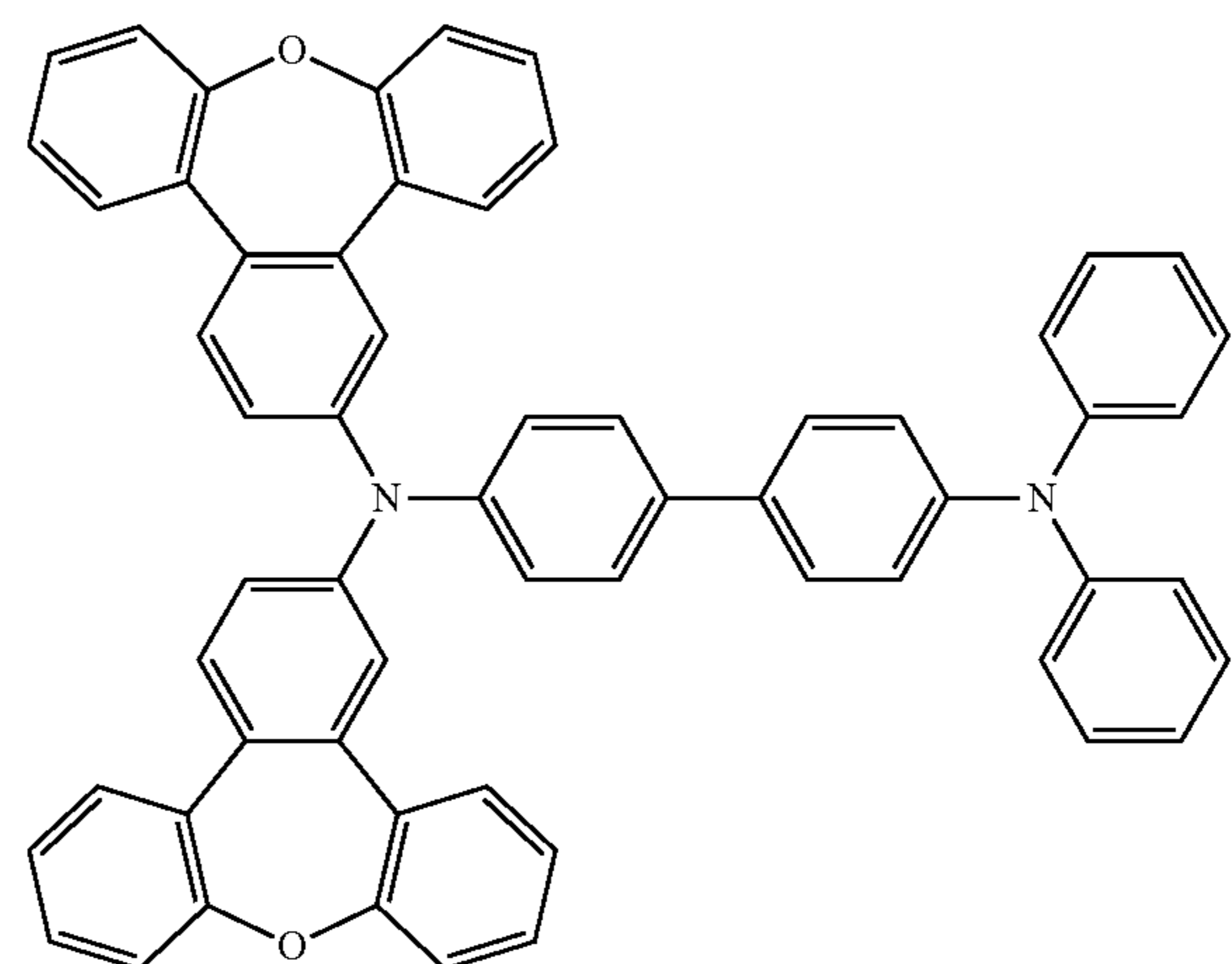
Compound 16
