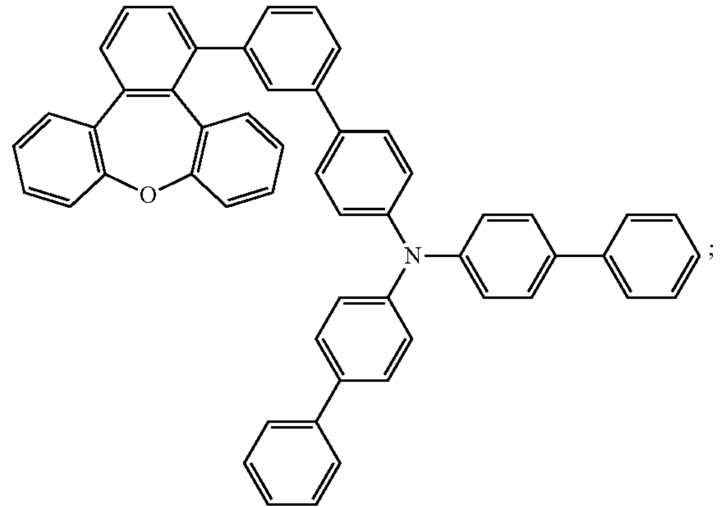
Compound 5
