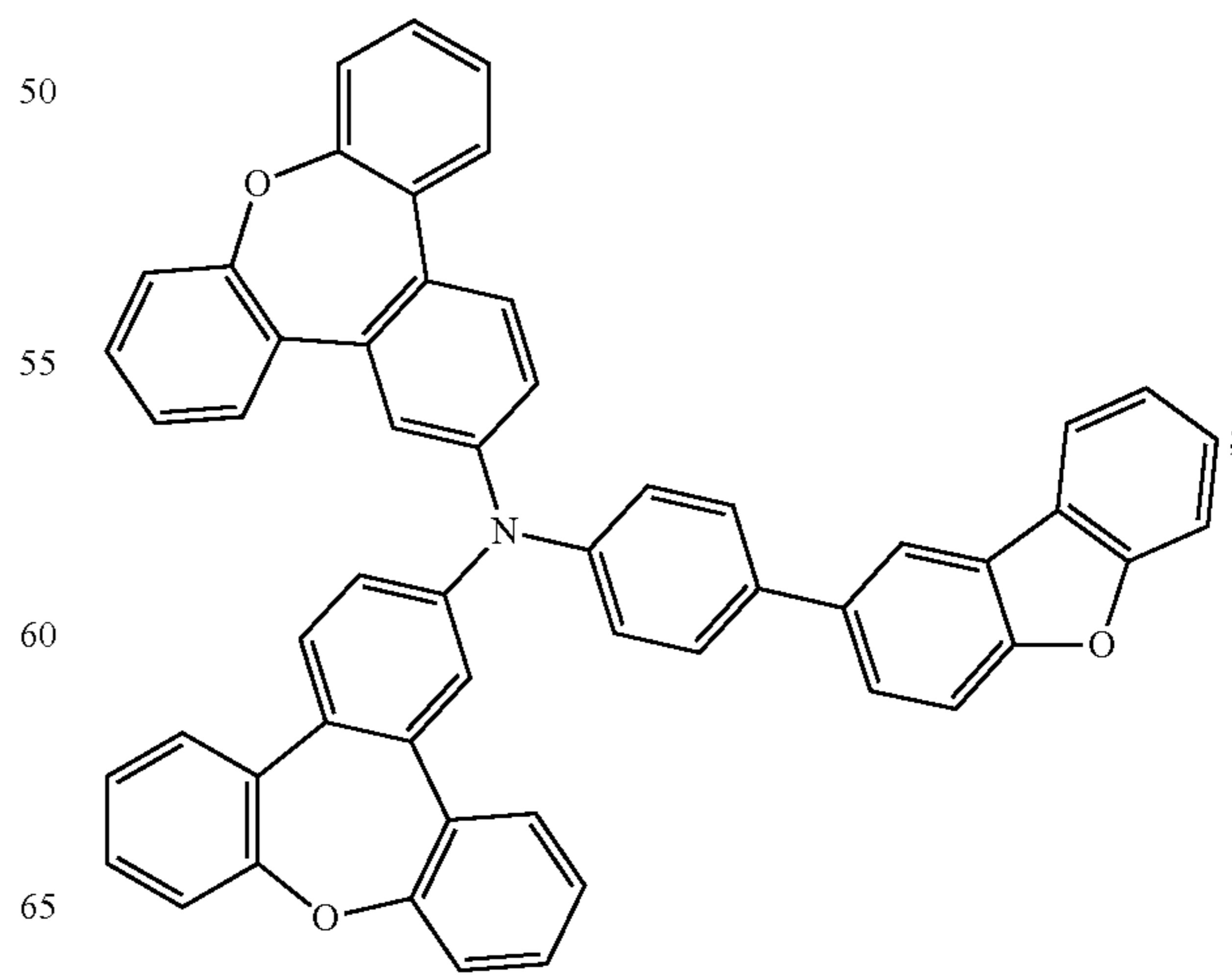
Compound 140
