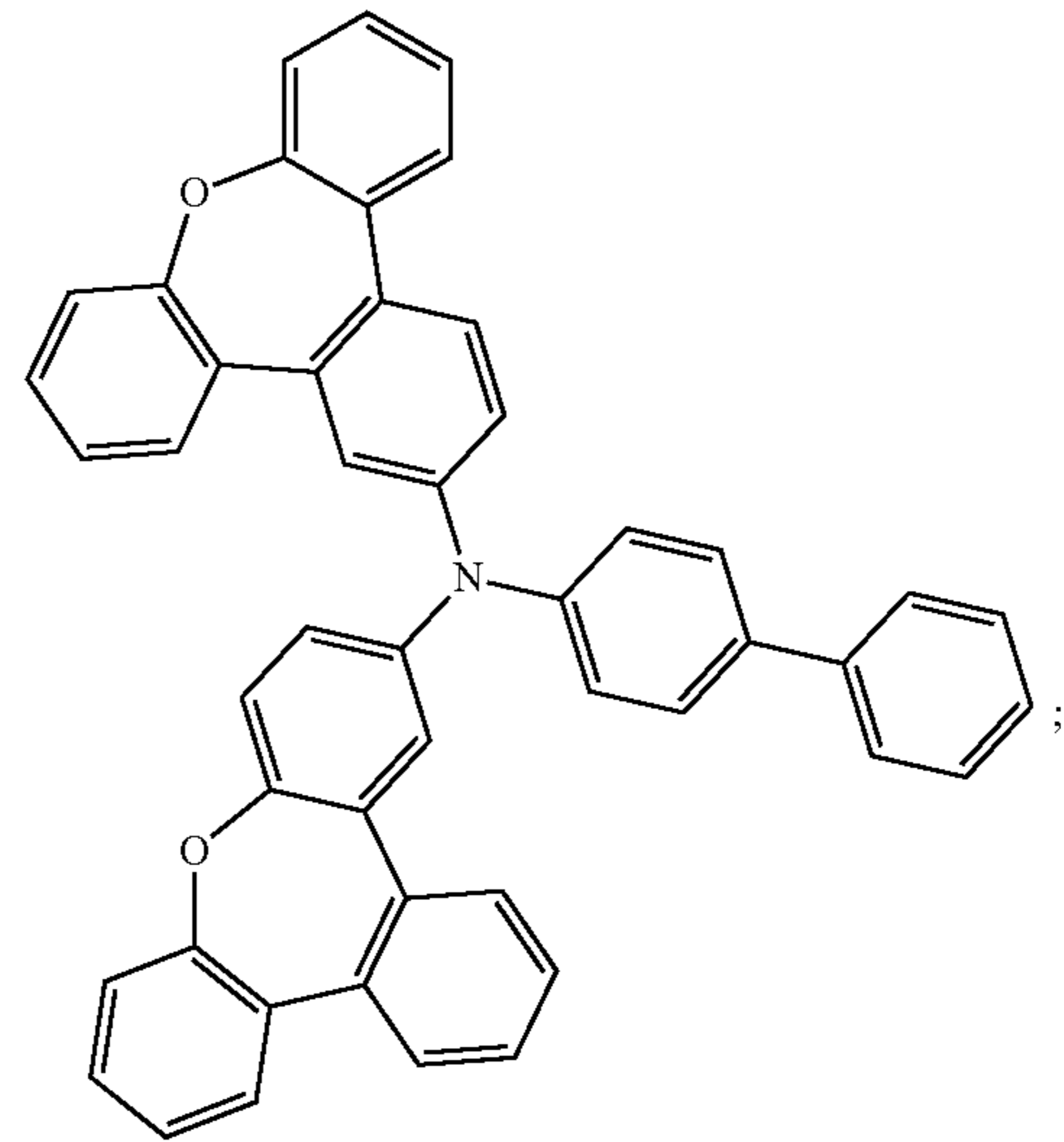
Compound 48
