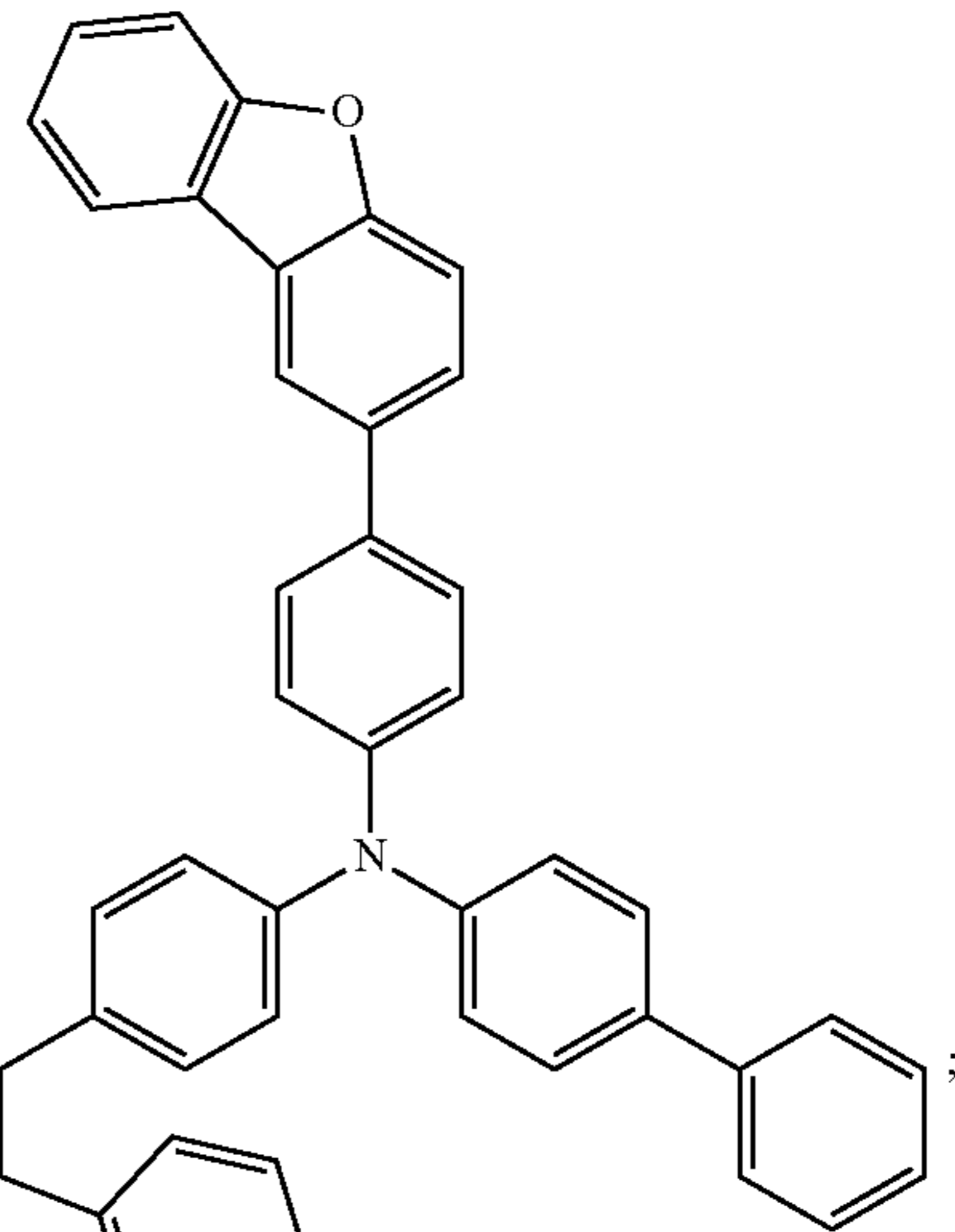
Compound 133
