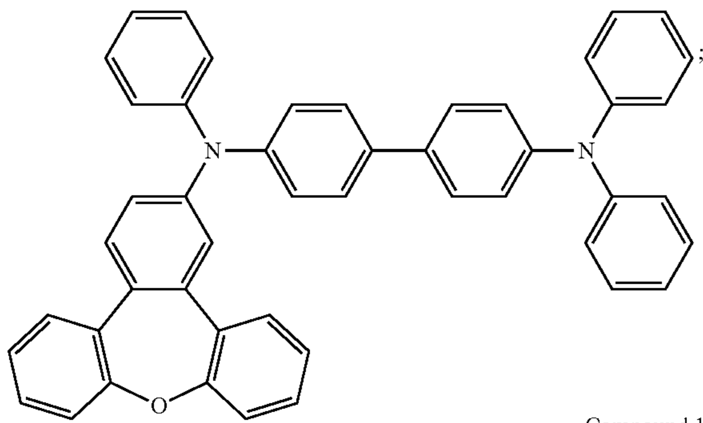
Compound 15
