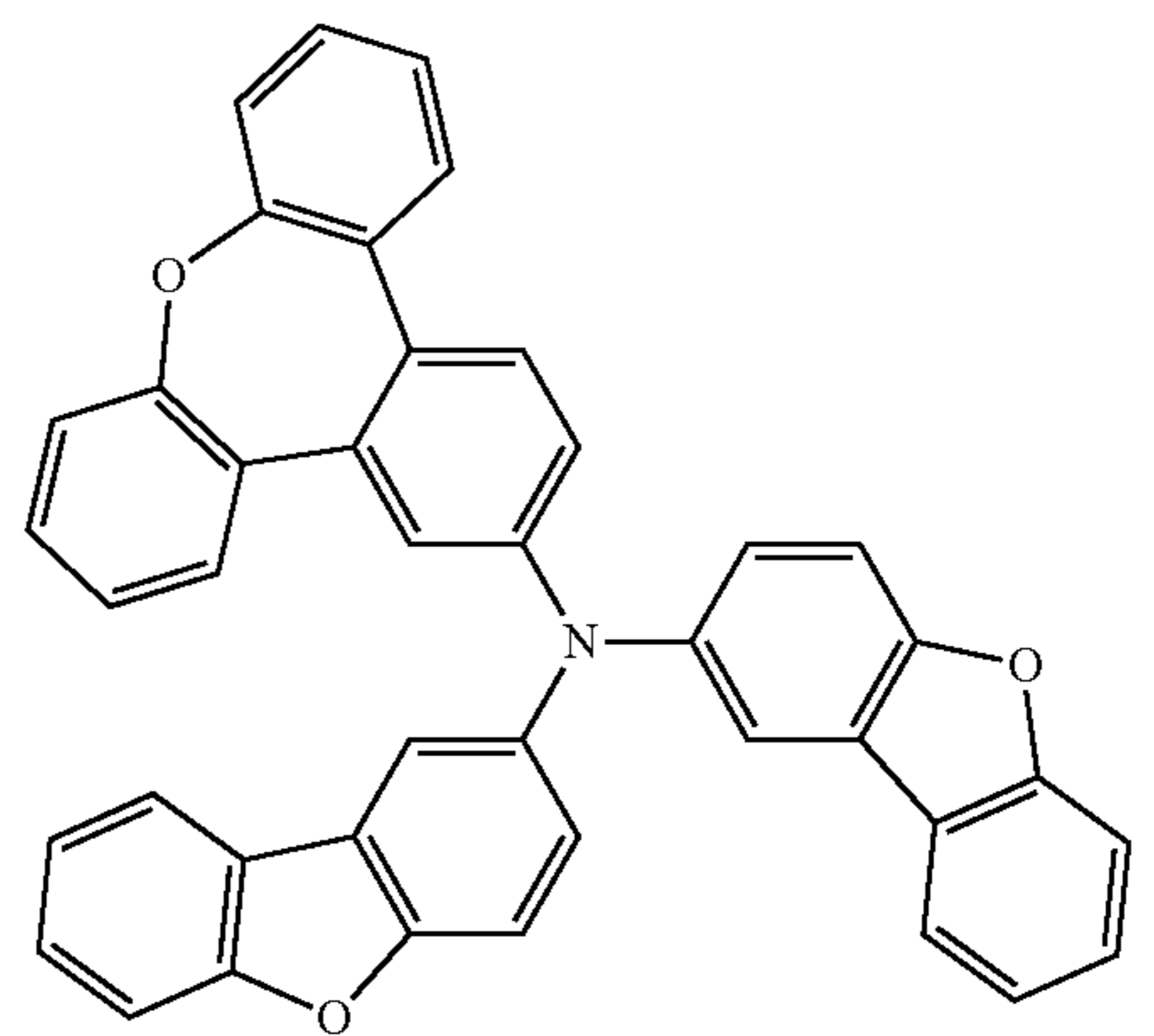
Compound 74
