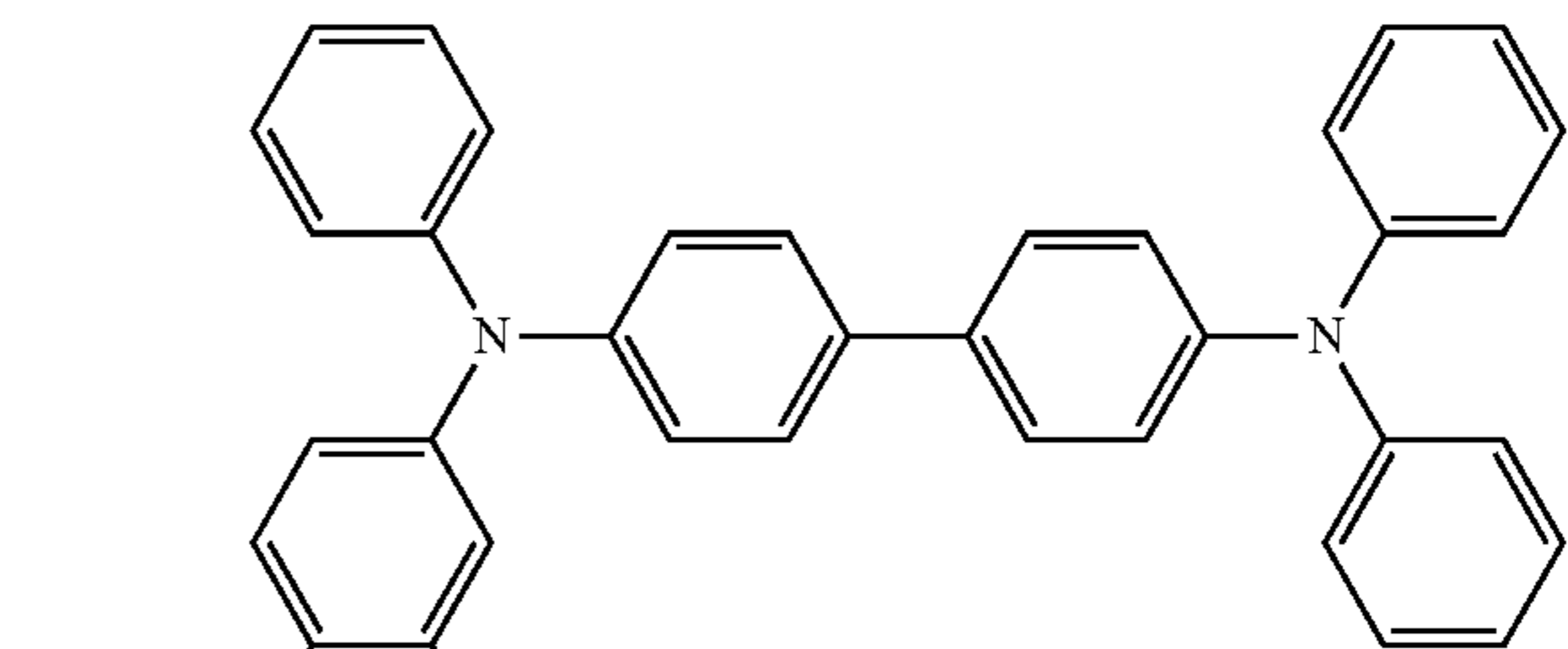
Compound 14
