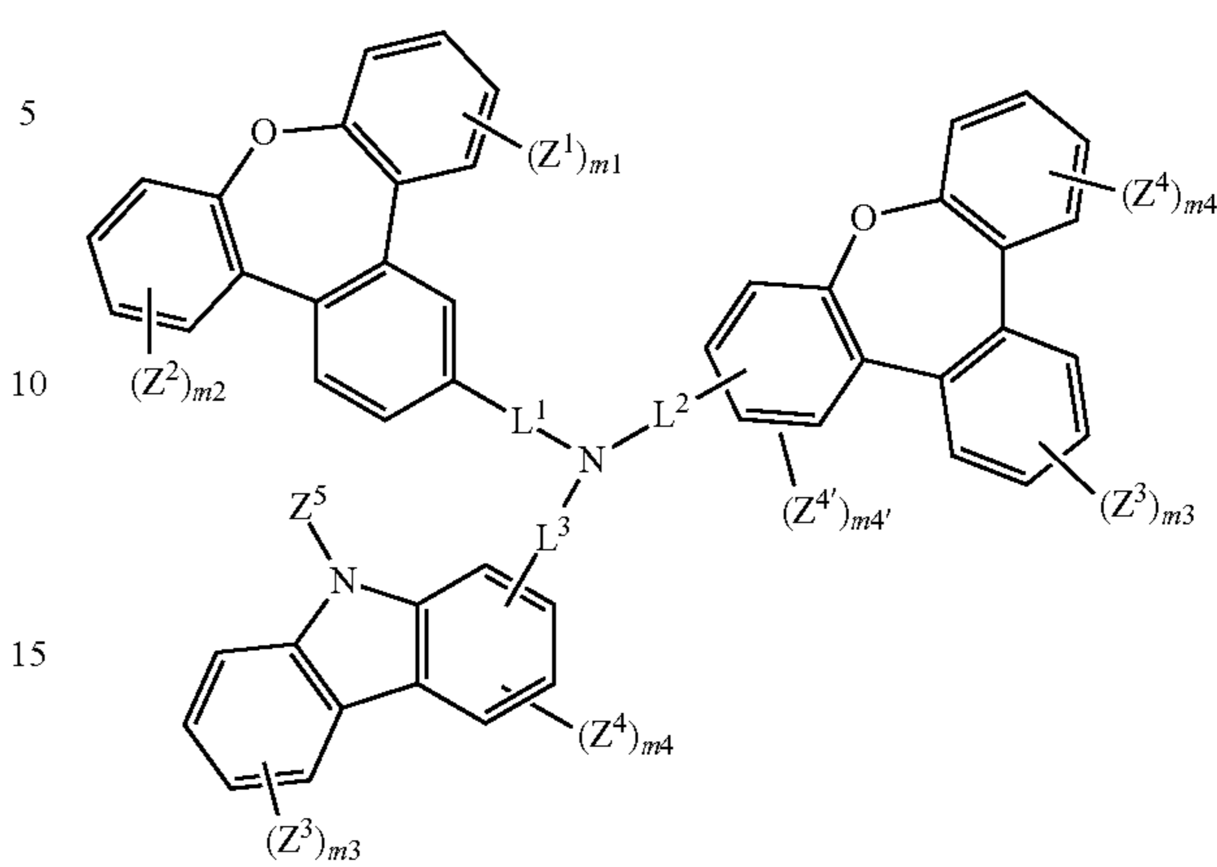
Formula (I-XIX)
