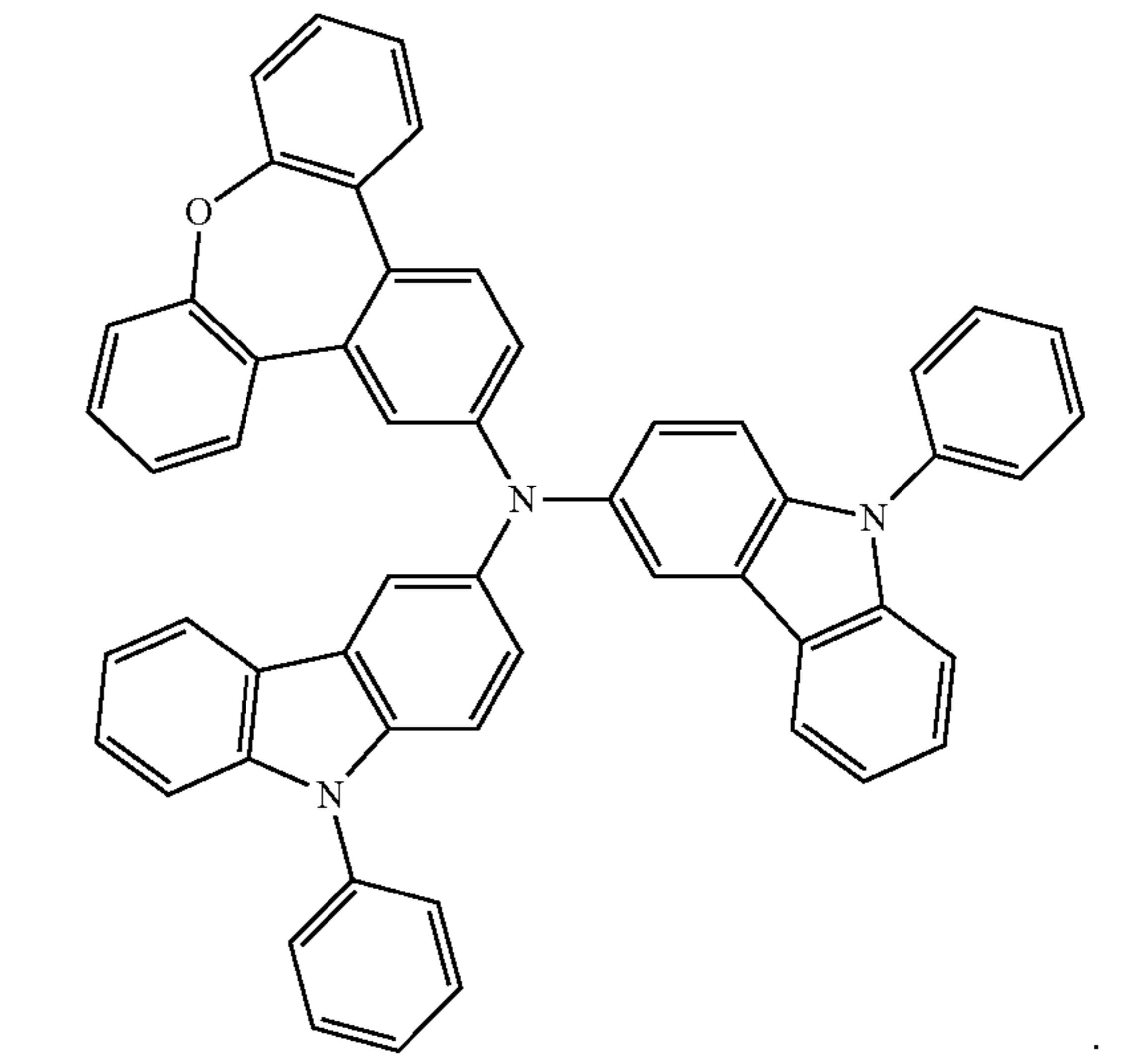
Compound 22
