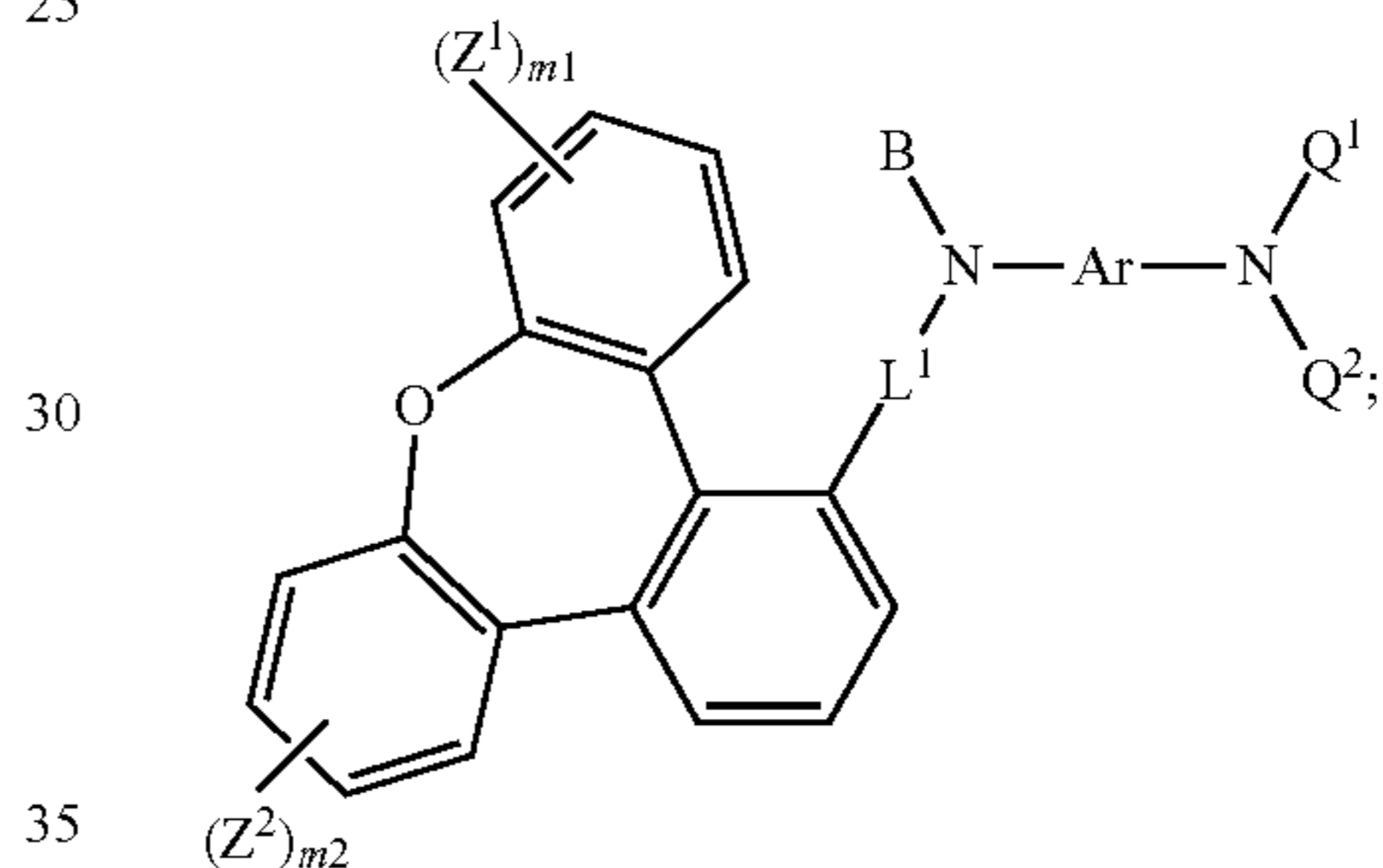
Formula (I-XXXIII)
