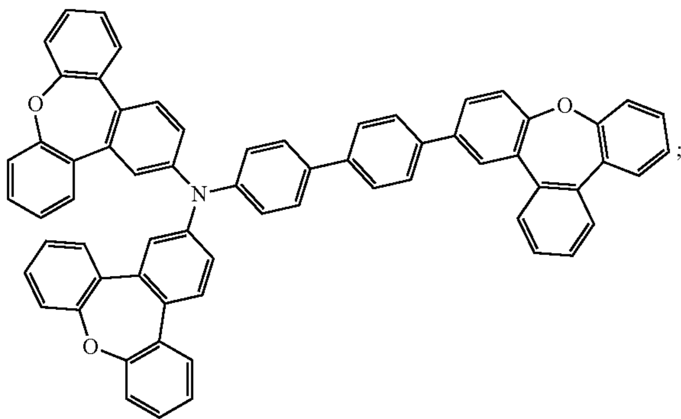
Compound 110
