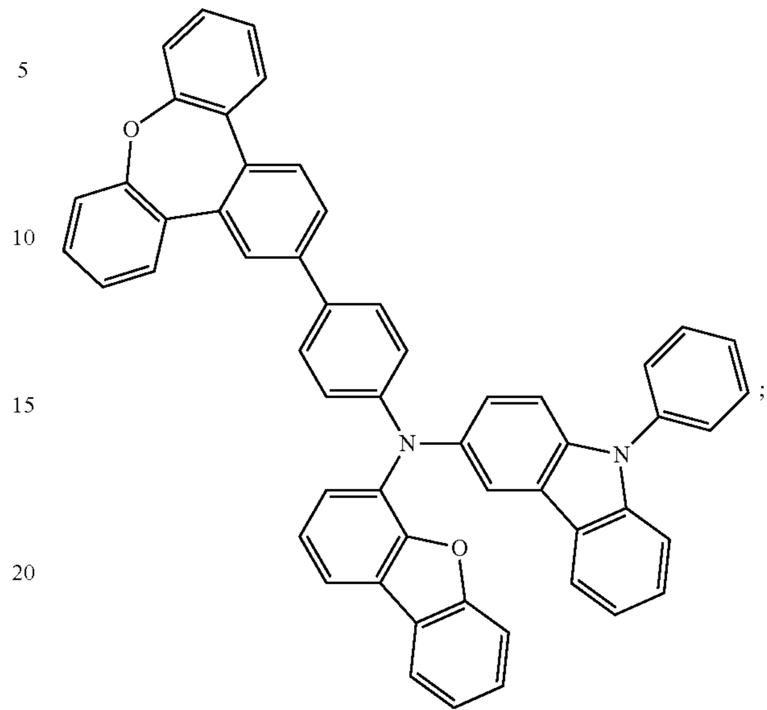
Compound 127
