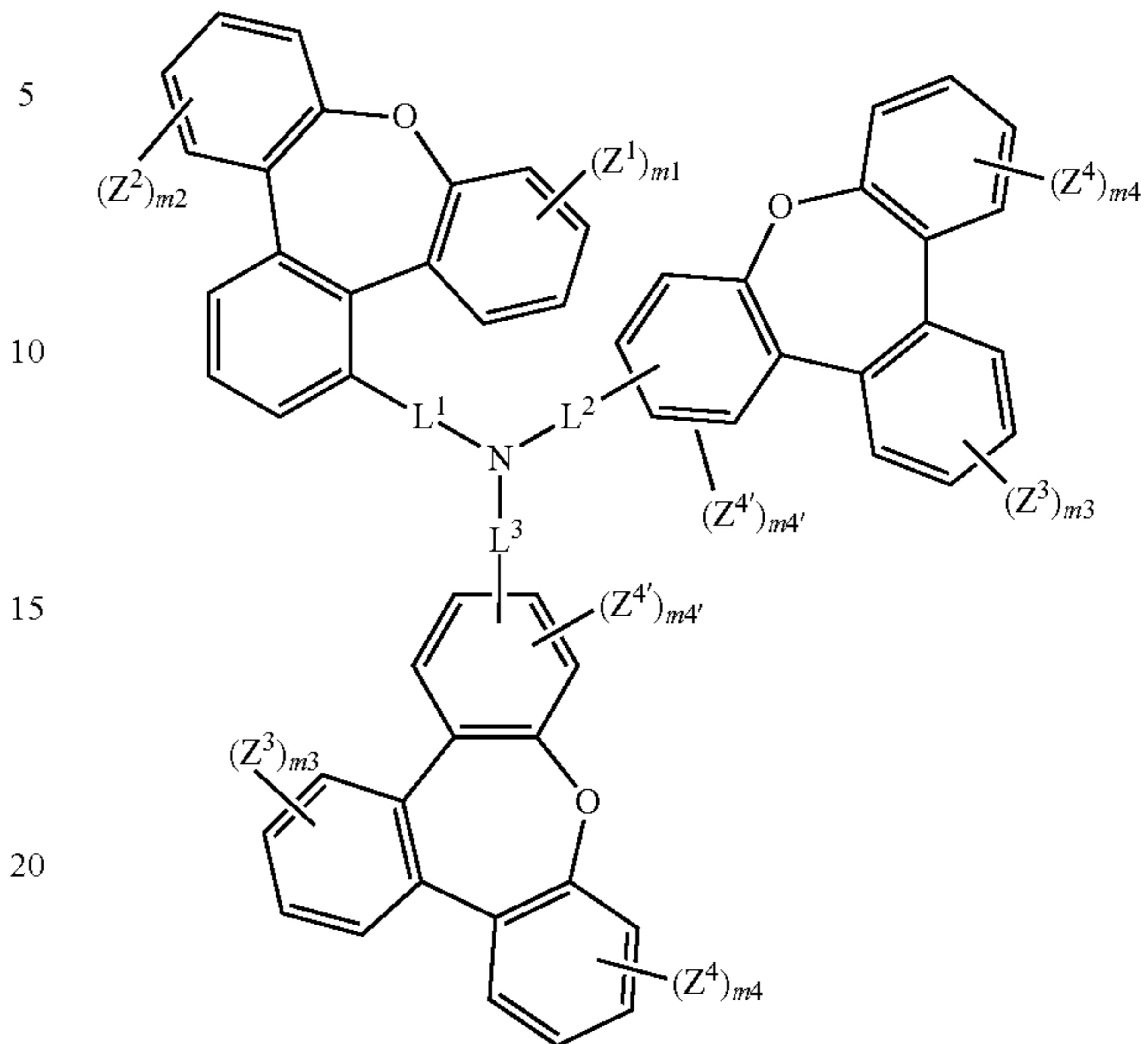
Formula (I-VII)
