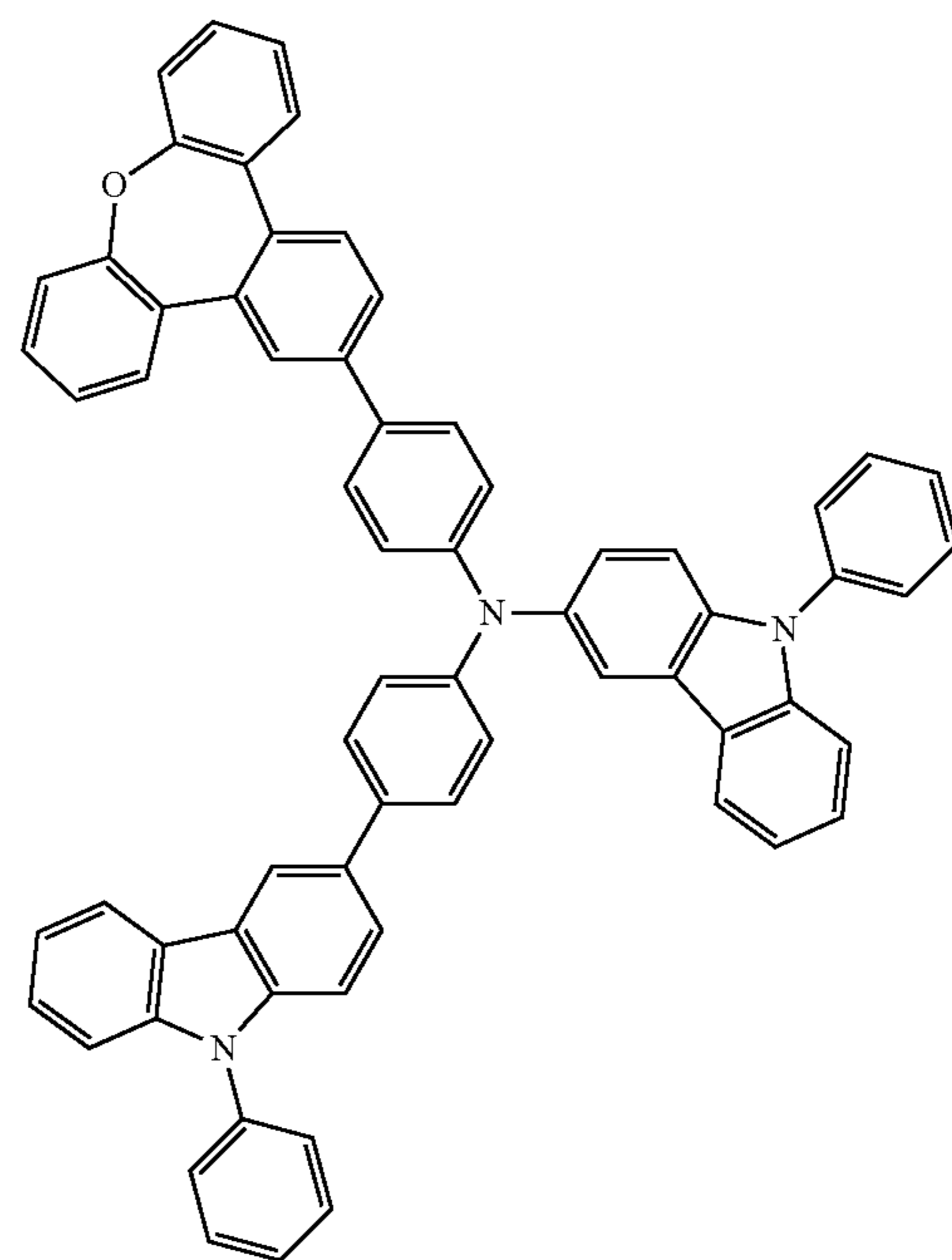
Compound 25
