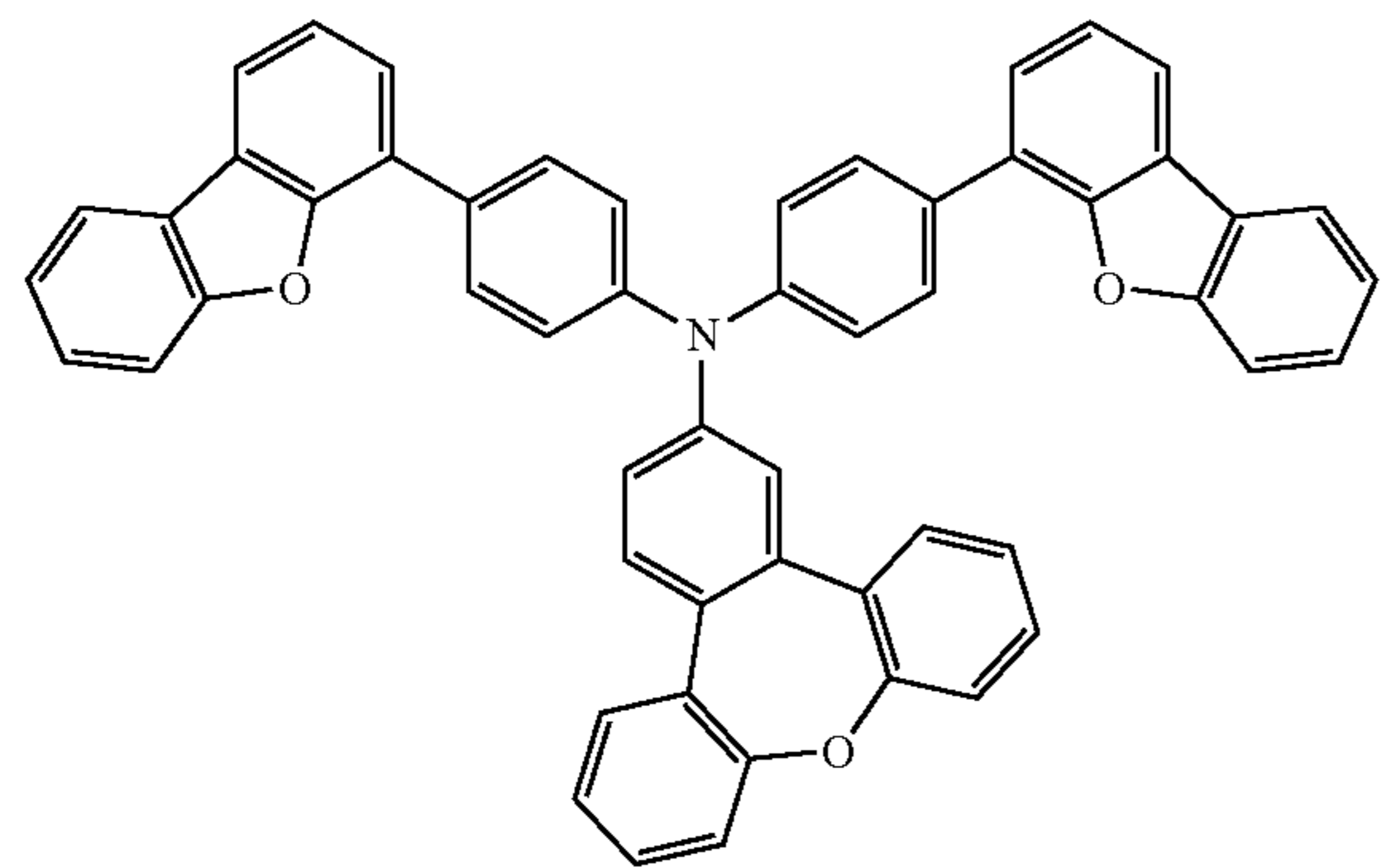
Compound 40
