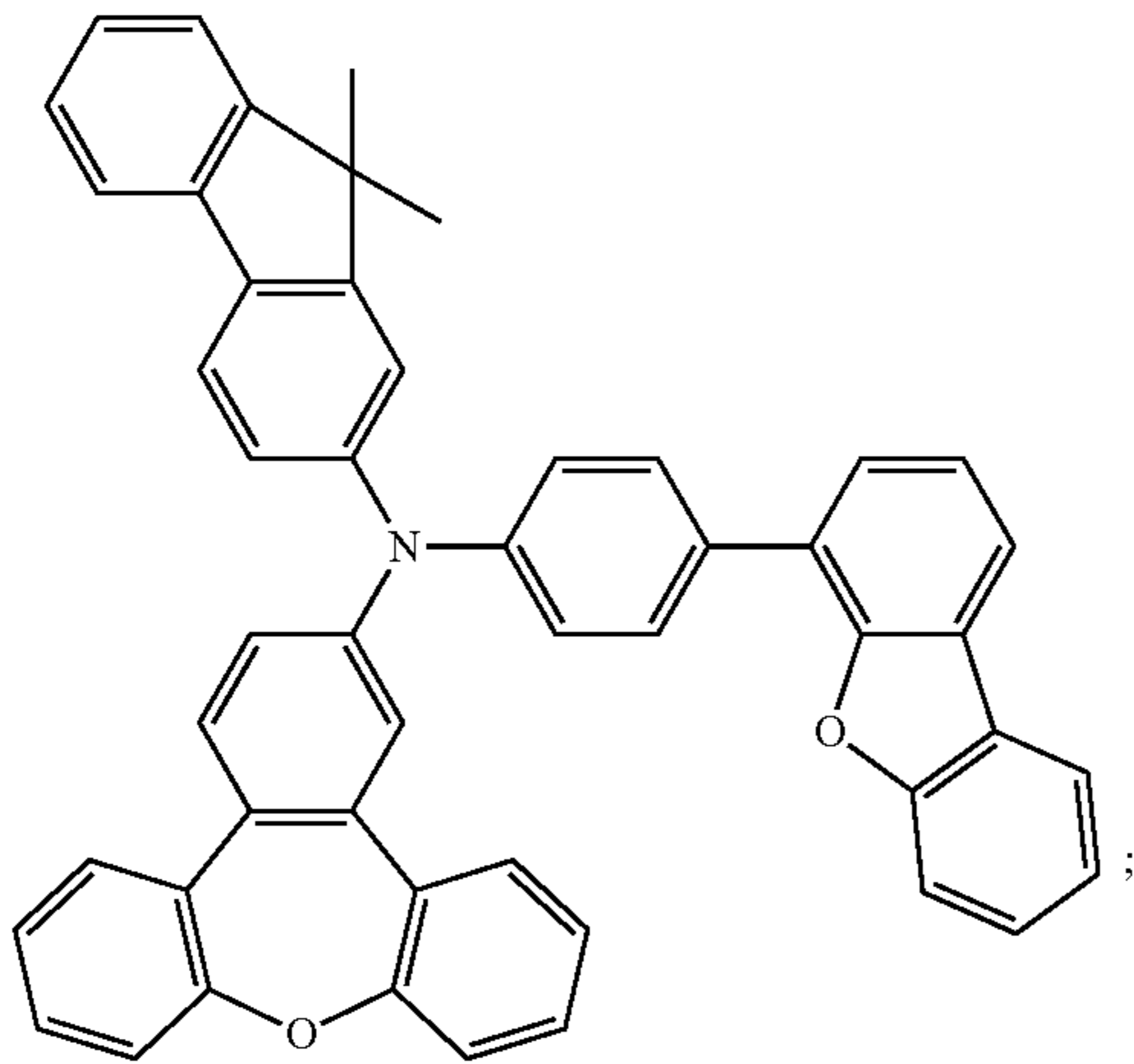
Compound 71
