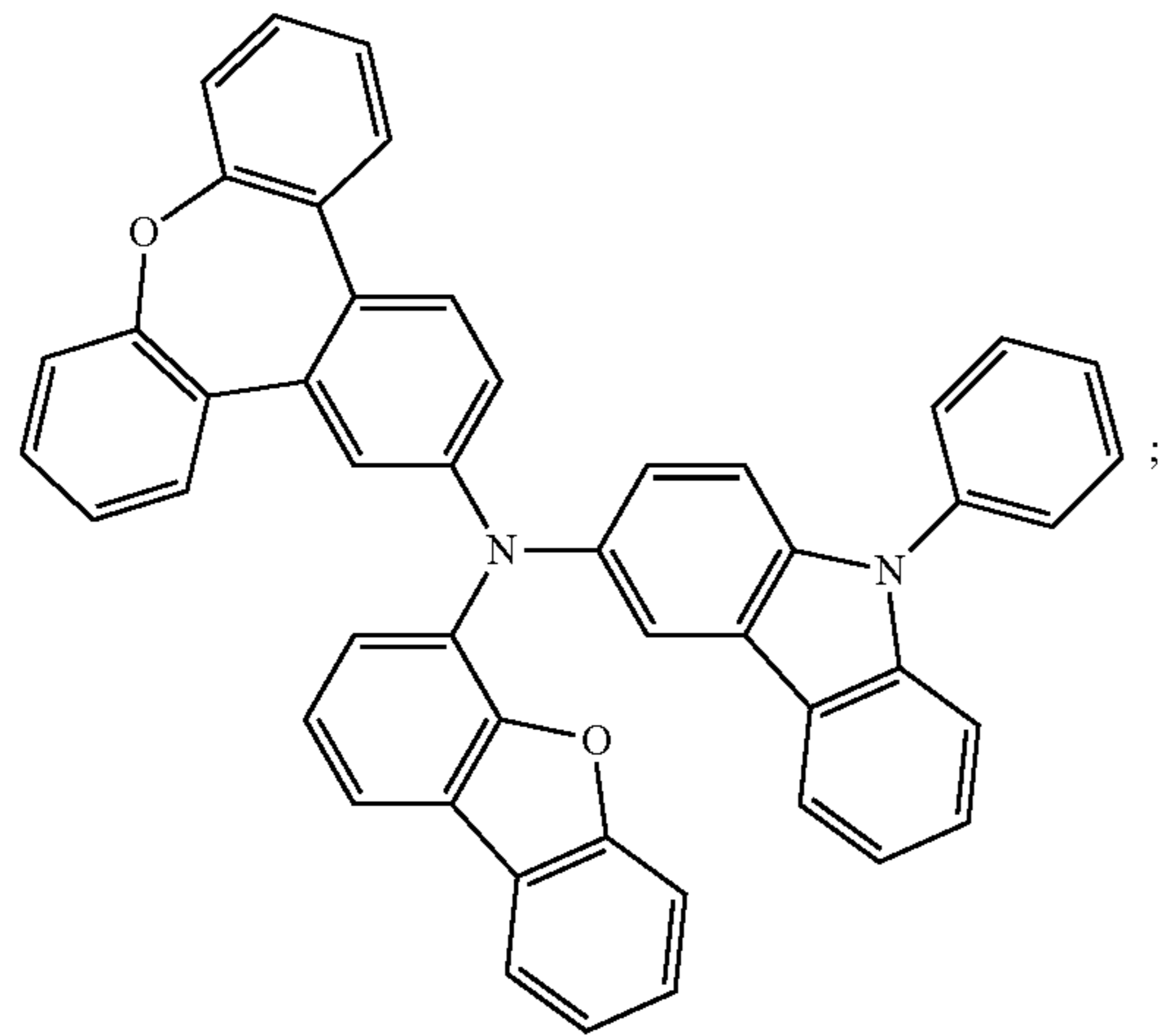
Compound 124
