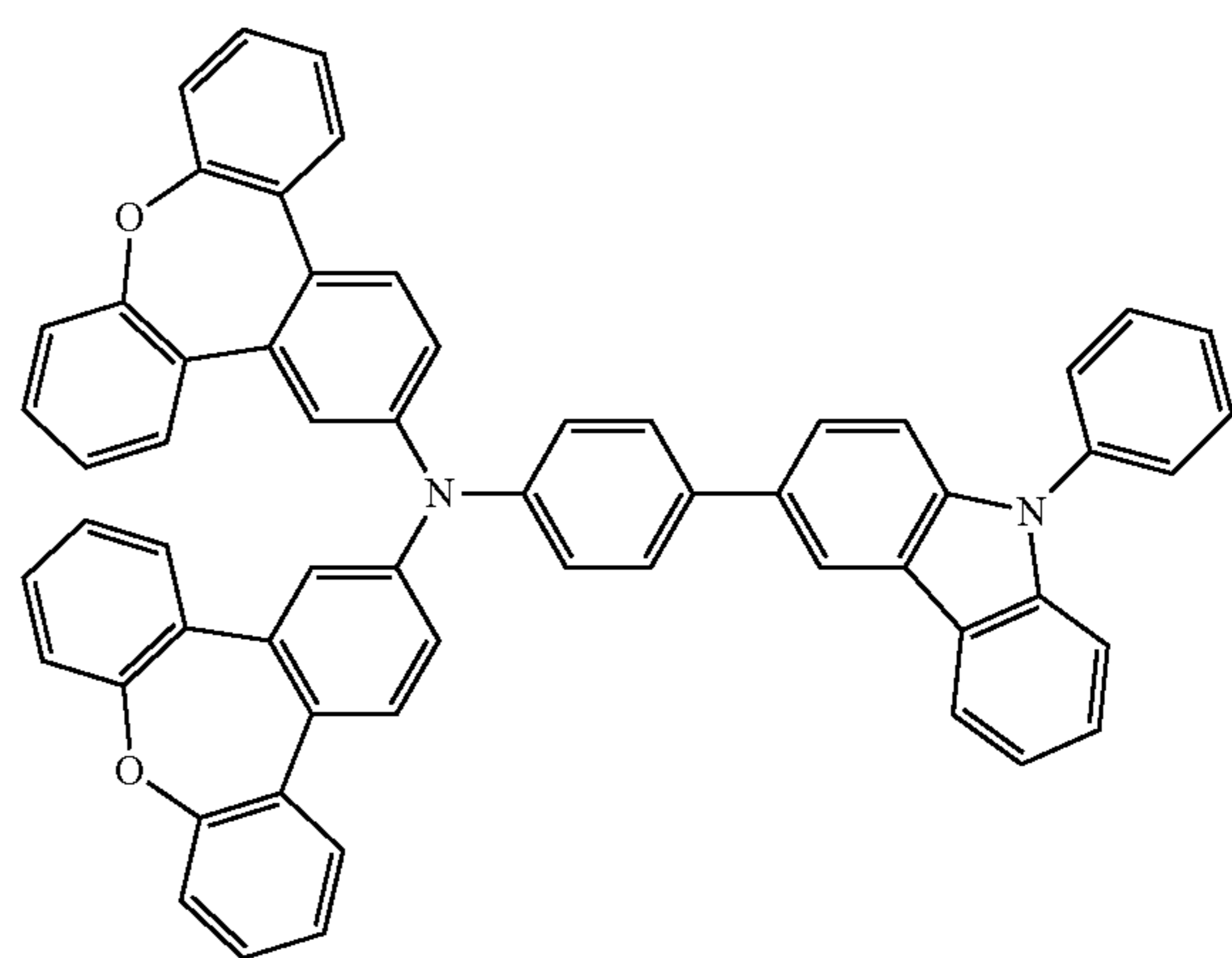
Compound 33
