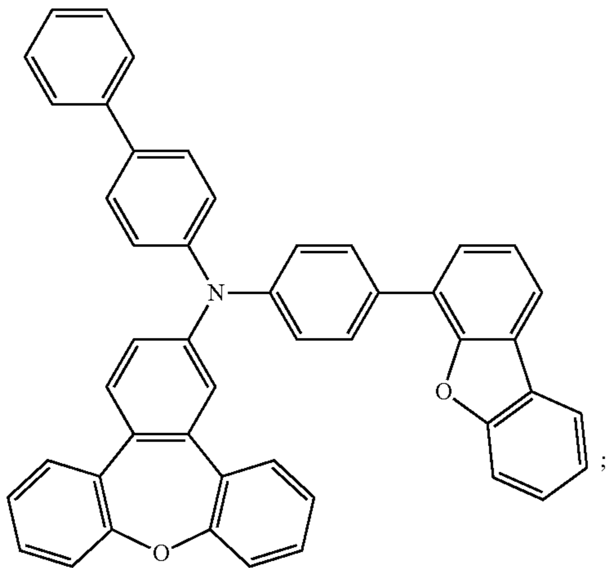
Compound 70
