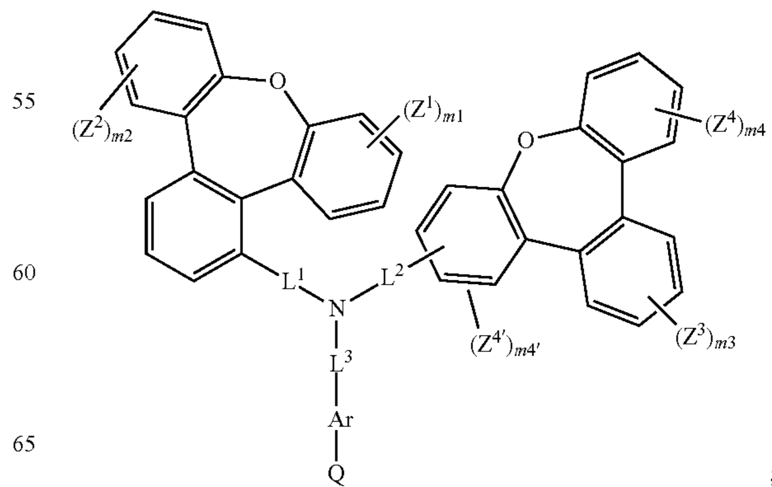
Formula (I-XV)
