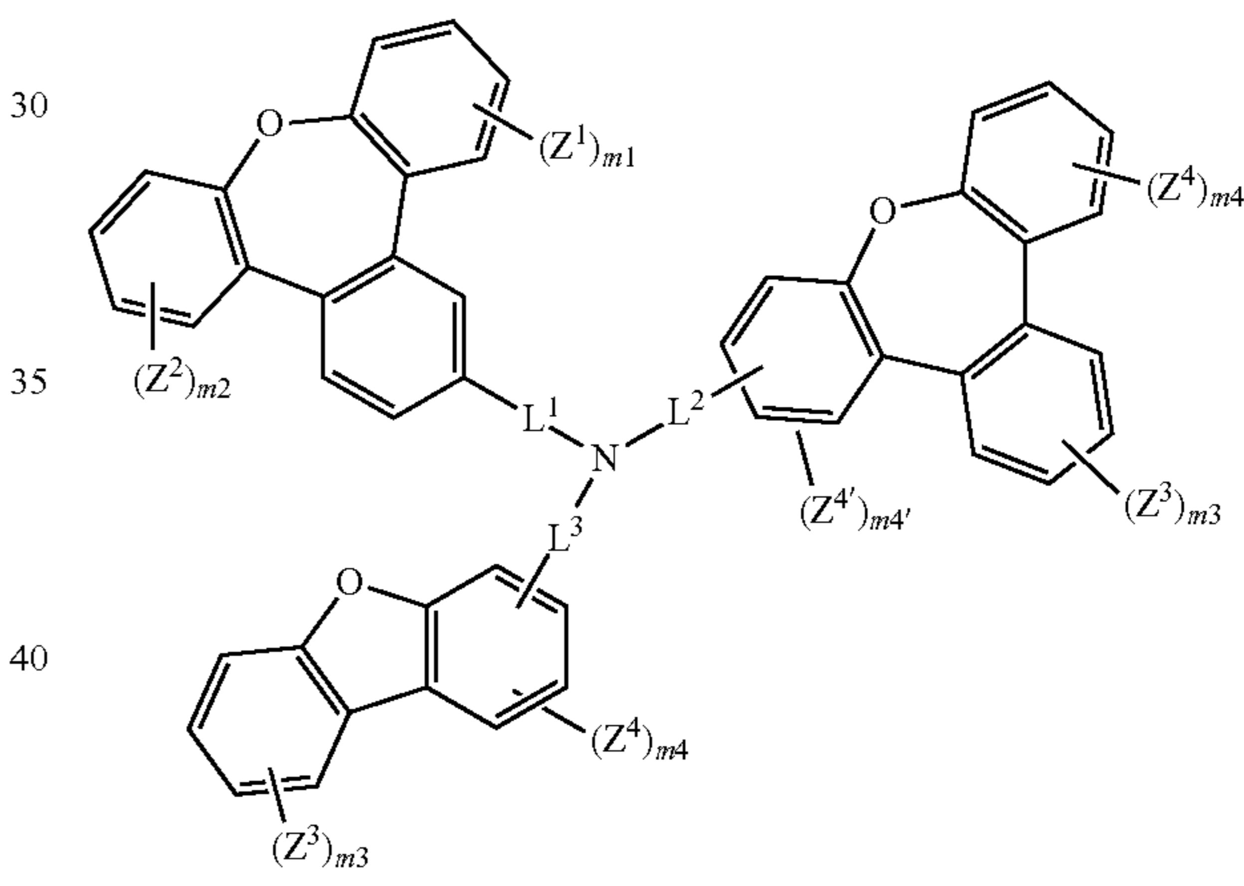
Formula (I-XX)
