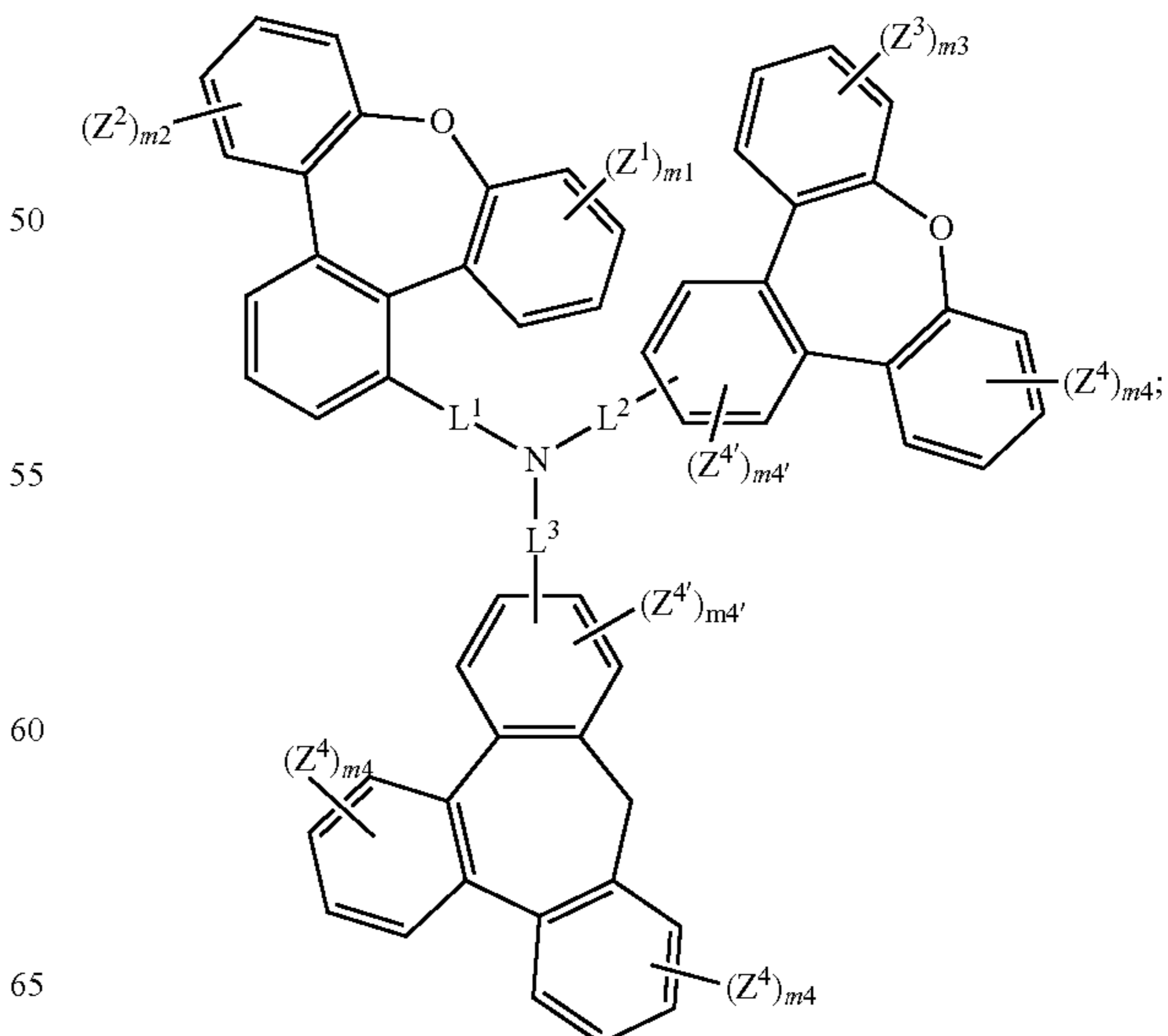
Formula (I-V)
