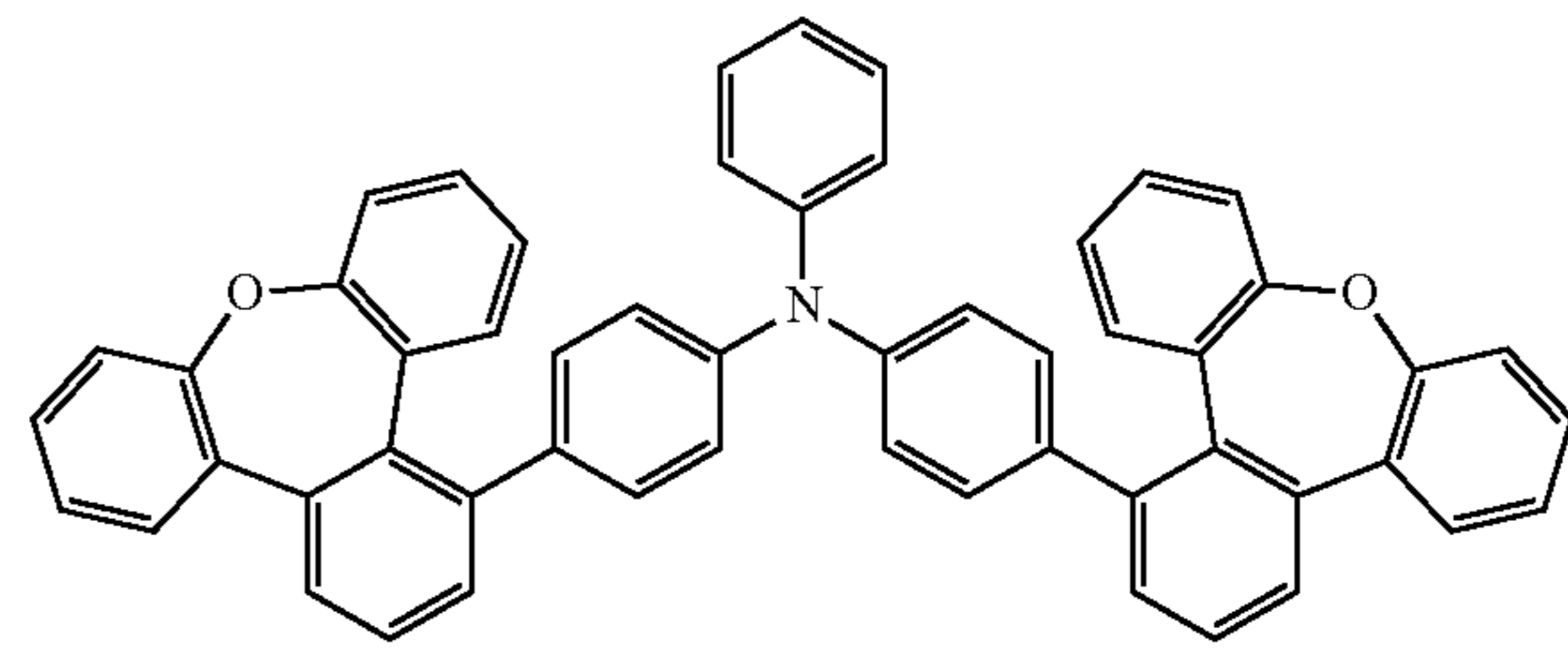
Compound 13
