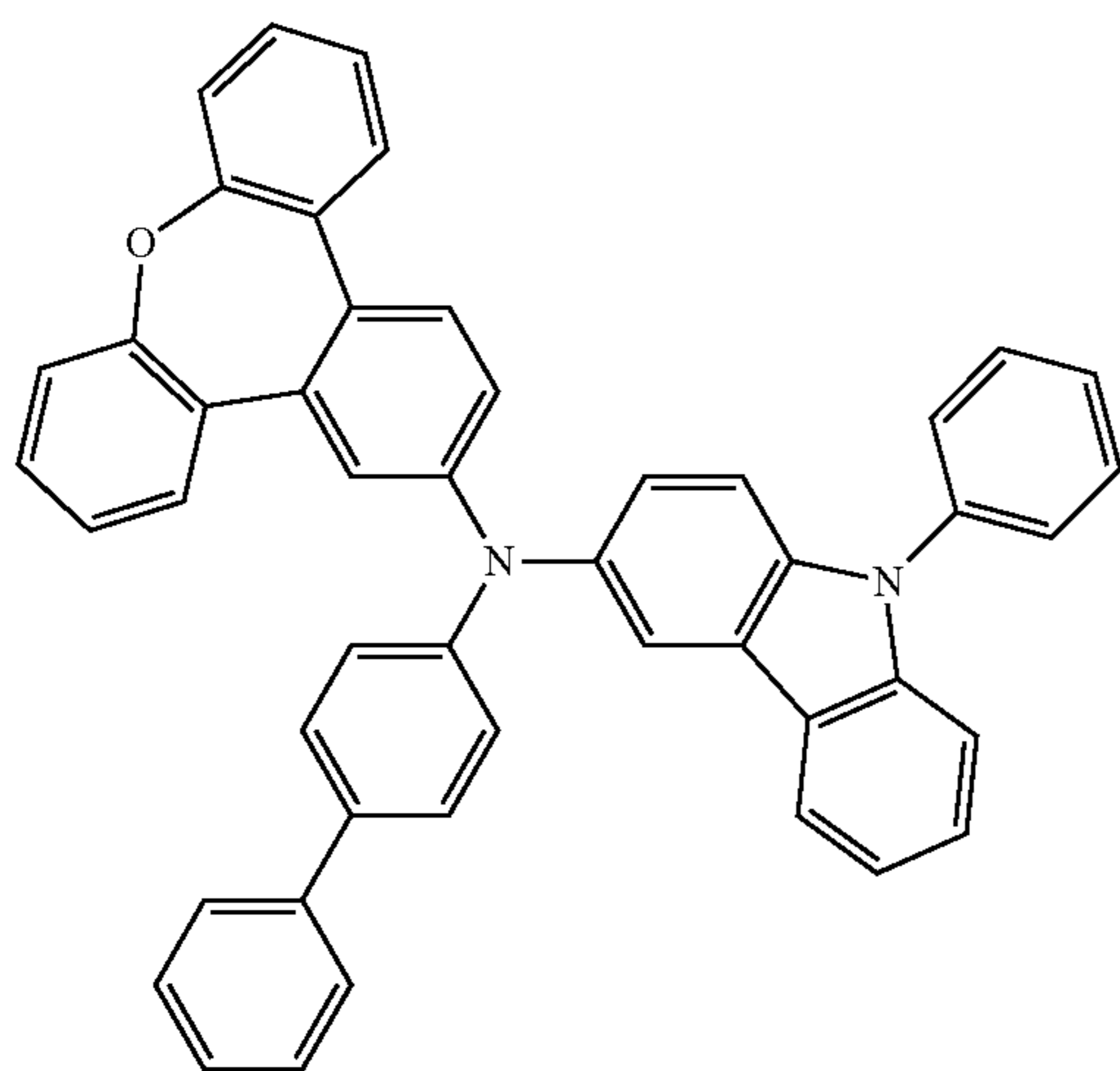
Compound 19
