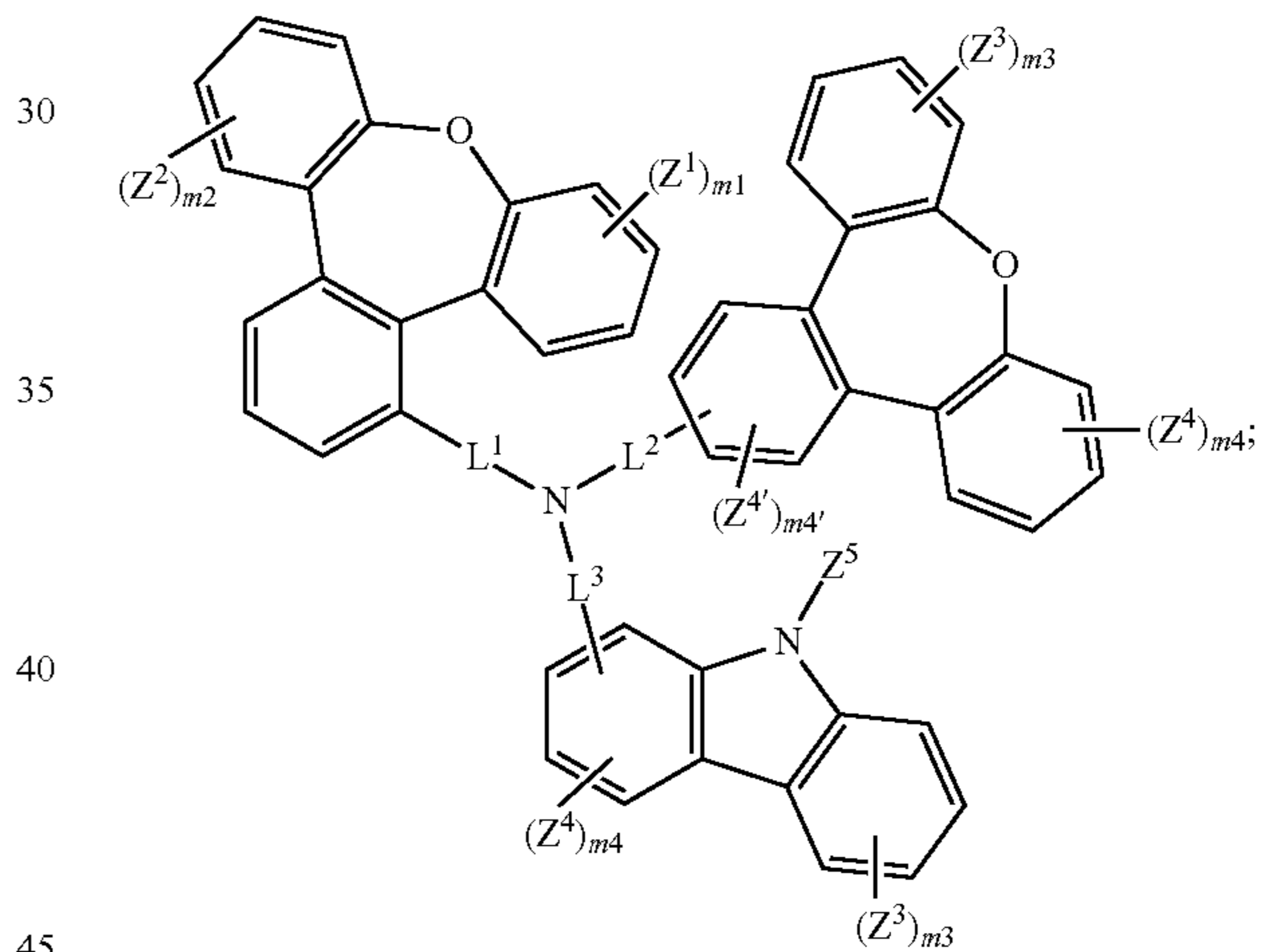
Formula (I-X)
