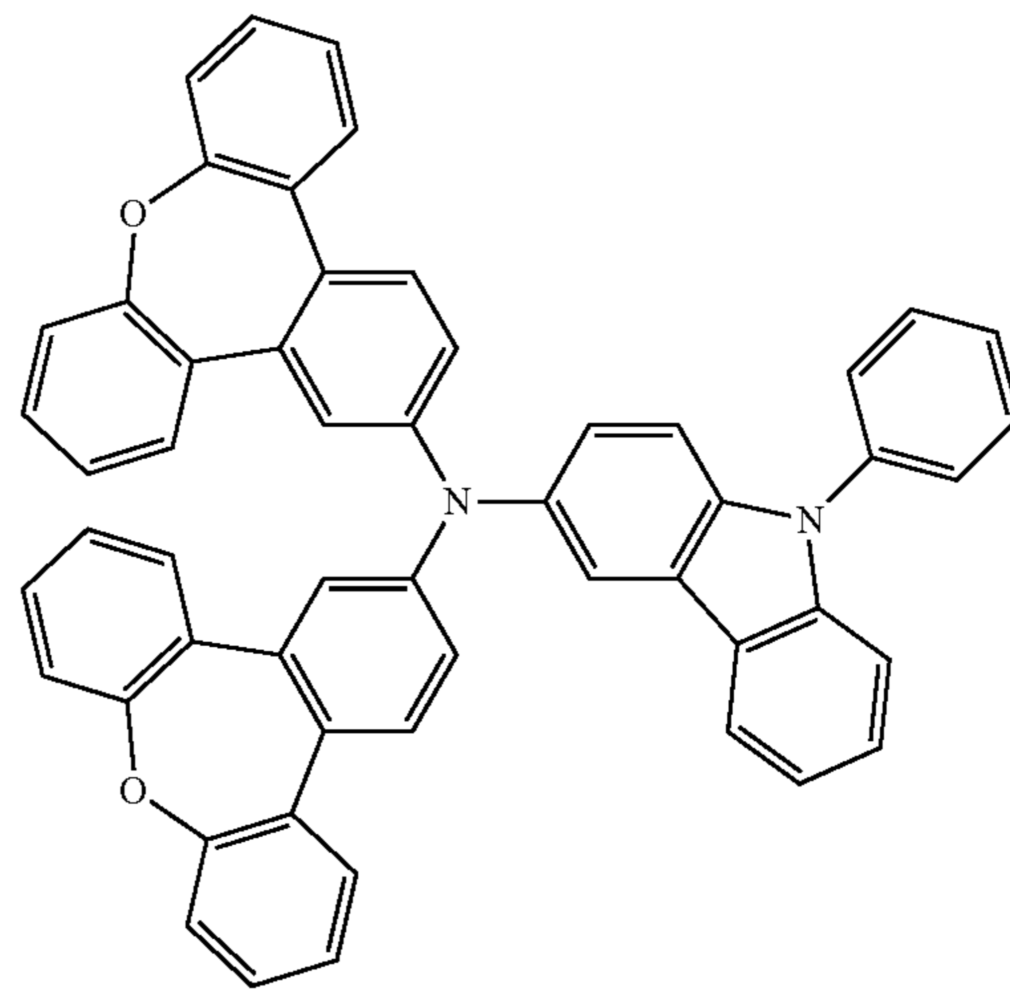
Compound 32
