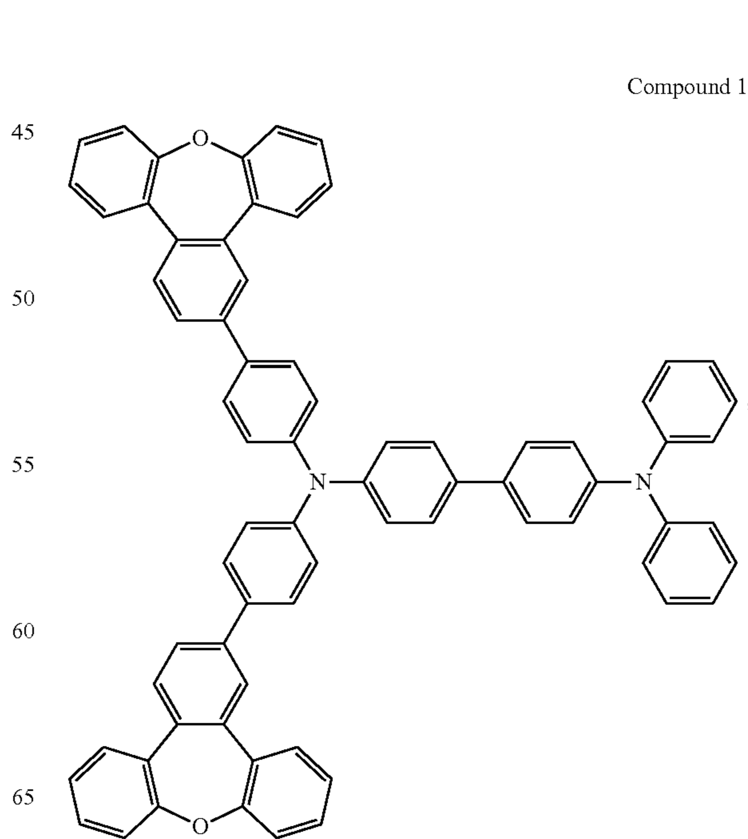
Compound 113
