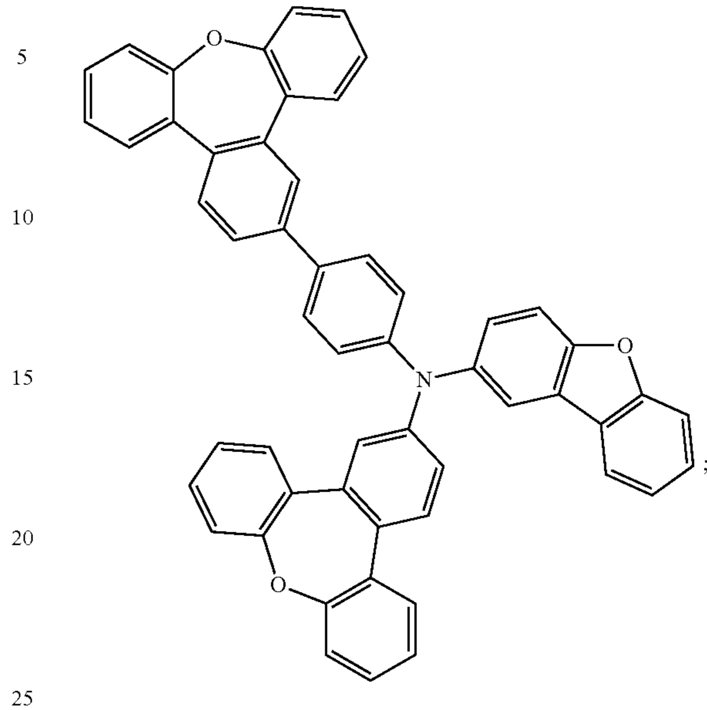
Compound 139
