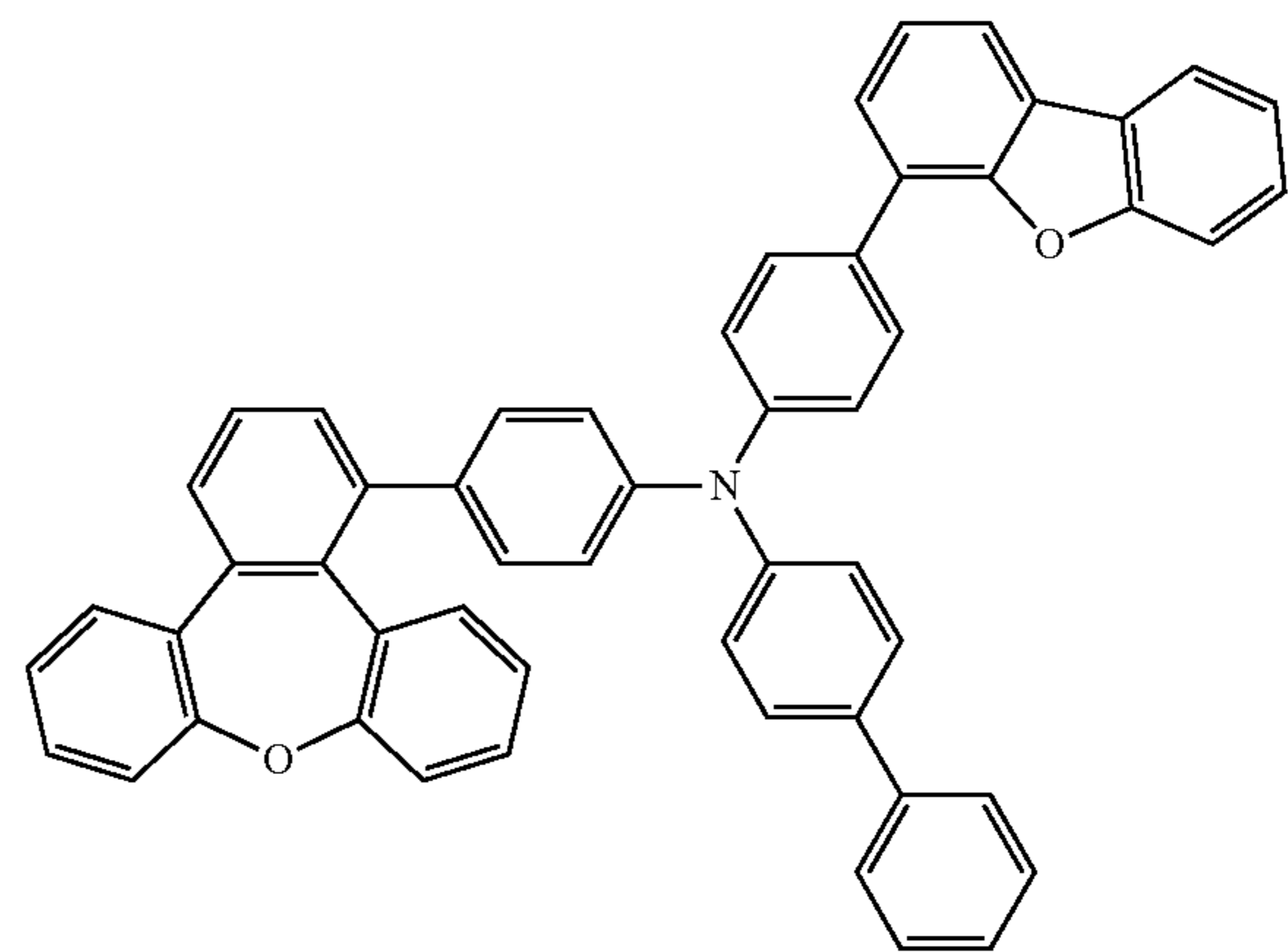
Compound 38
