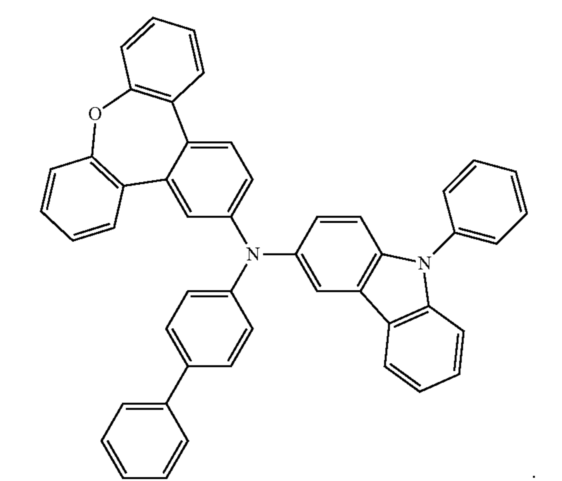
Compound 19
