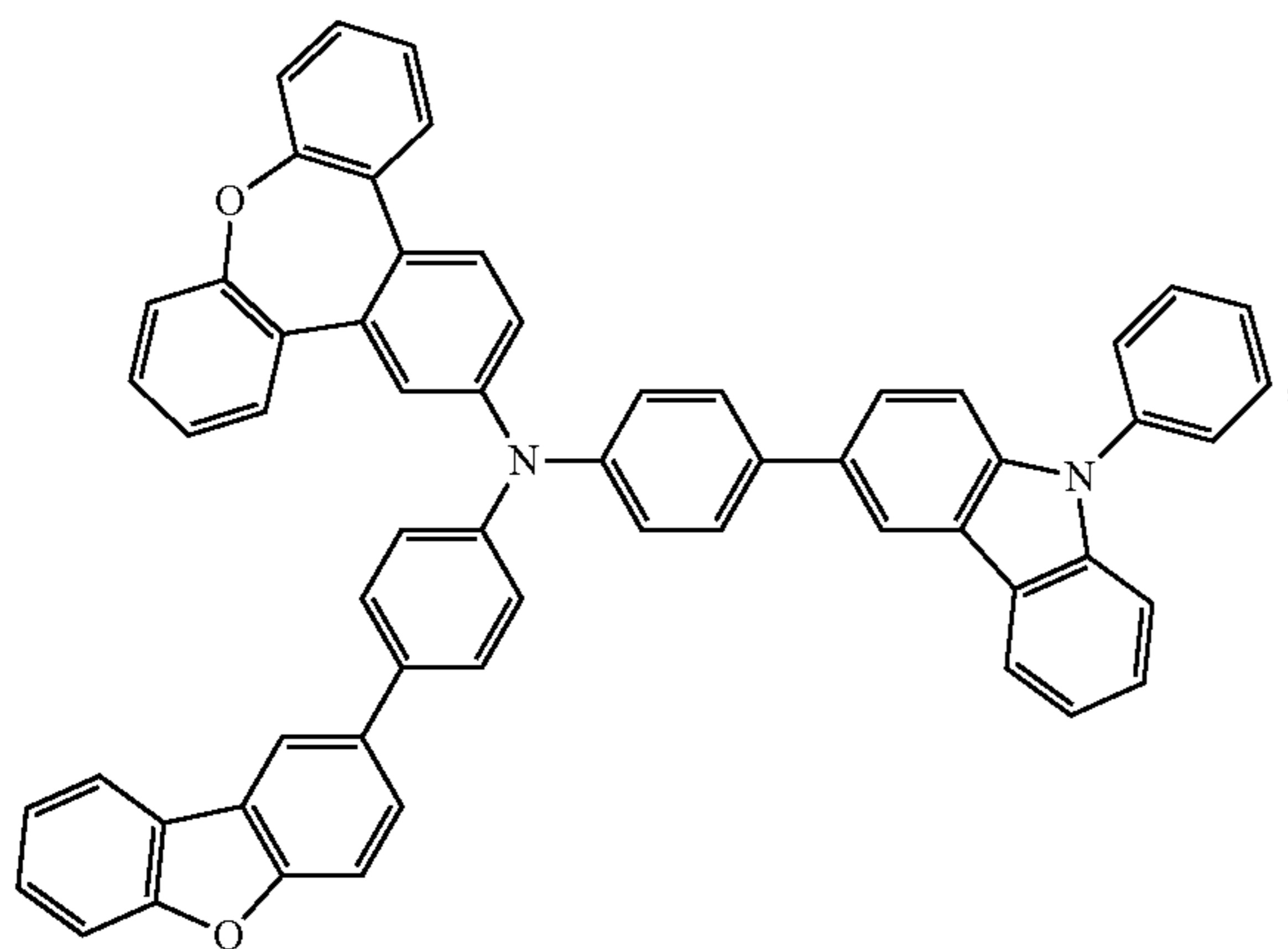
Compound 126
