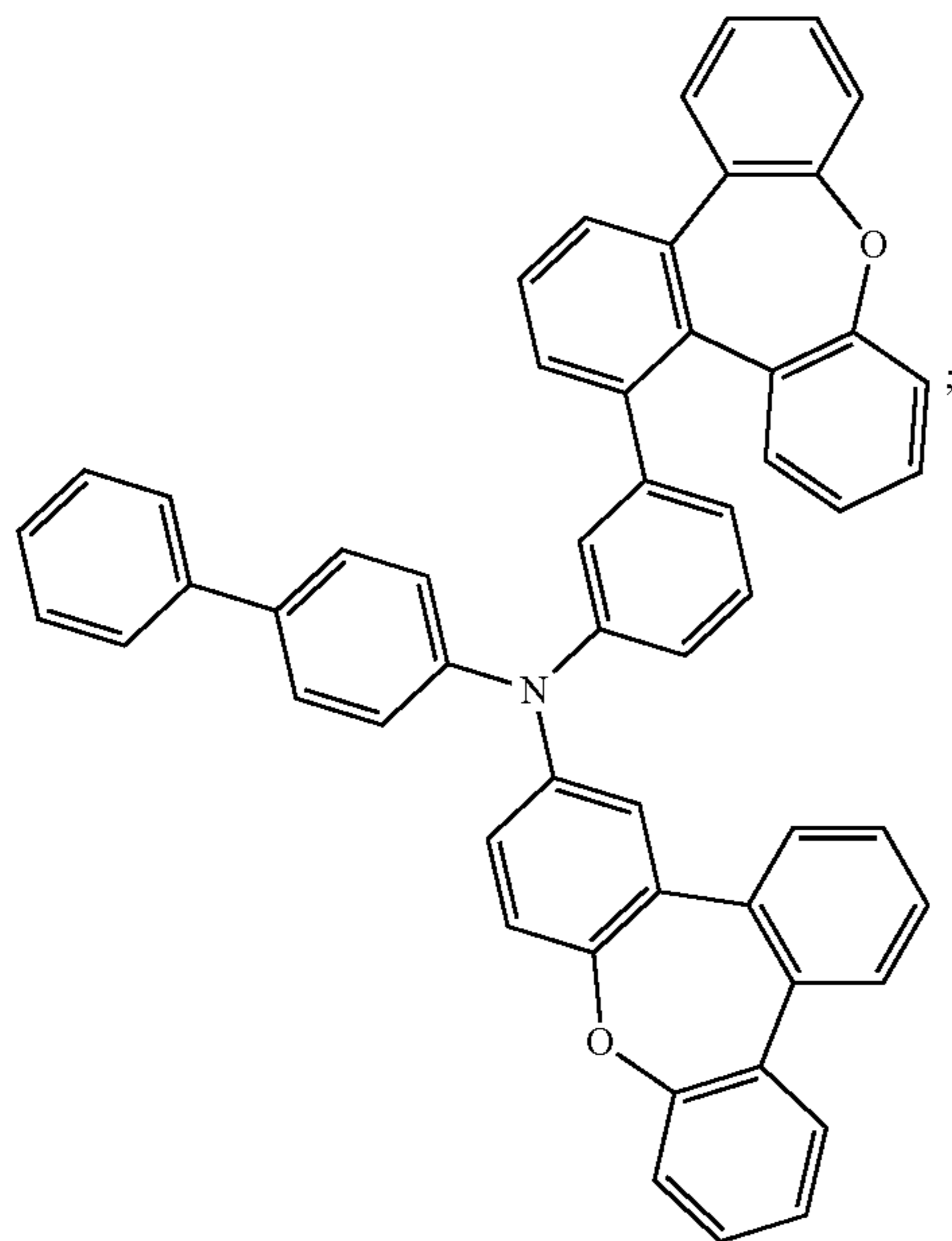
Compound 103
