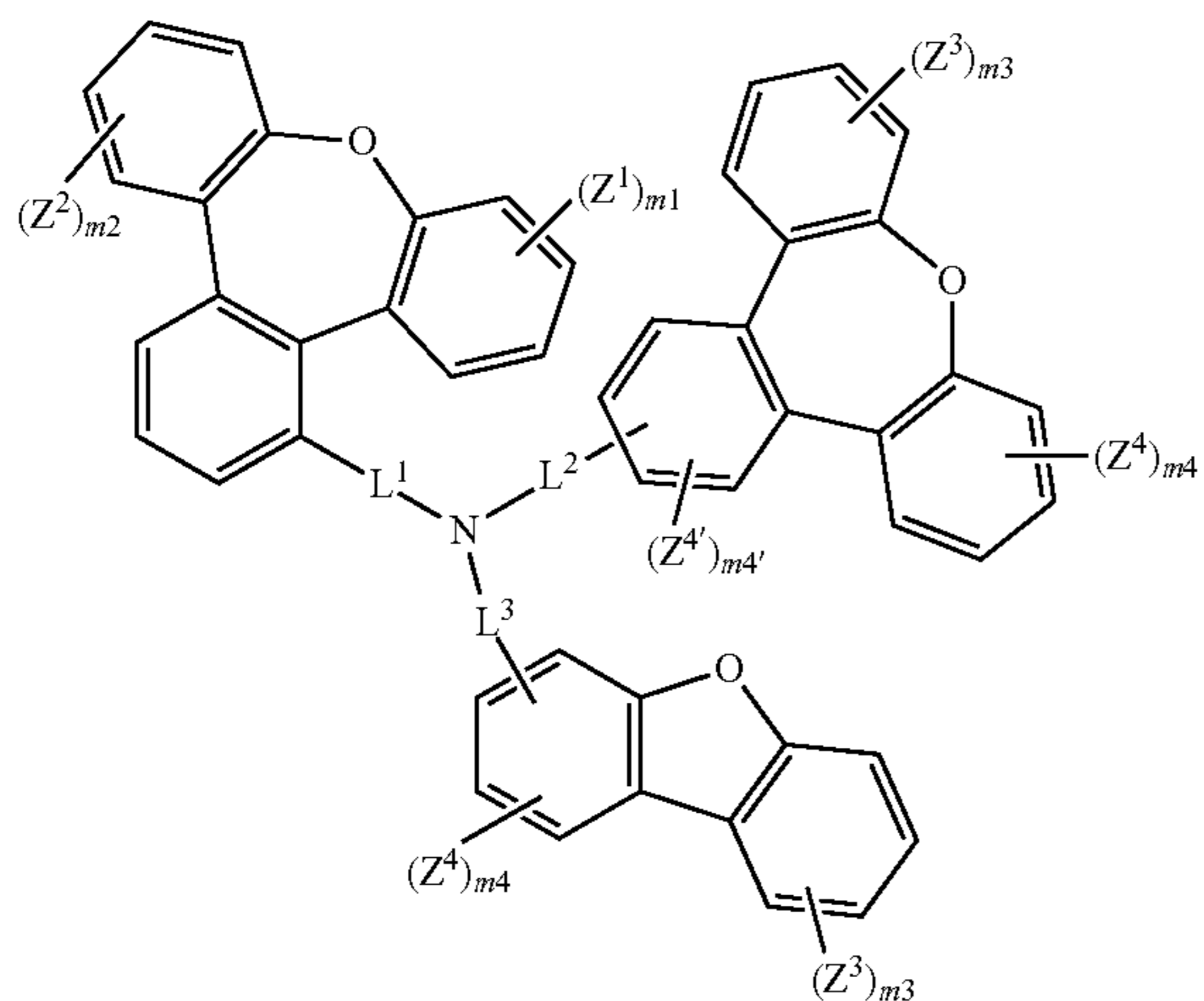
Formula (I-XI)
