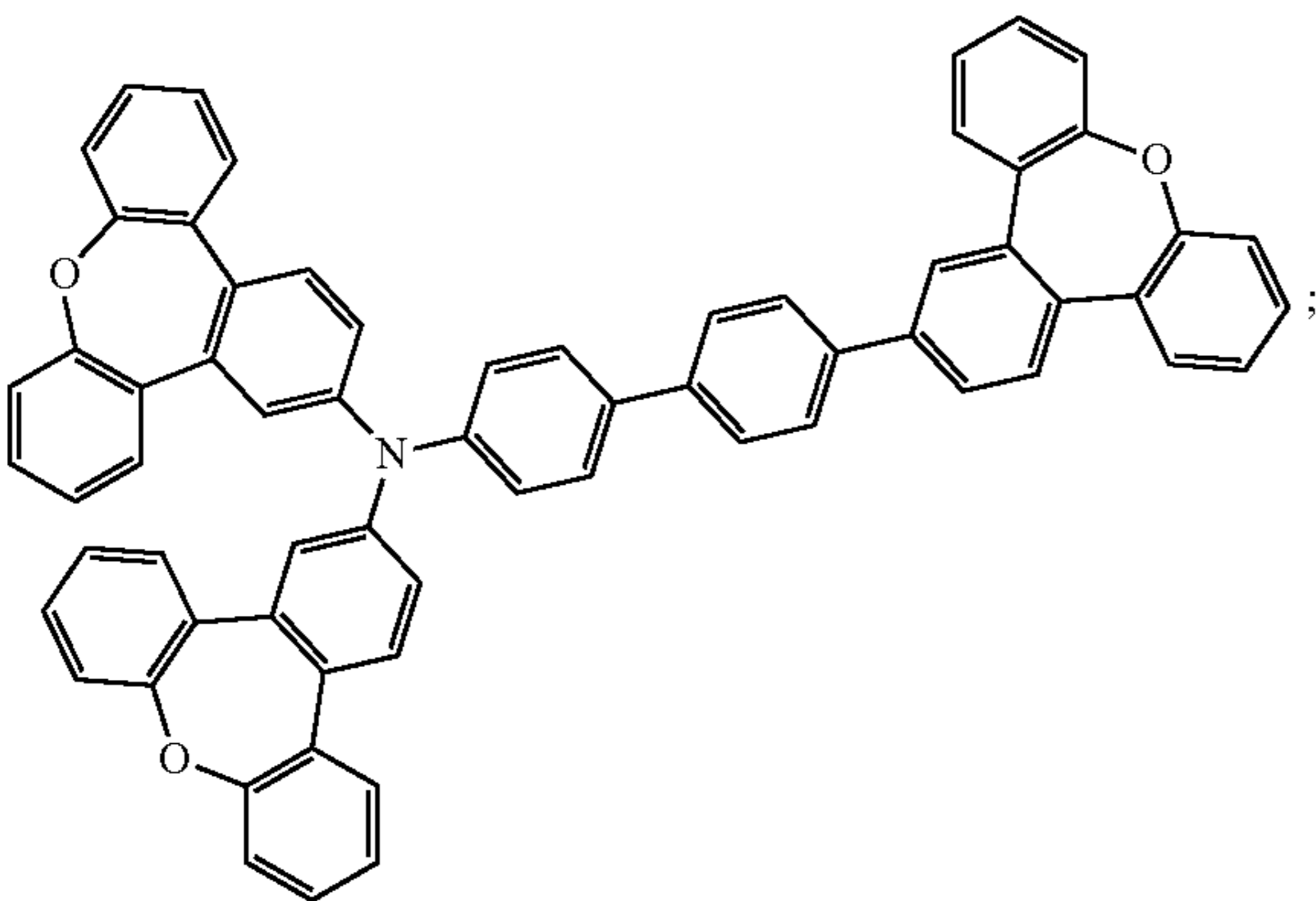
Compound 110
