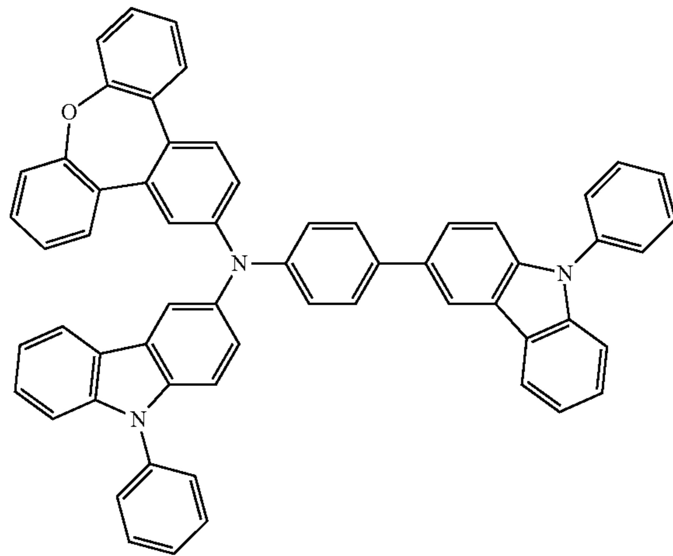
Compound 24
