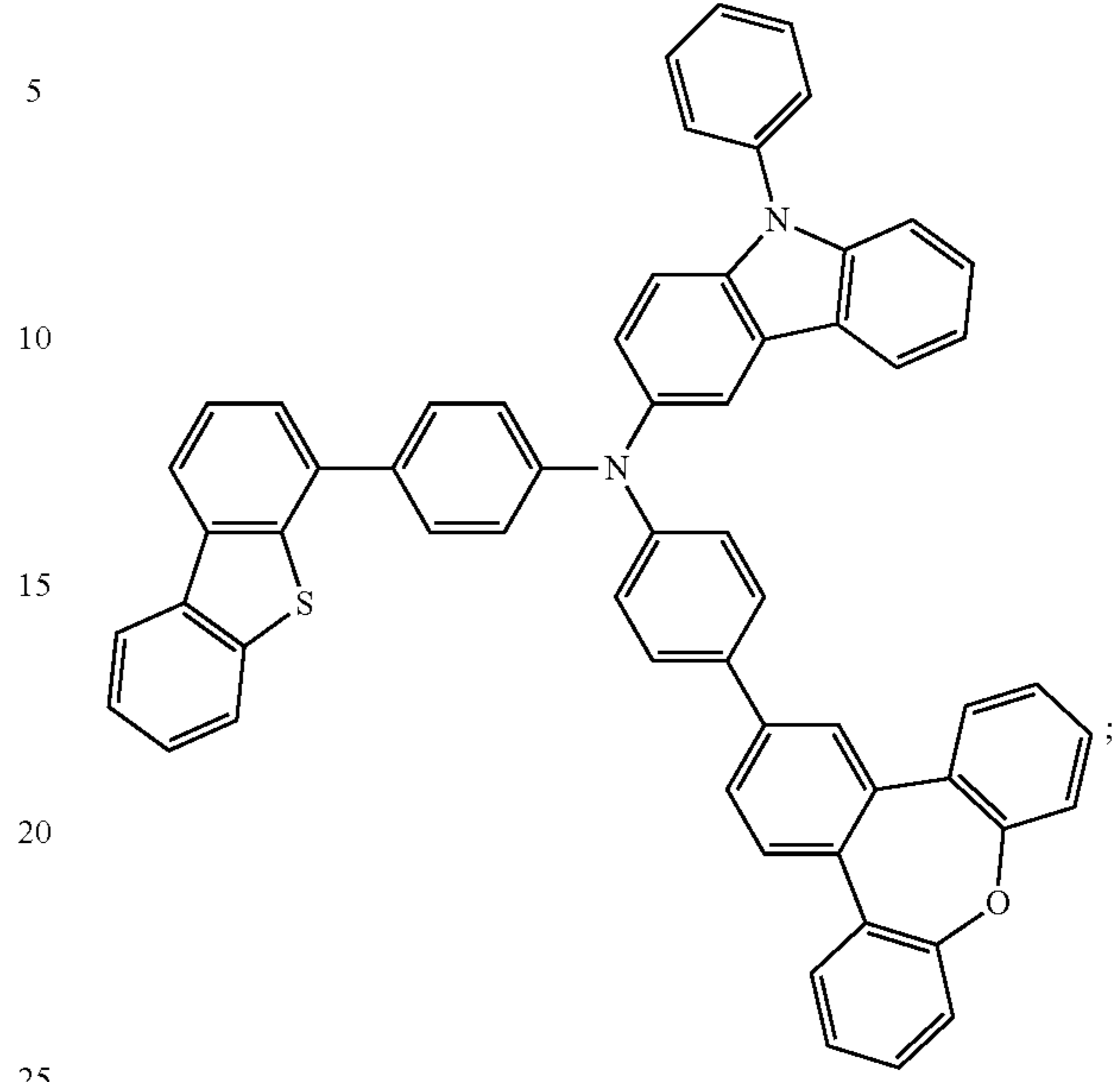
Compound 122
