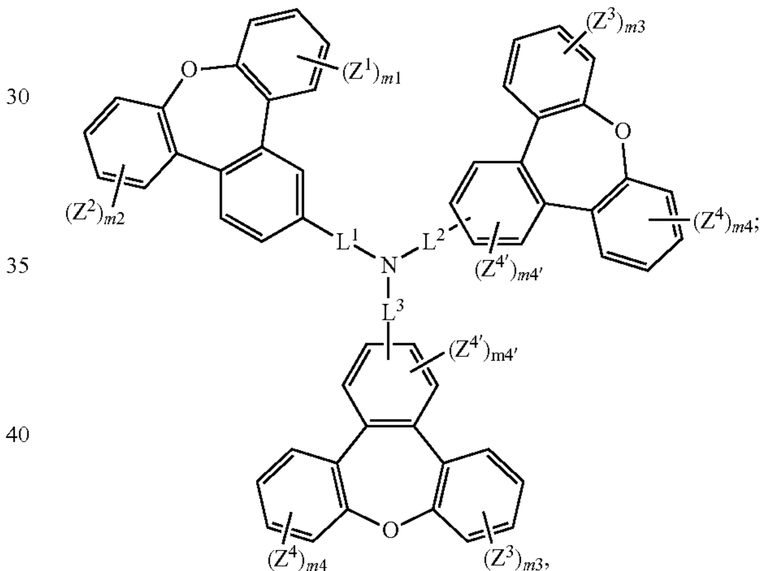
Formula (I-V)
