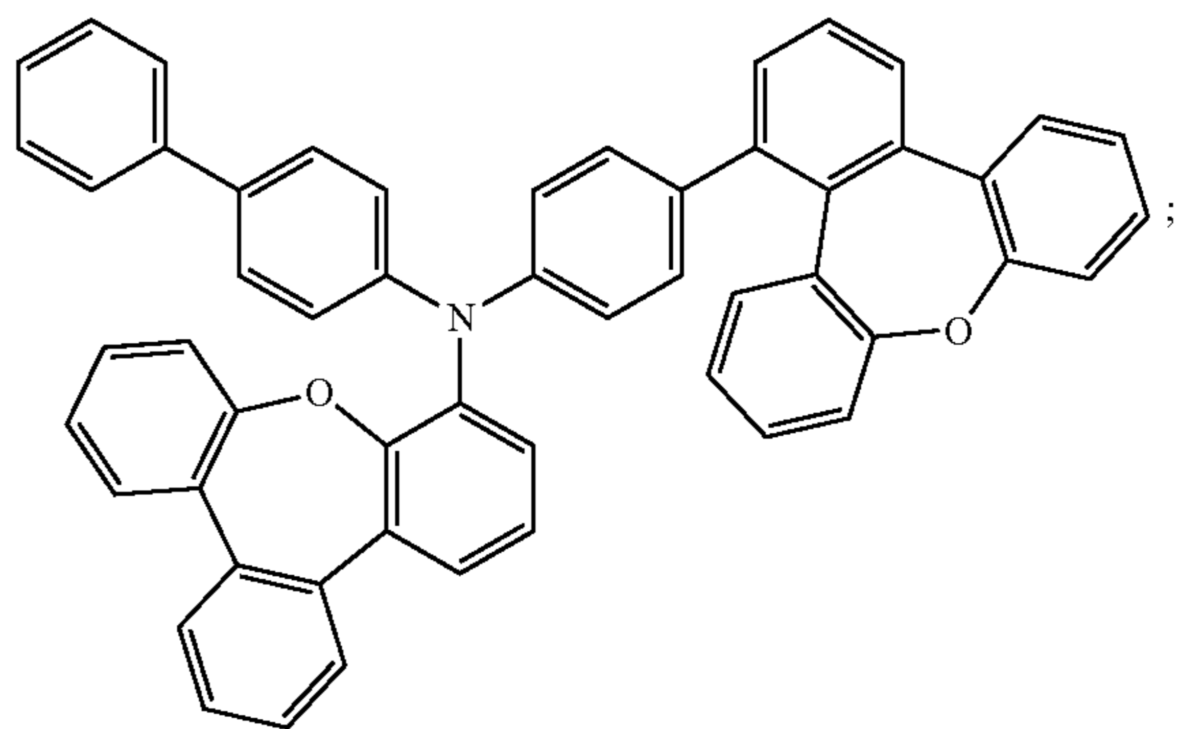
Compound 106
