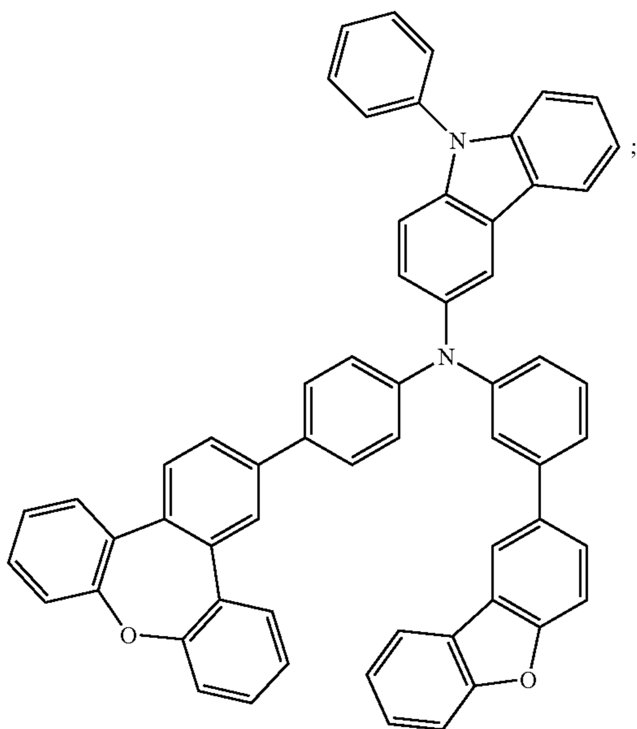
Compound 121
