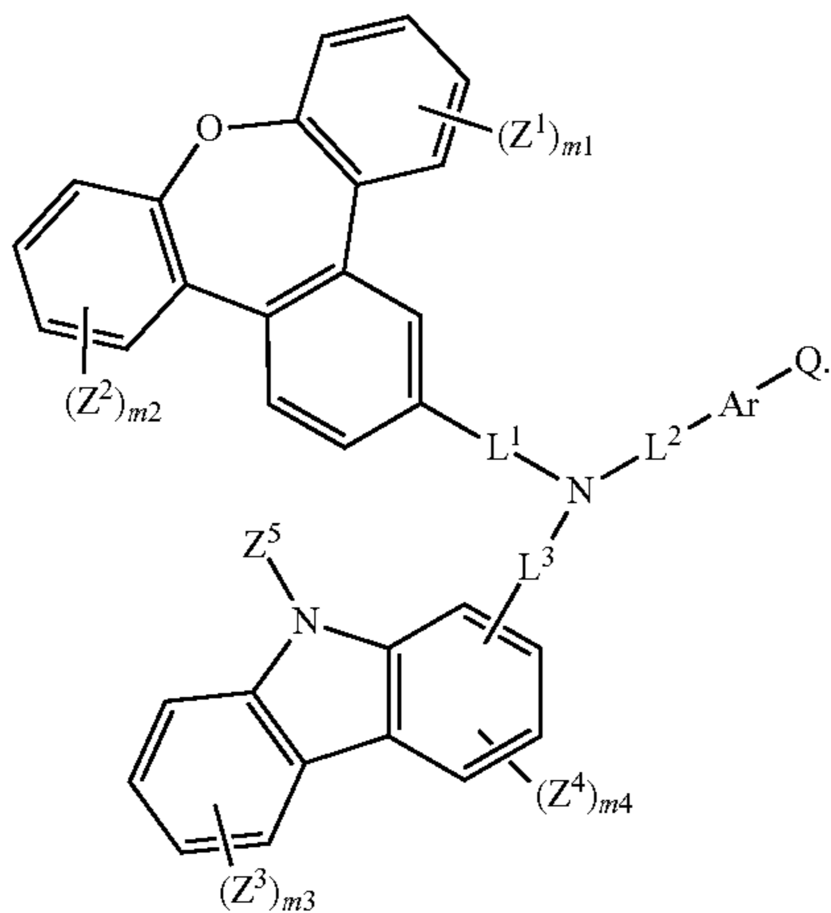
Formula (I-XXVI)
