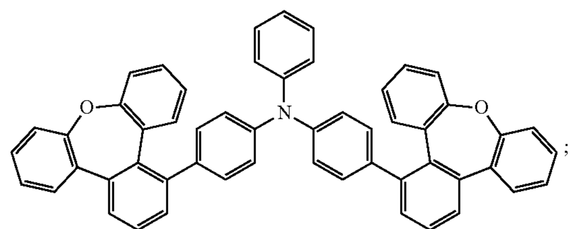
Compound 13
