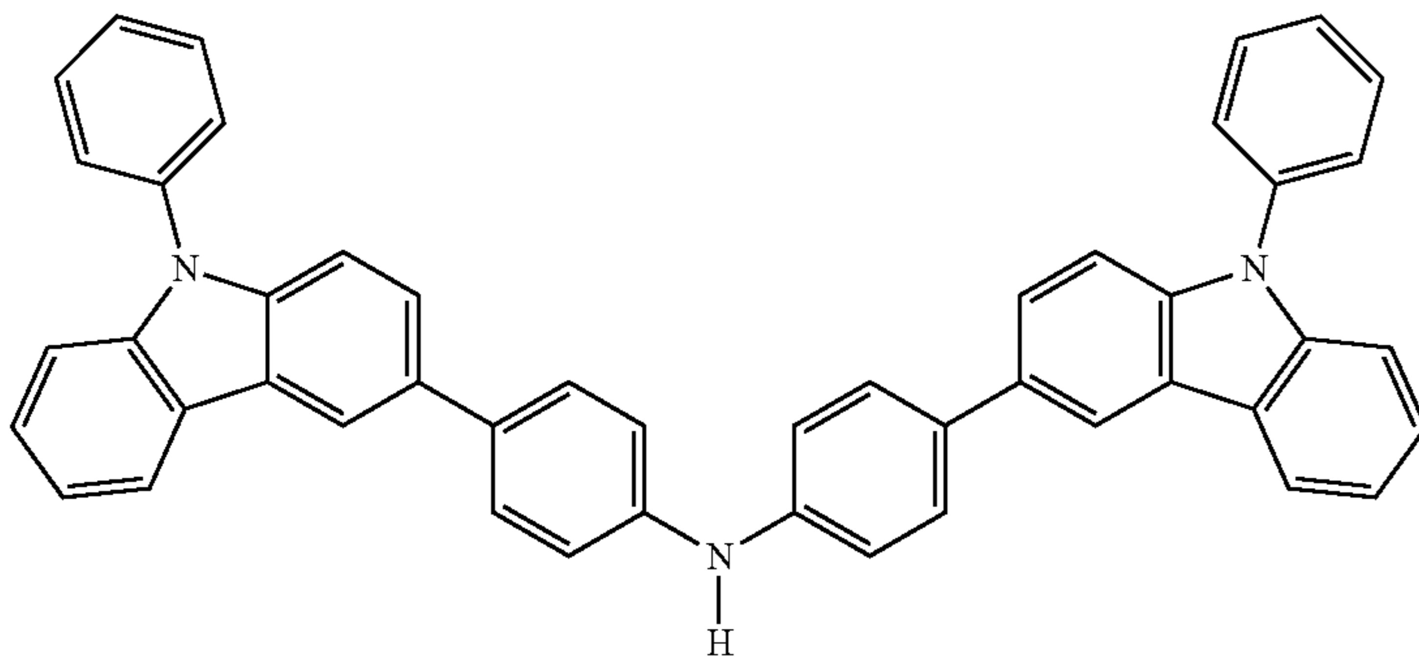
Intermediate A17
