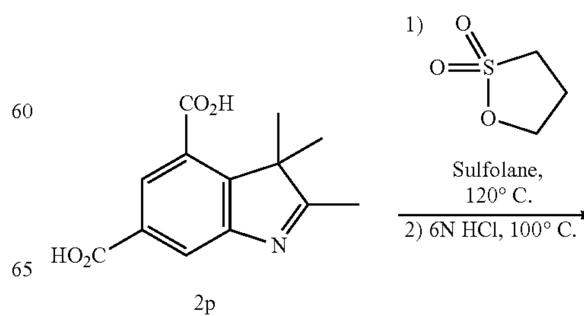
Scheme 3: Synthesis of carboxyl indolenine cyanine dyes
