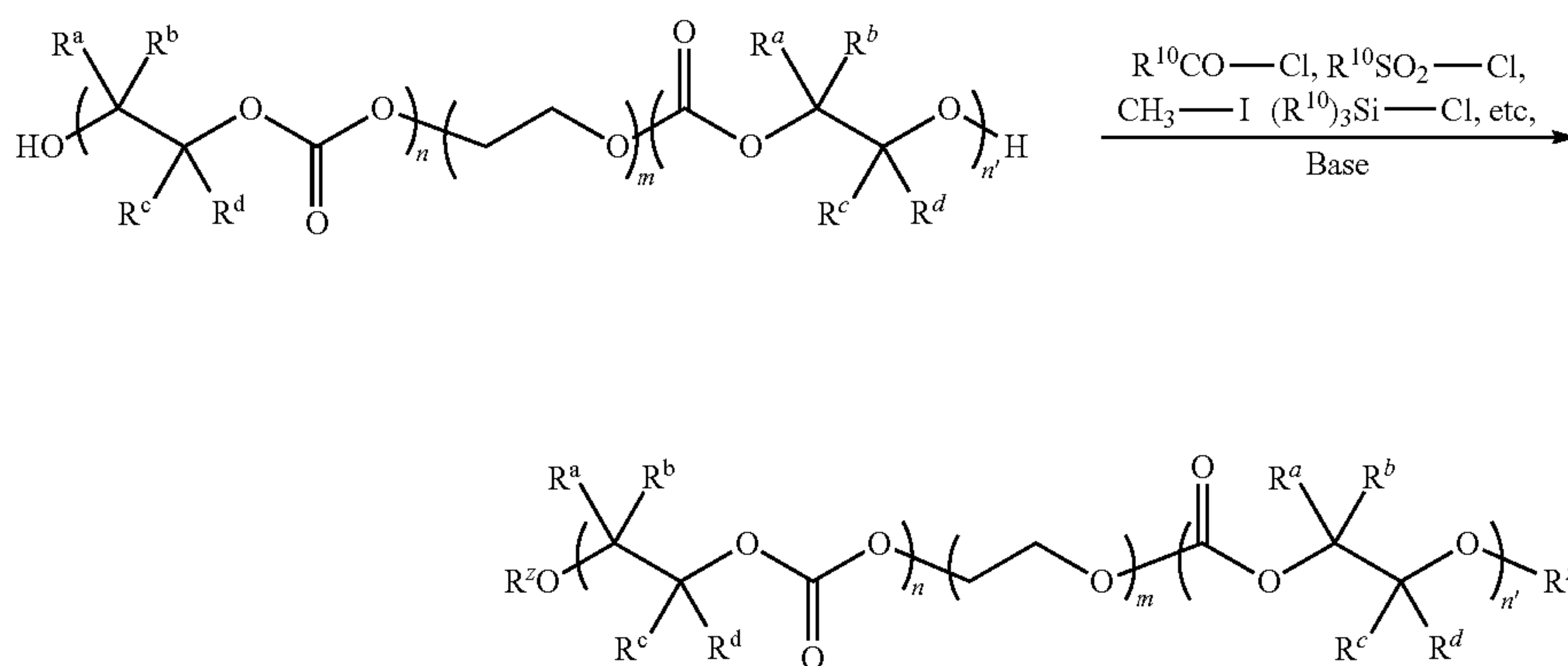
Scheme 4
