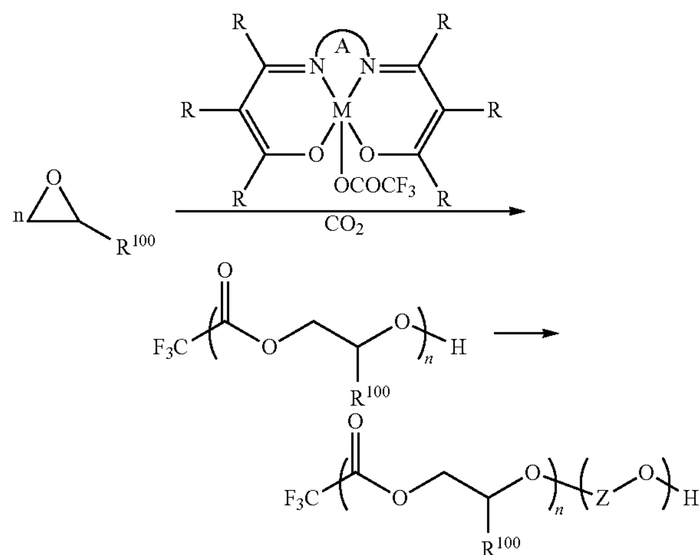
Scheme 5
