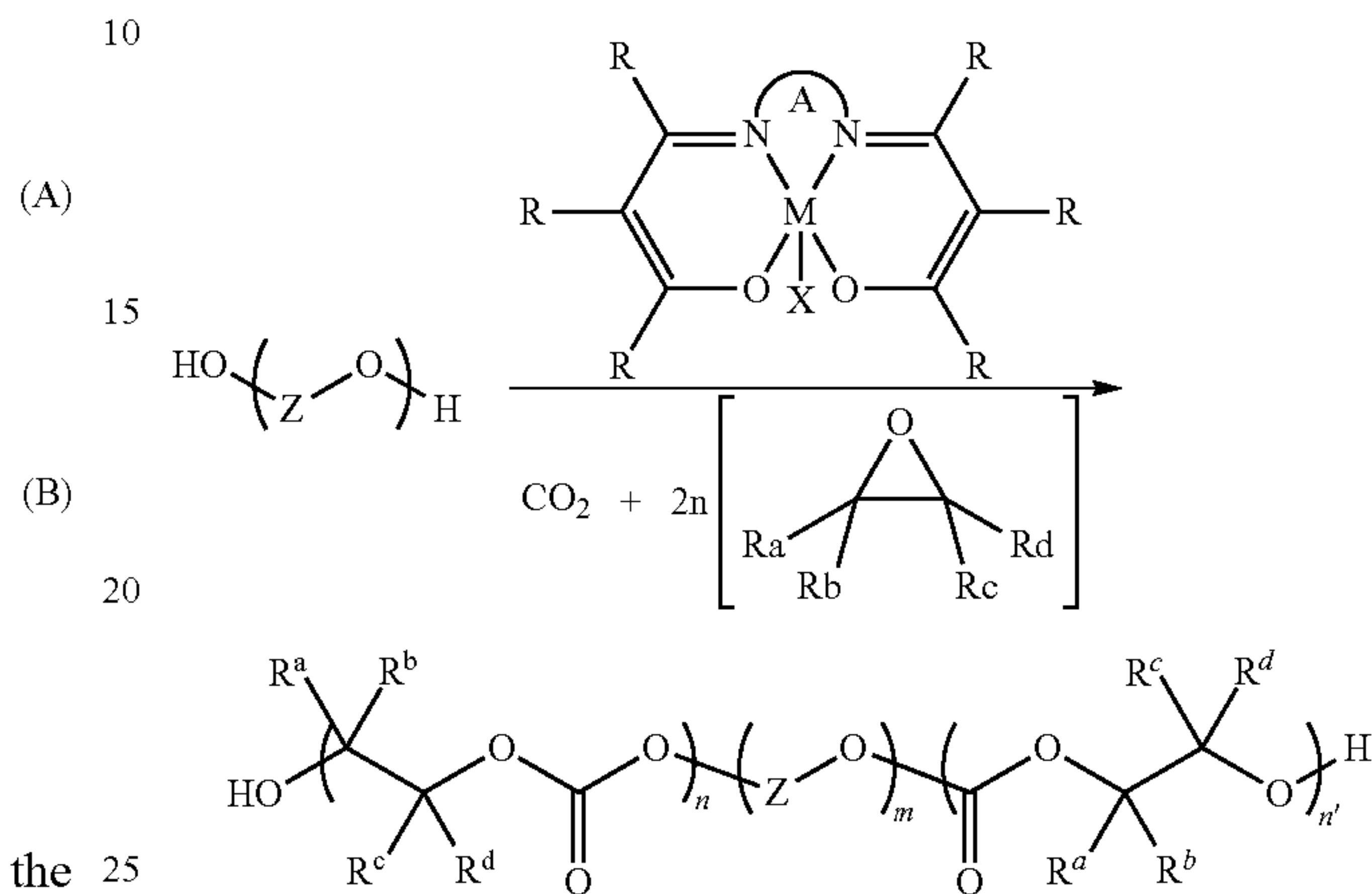
Scheme 3
