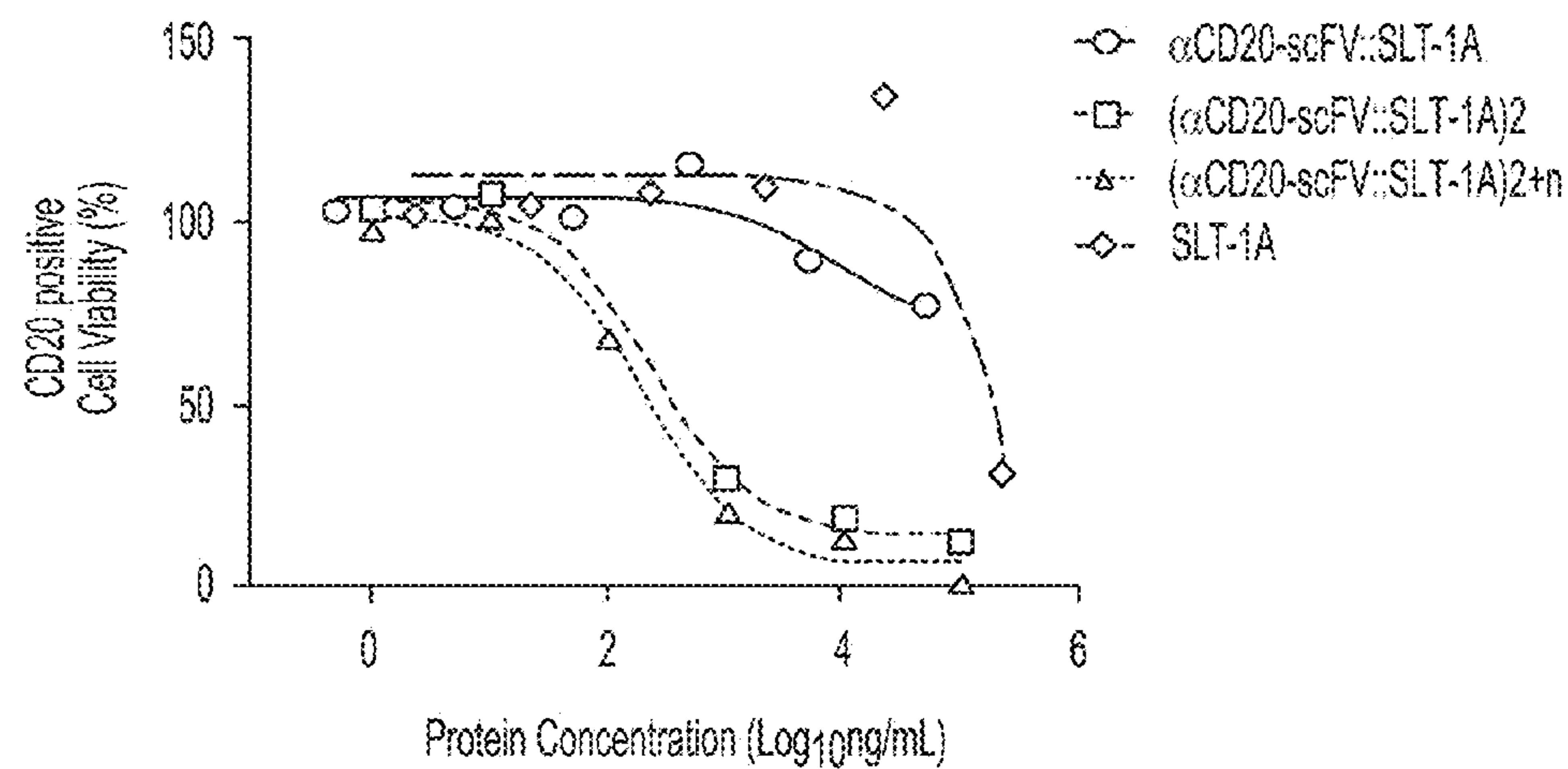
Figure 6. Cytotoxicities of Exemplary, Multivalent CD20-Binding Molecule Compositions of the Present Invention as Compared to a Monovalent CD20-Binding Protein Composition
