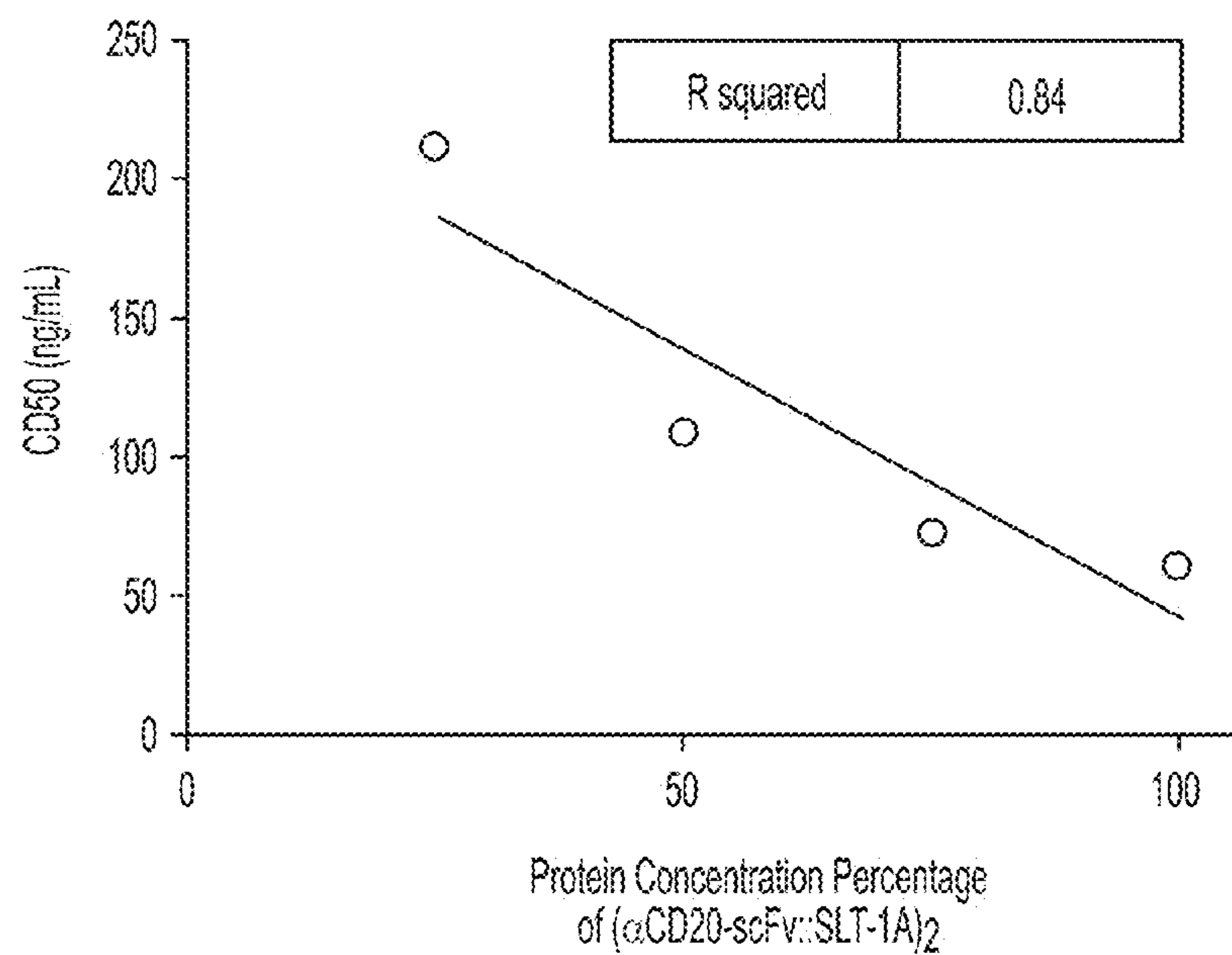
Figure 10. Cytotoxicities of Fixed-Ratio Mixtures of the Monovalent \alpha CD20-scFv::SLT-1A Composition with the Multivalent (\alpha CD20-scFv::SLT-1A) 2 Composition
