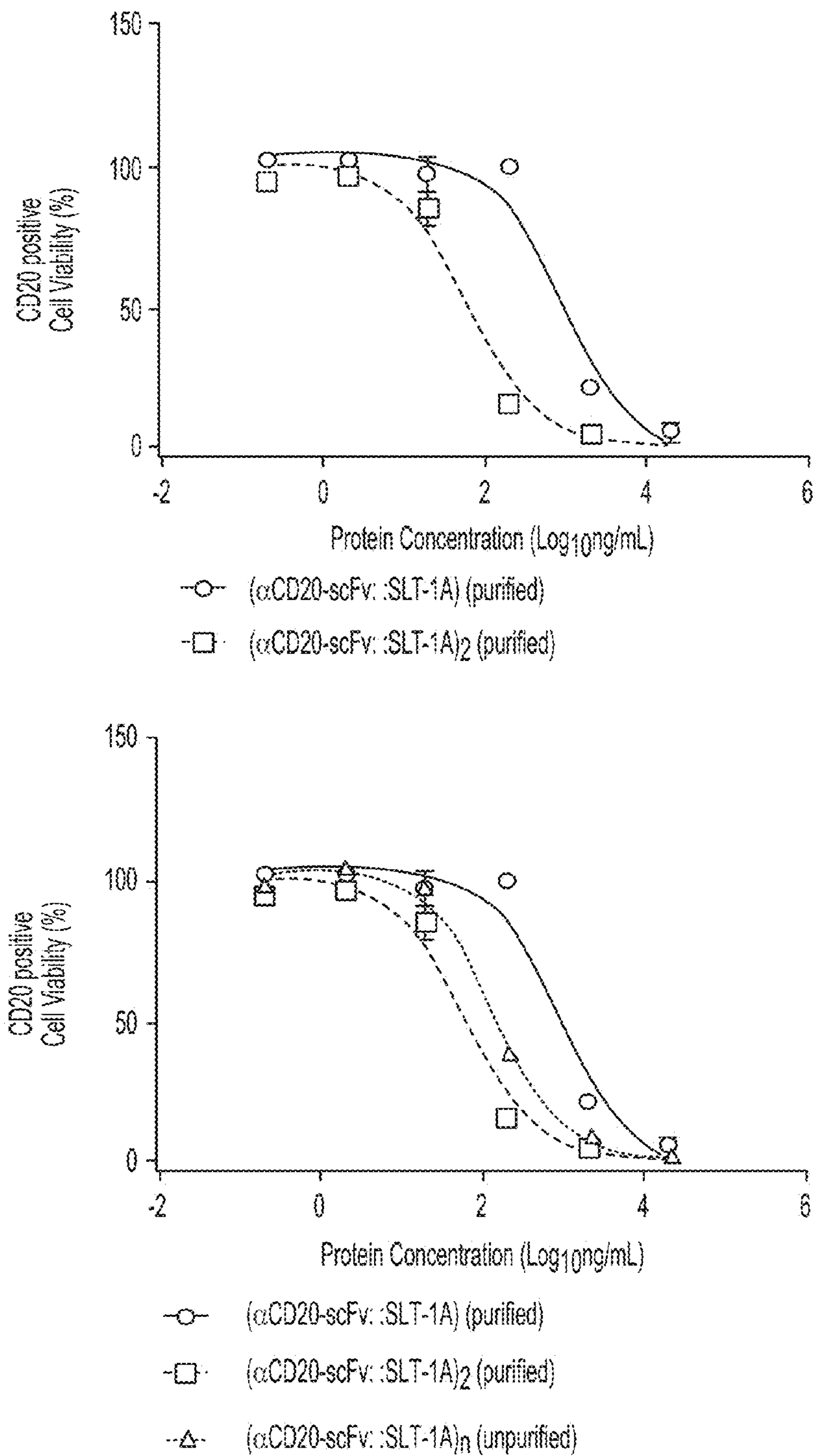
Figure 7. Cytotoxicity of an Exemplary, Multivalent CD20-Binding Molecule Composition of the Present Invention as Compared to Monovalent CD20-Binding Protein Compositions
