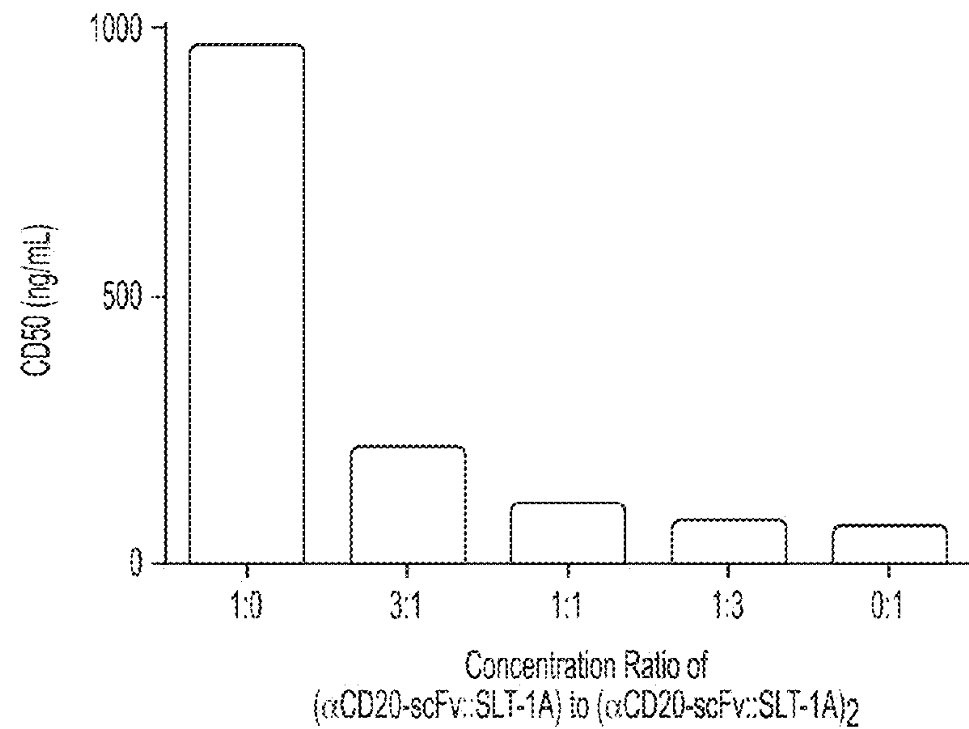
Figure 11. Cytotoxicities of Fixed-Ratio Mixtures of the Monovalent \alpha CD20-scFv::SLT-1A Composition with the Multivalent (\alpha CD20-scFv::SLT-1A) 2 Composition
