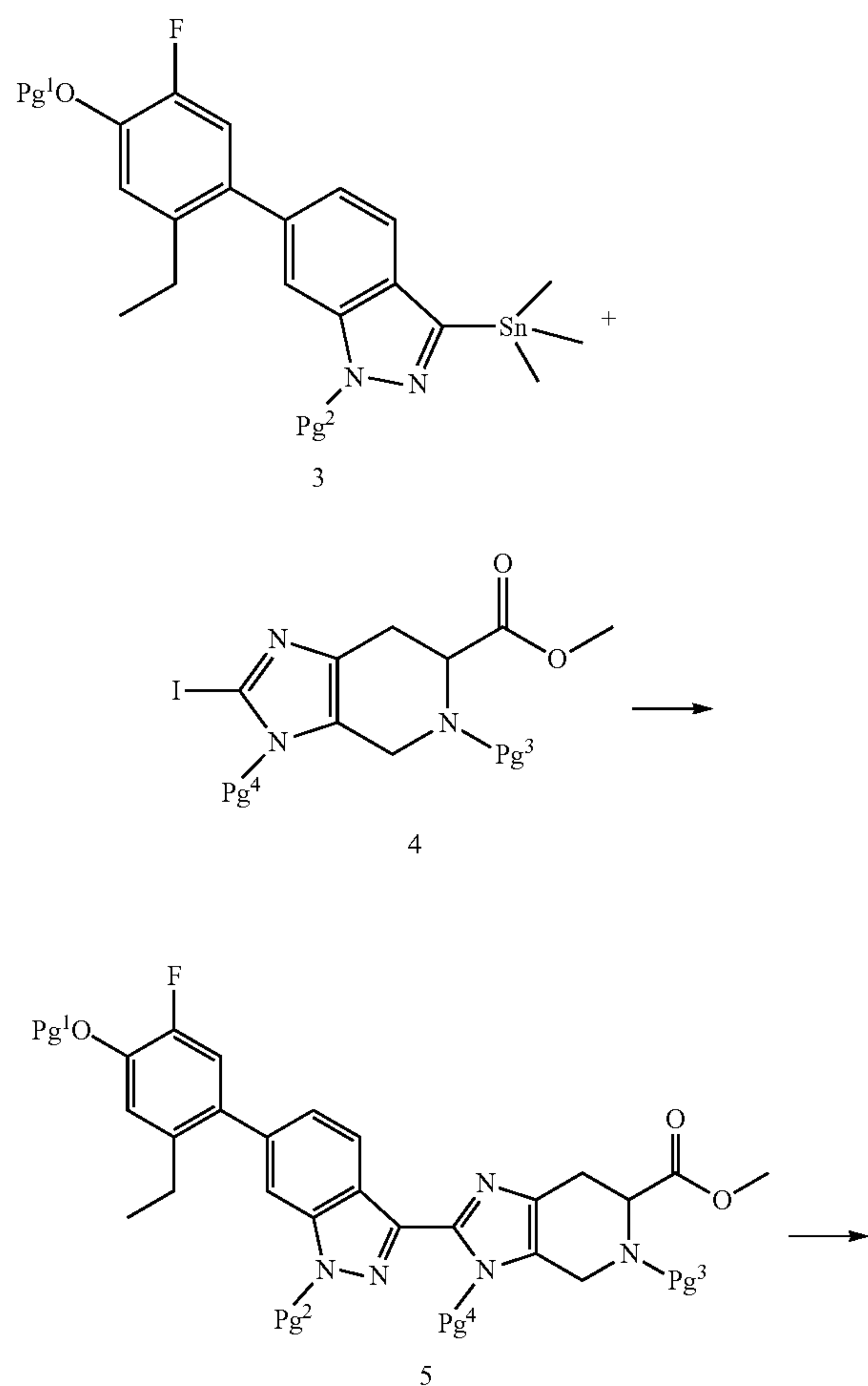
Scheme 2
