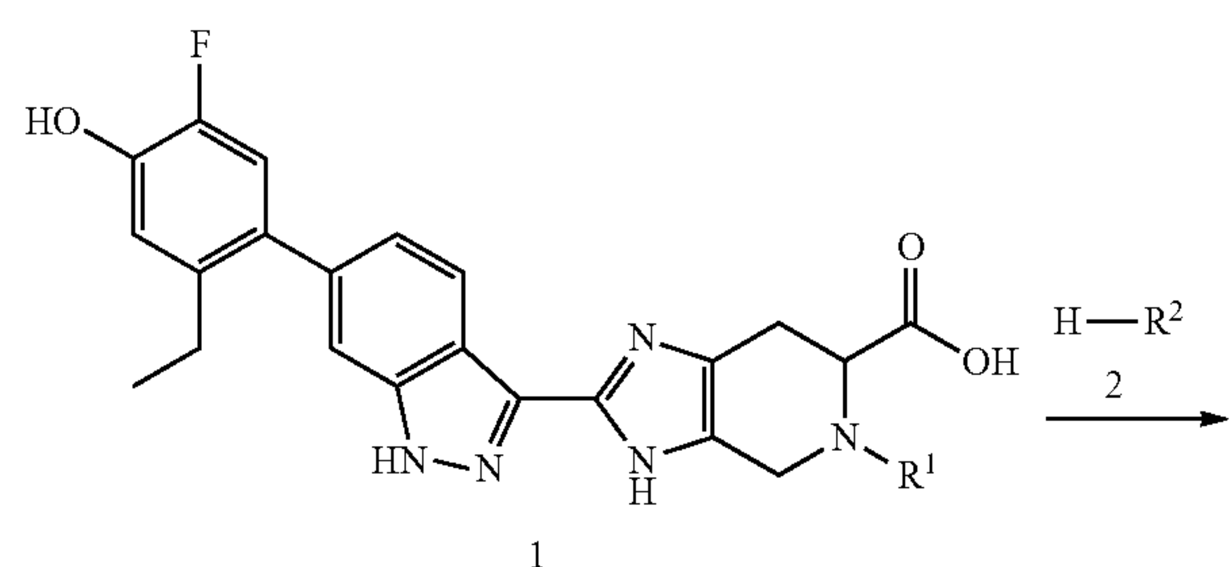
Scheme 1
