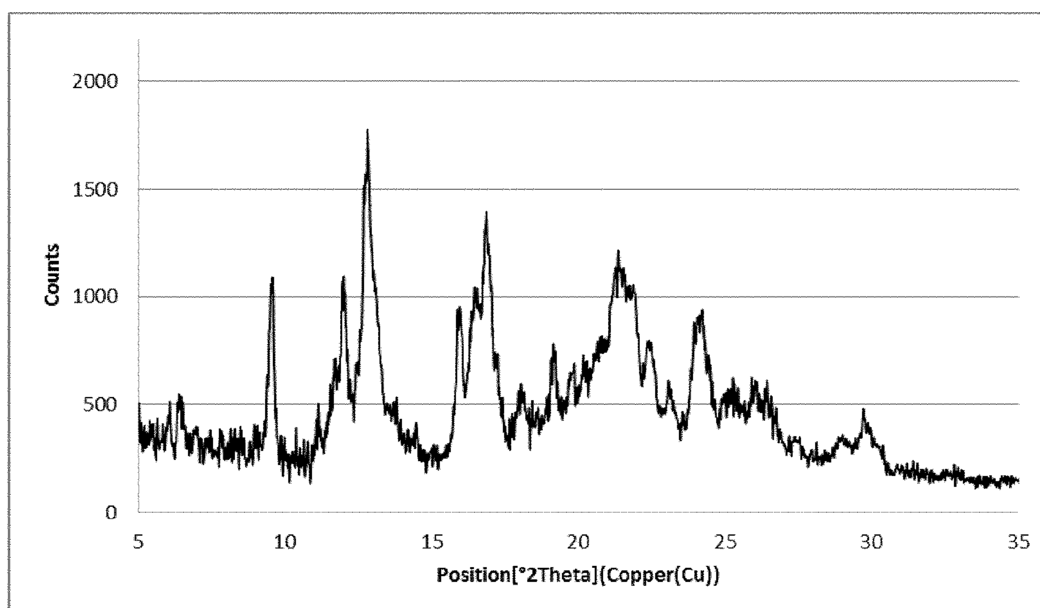
Figure 10. XRPD of (1R,2S)-(E)-2-(3-(4-((cis-2,6-dimethylmorpholino)methyl)styryl)-1H-indazol-6-yl)-5'-methoxyspiro[cyclopropane-1,3'-indolin]-2'-one fumarate form D
