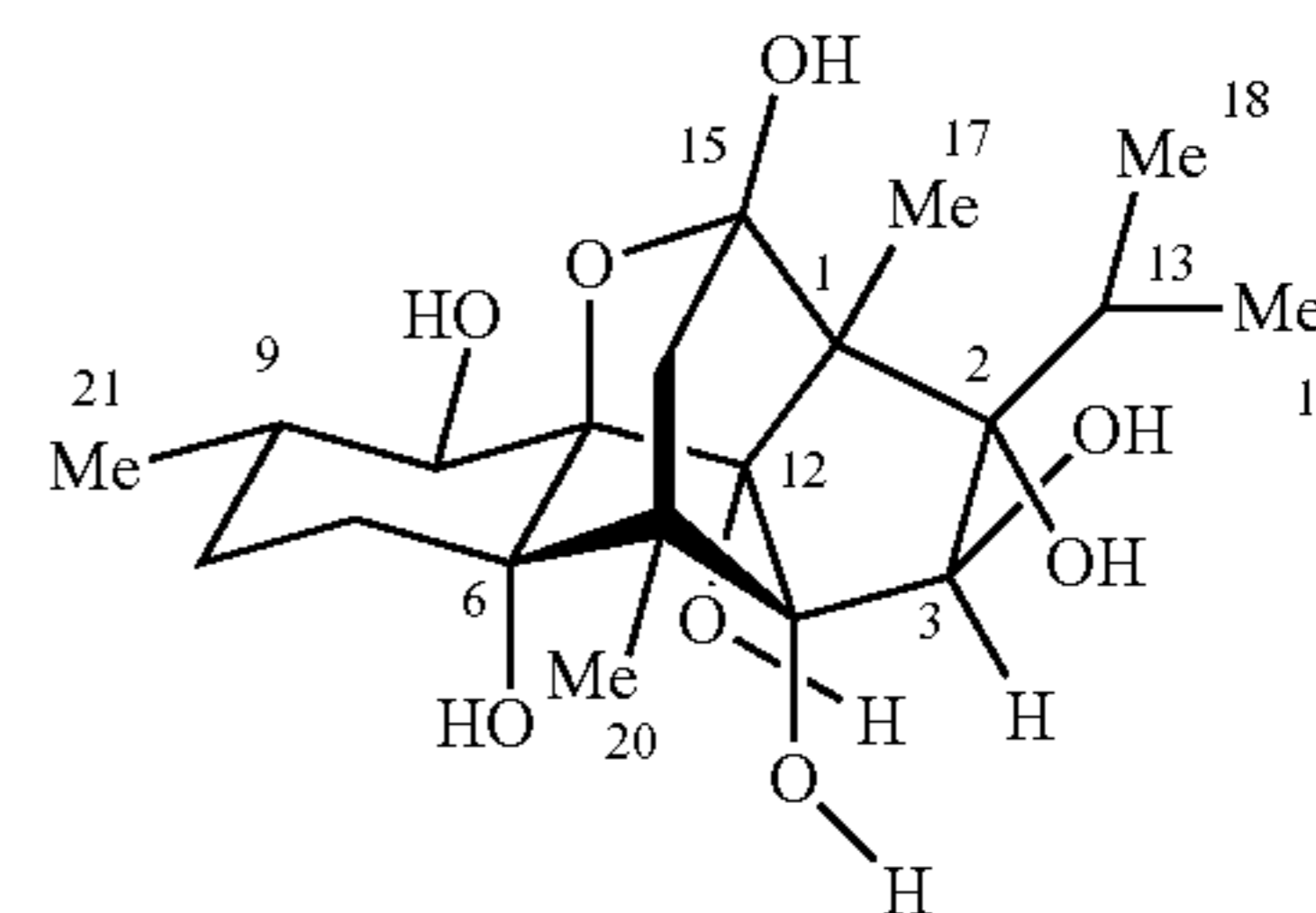
(+)-ryanodol (2)
