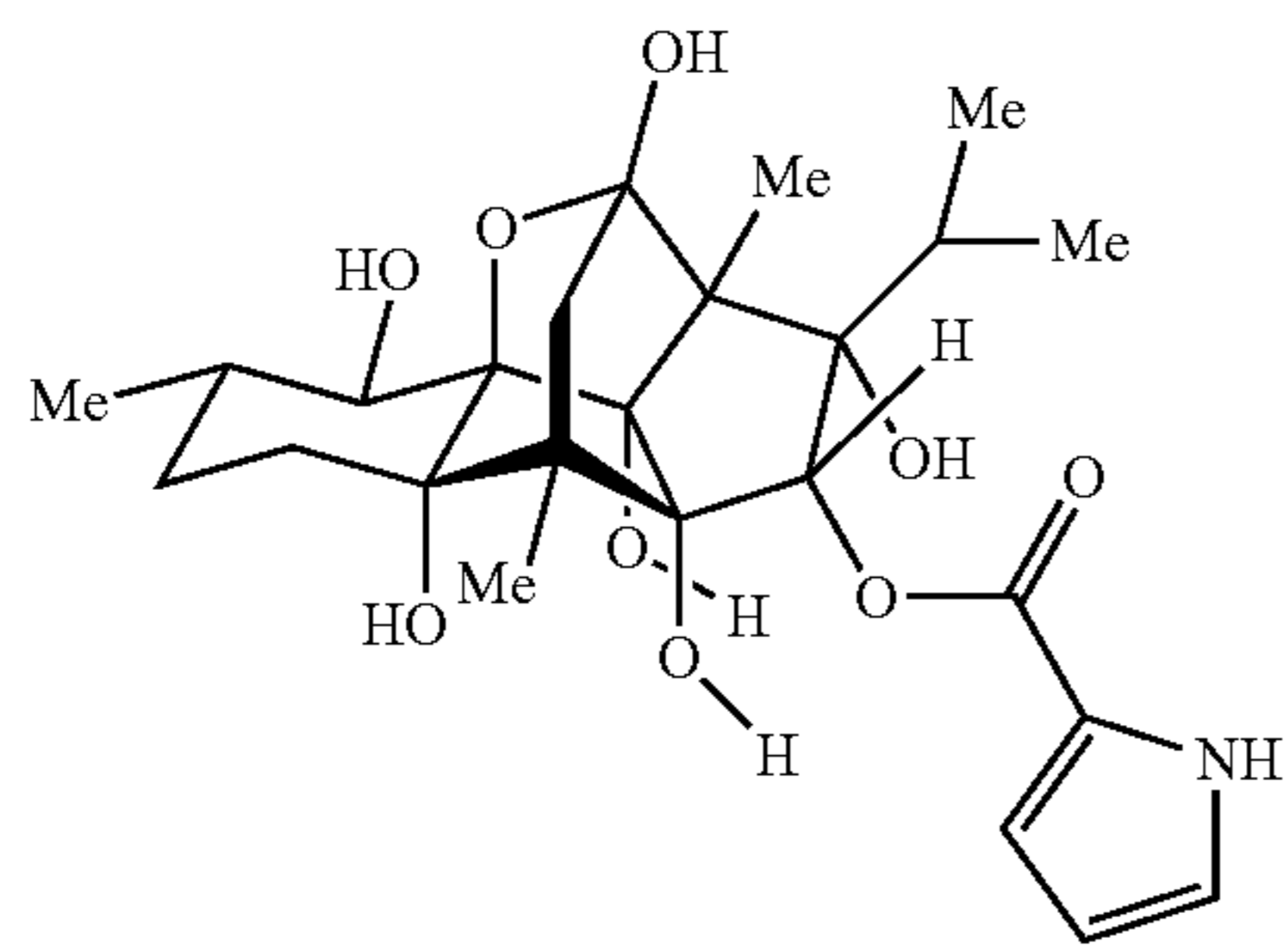
(+)-3-epi-ryanodine
