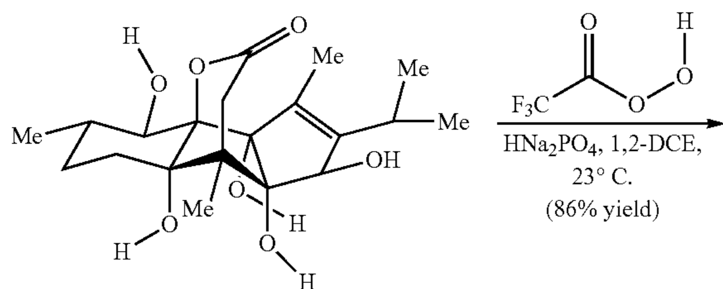
(+)-anhydroryanodol (3)
