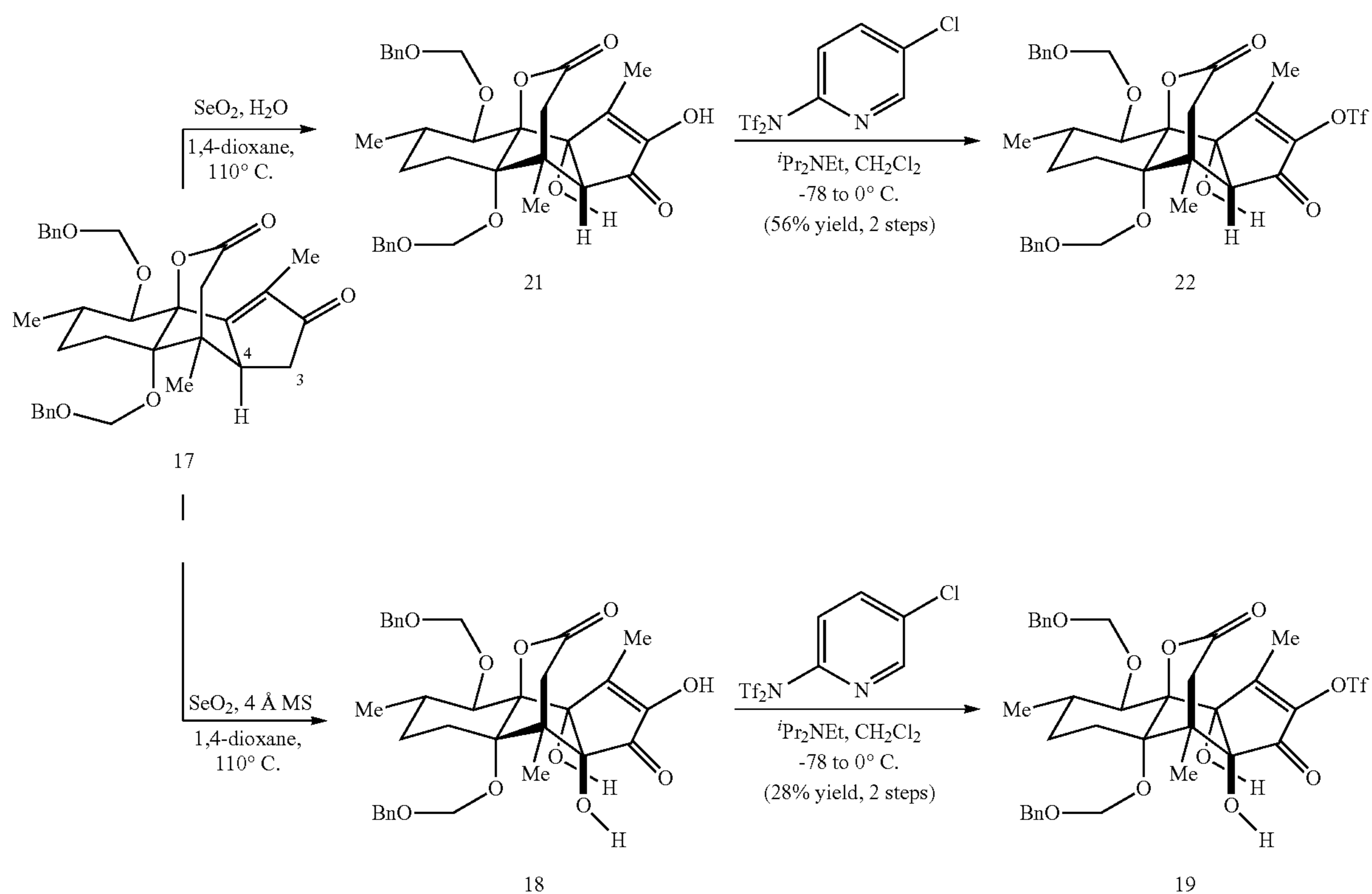
Scheme 5
