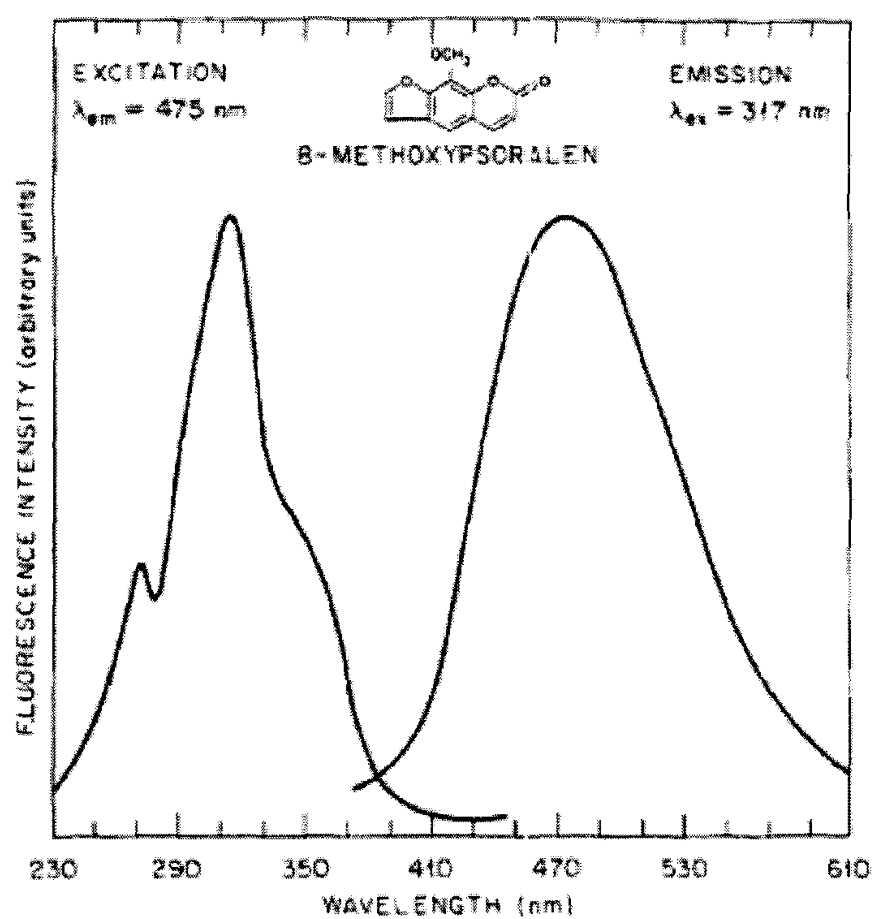
Figure 19. Excitation and Emission Fluorescence Spectra of Psoralens
