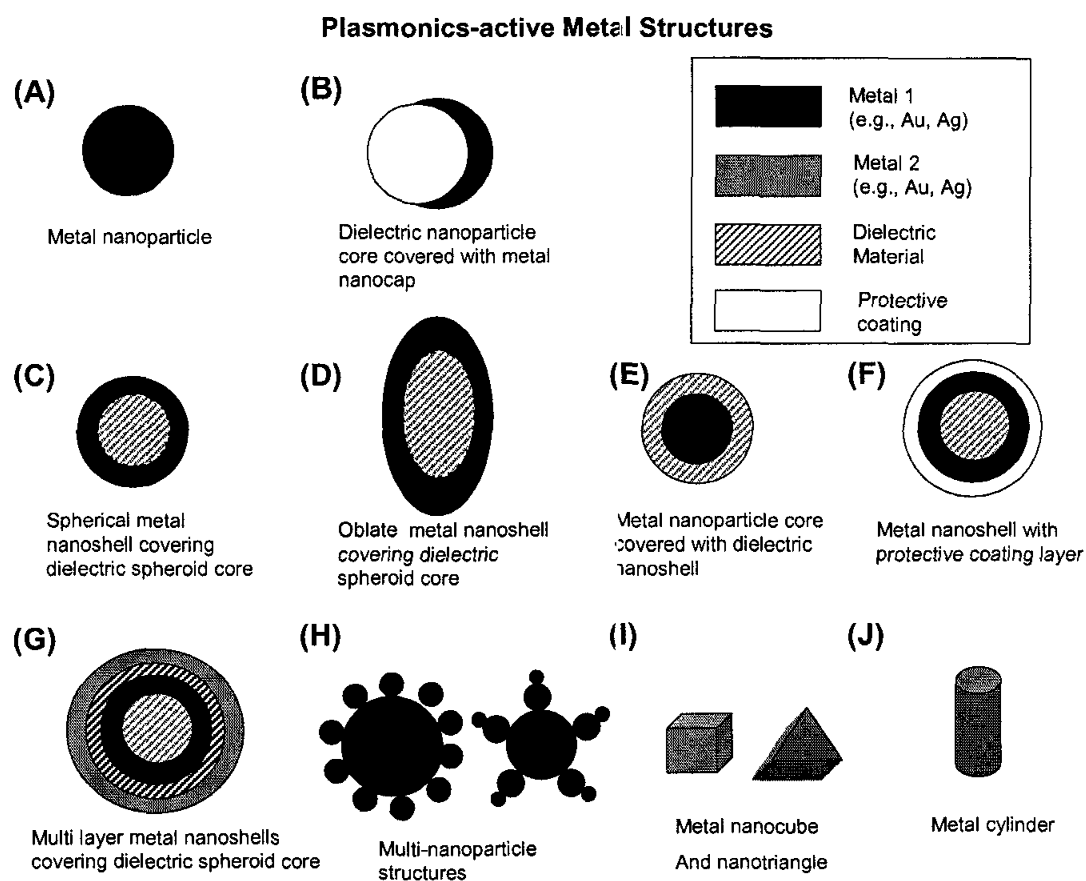
Figure 9. Plasmonics-active Nanostructures
