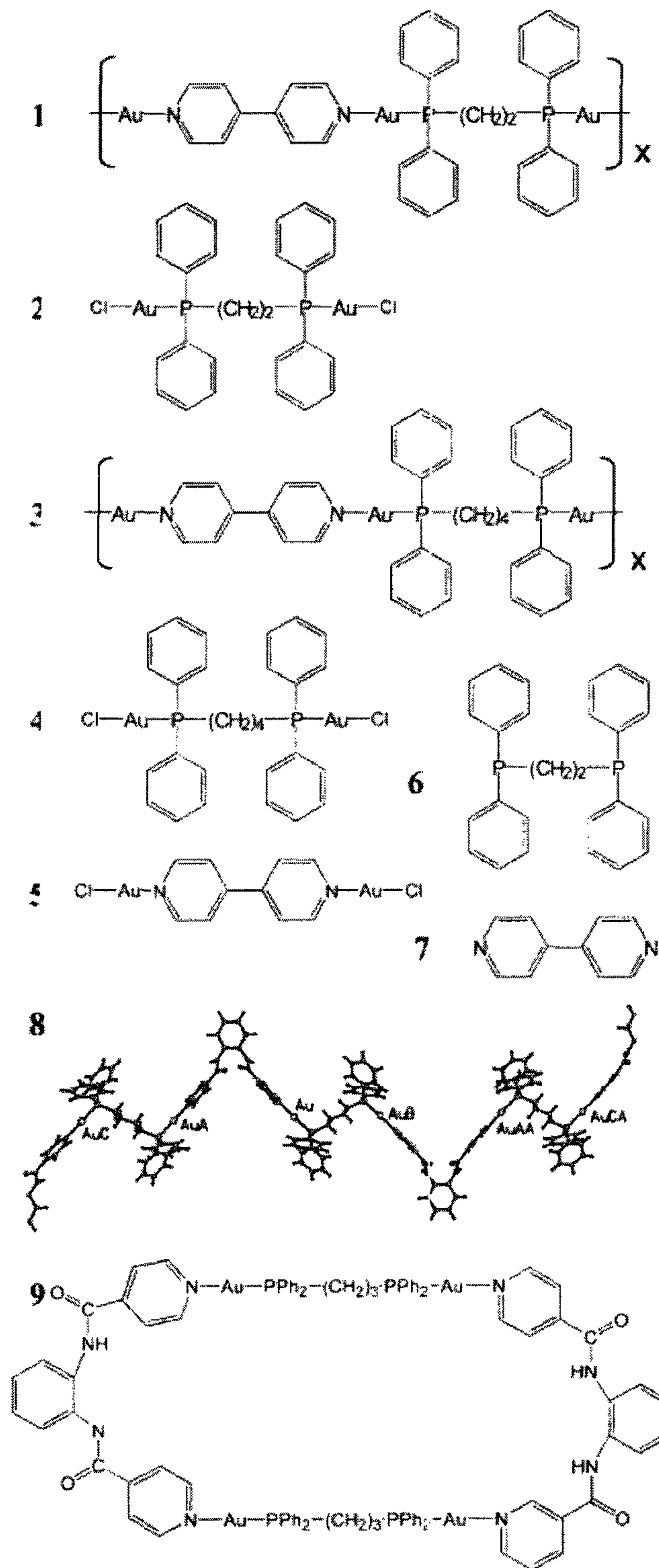
Figure 16. Gold complexes Exhibiting XEOL
