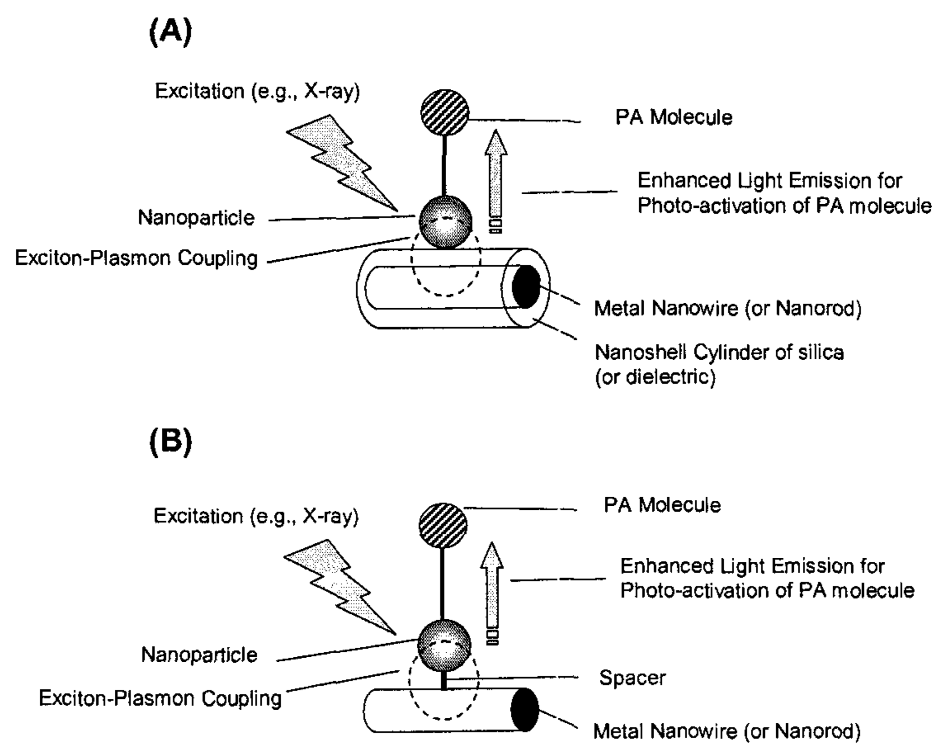
Exciton-Plasmon coupling Between Metal Nanorod and Nanoparticle
