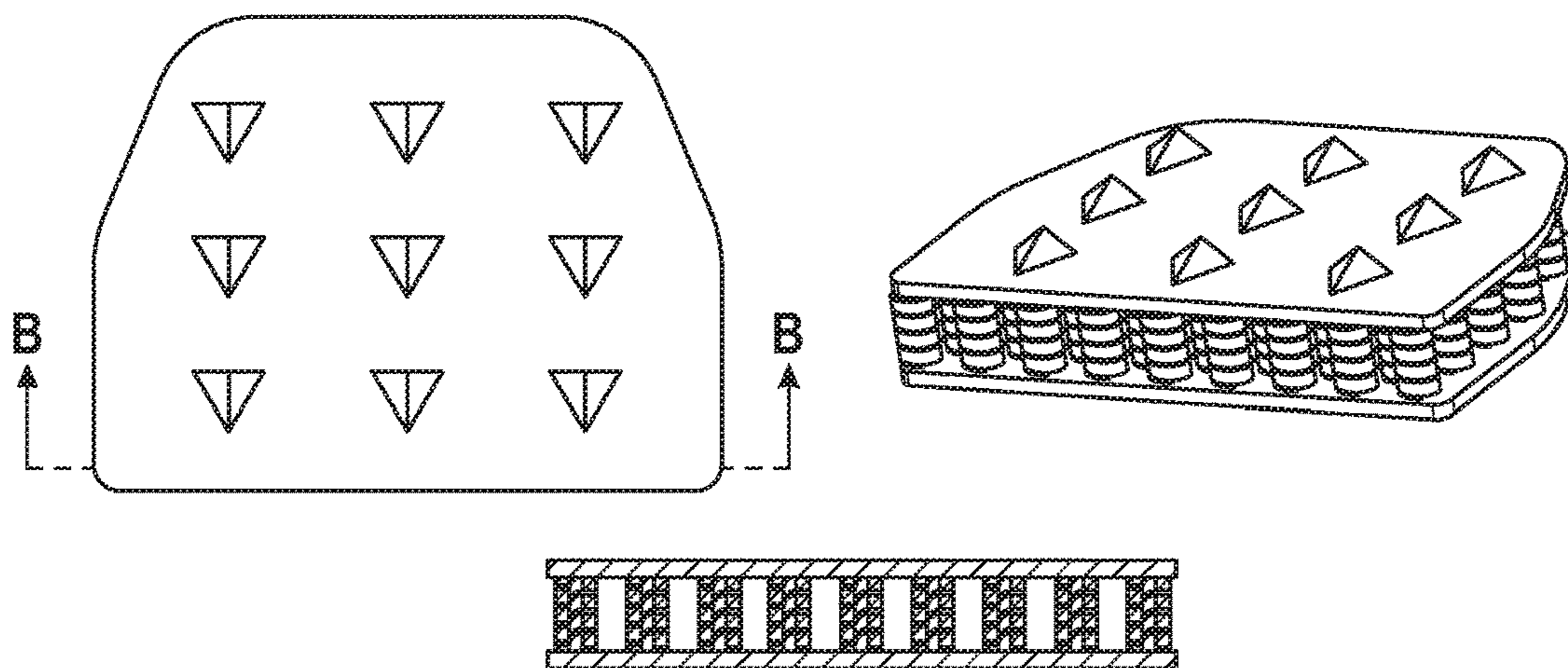
SECTION B-B
