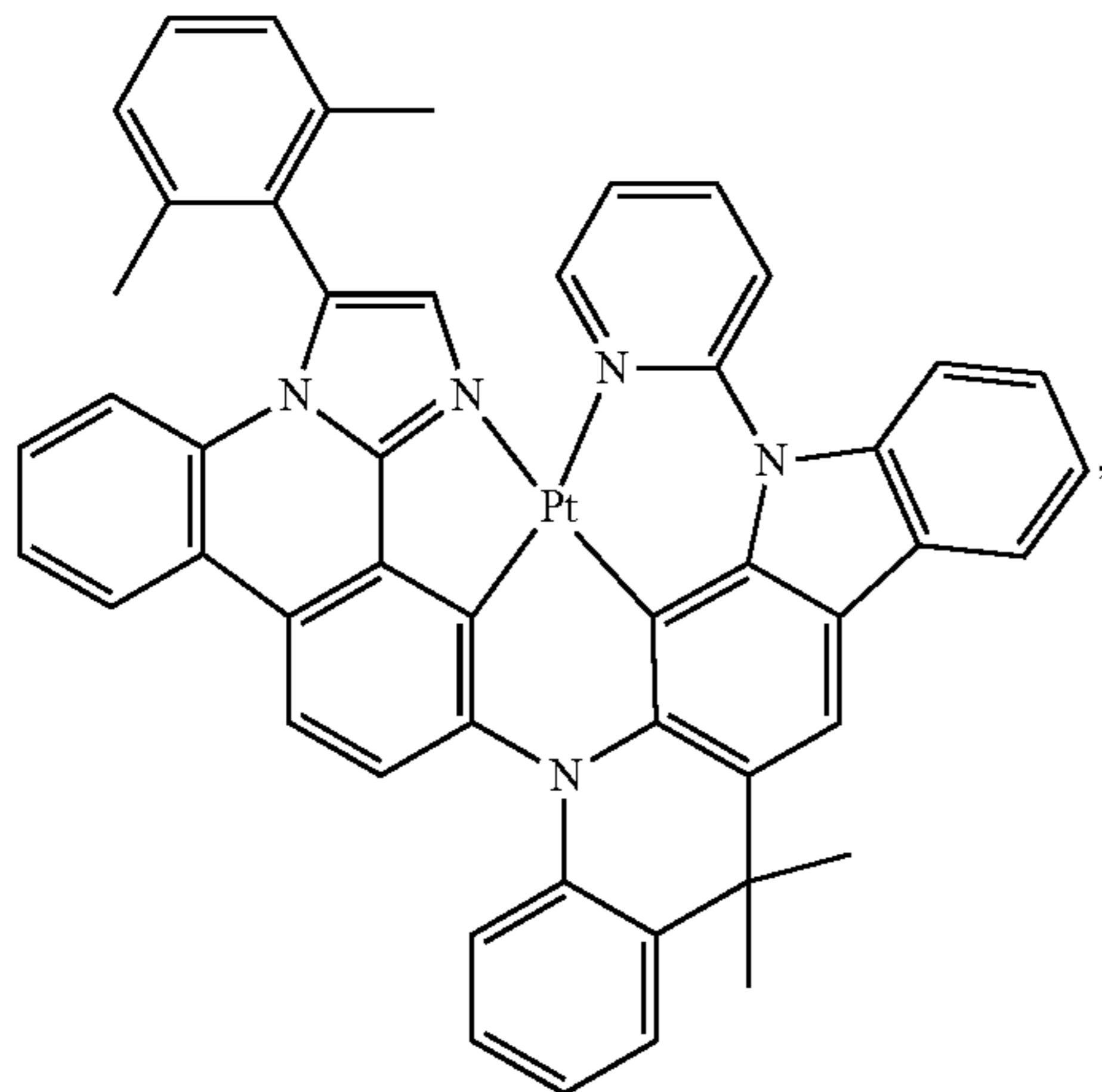
Compound 38
