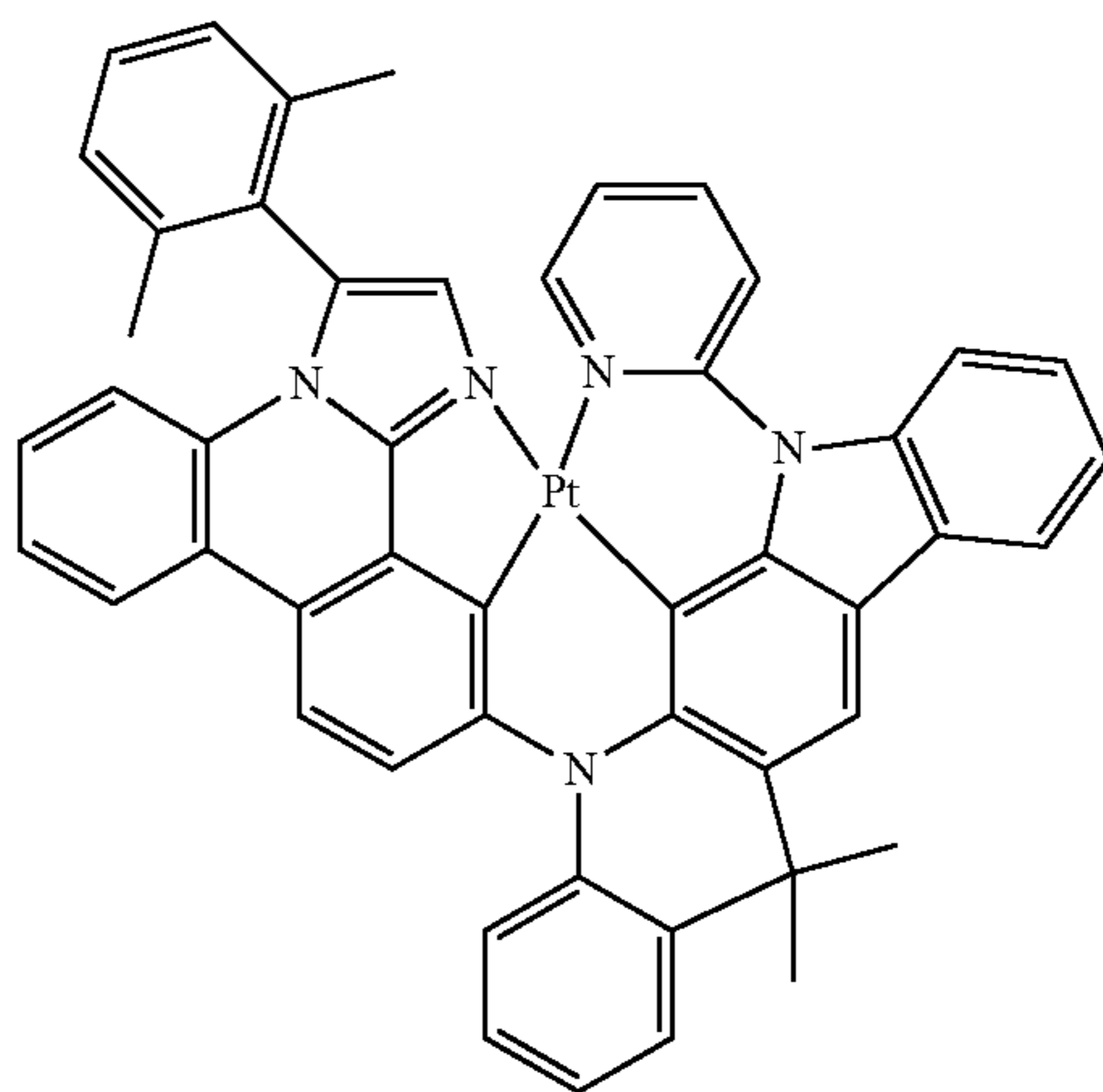
Compound 39
