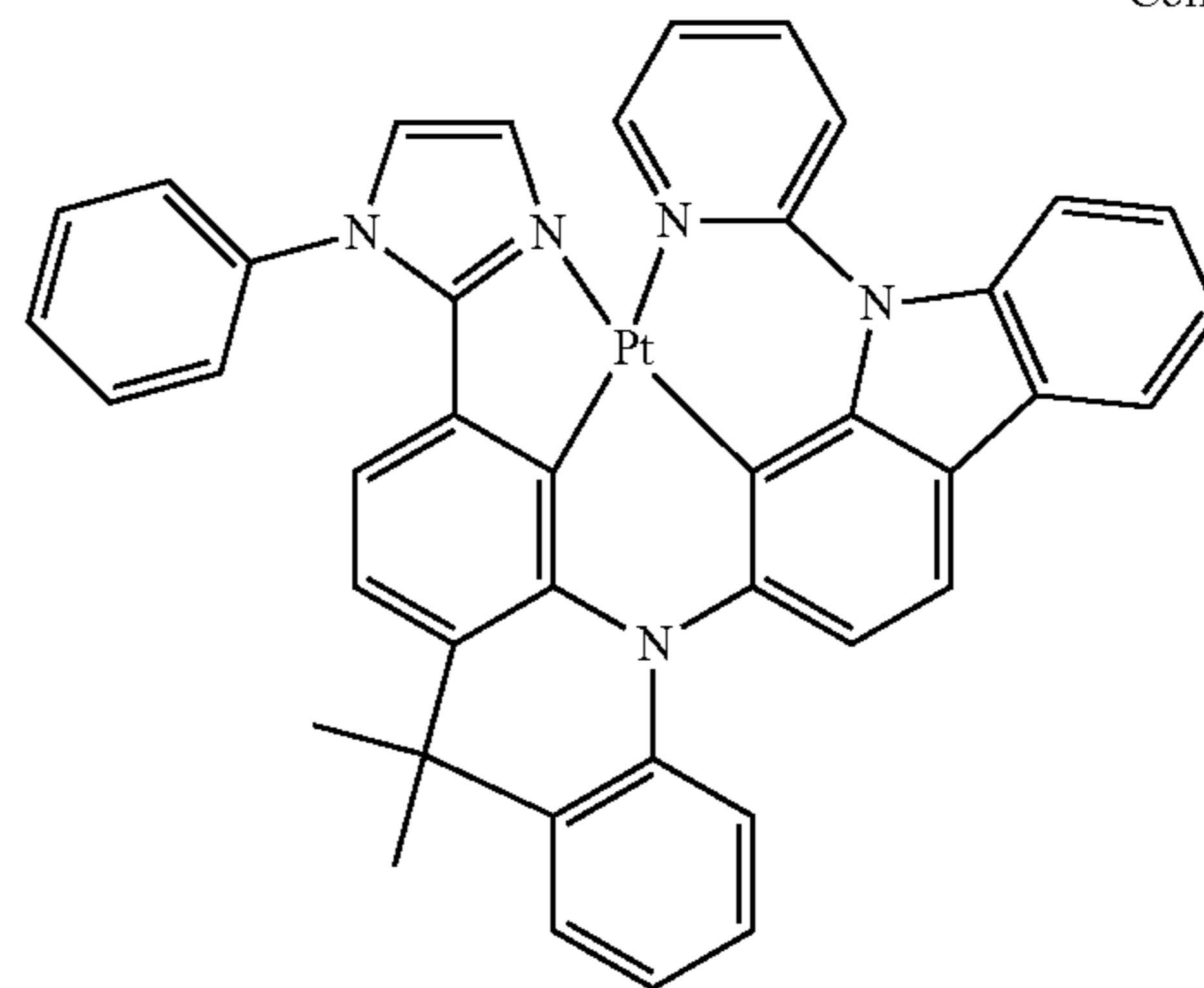
Compound 15
