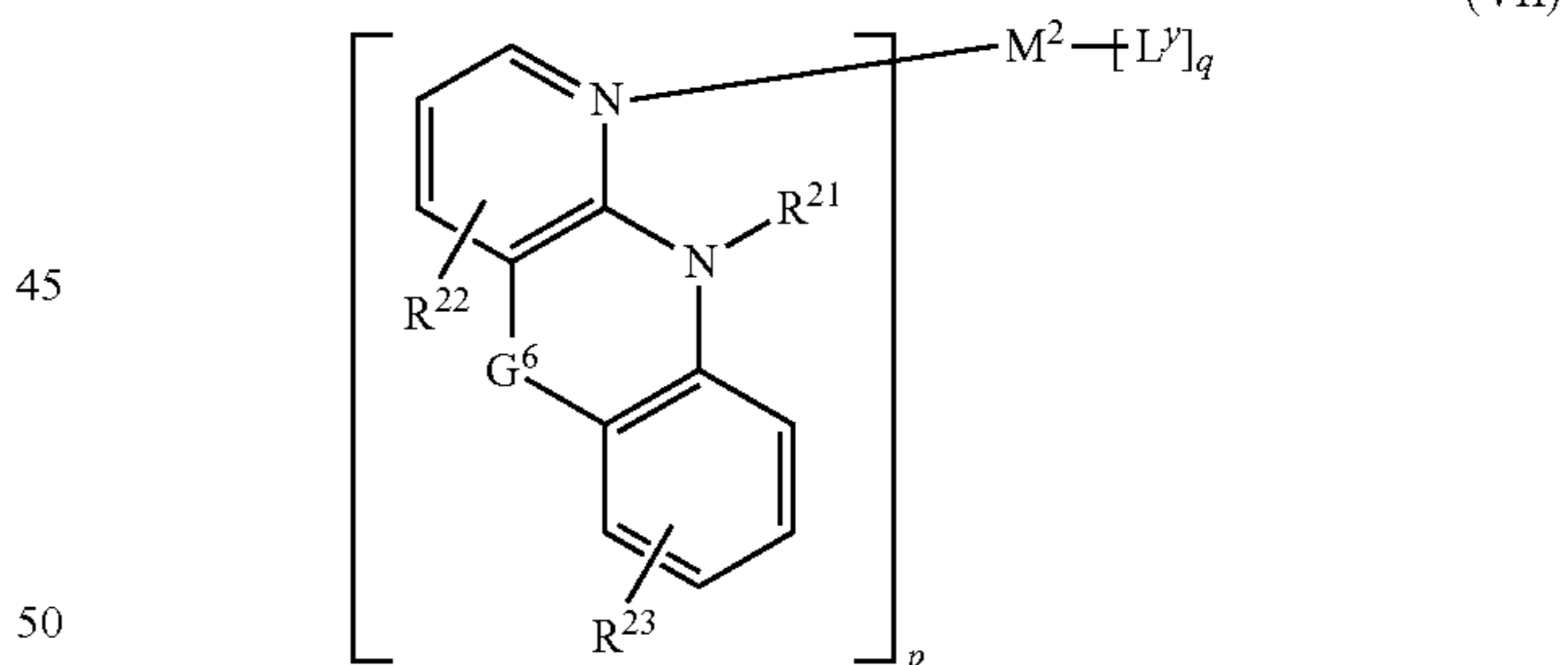
Compound 38
