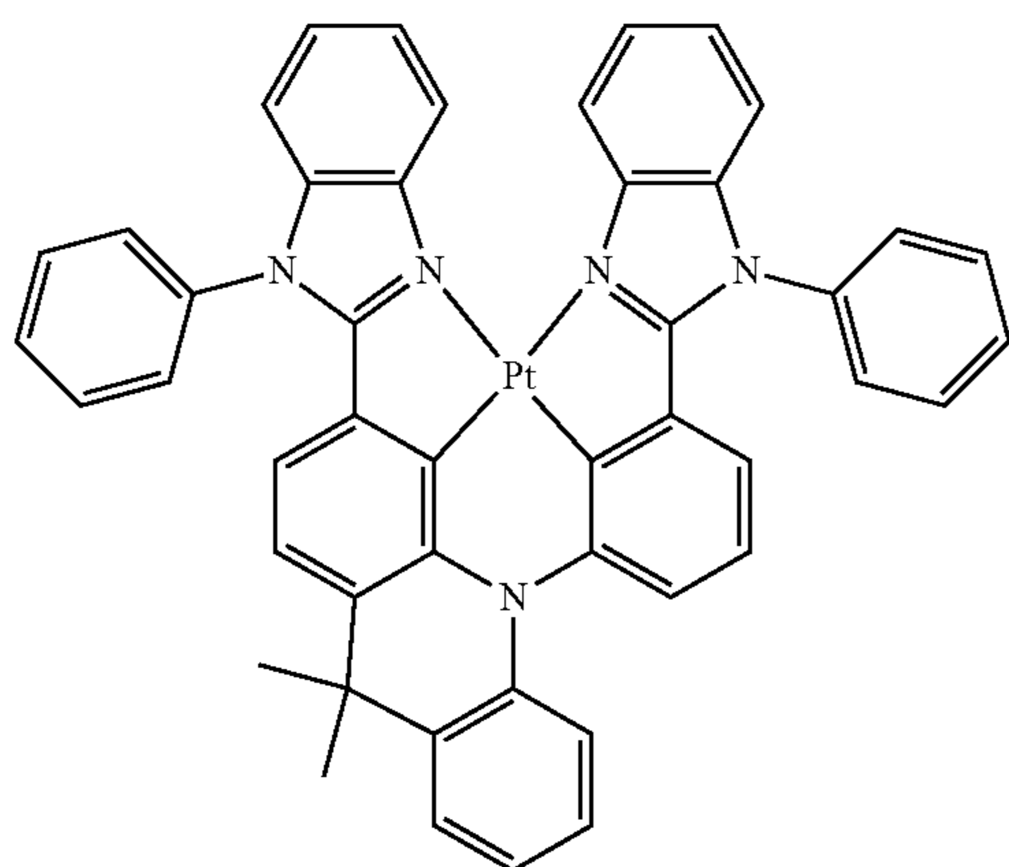
Compound 12
