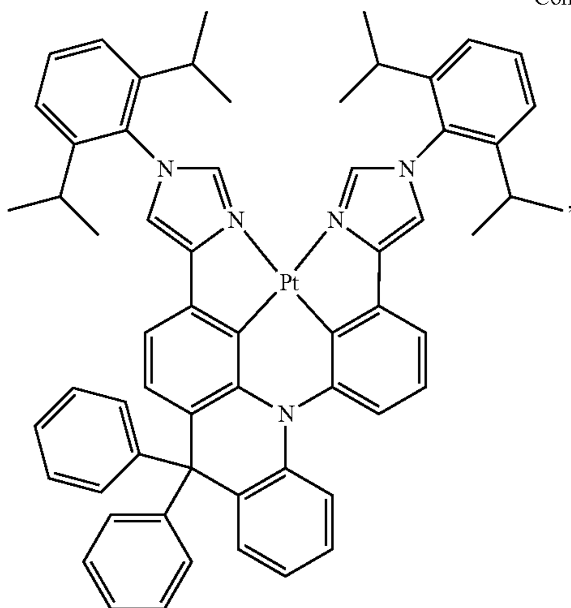
Compound 4
