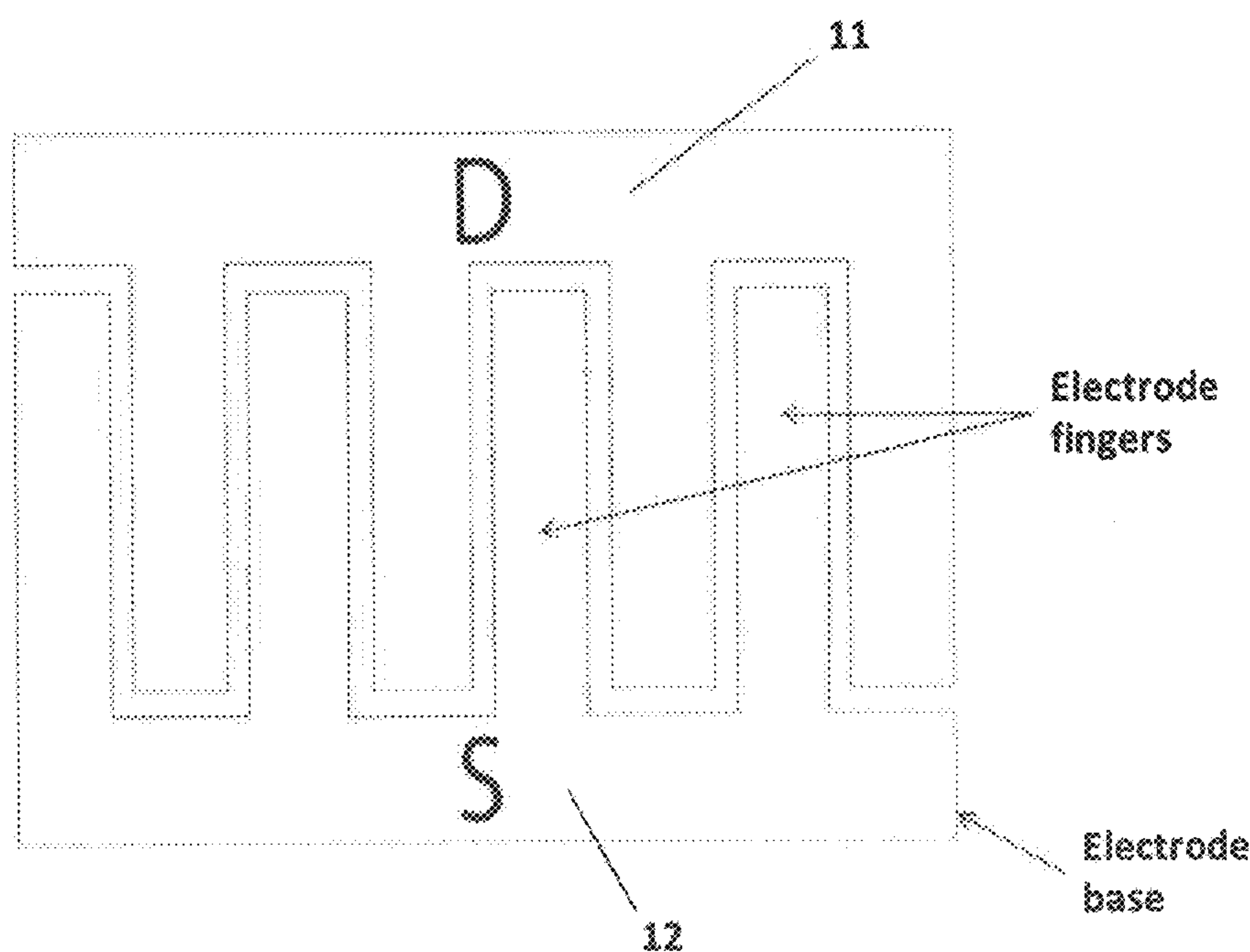
Fig. 1 (PRIOR ART)
