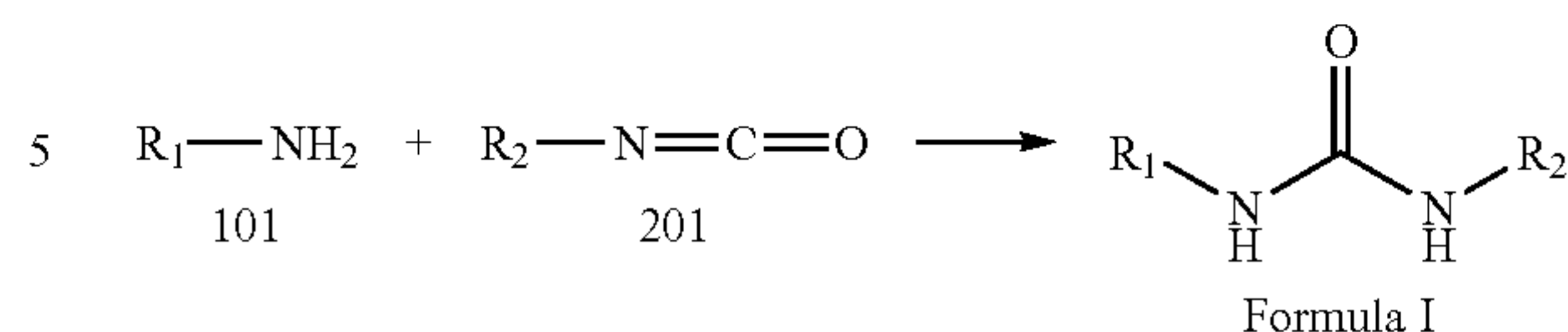
REACTION SCHEME 2
