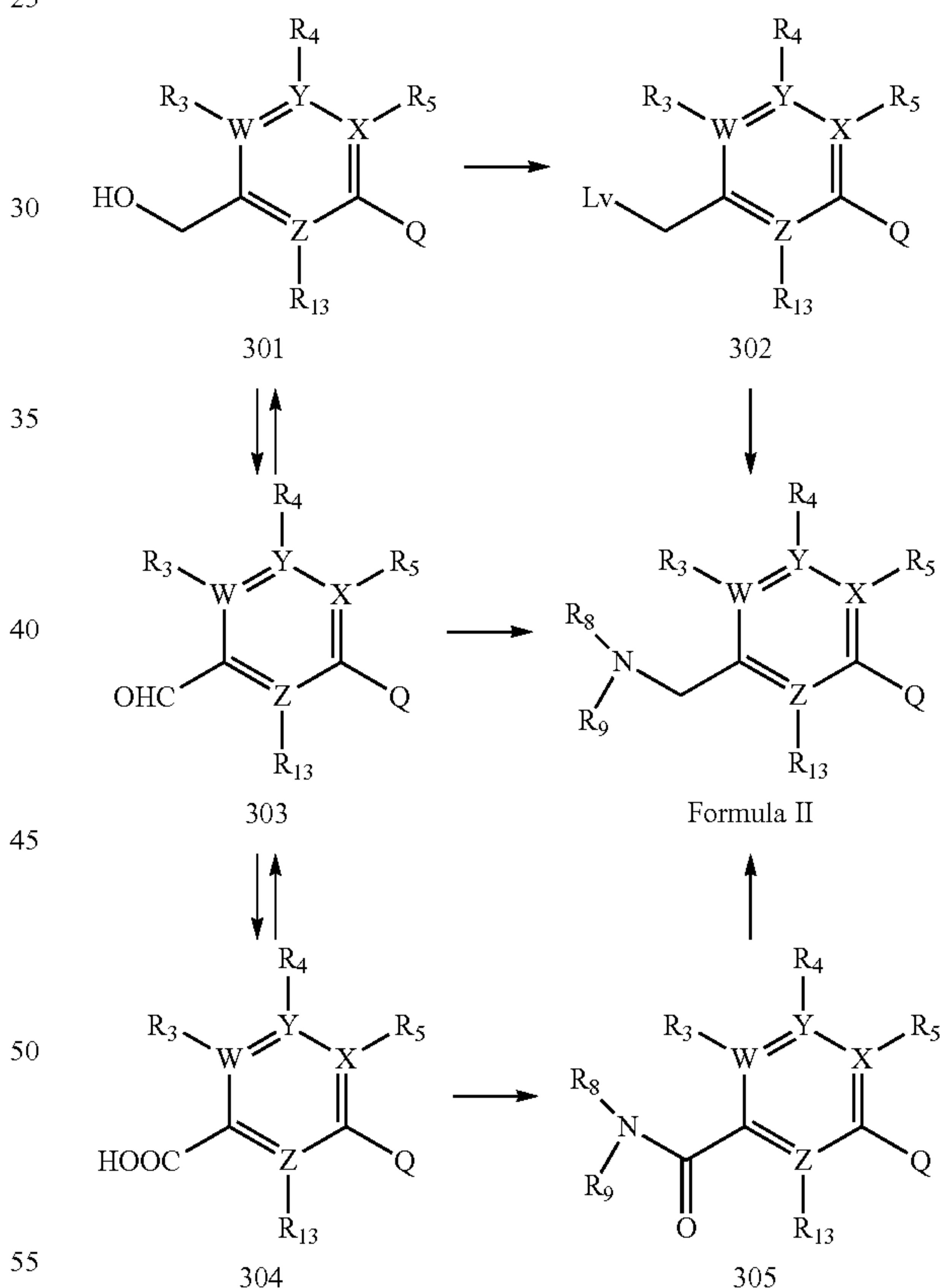
REACTION SCHEME 3
