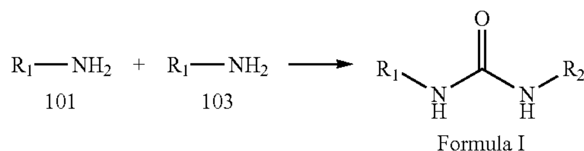
REACTION SCHEME 1
