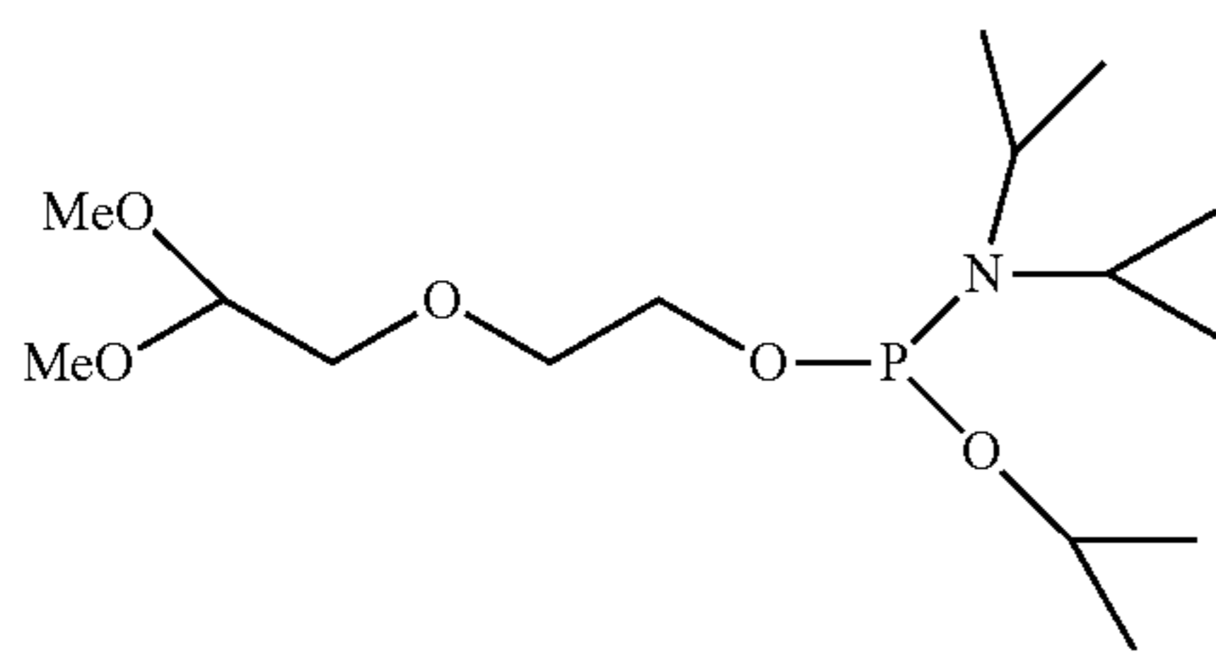
2-(2,2-Dimethoxy-ethoxy)-ethanol
