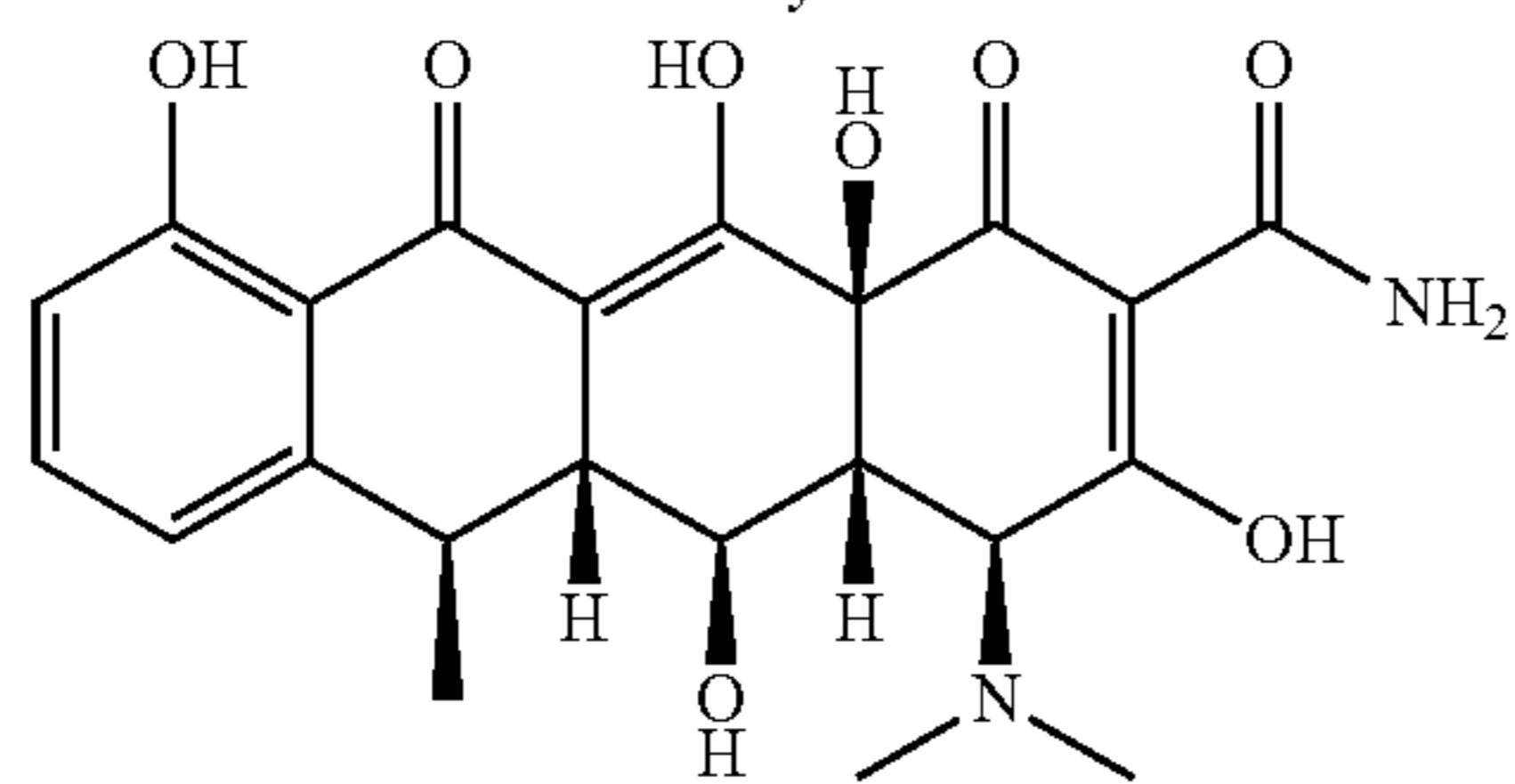
Doxycycline
