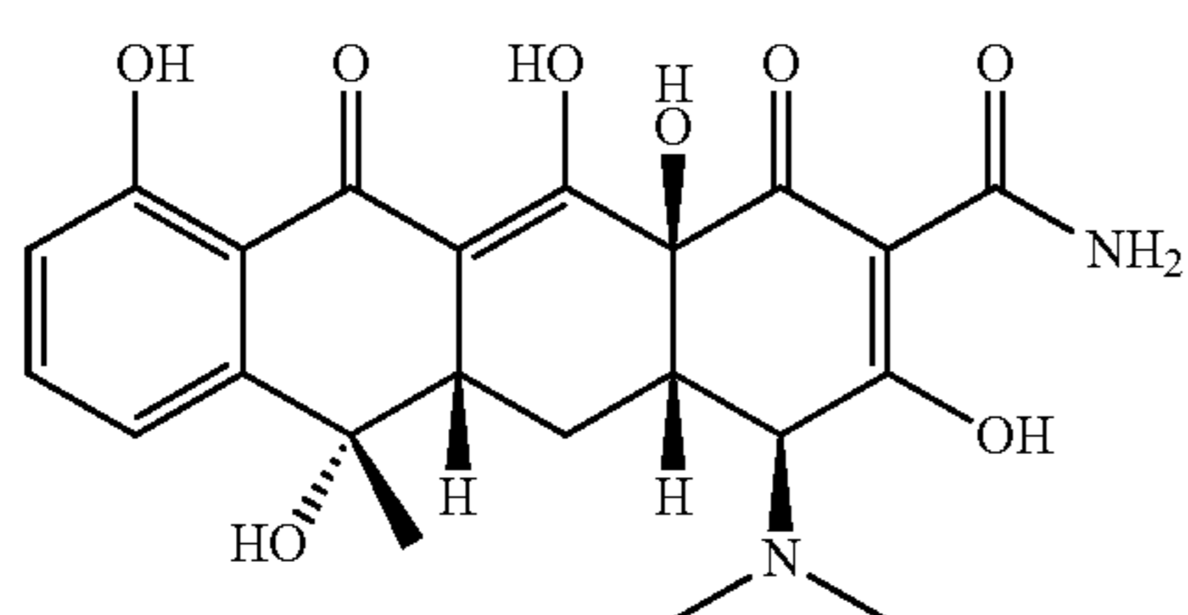
Tetracycline
